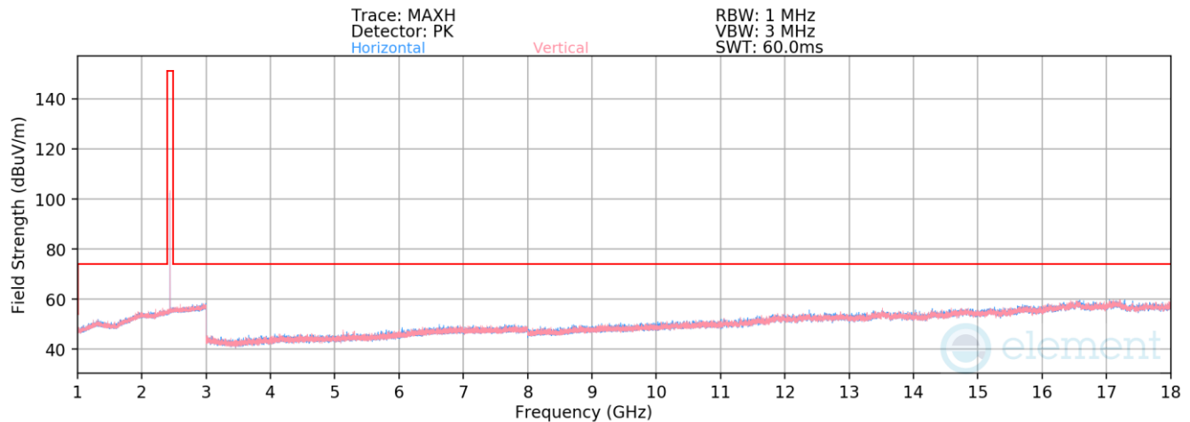
Plot 7-30. Radiated Spurious Emissions above 1GHz (BT GFSK ePA – Ch. 39)
