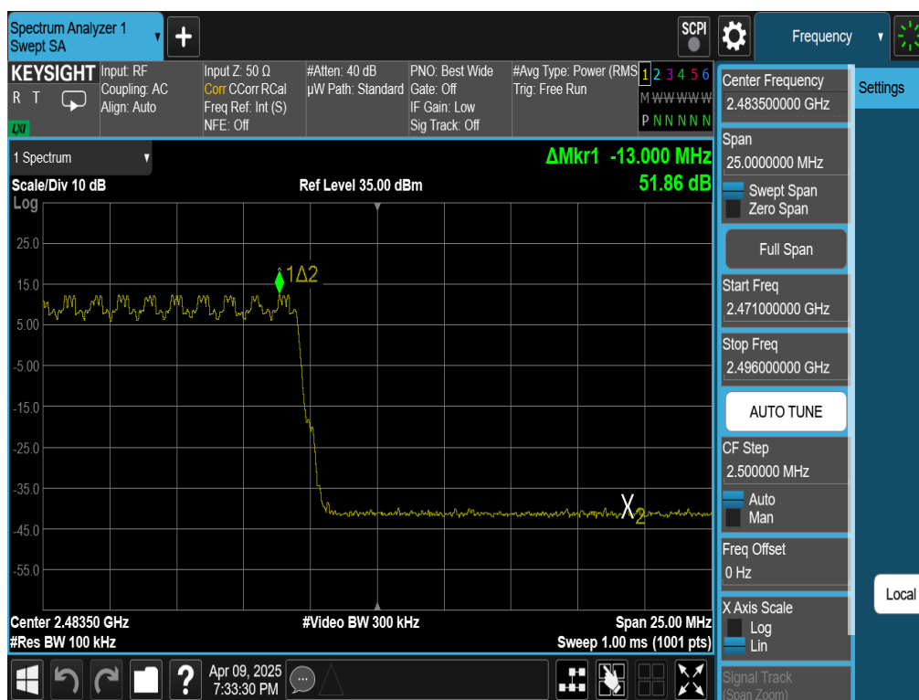
Plot 7-14. Band Edge Plot (Bluetooth with Hopping Enabled, 8DPSK, ePA)
