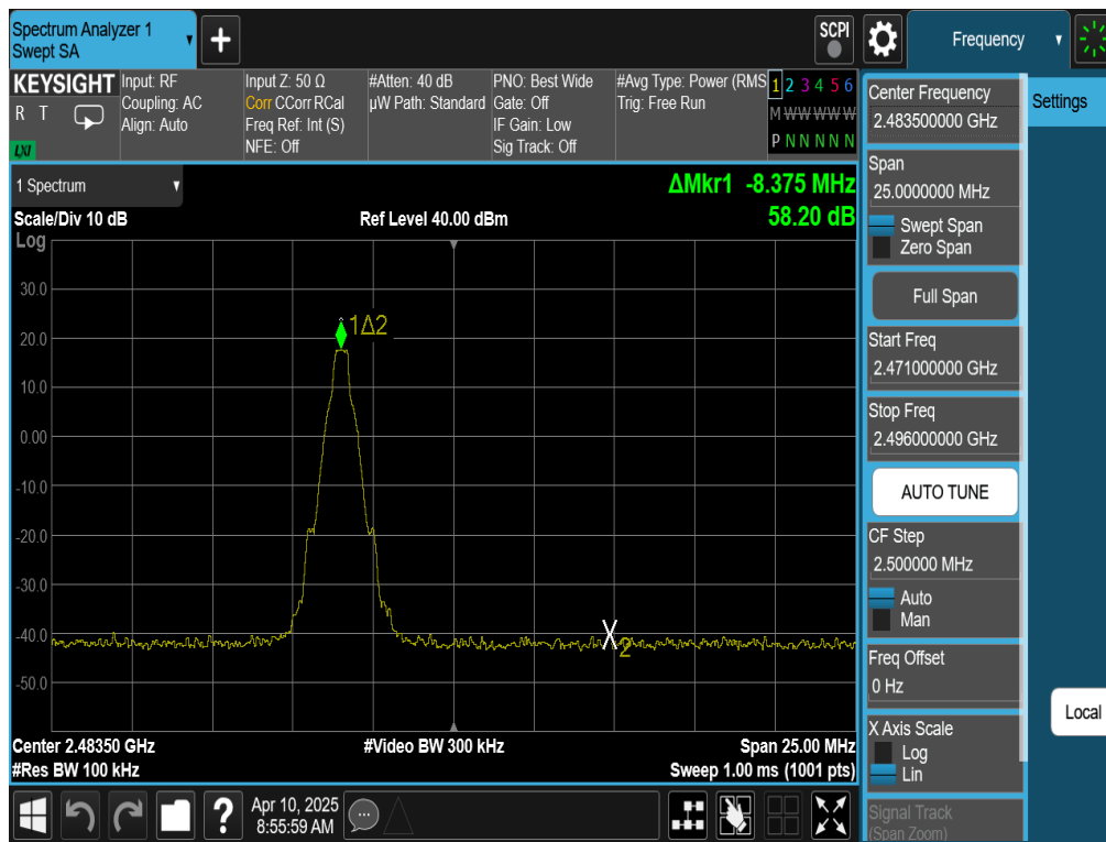
Plot 7-8. Band Edge Plot (Bluetooth with Hopping Disabled, GFSK, ePA – Ch. 78)
