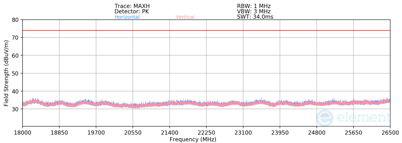
Plot 7-31. Radiated Spurious Emissions above 18GHz (GFSK ePA – Ch.39)
