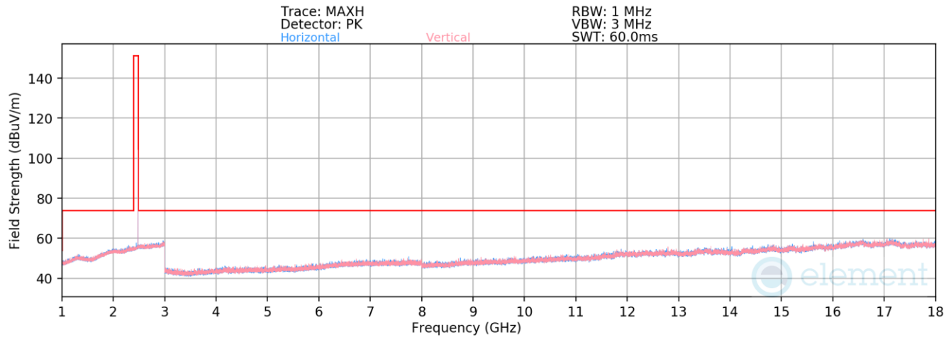
Plot 7-32. Radiated Spurious Emissions above 1GHz (BT GFSK ePA – Ch. 78)
