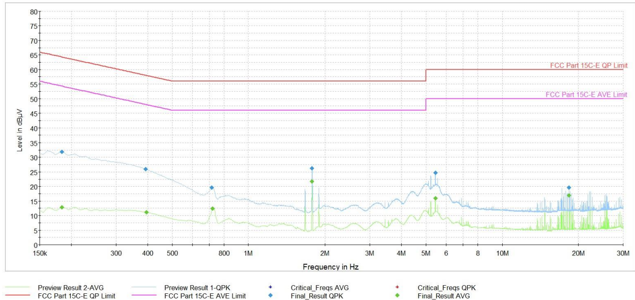
Plot 7-38. AC Line-Conducted Test Plot (L1, GFSK ePA – Ch.39, with AC/DC Adapter via USB-C cable with magnetic charger)
