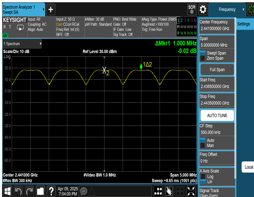
Plot 7-15. Channel Spacing Plot (Bluetooth, GFSK, ePA)
