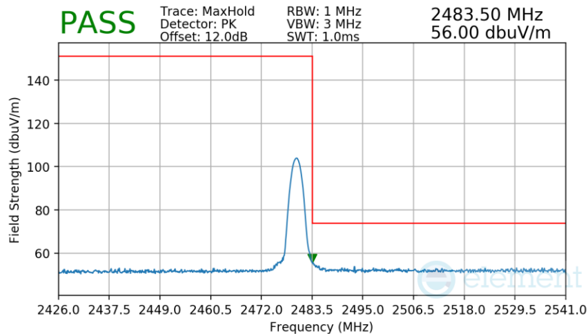
Plot 7-36. Radiated Restricted Upper Band Edge Measurement
