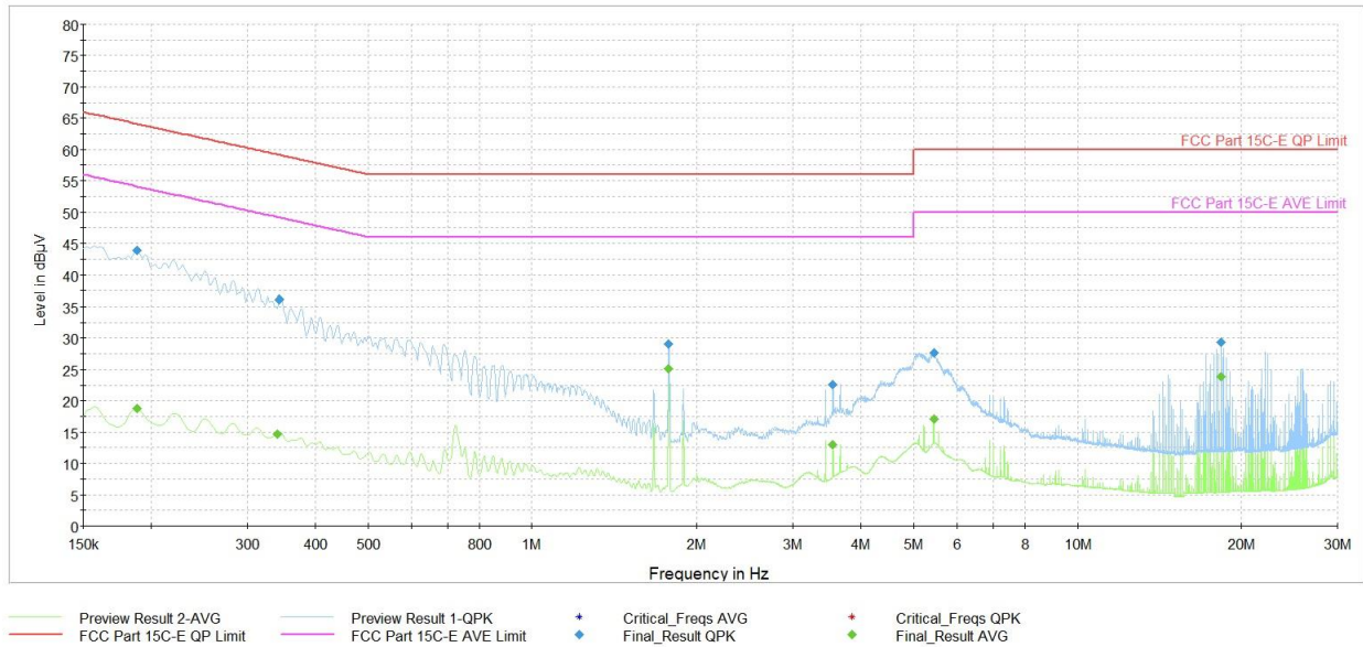
Plot 7-39. AC Line-Conducted Test Plot (N, GFSK ePA – Ch.39, with AC/DC Adapter via USB-C cable with magnetic charger)
