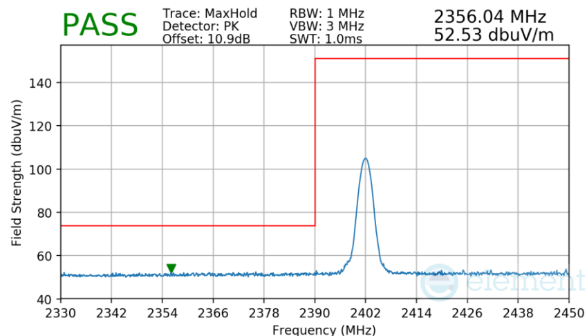
Plot 7-34. Radiated Restricted Lower Band Edge Measurement
