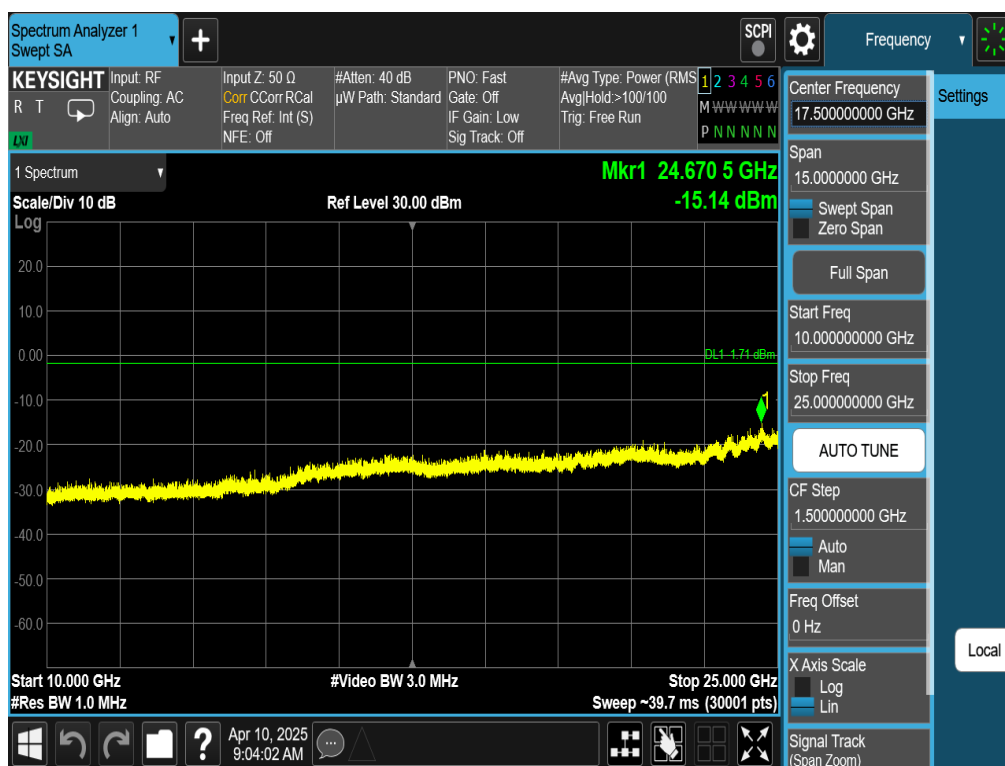
Plot 7-26. Conducted Spurious Plot (Bluetooth, GFSK, ePA Ch. 39)
