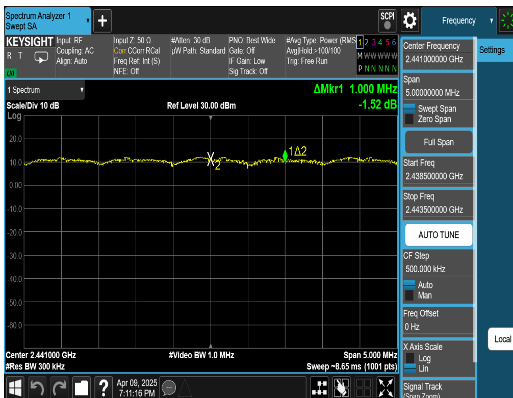
Plot 7-16. Channel Spacing Plot (Bluetooth, 8DPSK, ePA)
