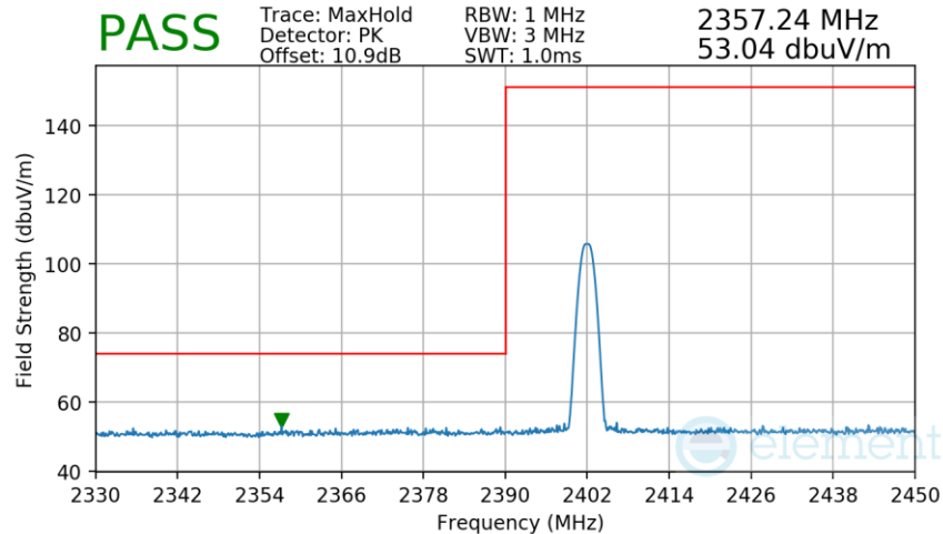
Plot 7-33. Radiated Restricted Lower Band Edge Measurement
