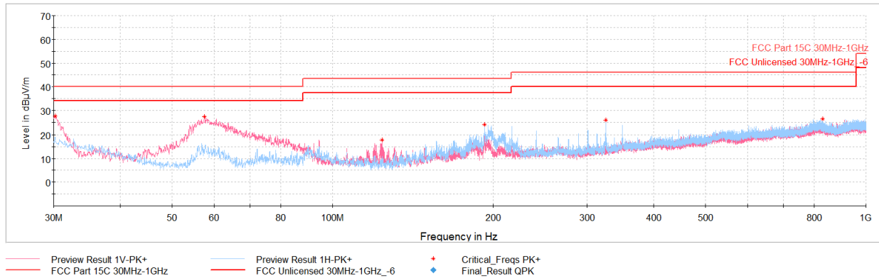
Plot 7-37. Radiated Spurious Emissions Below 1GHz (GFSK ePA – Ch.39, with AC/DC Adapter via USB-C cable with magnetic charger)
