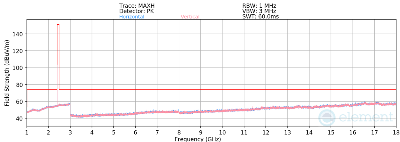
Plot 7-29. Radiated Spurious Emissions above 1GHz (BT GFSK ePA – Ch. 0)
