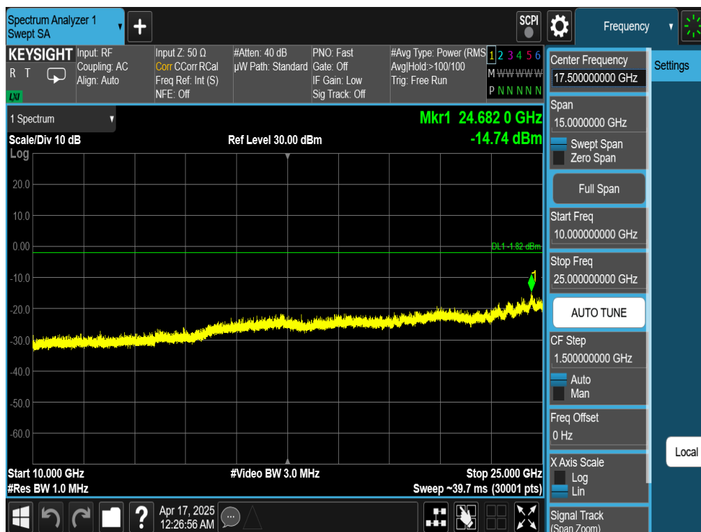
Plot 7-24. Conducted Spurious Plot (Bluetooth, GFSK, ePA – Ch. 0)
