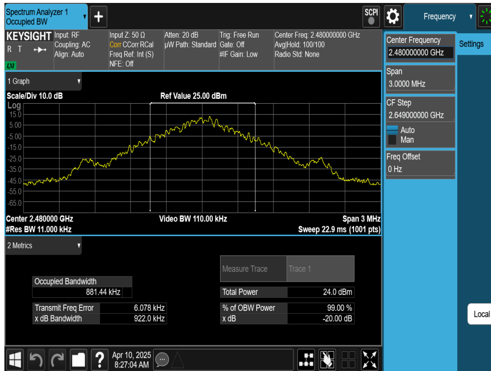
Plot 7-3. 20dB BW and 99% OBW Plot (Bluetooth, GFSK, ePA – Ch. 78)
