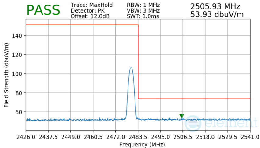
Plot 7-35. Radiated Restricted Upper Band Edge Measurement
