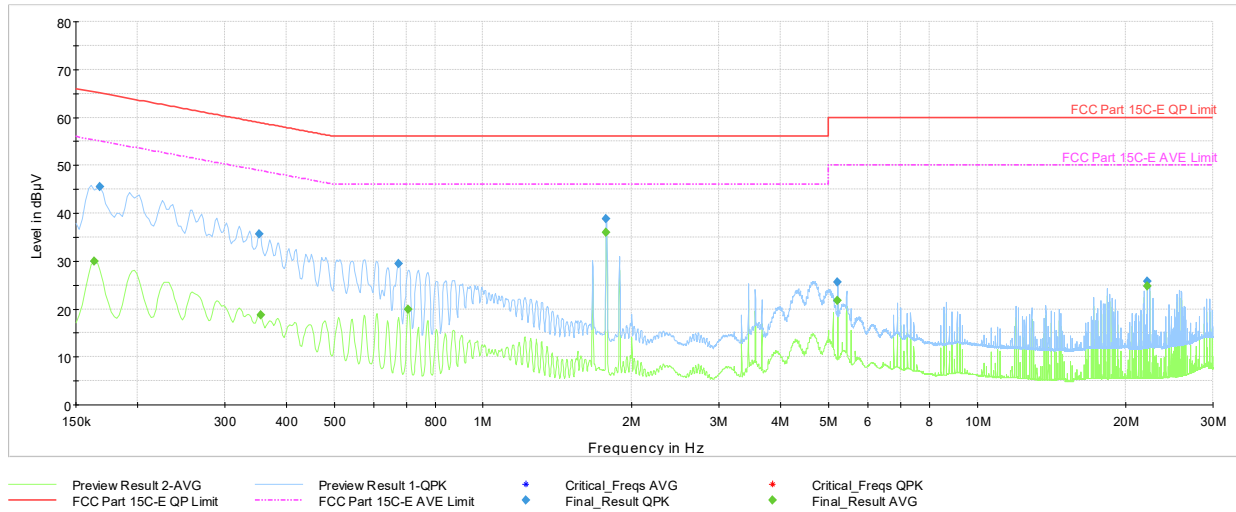
Plot 7-44. AC Line-Conducted Test Plot (N, GFSK ePA – Ch.39, with AC/DC Adapter + Magnetic Charger)
