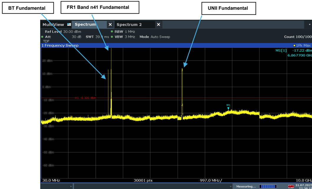
Plot 7-29. Conducted Simultaneous Tx Spurious Plot
