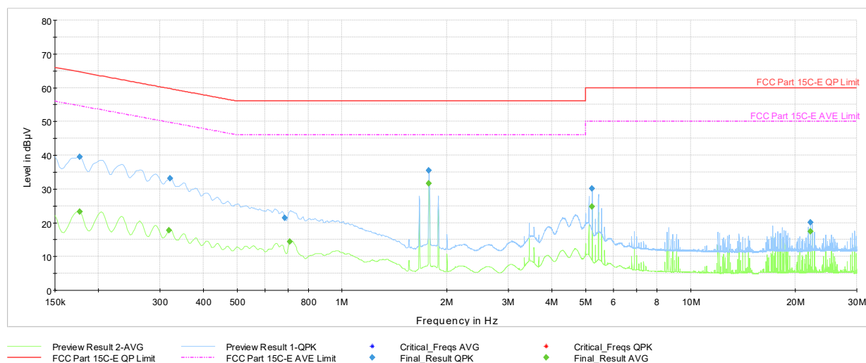
Plot 7-43. AC Line-Conducted Test Plot (L1, GFSK ePA – Ch.39, with AC/DC Adapter + Magnetic Charger)
