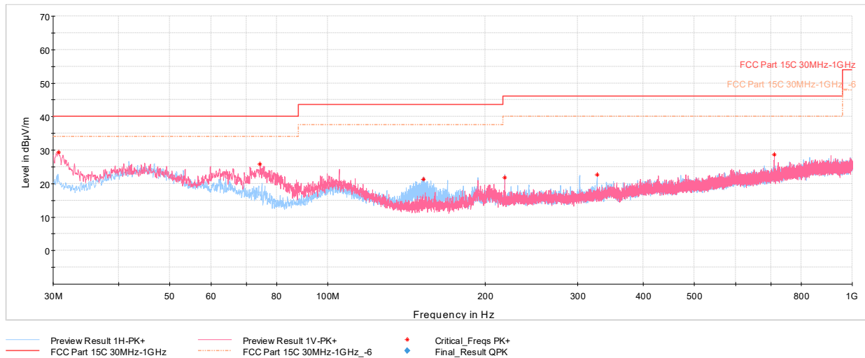
Plot 7-41. Radiated Spurious Emissions Below 1GHz (GFSK ePA – Ch.39, with AC/DC Adapter & Magnetic Charger)
