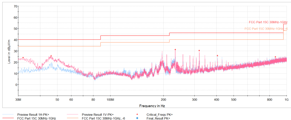
Plot 7-31. Radiated Spurious Emissions Below 1GHz (1Mbps, iPA – Ch.39, Pol. H & V, with AC/DC adaptor with USB-C cable)
