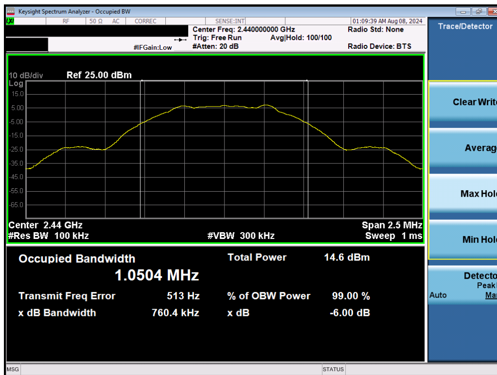
Plot 7-2. 6dB BW & 99% OBW Plot (Bluetooth (LE), 1Mbps, iPA – Ch. 19)
