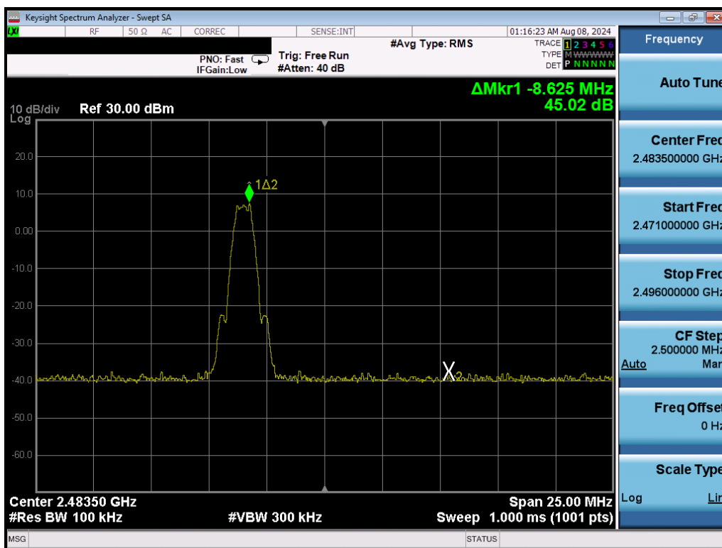
Plot 7-14. Band Edge Plot (Bluetooth (LE), 1Mbps, iPA – Ch. 39)
