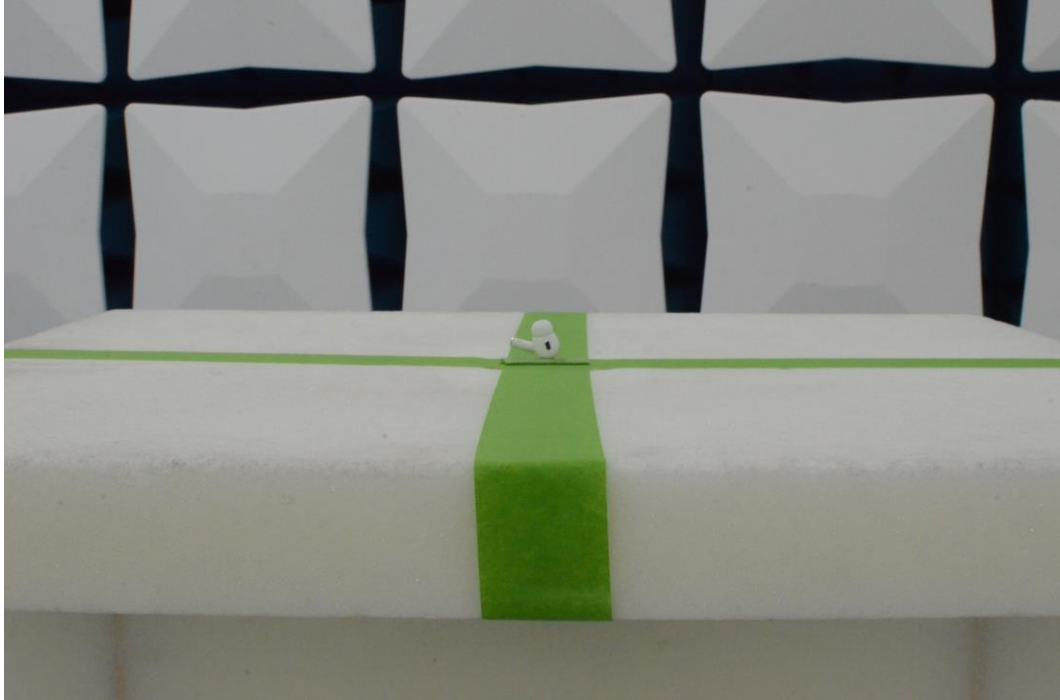
Figure 9: 1-18GHz Test Setup (Front View)
