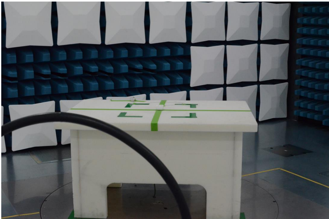
Figure 24: 9kHz-30MHz Test Setup (Front View)
