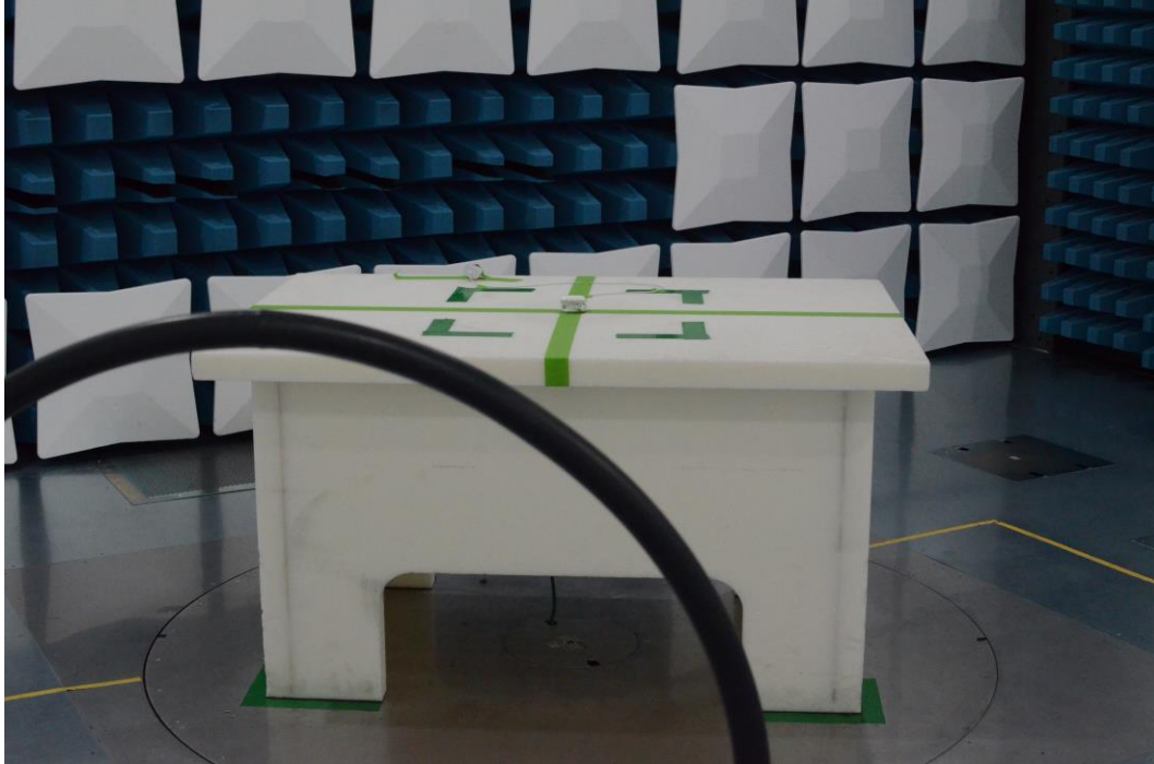
Figure 23: 9kHz-30MHz Test Setup (Front View)
