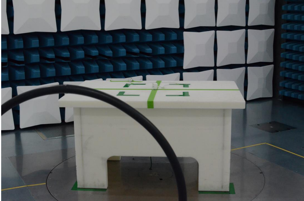
Figure 25: 9kHz-30MHz Test Setup (Front View)
