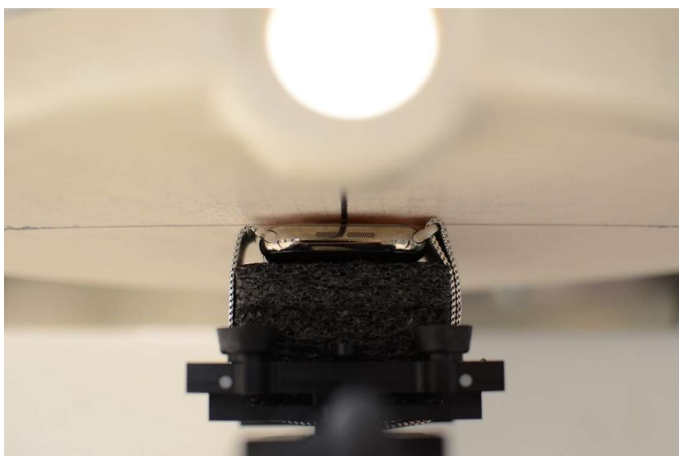
SAR Test Setup Photo 12 – Titanium with Metal Loop Wristband, Extremity, Back Side at 0mm
