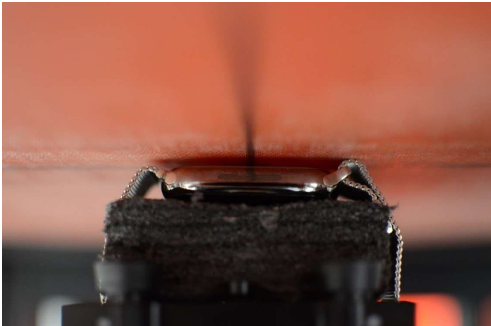
NFC Test Setup Photo 18 – Titanium with Metal Loop Wristband, Extremity, Back Side at 0mm
