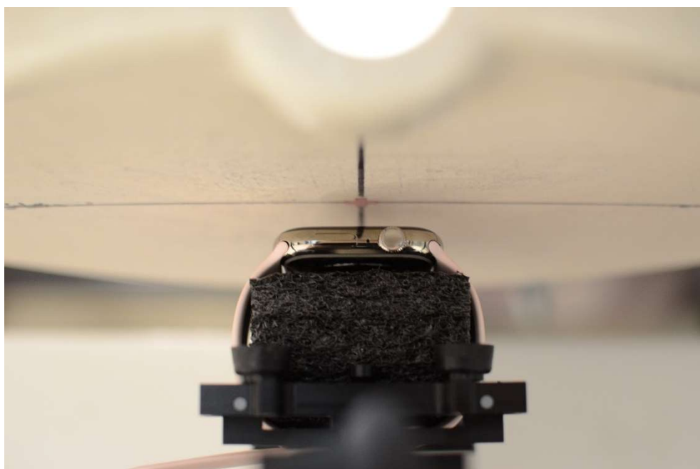
SAR Test Setup Photo 4 –Titanium with Sport Wristband, Head, Front side at 10 mm
