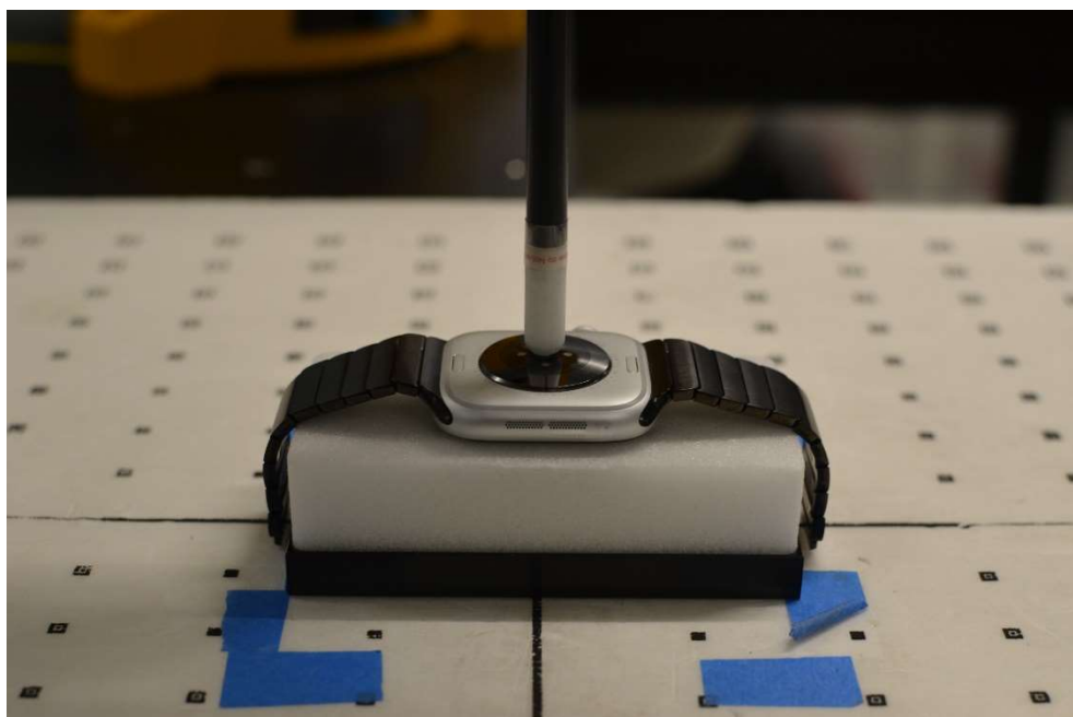
Near Field Power Density Test Setup Photo 20 – Aluminum with Metal Links Wristband, Extremity, Back side at 2mm
