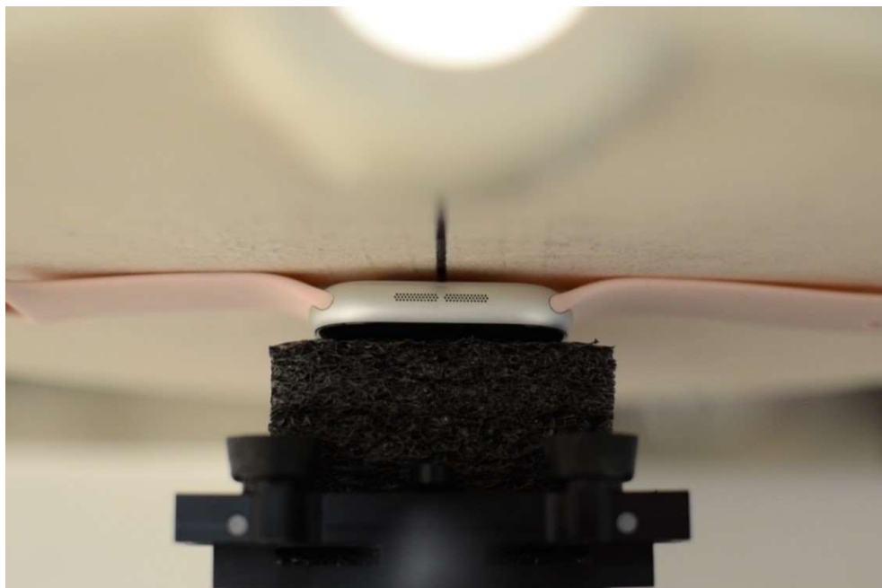
SAR Test Setup Photo 7 – Aluminum with Sport Wristband, Extremity, Back Side at 0mm
