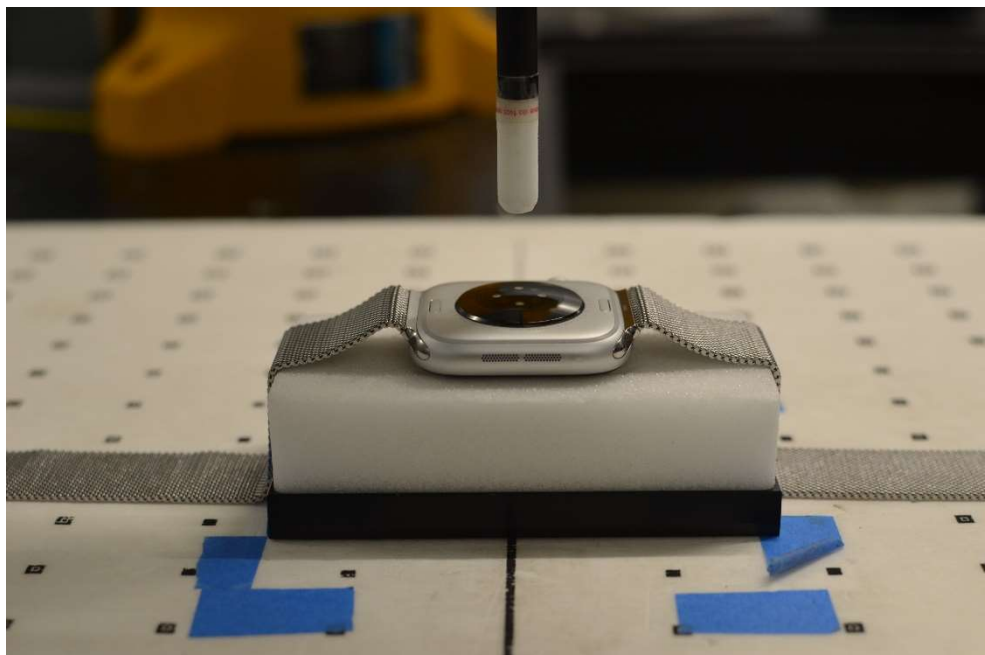
Near Field Power Density Test Setup Photo 22 – Aluminum with Metal Loop Wristband, Extremity, Back side at 9.24 mm
