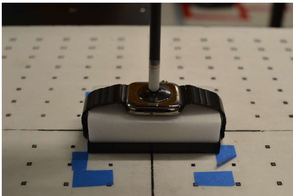
Near Field Power Density Test Setup Photo 24 – Titanium with Metal Links Wristband, Extremity, Back side at 2mm
