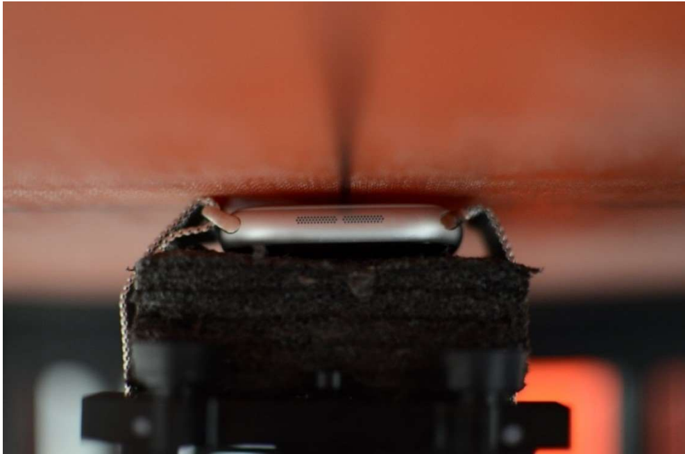
NFC Test Setup Photo 15 – Aluminum with Metal Loop Wristband, Extremity, Back Side at 0mm
