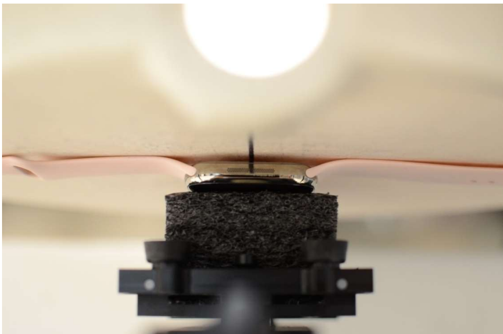
SAR Test Setup Photo 10 – Titanium with Sport Wristband, Extremity, Back Side at 0mm
