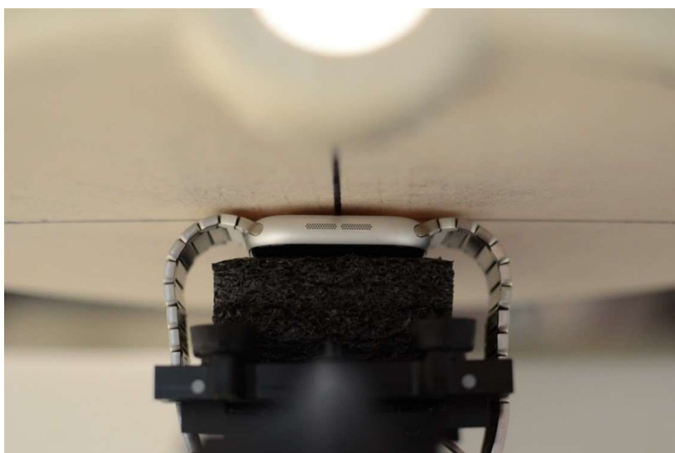
SAR Test Setup Photo 8 – Aluminum with Metal Links Wristband, Extremity, Back Side at 0mm
