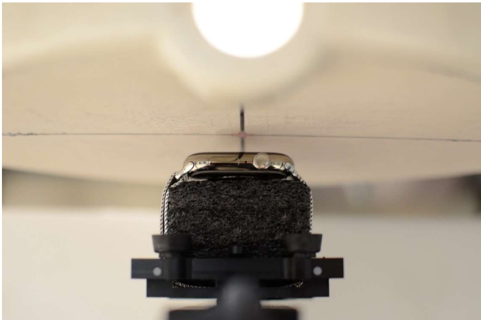
SAR Test Setup Photo 6 – Titanium with Metal Loop Wristband, Head, Front side at 10 mm
