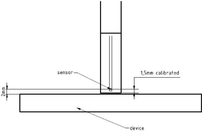
Figure H-3 EUmWVx Probe
