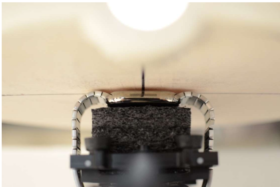
SAR Test Setup Photo 11 – Titanium with Metal Links Wristband, Extremity, Back Side at 0mm
