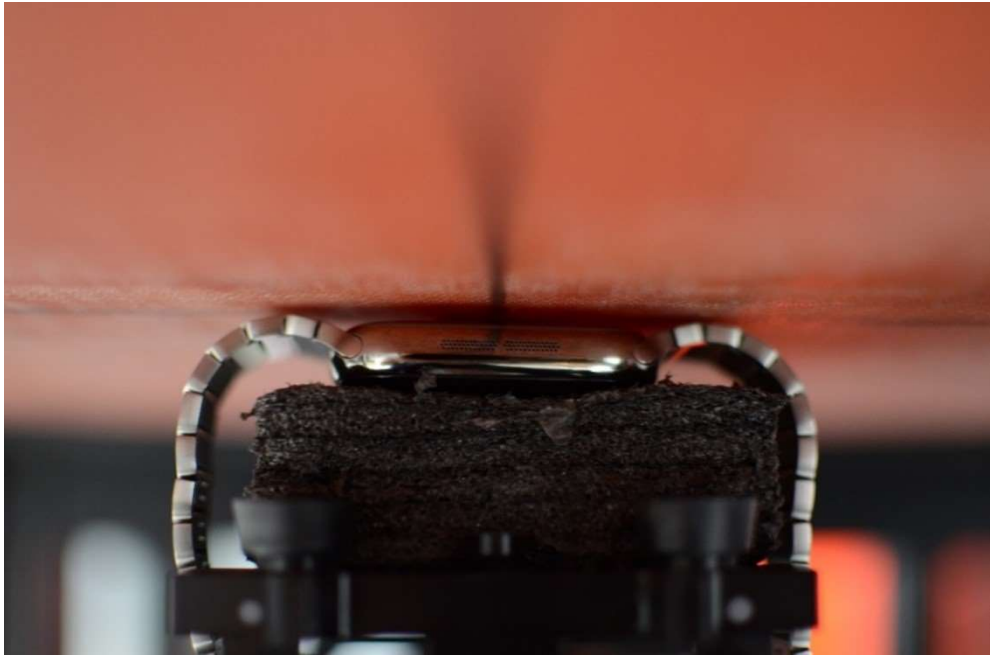
NFC Test Setup Photo 17 – Titanium with Metal Links Wristband, Extremity, Back Side at 0mm
