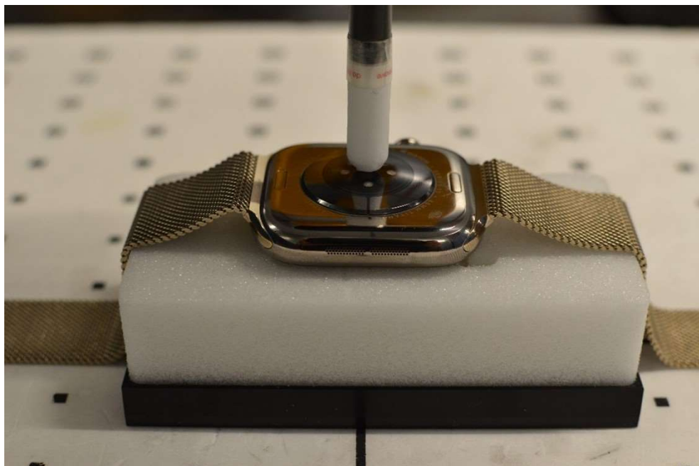
Near Field Power Density Test Setup Photo 25 – Titanium with Metal Loop Wristband, Extremity, Back side at 2mm
