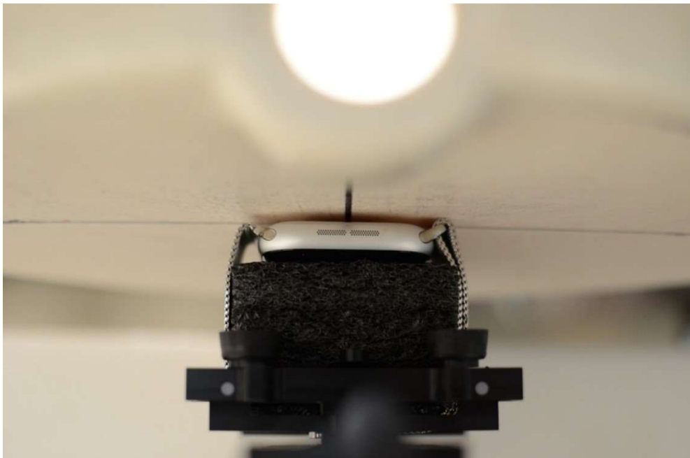
SAR Test Setup Photo 9 – Aluminum with Metal Loop Wristband, Extremity, Back Side at 0mm
