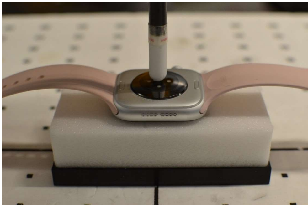
Near Field Power Density Test Setup Photo 19 – Aluminum with Sport Wristband, Extremity, Back side at 2mm
