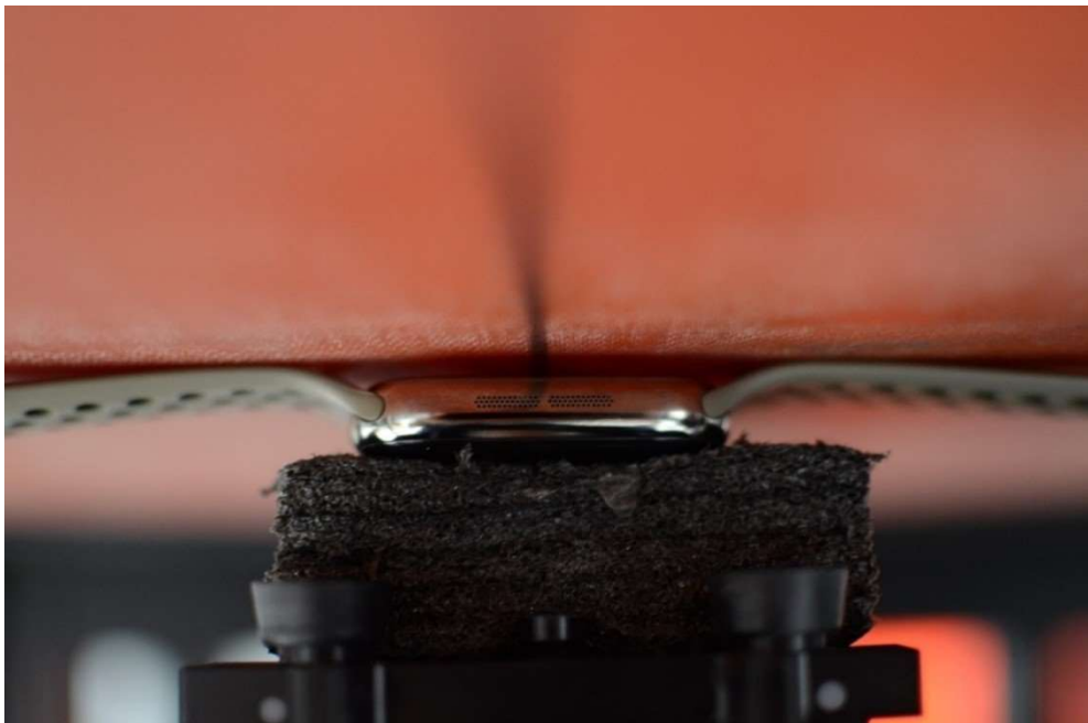
NFC Test Setup Photo 16 – Titanium with Sport Wristband, Extremity, Back Side at 0mm
