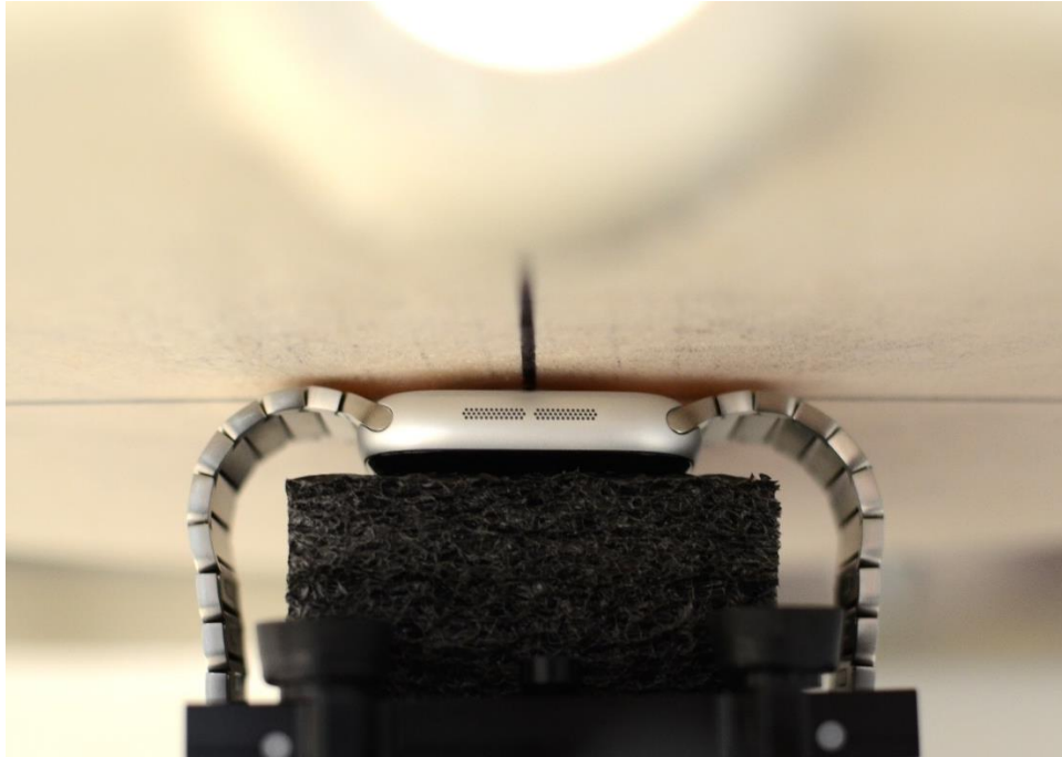
SAR Test Setup Photo 5 – Aluminum with Metal Links Wristband, Extremity, Back Side at 0mm
