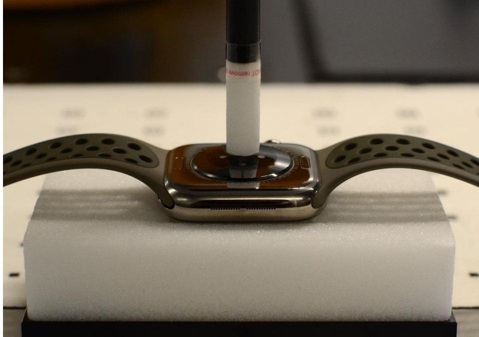
Near Field Power Density Test Setup Photo 23 – Titanium with Sport Wristband, Extremity, Back side at 2mm
