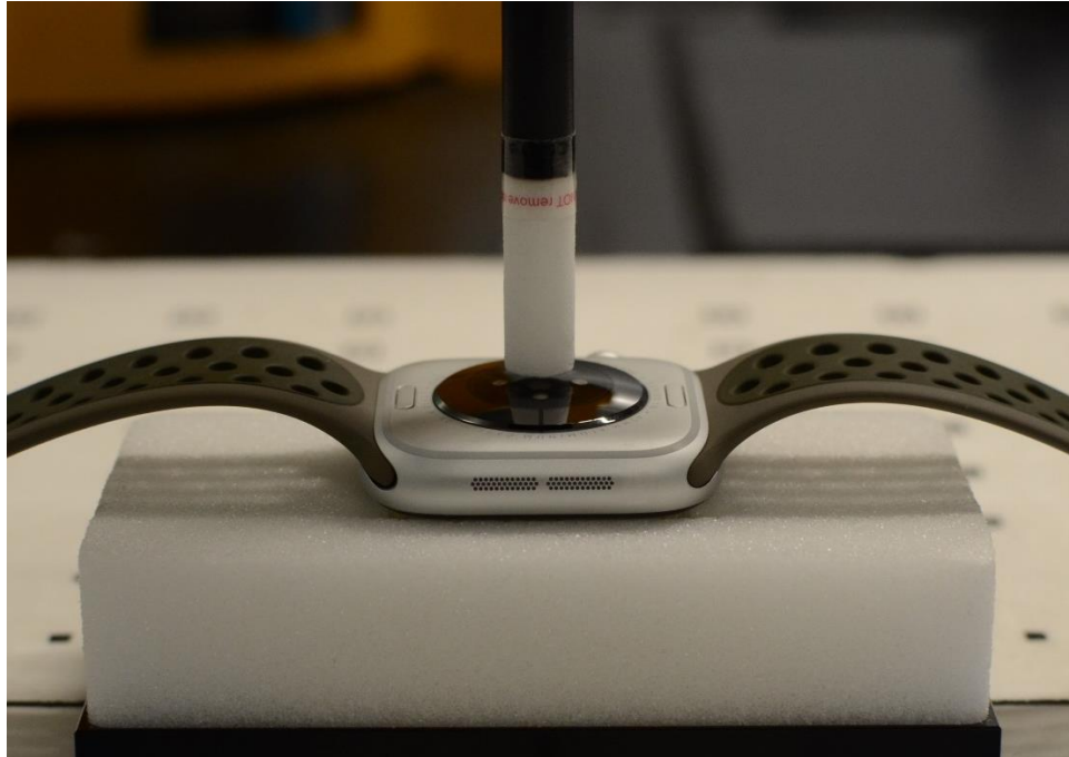
Near Field Power Density Test Setup Photo 19 – Aluminum with Sport Wristband, Extremity, Back side at 2mm
