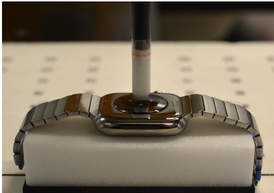
Near Field Power Density Test Setup Photo 24 – Titanium with Metal Links Wristband, Extremity, Back side at 2mm
