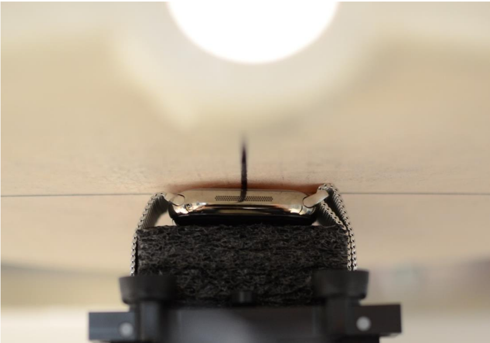
SAR Test Setup Photo 12 – Titanium with Metal Loop Wristband, Extremity, Back Side at 0mm
