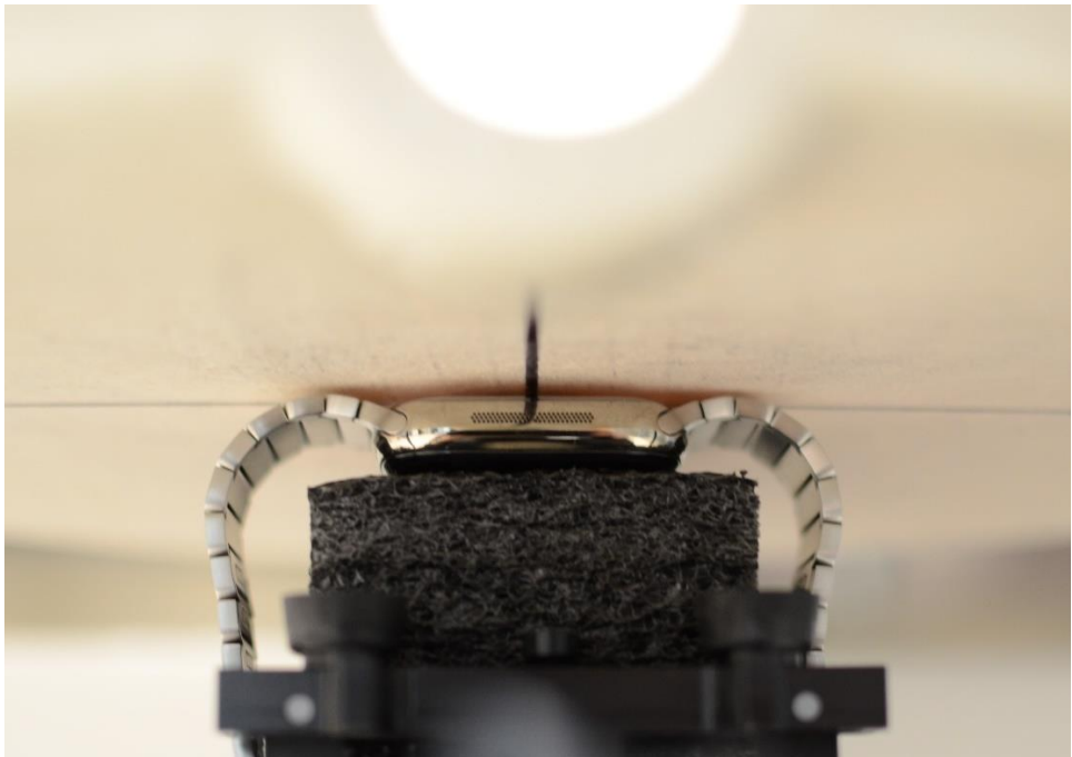
SAR Test Setup Photo 11 – Titanium with Metal Links Wristband, Extremity, Back Side at 0mm
