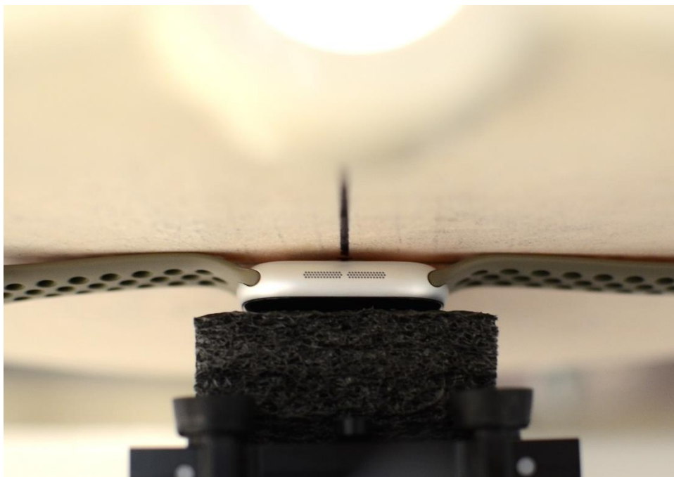
SAR Test Setup Photo 4 – Aluminum with Sport Wristband, Extremity, Back Side at 0mm
