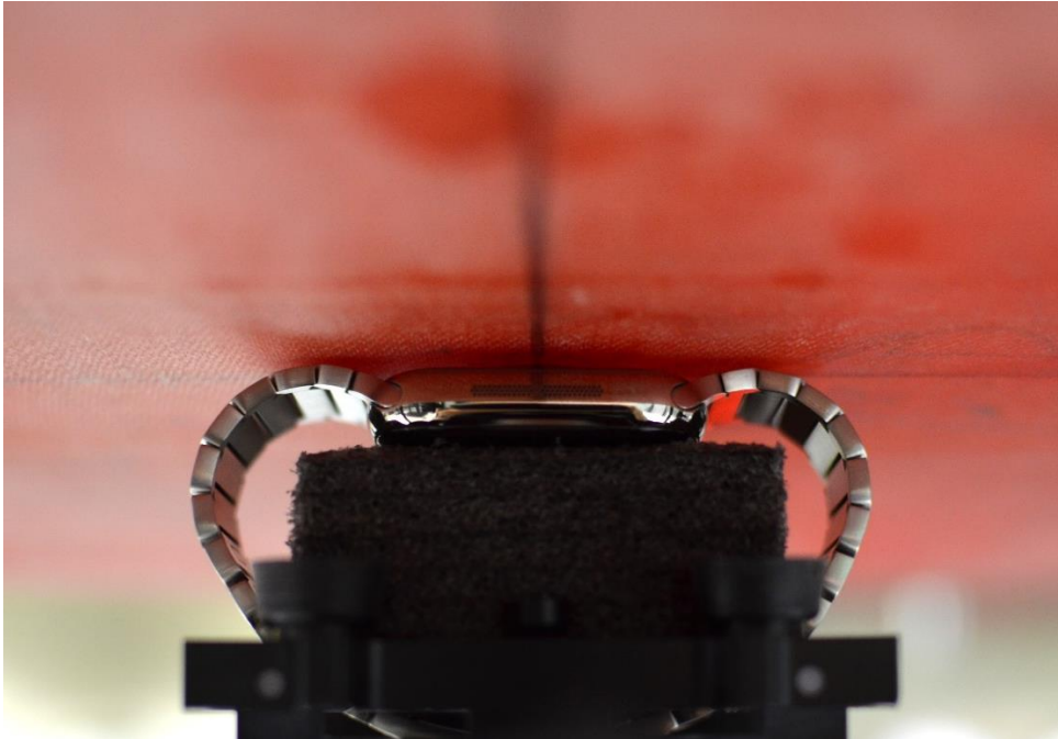
NFC Test Setup Photo 17 – Titanium with Metal Links Wristband, Extremity, Back side at 0mm
