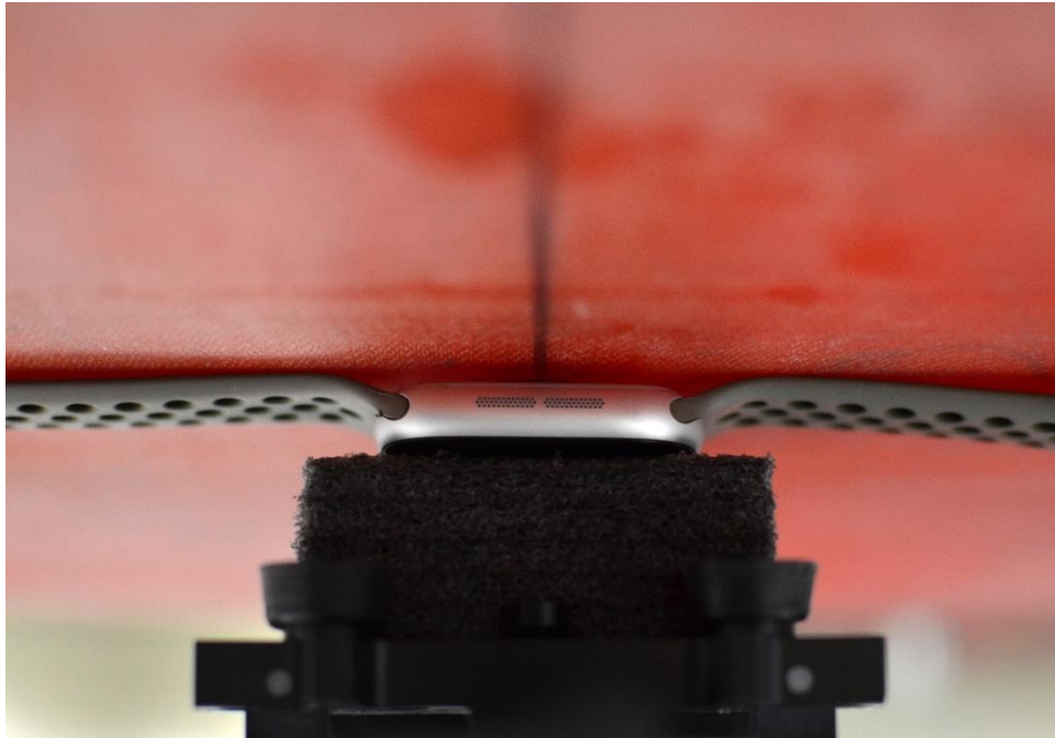
NFC Test Setup Photo 13 – Aluminum with Sport Wristband, Extremity, Back side at 0mm
