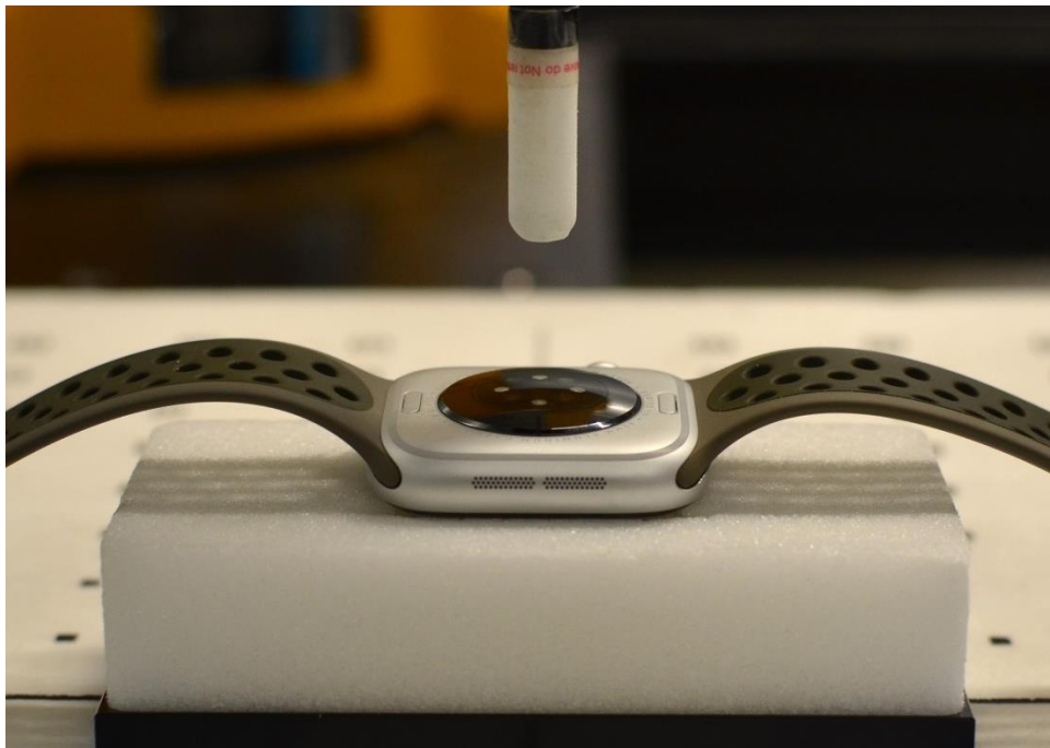
Near Field Power Density Test Setup Photo 20 – Aluminum with Sport Wristband, Extremity, Back side at 9.24mm
