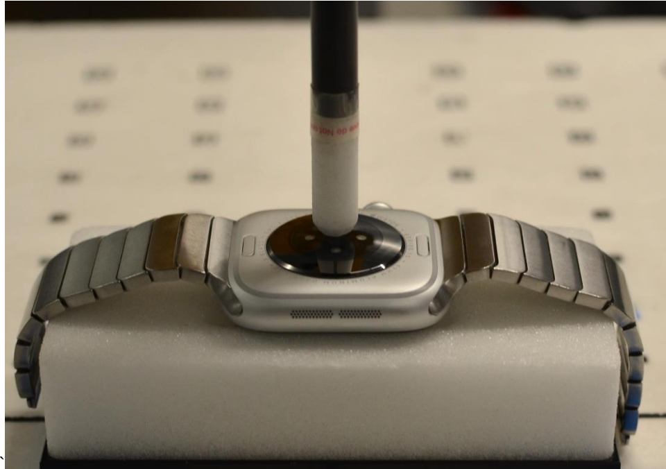
Near Field Power Density Test Setup Photo 21 – Aluminum with Metal Links Wristband, Extremity, Back side at 2mm
