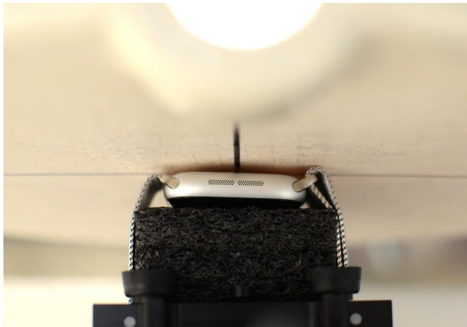
SAR Test Setup Photo 6 – Aluminum with Metal Loop Wristband, Extremity, Back Side at 0mm
