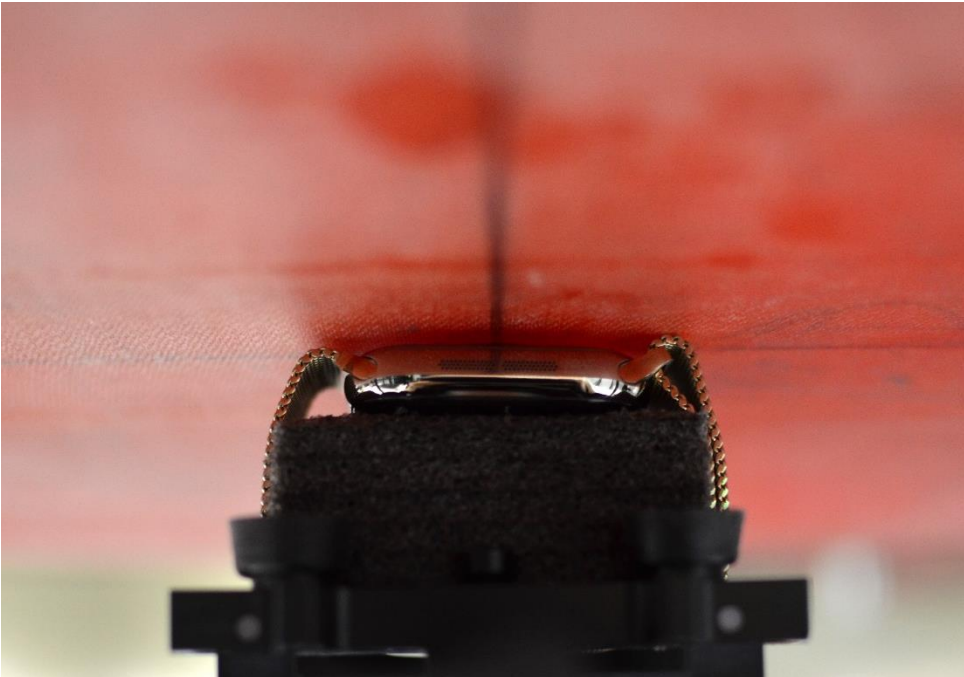
NFC Test Setup Photo 18 – Titanium with Metal Loop Wristband, Extremity, Back side at 0mm
