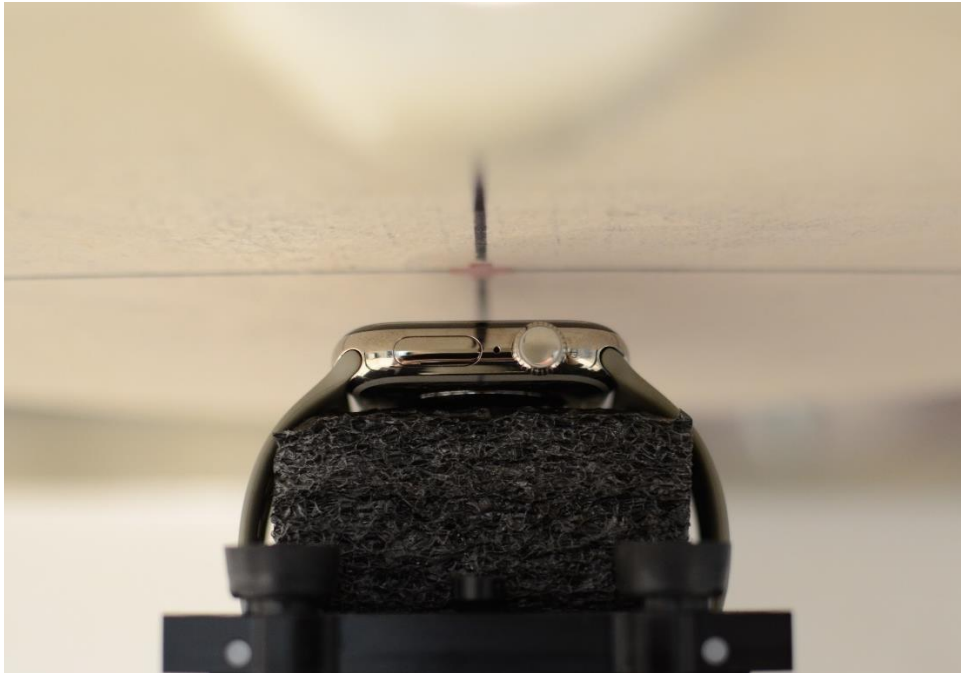
SAR Test Setup Photo 7 – Titanium with Sport Wristband, Head, Front Side at 10mm
