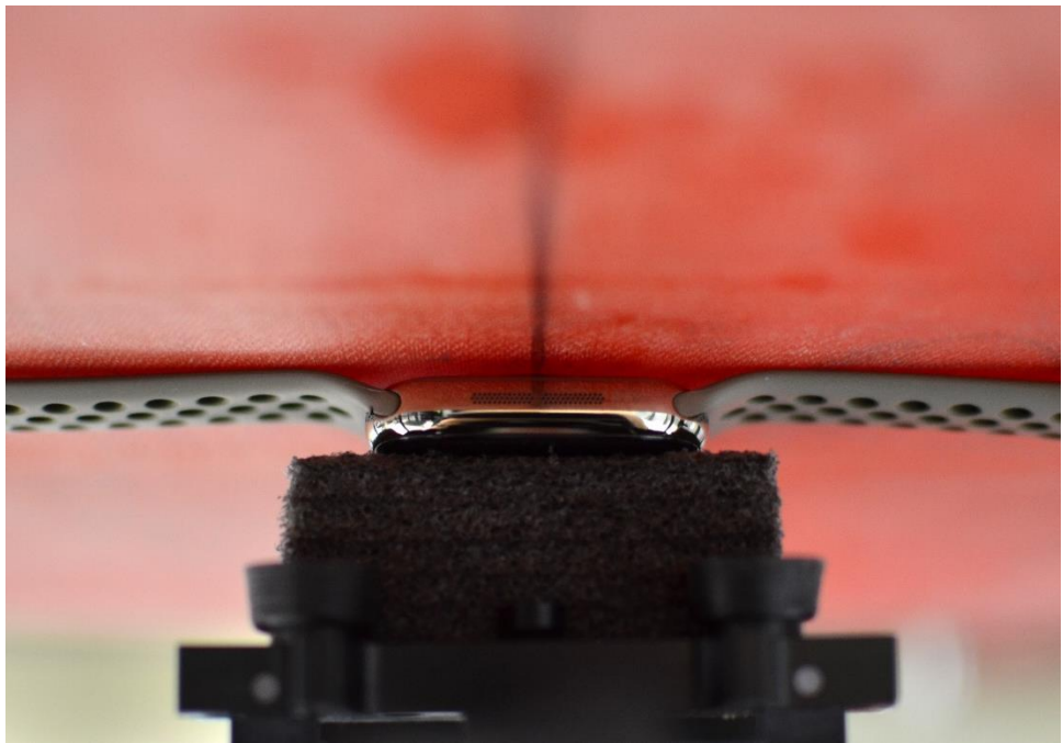
NFC Test Setup Photo 16 – Titanium with Sport Wristband, Extremity, Back side at 0mm
