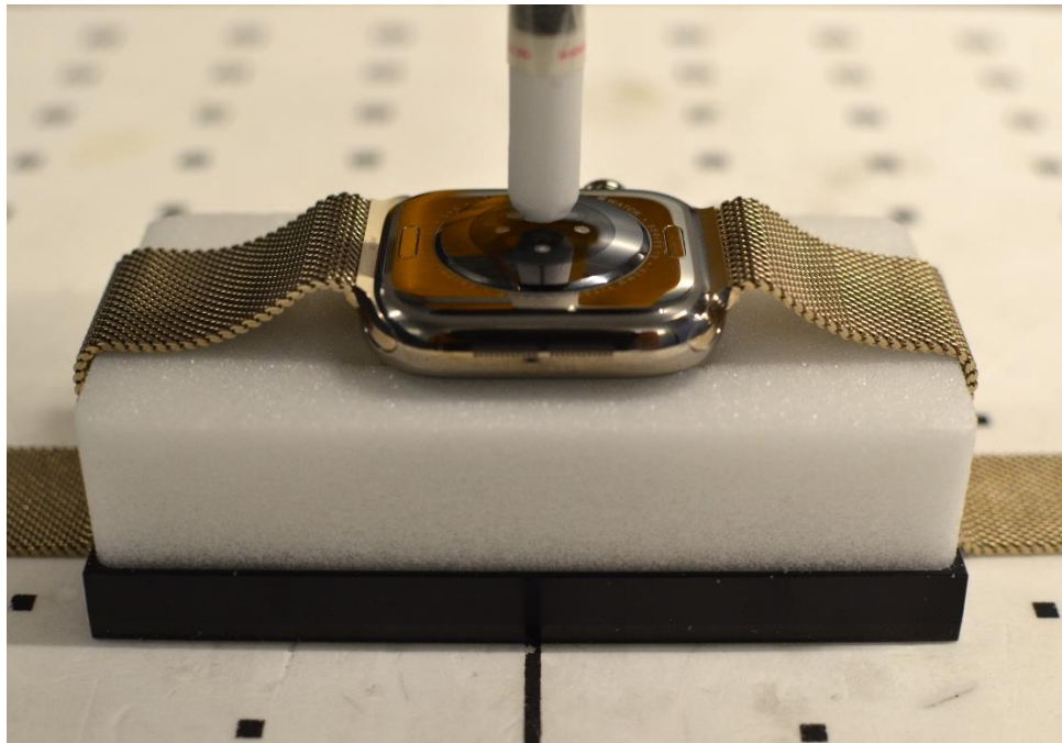
Near Field Power Density Test Setup Photo 25 – Titanium with Metal Loop Wristband, Extremity, Back side at 2mm
