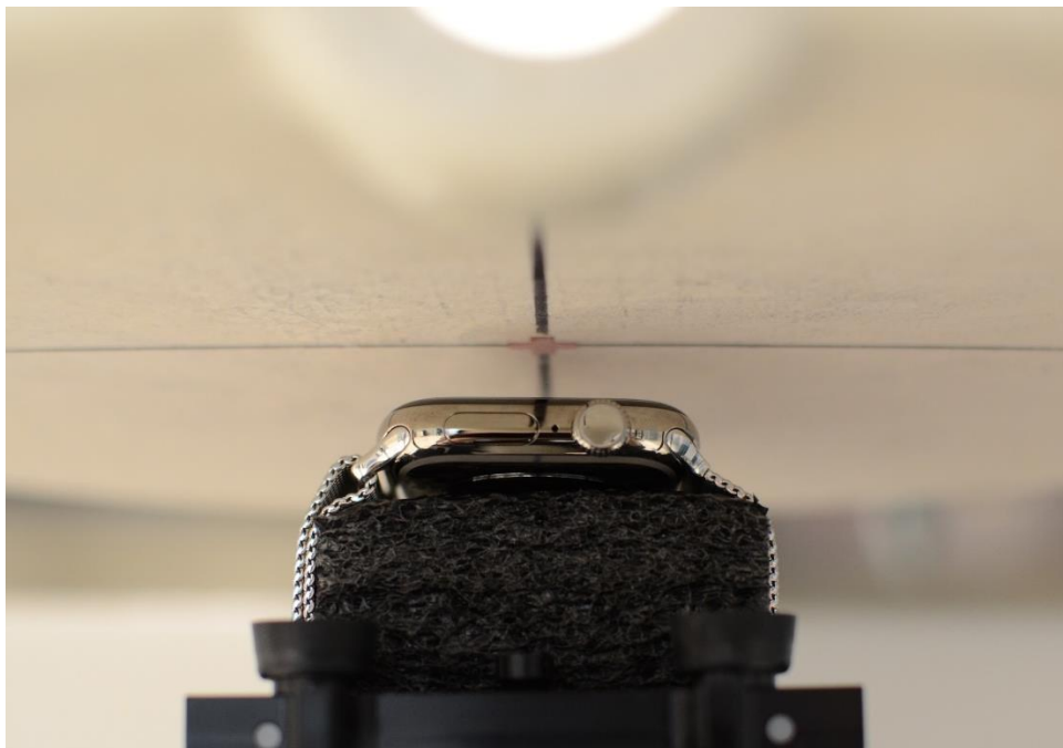
SAR Test Setup Photo 9 – Titanium with Metal Loop Wristband, Head, Front Side at 10mm
