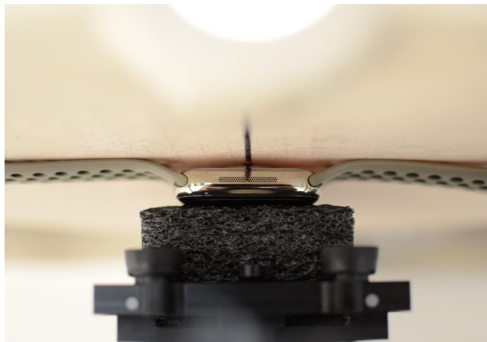
SAR Test Setup Photo 10 – Titanium with Sport Wristband, Extremity, Back Side at 0mm
