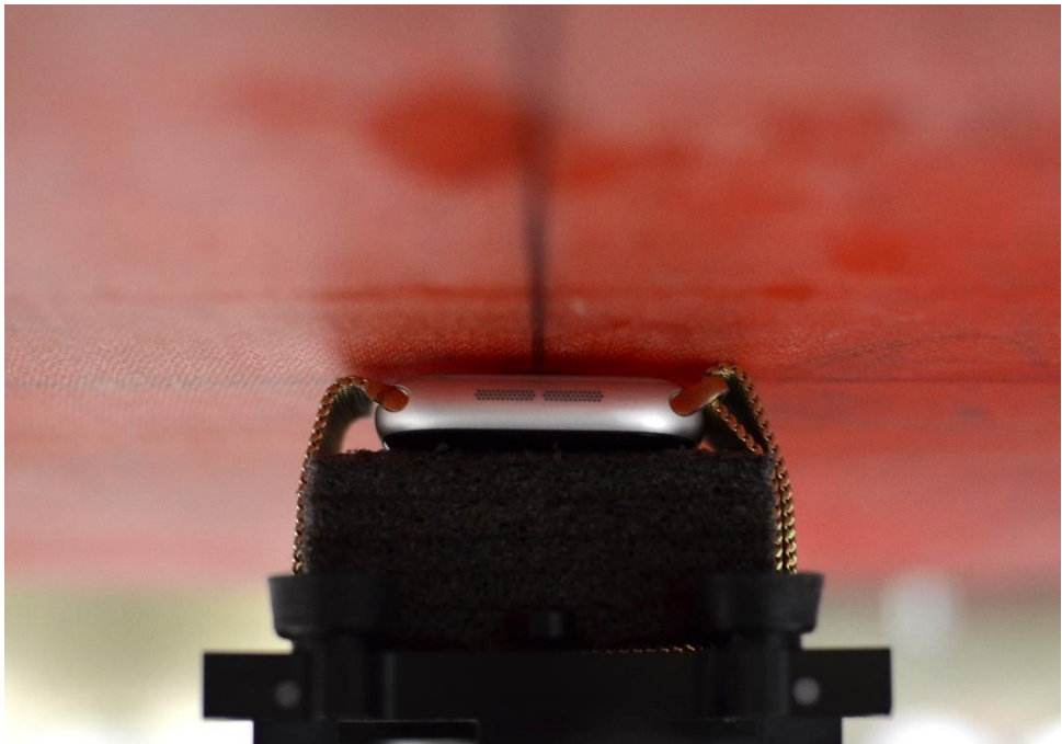
NFC Test Setup Photo 15 – Aluminum with Metal Loop Wristband, Extremity, Back side at 0mm
