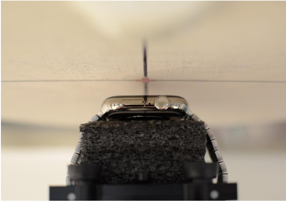
SAR Test Setup Photo 8 – Titanium with Metal Links Wristband, Head, Front Side at 10mm
