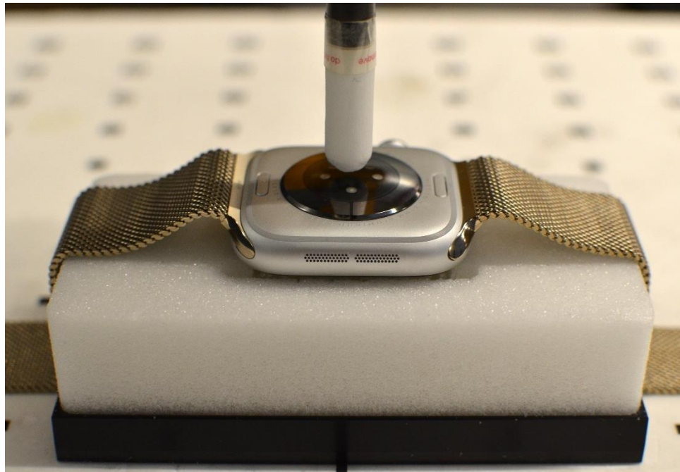
Near Field Power Density Test Setup Photo 22 – Aluminum with Metal Loop Wristband, Extremity, Back side at 2mm
