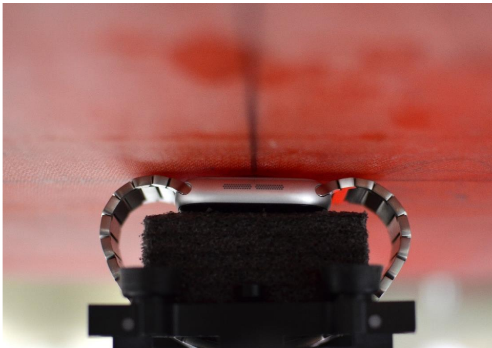
NFC Test Setup Photo 14 – Aluminum with Metal Links Wristband, Extremity, Back side at 0mm
