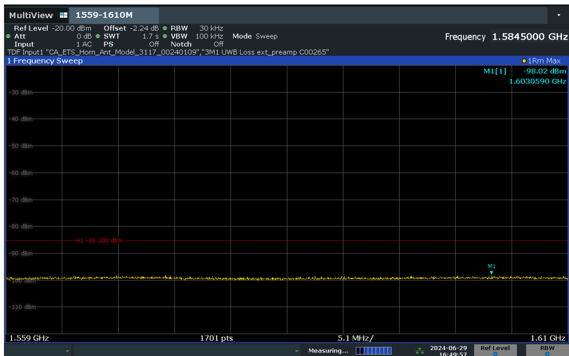
Plot 7-22. Radiated Spurious Emission 1559-1610MHz (Ch. 5, Config 409, Payload 4093 Ant. Pol. V)
