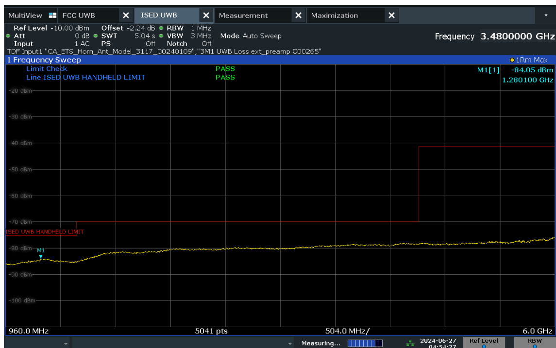
Plot 7-17. ISED Radiated Spurious Emission 960-6000MHz (Ch. 5, Config 409, Payload 4093 Ant. Pol. H)
