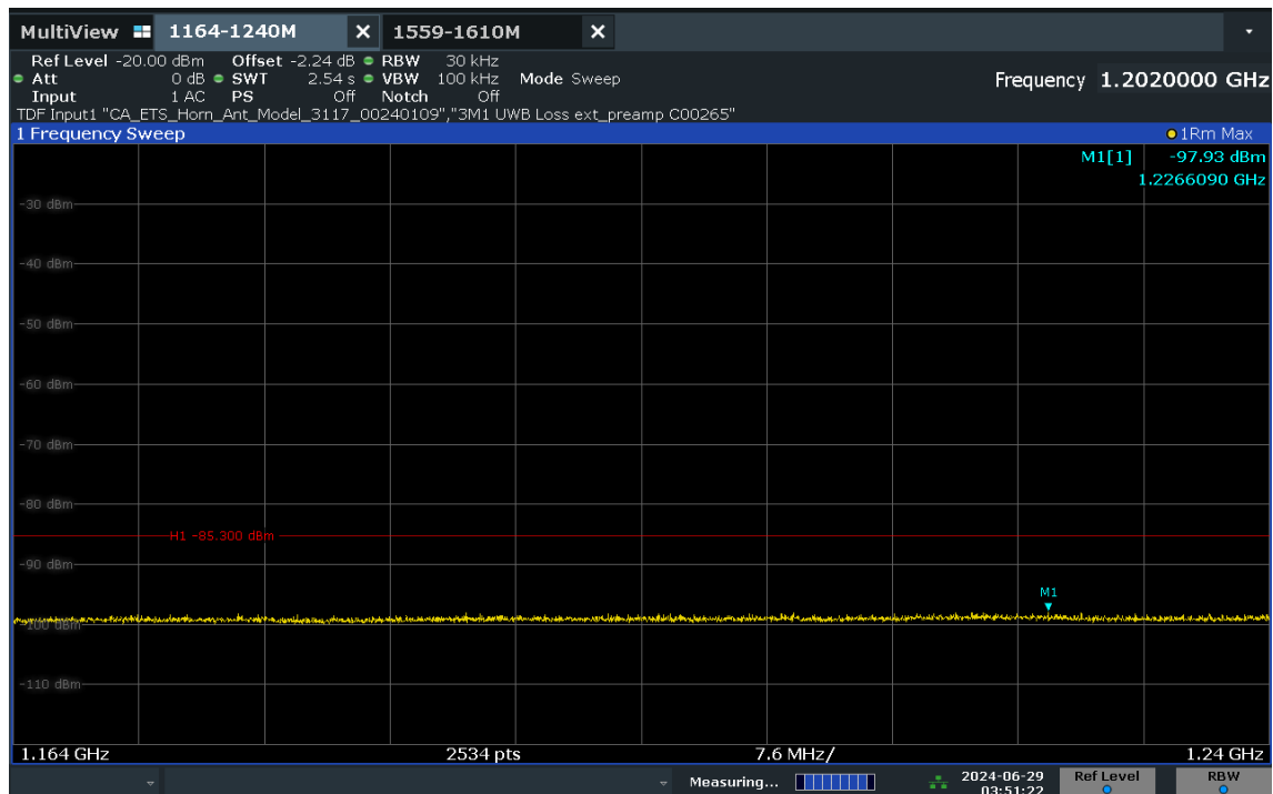
Plot 7-20. Radiated Spurious Emission 1164-1240MHz (Ch. 5, Config 409, Payload 4093 Ant. Pol. V)
