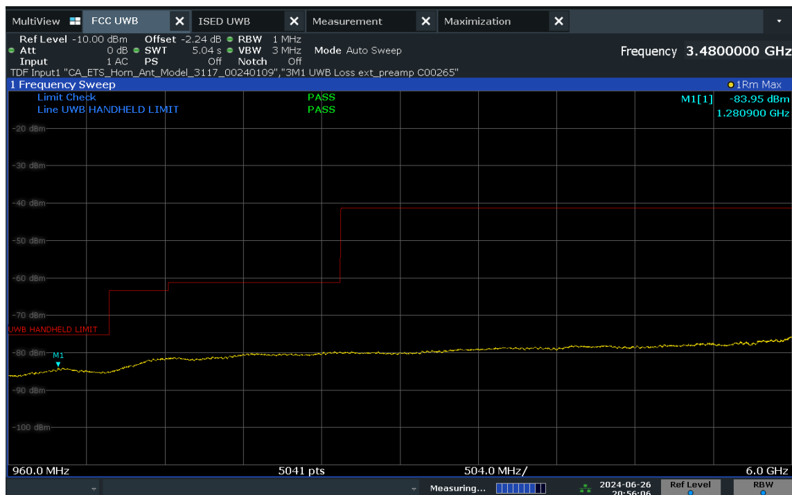
Plot 7-15. FCC Radiated Spurious Emission 960-6000MHz (Ch. 5, Config 409, Payload 4093 Ant. Pol. H)
