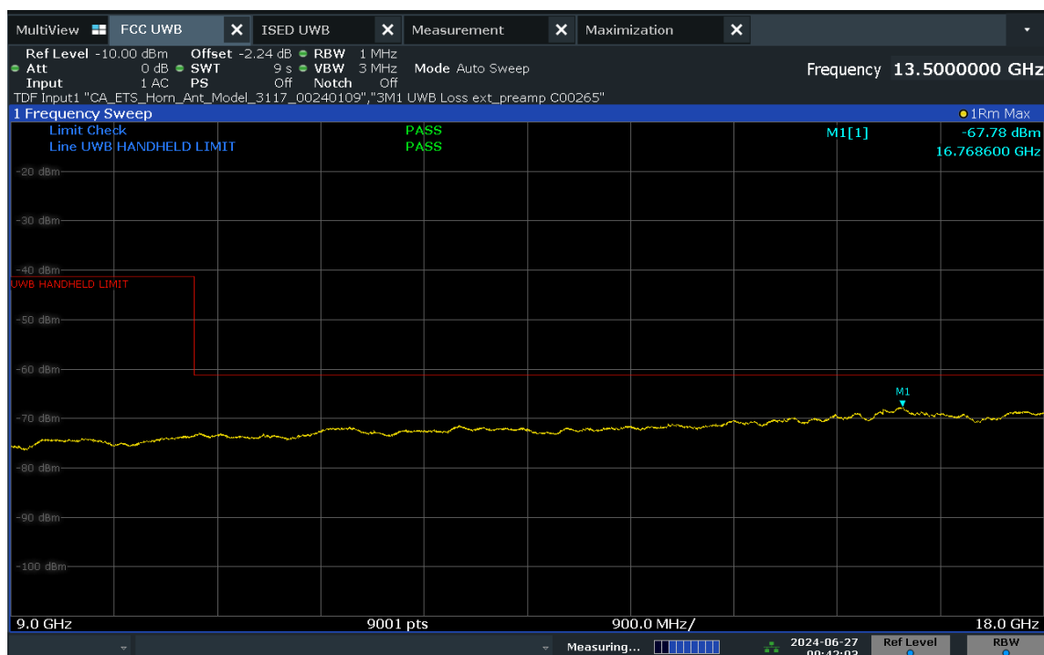
Plot 7-34. Radiated Spurious Emission 9-18GHz (Ch. 9, Config 409, Payload 4093 Ant. Pol. V)
