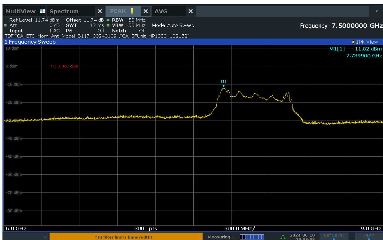
Plot 7-6. Peak Radiated Power (Ch. 9, Config 409/Payload 4093)
