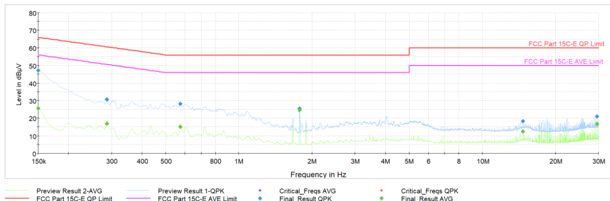
Plot 7-44. AC Line Conducted Plot (Ch. 9, Config 409, Payload 4093 N, with Laptop + Magnetic Charger)
