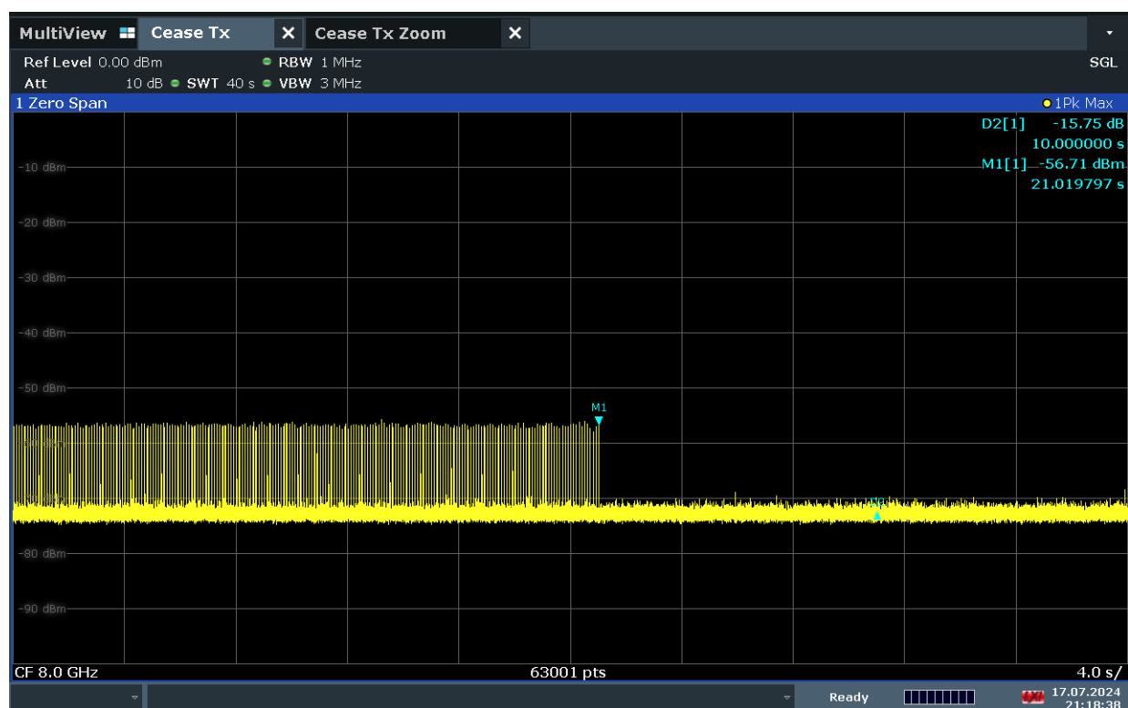
Plot 7-14. Cessation Time – Mode2 (Ch. 9, 8 GHz)
