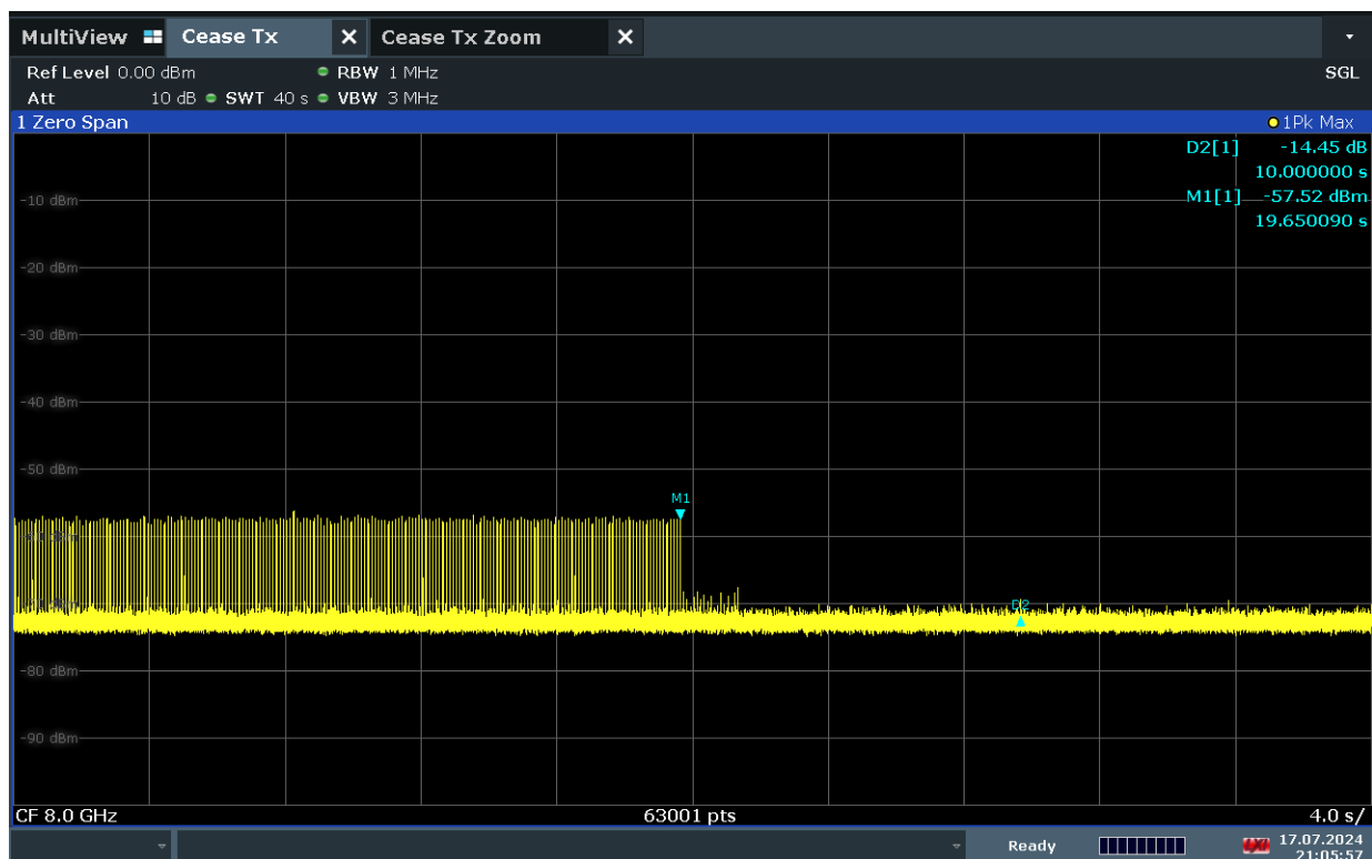
Plot 7-12. Cessation Time – Mode1 (Ch. 9, 8 GHz)
