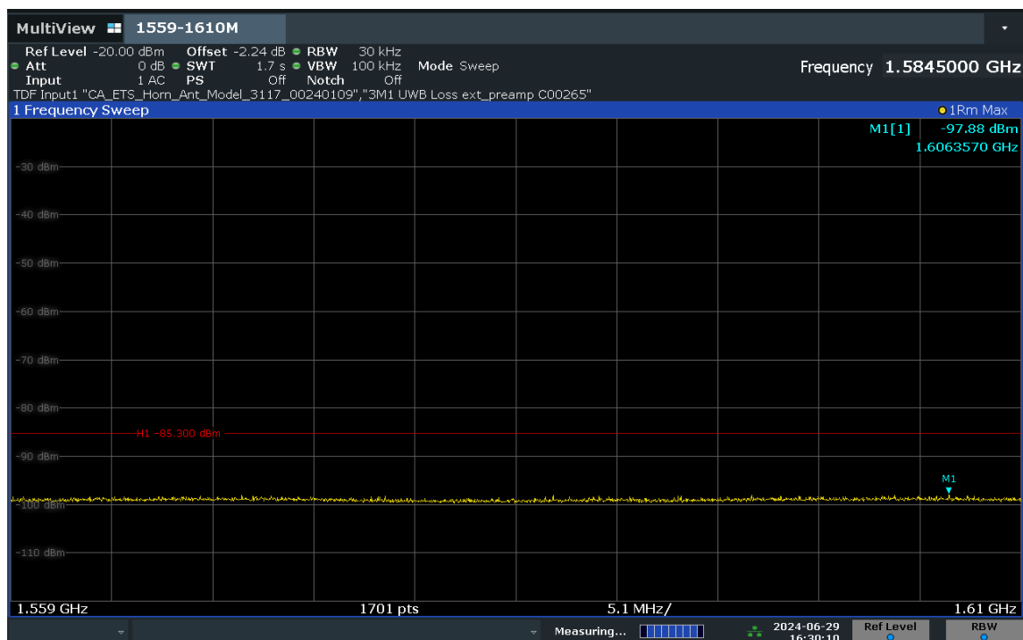
Plot 7-21. Radiated Spurious Emission 1559-1610MHz (Ch. 5, Config 409, Payload 4093 Ant. Pol. H)
