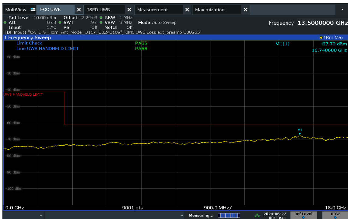
Plot 7-33. Radiated Spurious Emission 9-18GHz (Ch. 9, Config 409, Payload 4093 Ant. Pol. H)
