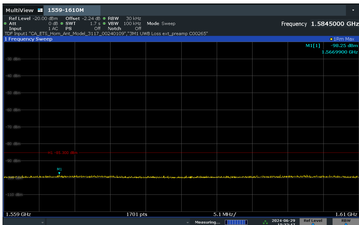
Plot 7-32. Radiated Spurious Emission 1559-1610MHz (Ch. 9, Config 409, Payload 4093 Ant. Pol. V)
