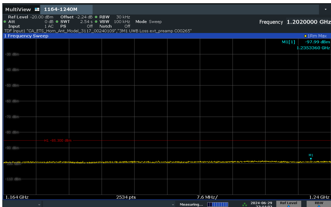
Plot 7-30. Radiated Spurious Emission 1164-1240MHz (Ch. 9, Config 409, Payload 4093 Ant. Pol. V)
