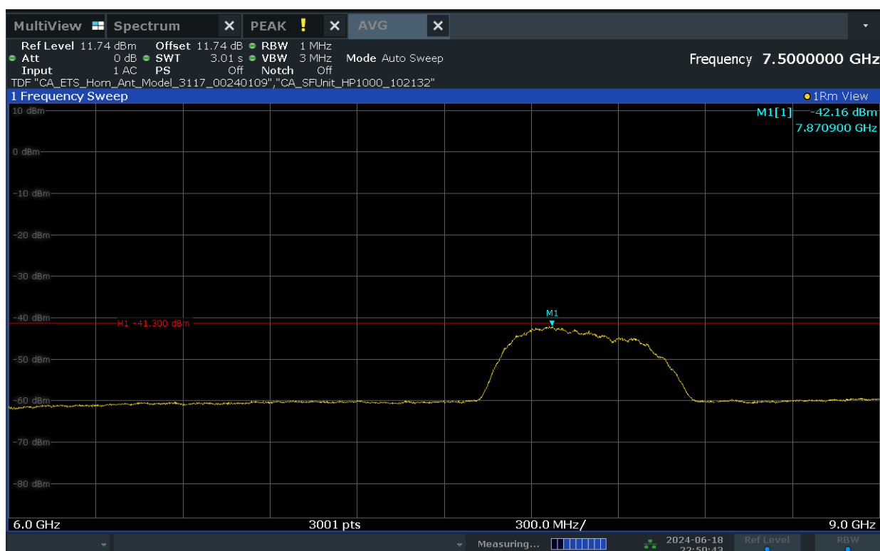
Plot 7-8. Average Radiated Power (Ch. 9, Config 409/Payload 4093)
