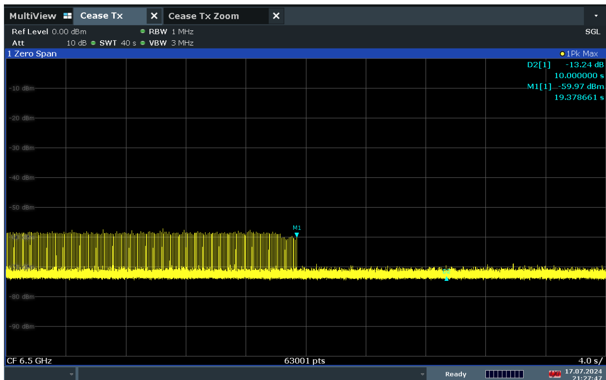
Plot 7-11. Cessation Time – Mode2 (Ch. 5, 6.5 GHz)
