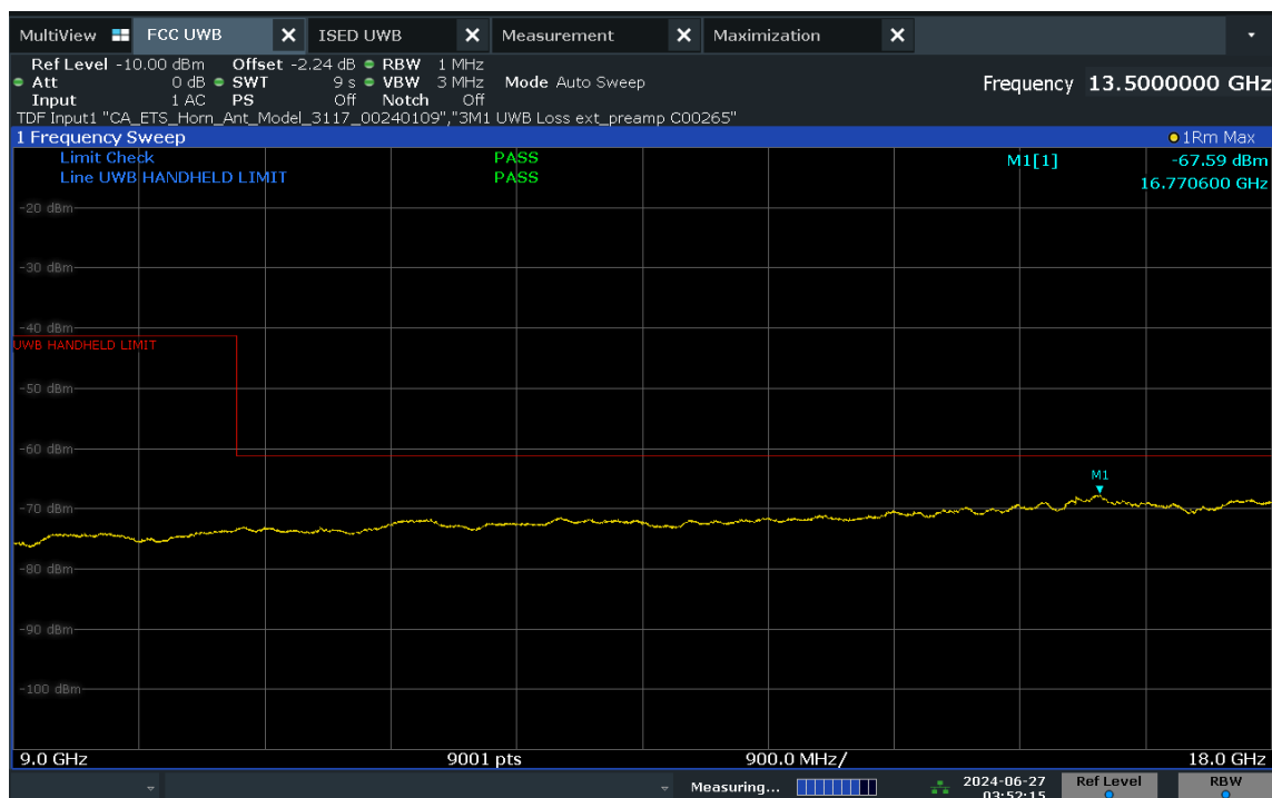
Plot 7-23. Radiated Spurious Emission 9-18GHz (Ch. 5, Config 409, Payload 4093 Ant. Pol. H)
