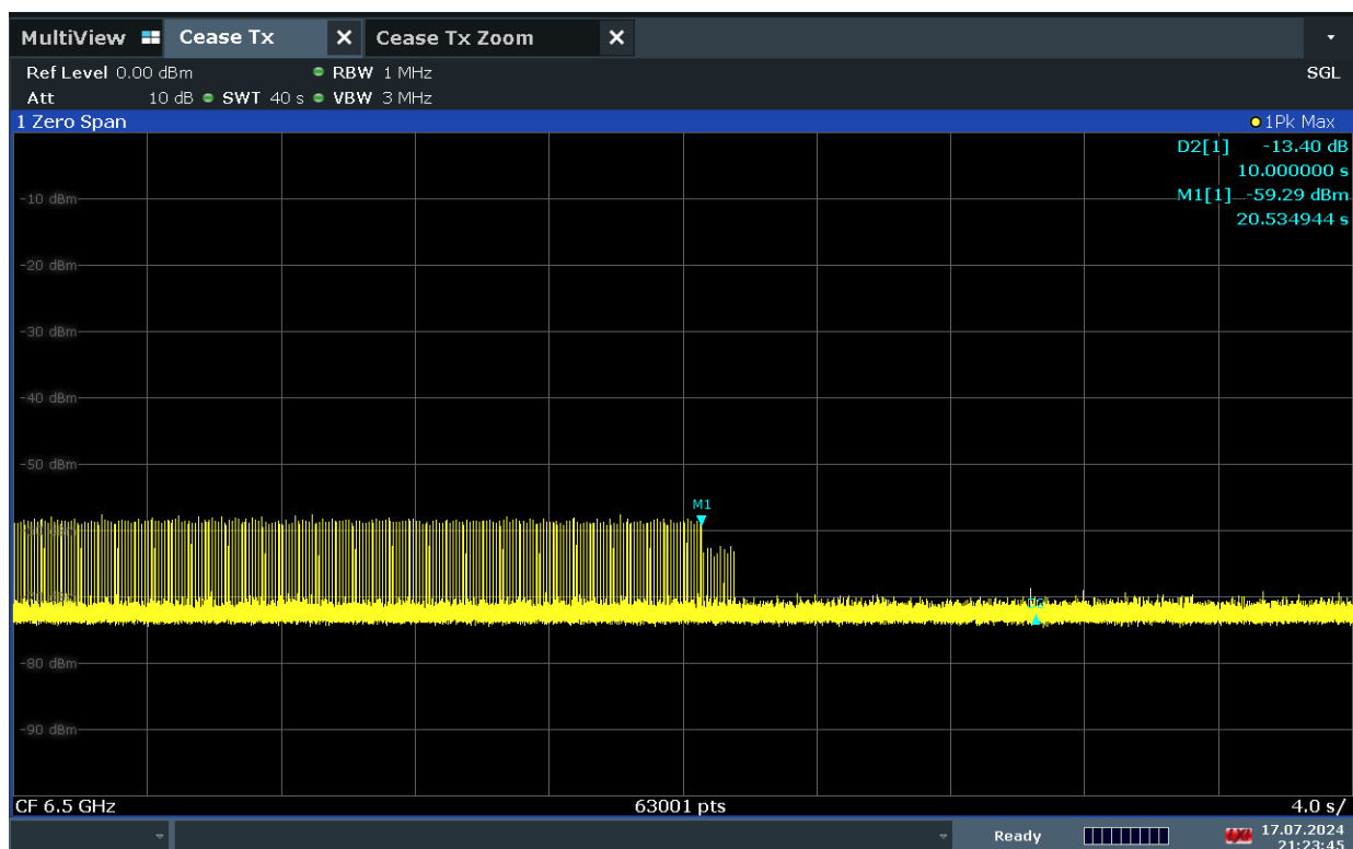
Plot 7-9. Cessation Time – Mode1 (Ch. 5, 6.5 GHz)
