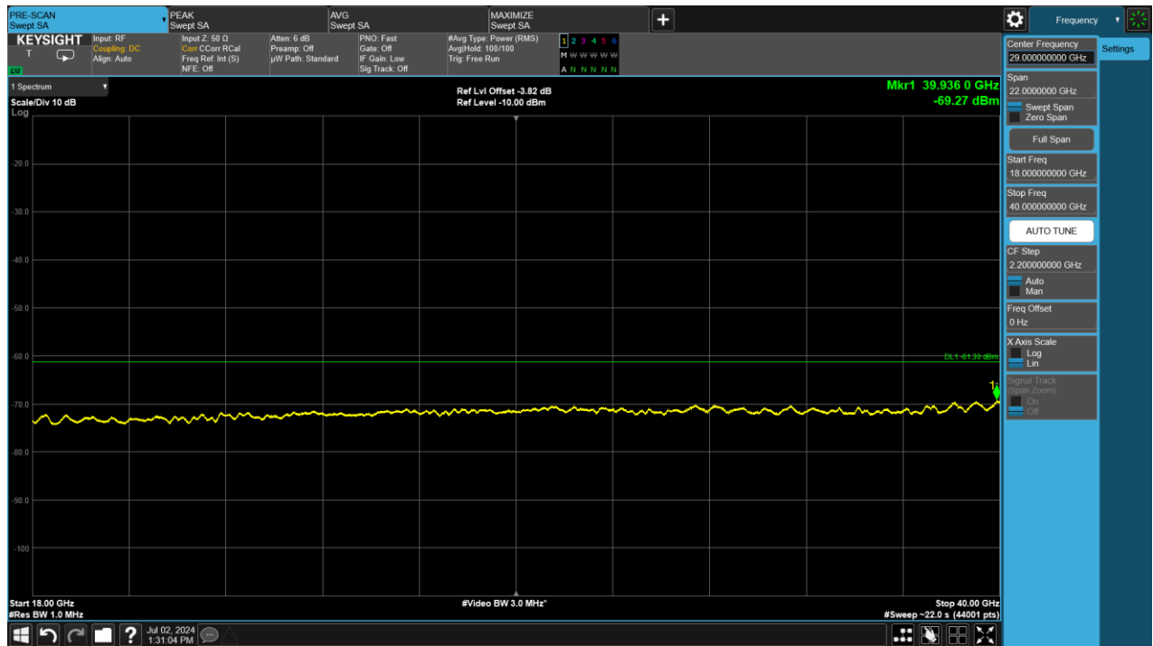
Plot 7-37. Radiated Spurious Emission 18-40GHz (Ch. 9, Config 409, Payload 4093 Ant. Pol. H)
