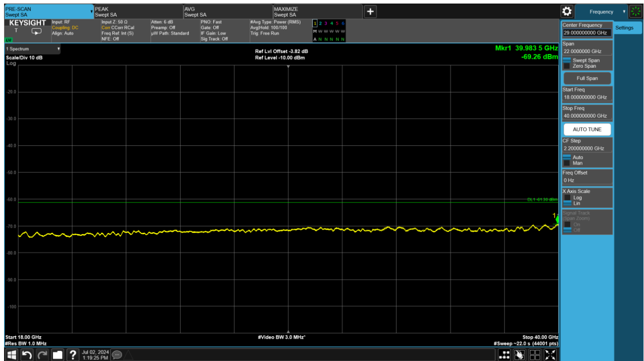
Plot 7-38. Radiated Spurious Emission 18-40GHz (Ch. 9, Config 409, Payload 4093 Ant. Pol. V)
