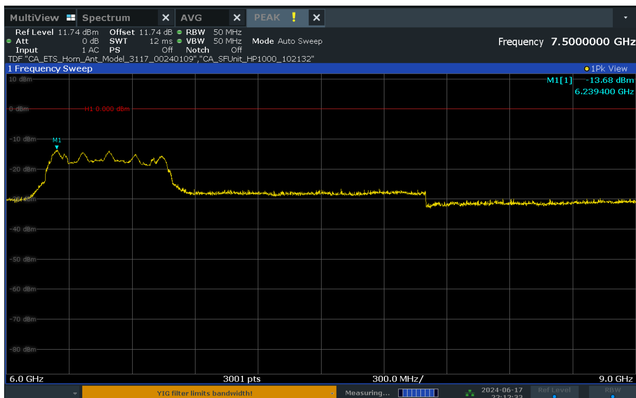
Plot 7-5. Peak Radiated Power (Ch. 5, Config 409/Payload 4093)
