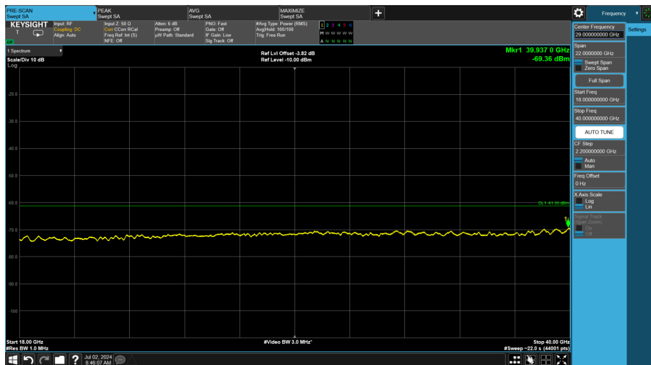
Plot 7-36. Radiated Spurious Emission 18-40GHz (Ch. 5, Config 409, Payload 4093 Ant. Pol. V)
