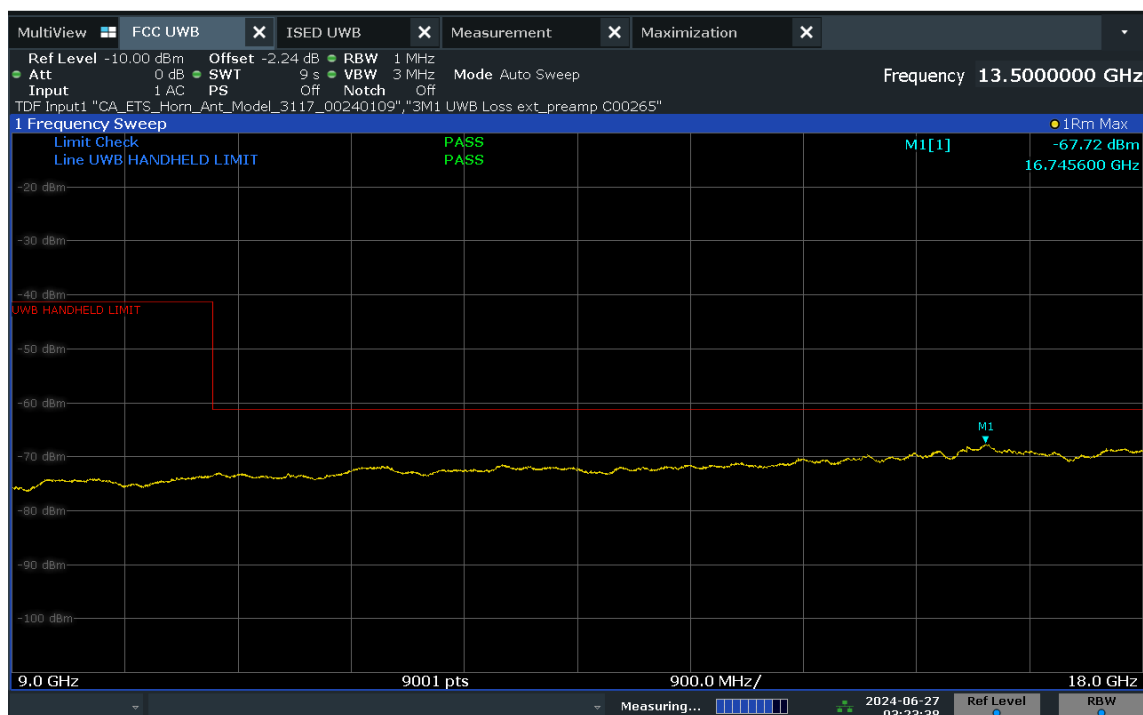
Plot 7-24. Radiated Spurious Emission 9-18GHz (Ch. 5, Config 409, Payload 4093 Ant. Pol. V)
