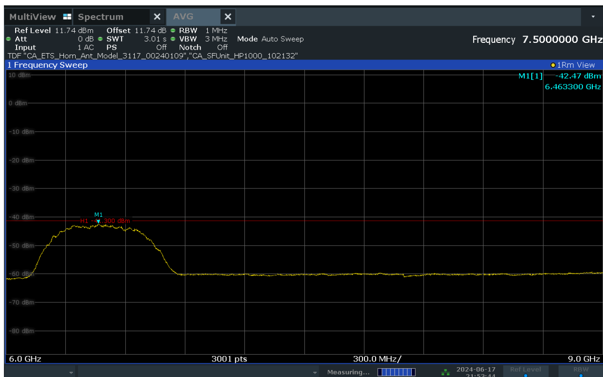
Plot 7-7. Average Radiated Power (Ch. 5, Config 409/Payload 4093)
