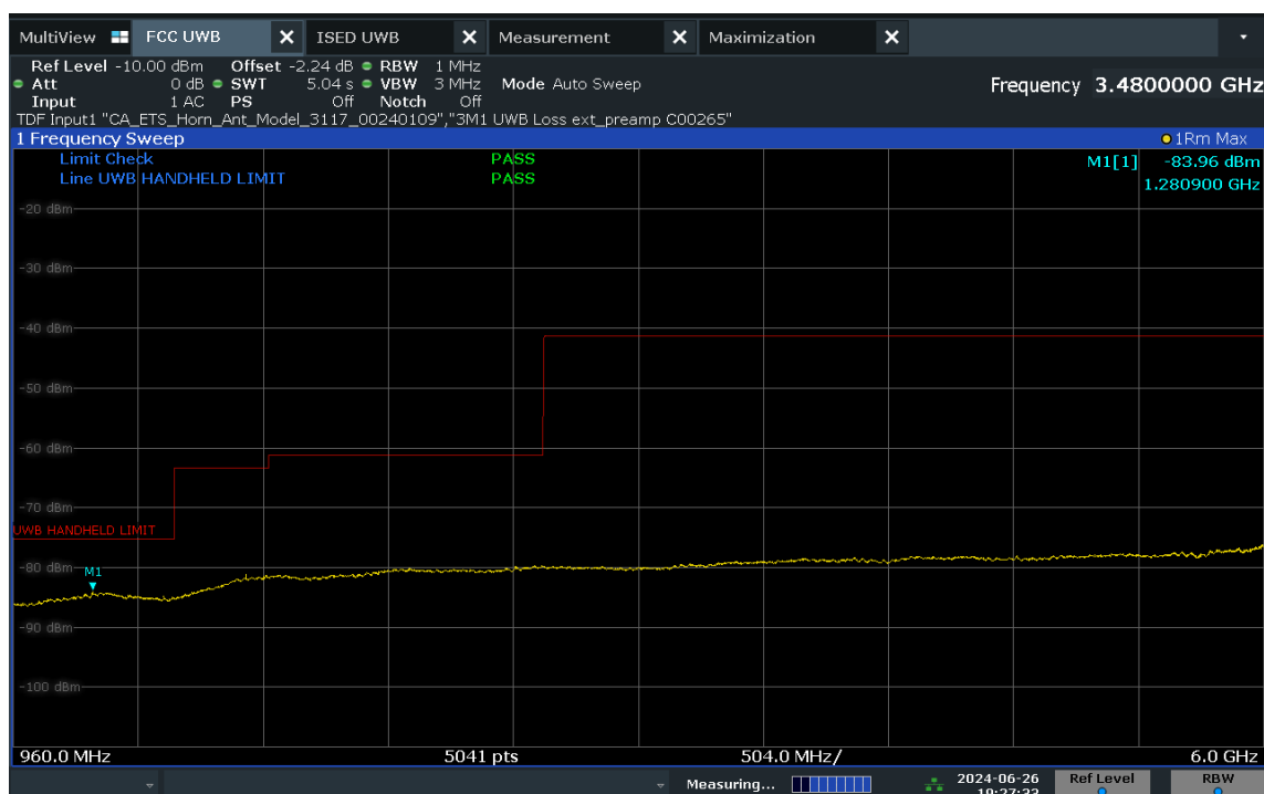
Plot 7-16. FCC Radiated Spurious Emissions 960-6000MHz (Ch. 5, Config 409, Payload 4093 Ant. Pol. V)
