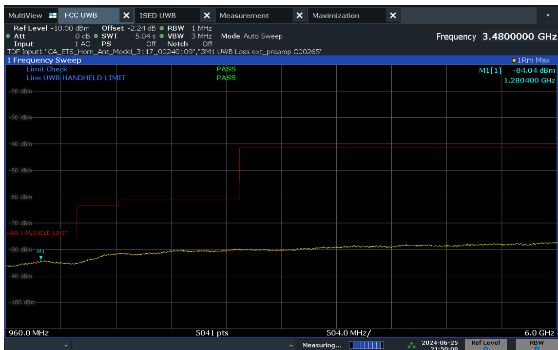
Plot 7-25. FCC Radiated Spurious Emission 960-6000MHz (Ch. 9, Config 409, Payload 4093 Ant. Pol. H)
