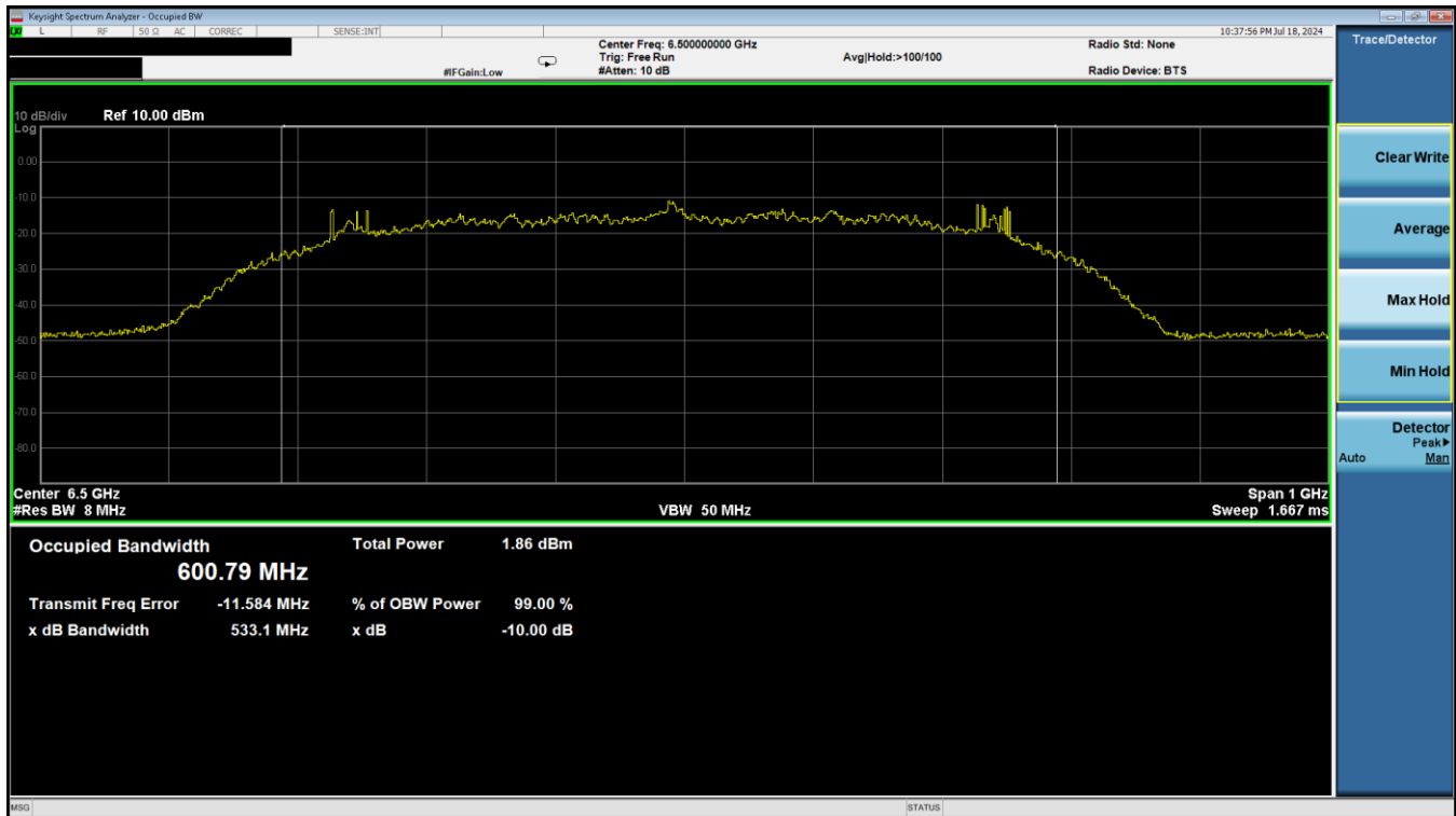
Plot 7-3. ISED 10dBc Bandwidth & 99% Occupied Bandwidth (Ch. 5, Config 409/Payload 4093)
