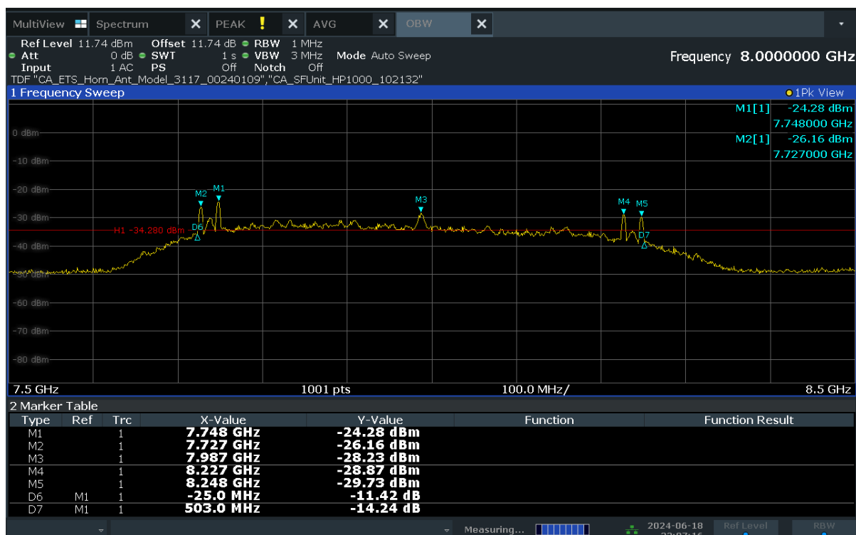
Plot 7-2. 10dBc Bandwidth (Ch. 9, Config 409/Payload 4093)
