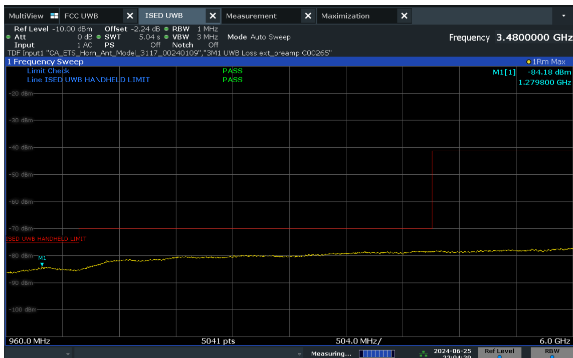
Plot 7-27. ISED Radiated Spurious Emission 960-6000MHz (Ch. 9, Config 409, Payload 4093 Ant. Pol. H)
