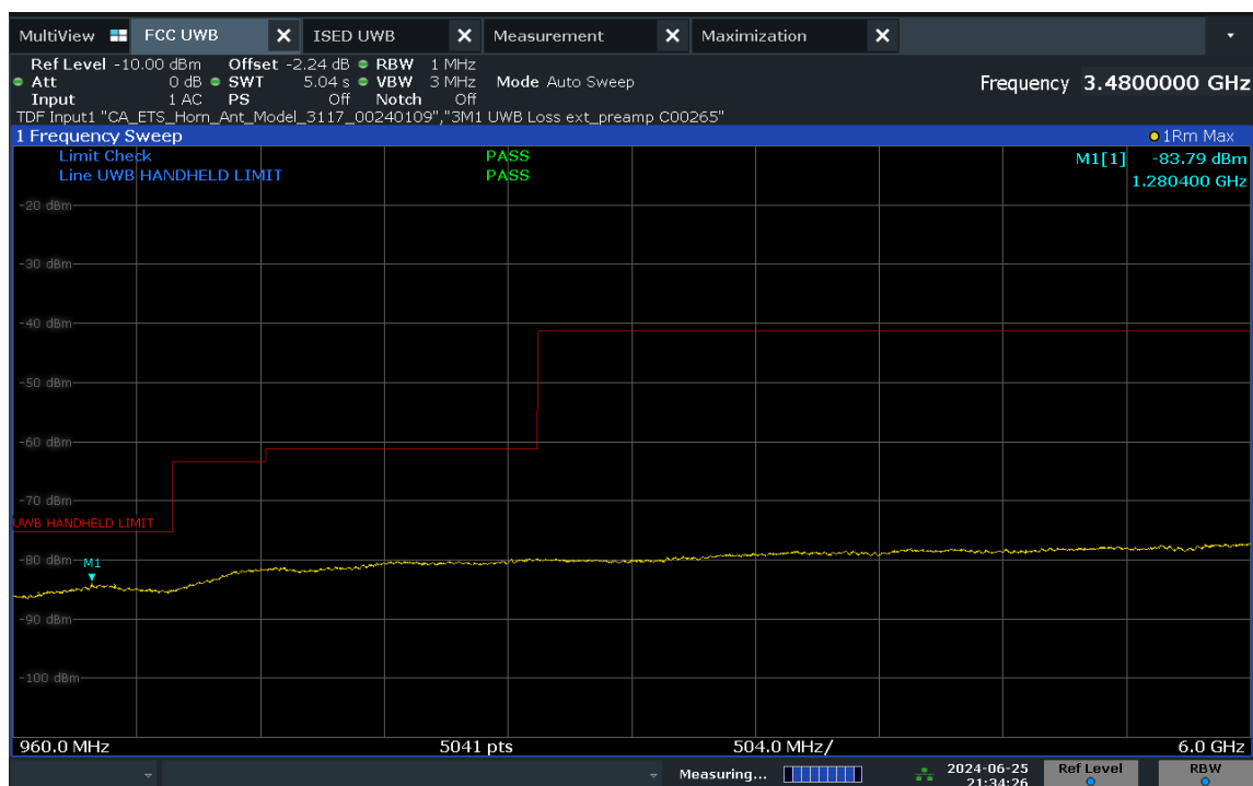
Plot 7-26. FCC Radiated Spurious Emission 960-6000MHz (Ch.9, Config 409, Payload 4093 Ant. Pol. V)
