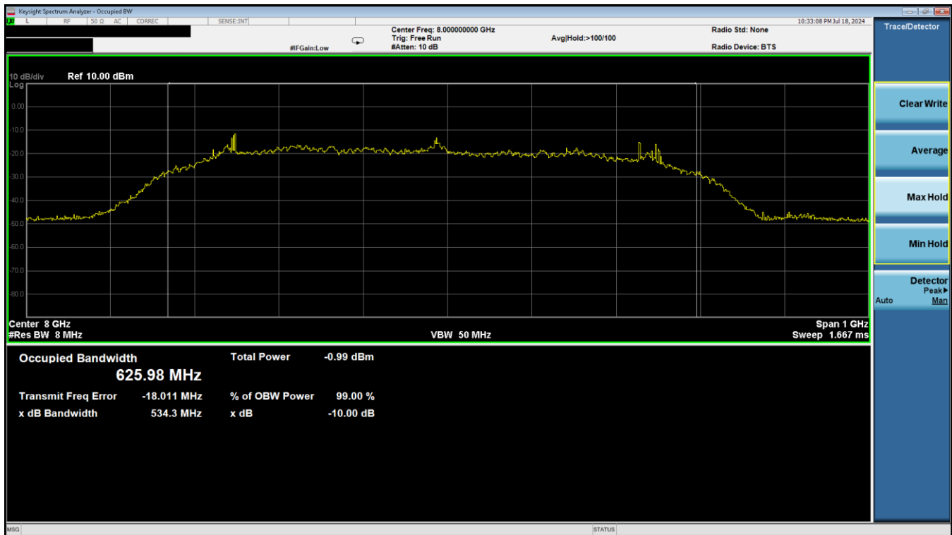
Plot 7-4. ISED 10dBc Bandwidth & 99% Occupied Bandwidth (Ch. 9, Config 409/Payload 4093)
