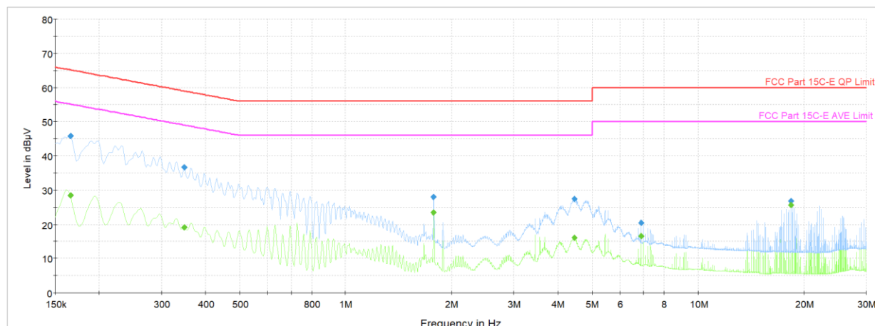
Plot 7-43. AC Line Conducted (Ch. 9, Config 409, Payload 4093 L1, with AC/DC Adapter + Magnetic Charger)
