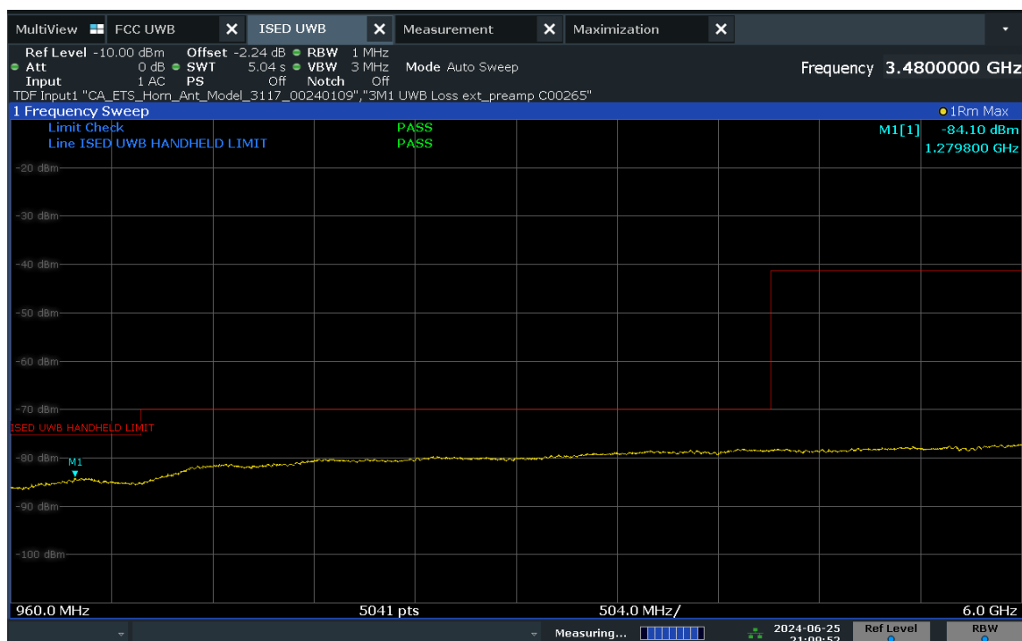
Plot 7-28. ISED Radiated Spurious Emission 960-6000MHz (Ch.9, Config 409, Payload 4093 Ant. Pol. V)
