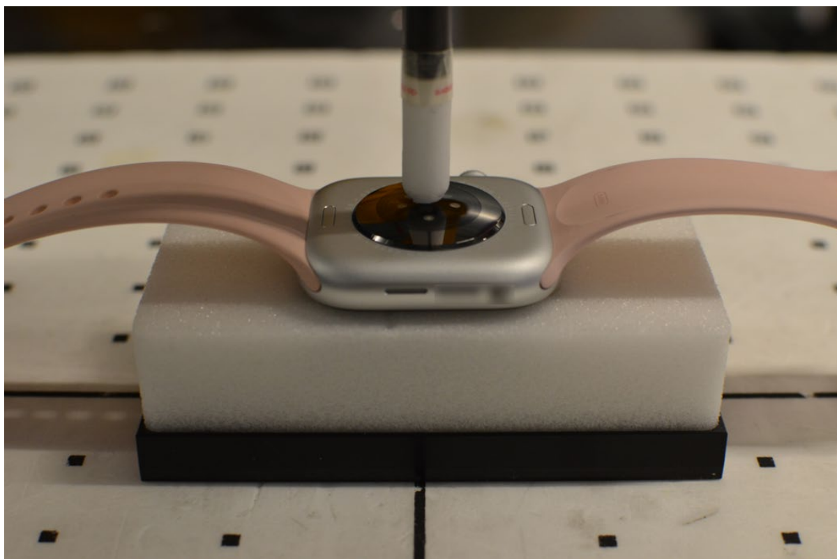
Near Field Power Density Test Setup Photo 10: Aluminum with Sport Wristband, Extremity, Backside at 0.2 cm
