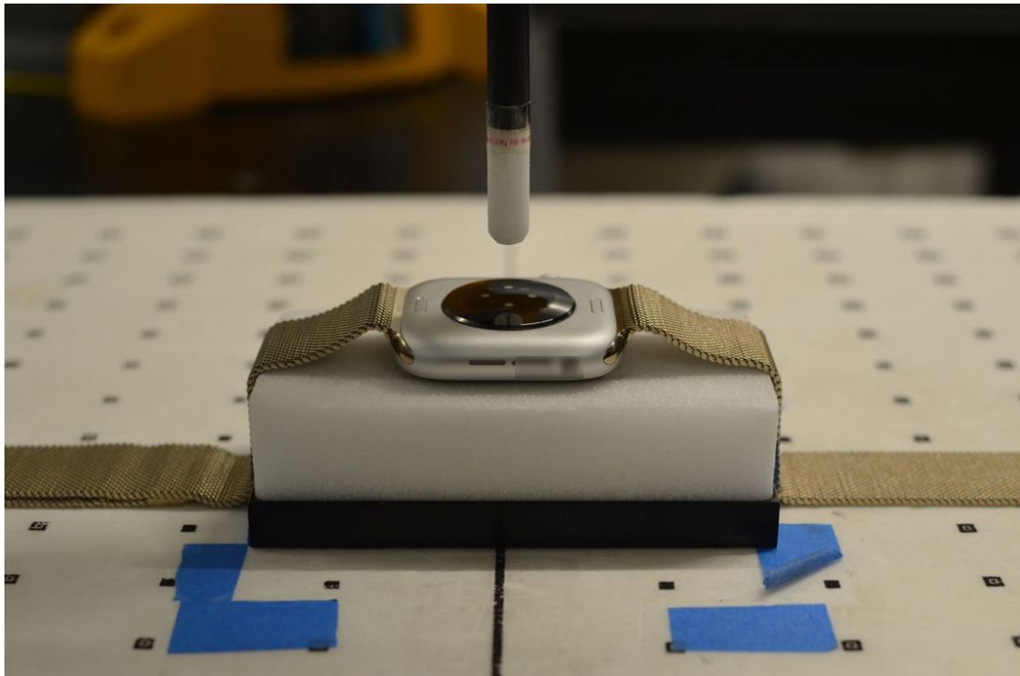
Near Field Power Density Test Setup Photo 13: Aluminum with Metal Loops Wristband, Extremity, Backside at 0.75 cm
