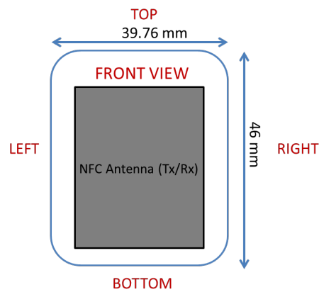
Figure F-2 NFC Antenna Locations
