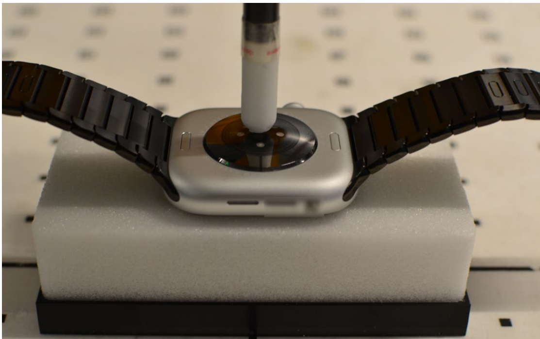
Near Field Power Density Test Setup Photo 11: Aluminum with Metal Links Wristband, Extremity, Backside at 0.2 cm
