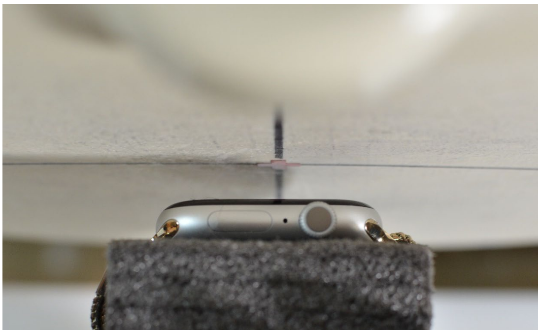
SAR Test Setup Photo 3: Aluminum with Metal Loops Wristband, Head, Front Side at 1.0 cm
