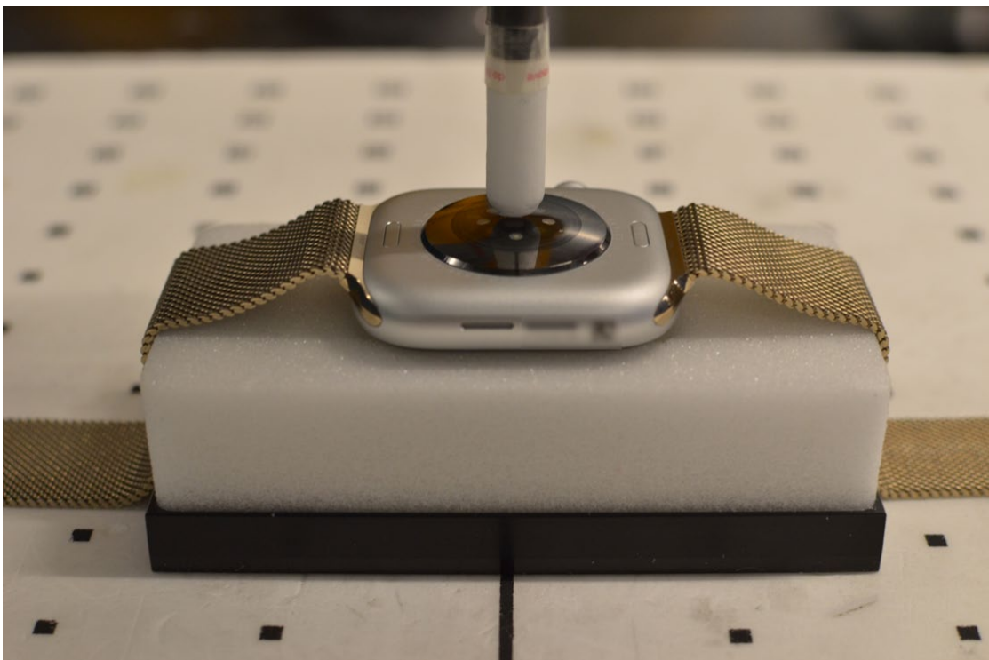
Near Field Power Density Test Setup Photo 12: Aluminum with Metal Loops Wristband, Extremity, Backside at 0.2 cm
