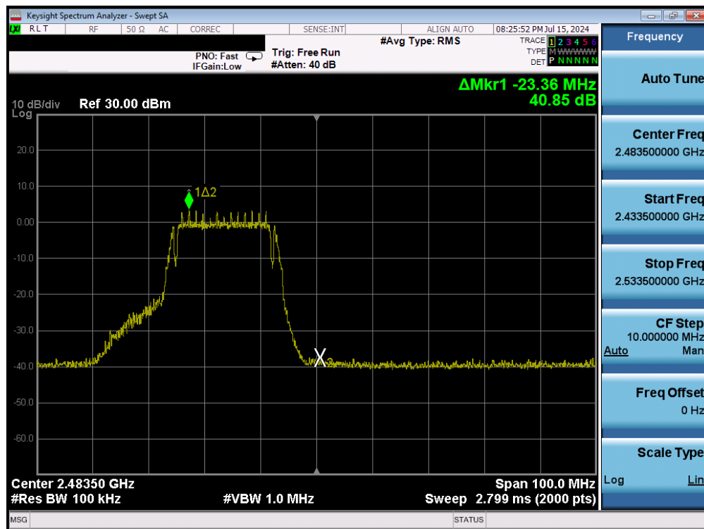
Plot 7-32. Band Edge Plot (802.11g – Ch. 12) – 6Mbps
