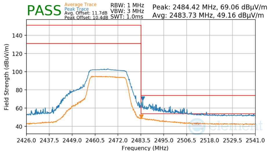
Plot 7-63. Radiated Restricted Upper Band Edge Measurement
