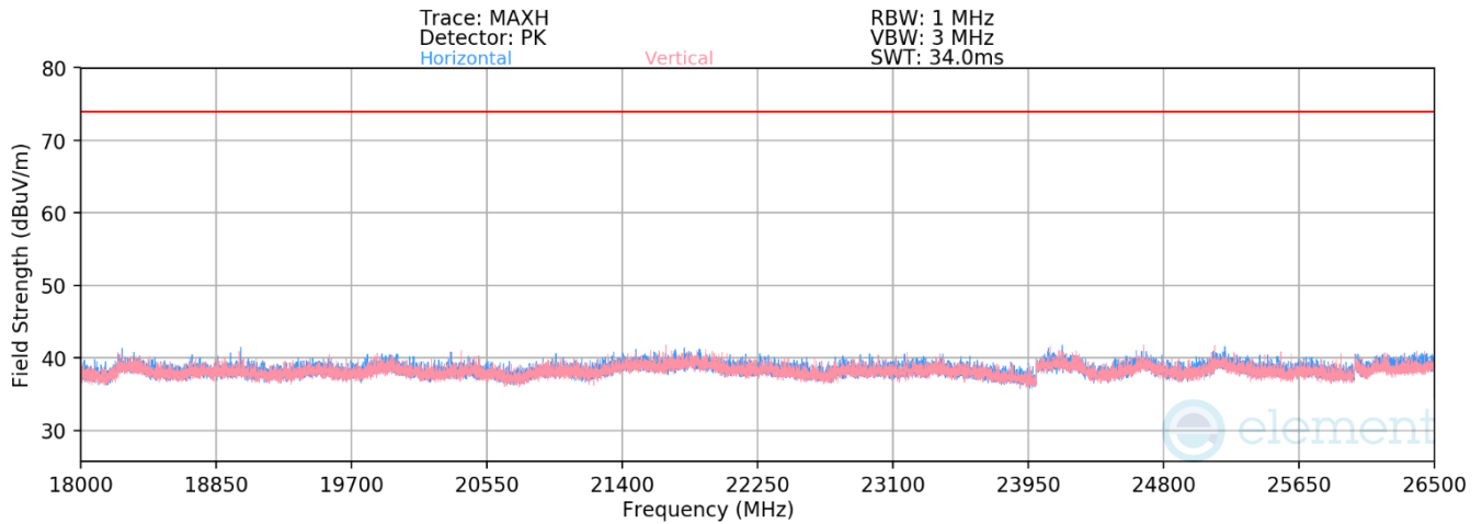
Plot 7-54. Radiated Spurious Emissions Above 18GHz (802.11b – Ch. 6)
