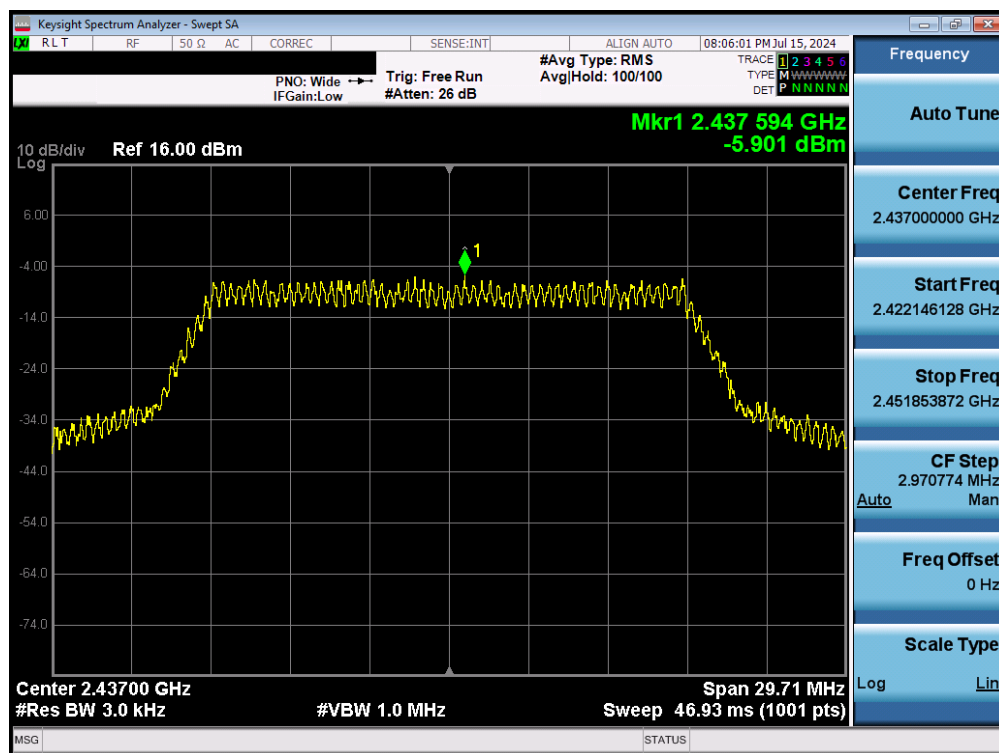
Plot 7-20. Power Spectral Density Plot (802.11n - Ch. 6) - MCS0
