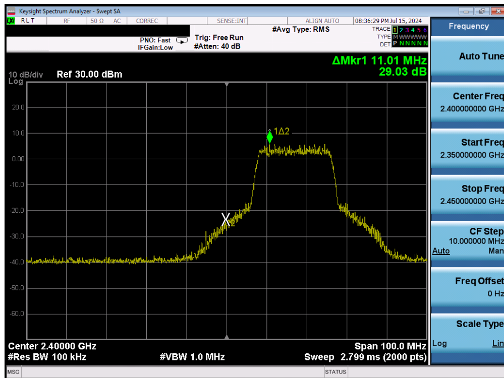
Plot 7-41. Band Edge Plot (802.11n – Ch. 2) – MCS7
