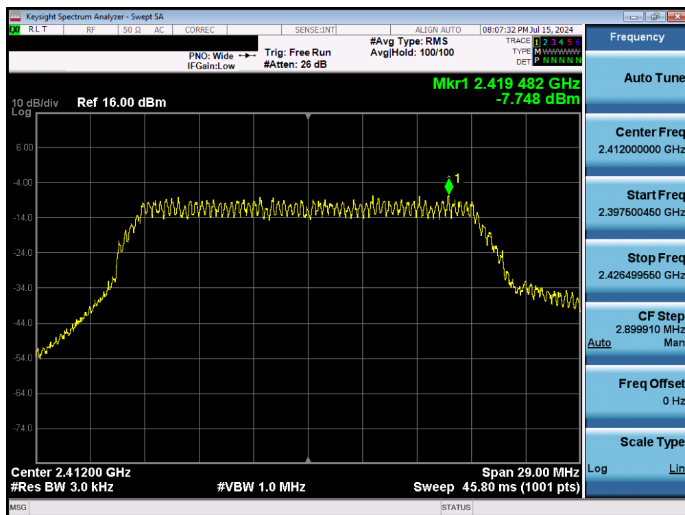
Plot 7-22. Power Spectral Density Plot (802.11n – Ch. 1) – MCS7
