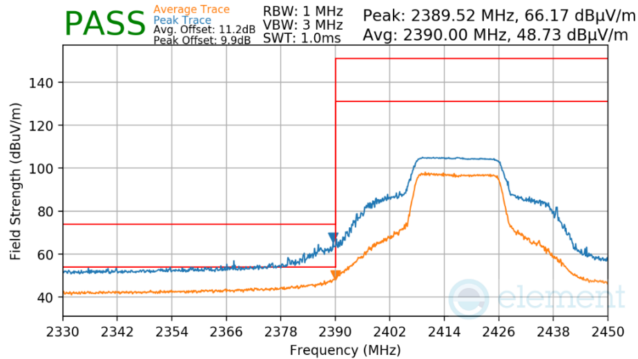
Plot 7-60. Radiated Restricted Lower Band Edge Measurement
