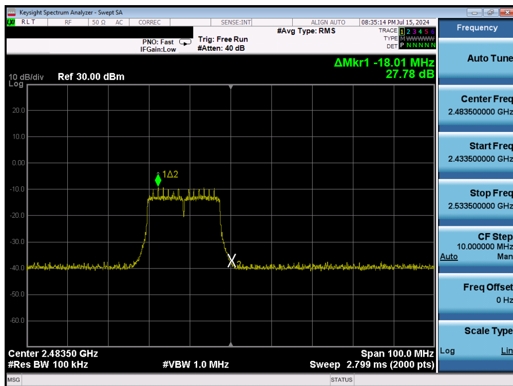
Plot 7-39. Band Edge Plot (802.11n – Ch. 13) – MCS0
