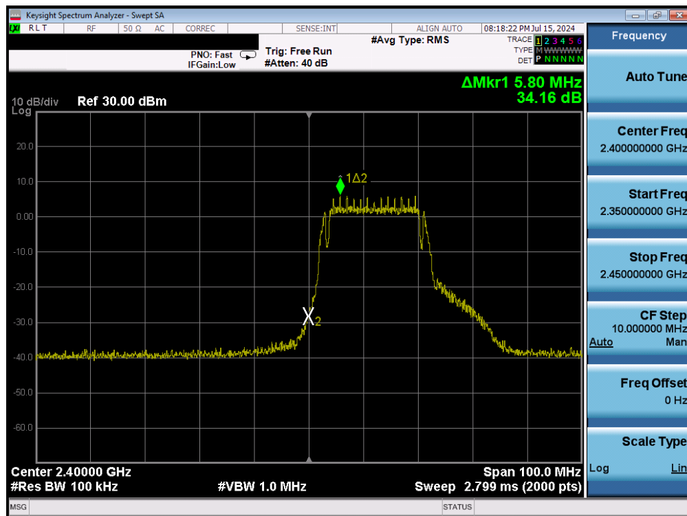
Plot 7-28. Band Edge Plot (802.11g – Ch. 1) – 6Mbps
