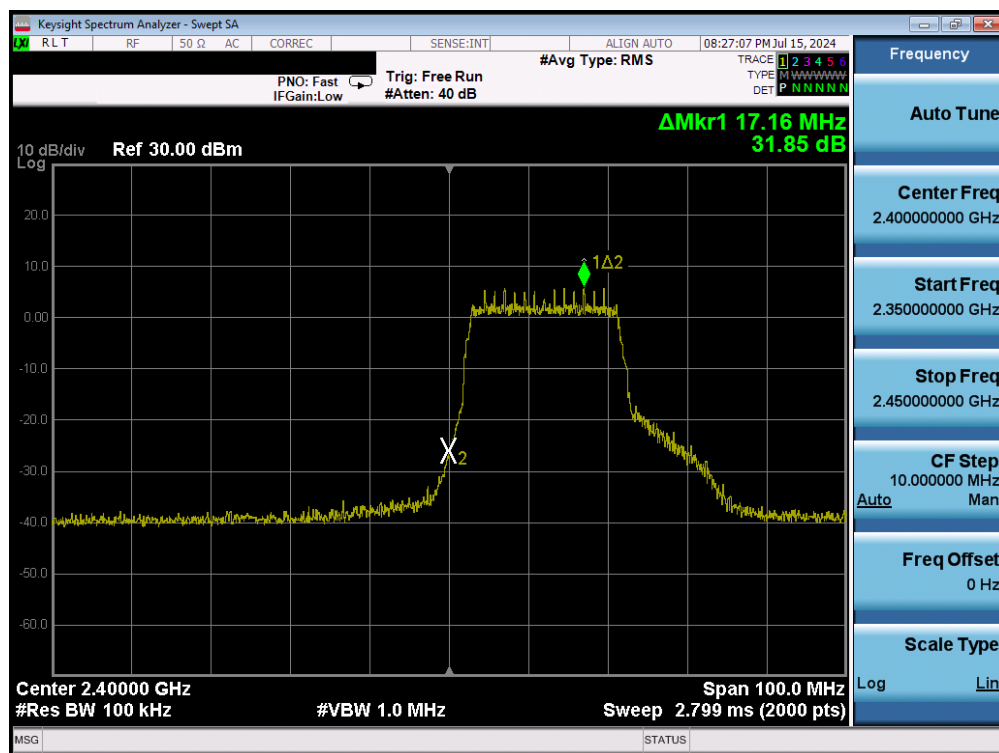
Plot 7-34. Band Edge Plot (802.11n – Ch. 1) – MCS0
