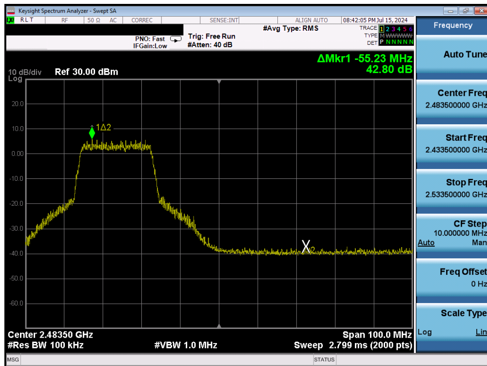
Plot 7-42. Band Edge Plot (802.11n – Ch. 10) – MCS7
