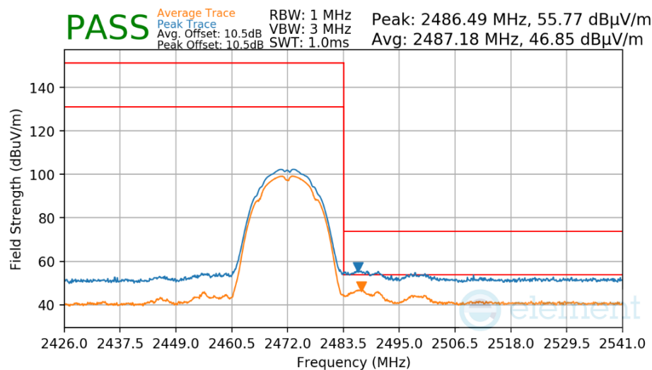
Plot 7-58. Radiated Restricted Upper Band Edge Measurement
