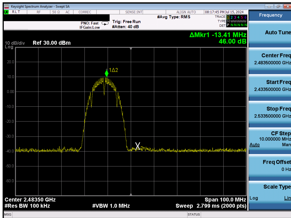
Plot 7-27. Band Edge Plot (802.11b – Ch. 13) – 1Mbps
