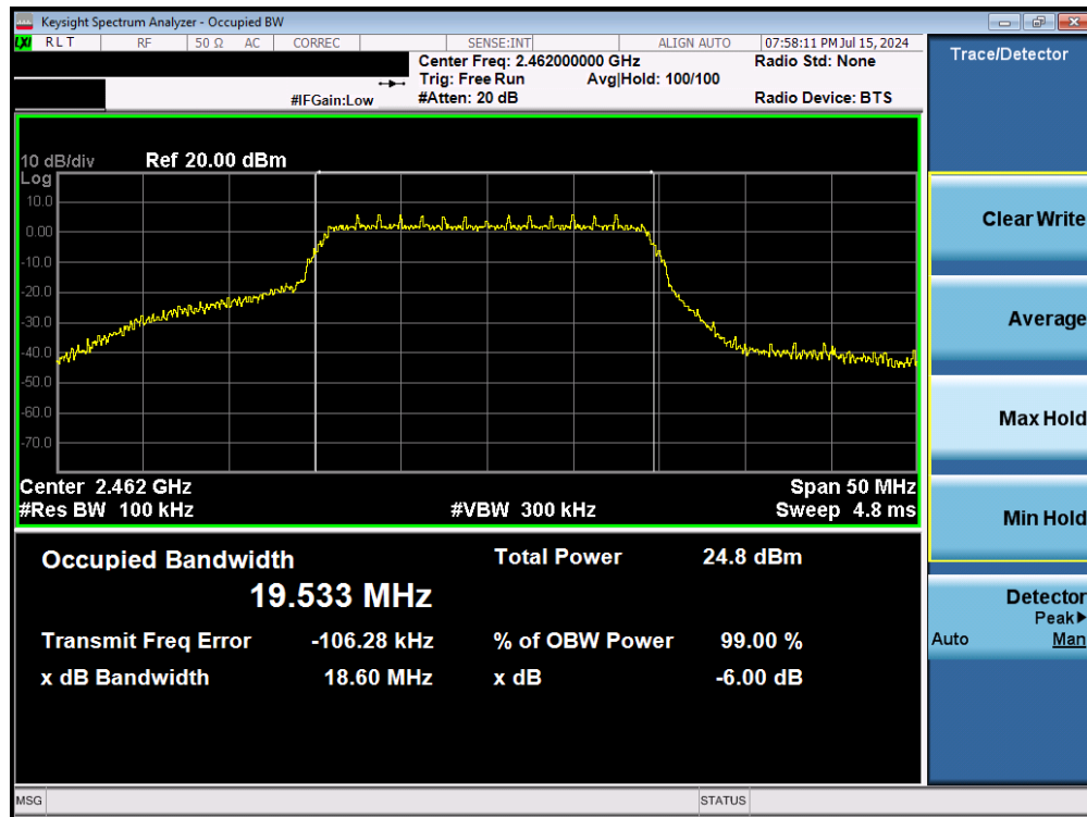
Plot 7-9. 6 dB BW and 99% OBW Plot (802.11n – Ch. 11) – MCS0
