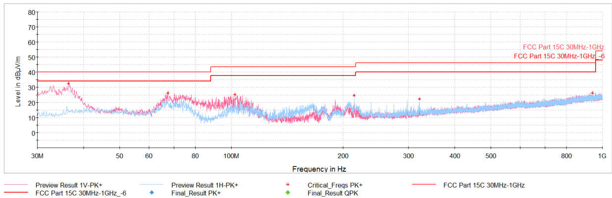
Plot 7-71. Radiated Spurious Emissions below 1GHz 11b Ch.6, with AC/DC Adapter and Magnetic Charger
