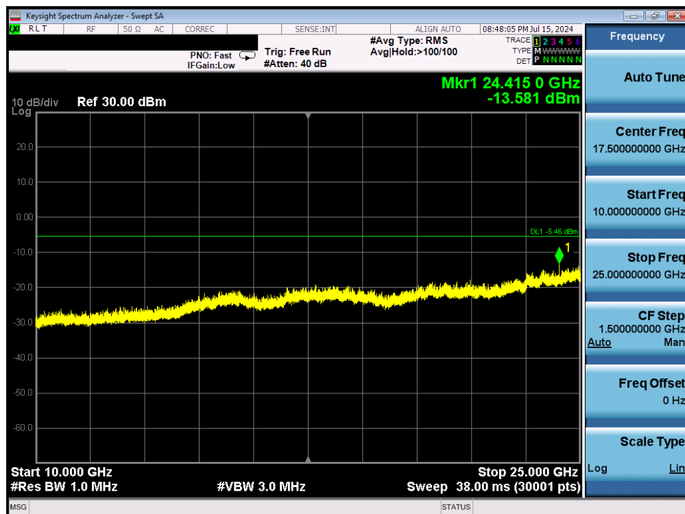
Plot 7-51. Conducted Spurious Plot (802.11b – Ch. 11) – 1Mbps
