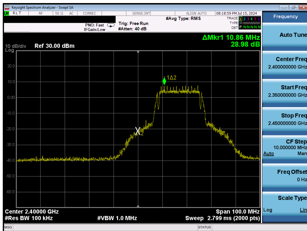
Plot 7-29. Band Edge Plot (802.11g – Ch. 2) – 6Mbps
