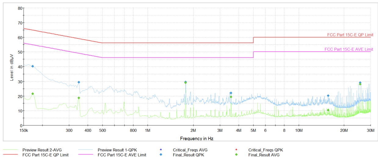
Plot 7-73. AC Line Conducted Plot 802.11b Ch.6 (N, with host PC and Magnetic charger)
