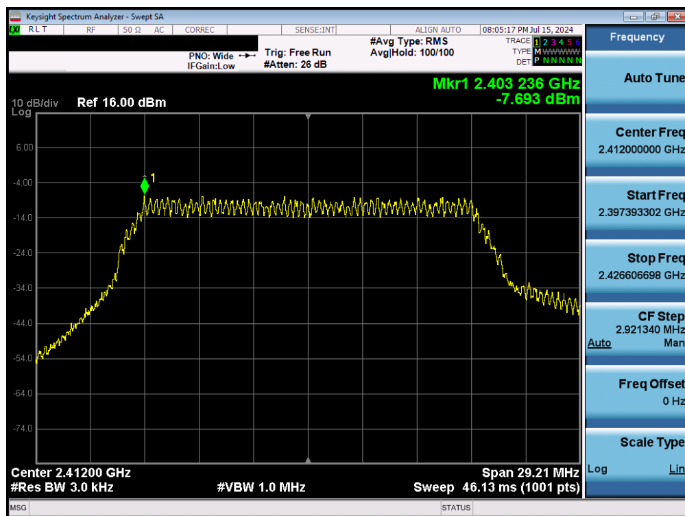
Plot 7-19. Power Spectral Density Plot (802.11n - Ch. 1) - MCS0
