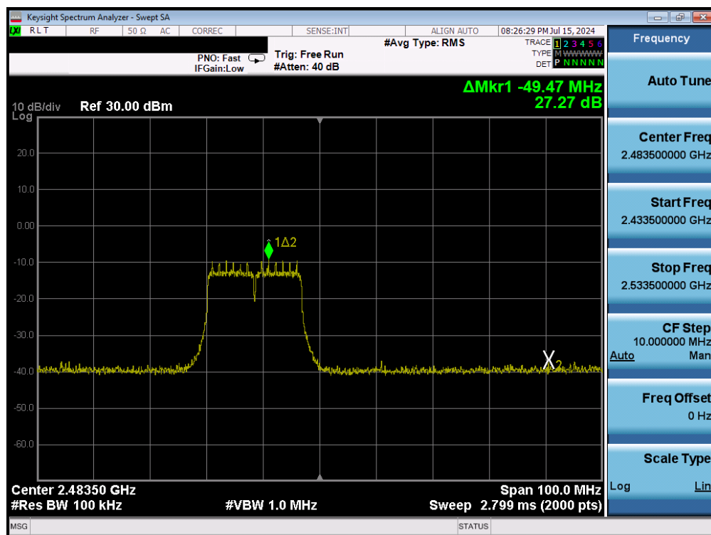
Plot 7-33. Band Edge Plot (802.11g – Ch. 13) – 6Mbps
