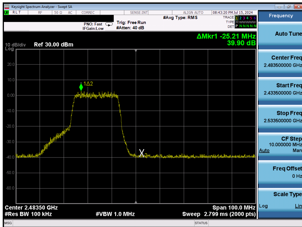
Plot 7-44. Band Edge Plot (802.11n - Ch. 12) - MCS7
