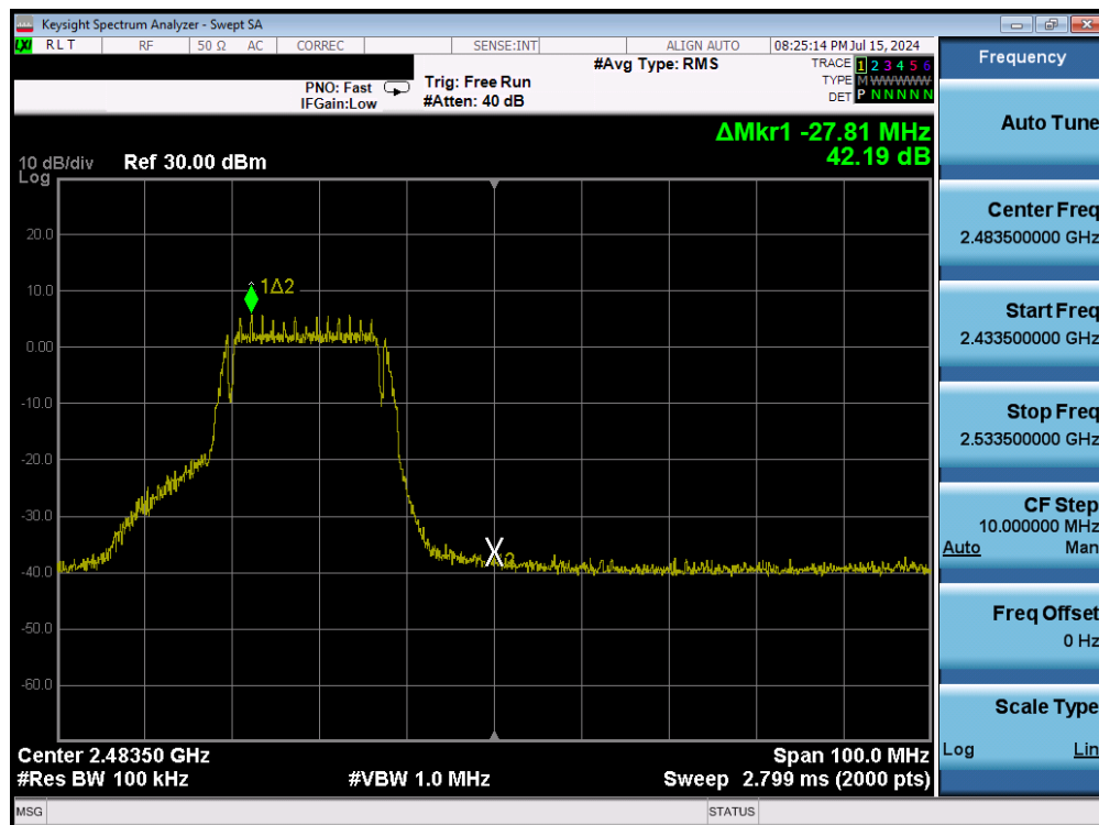
Plot 7-31. Band Edge Plot (802.11g – Ch. 11) – 6Mbps
