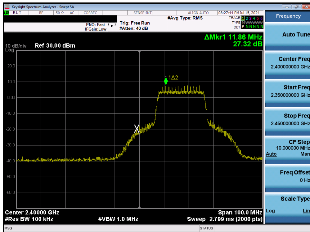
Plot 7-35. Band Edge Plot (802.11n – Ch. 2) – MCS0
