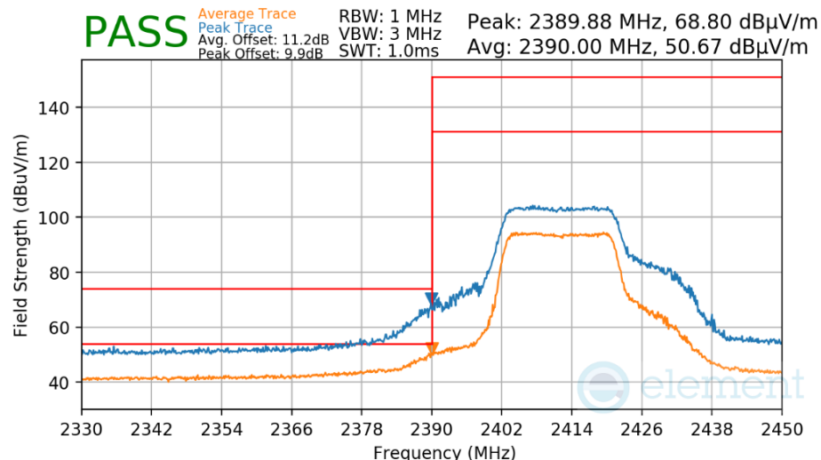
Plot 7-65. Radiated Restricted Lower Band Edge Measurement
