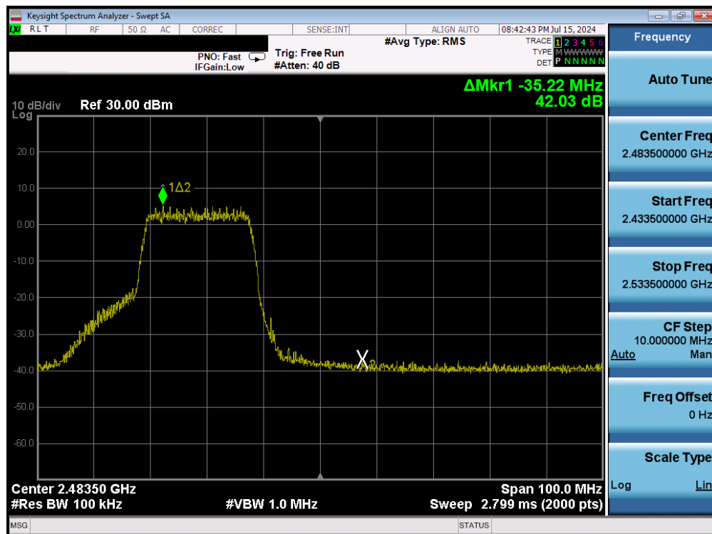
Plot 7-43. Band Edge Plot (802.11n - Ch. 11) - MCS7
