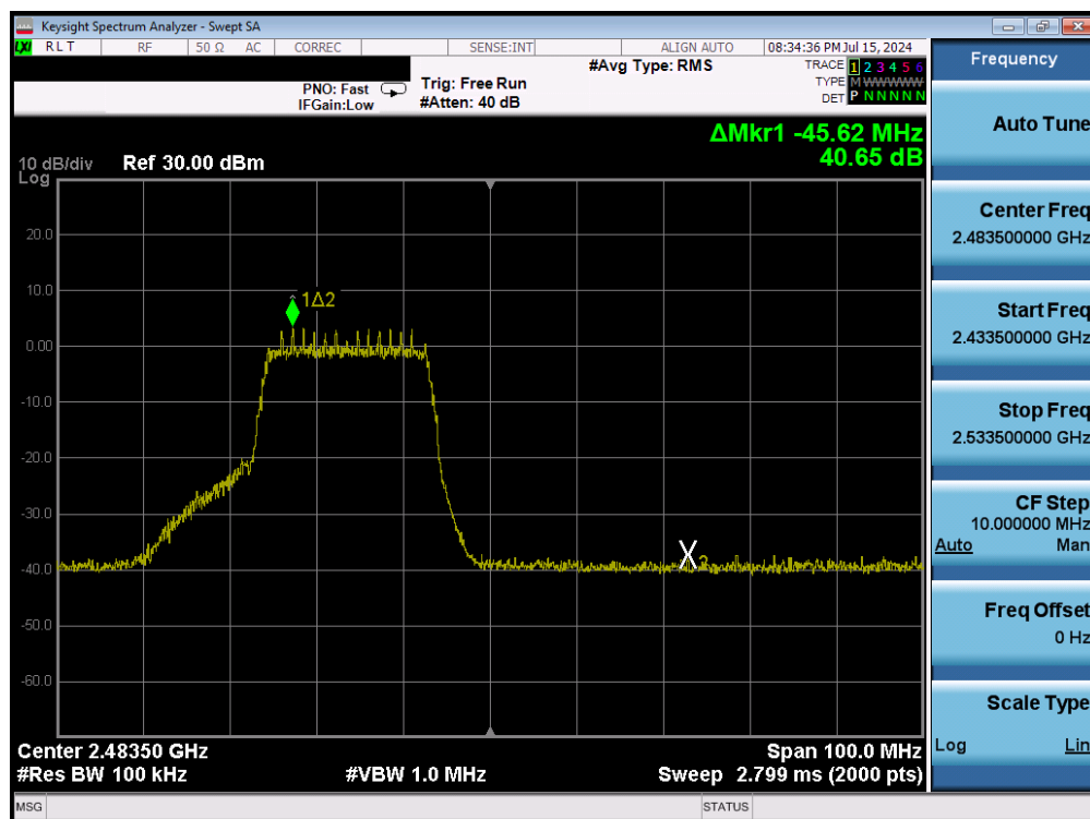
Plot 7-38. Band Edge Plot (802.11n - Ch. 12) - MCS0
