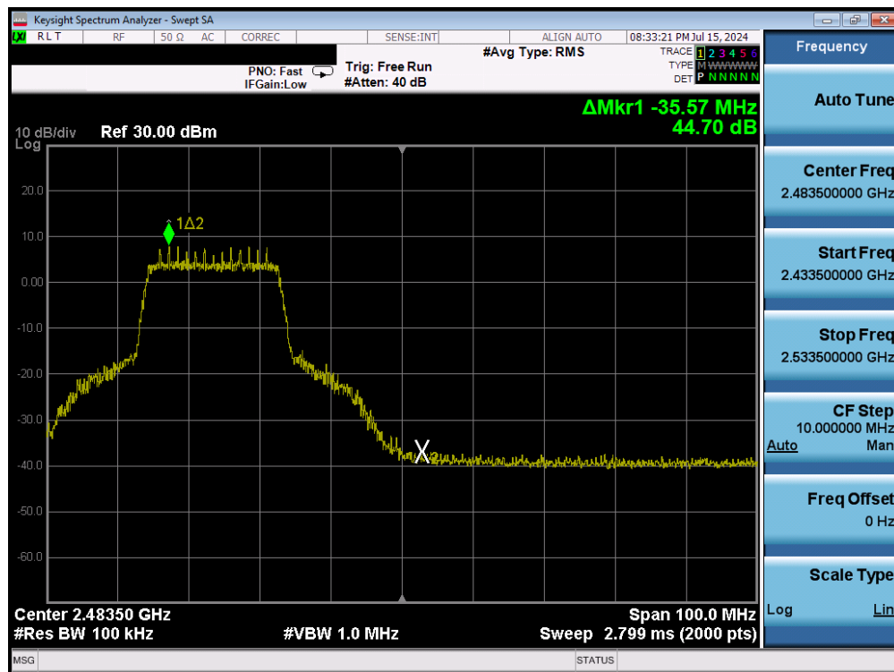
Plot 7-36. Band Edge Plot (802.11n – Ch. 10) – MCS0
