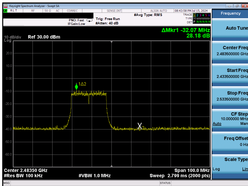
Plot 7-45. Band Edge Plot (802.11n - Ch. 13) - MCS7
