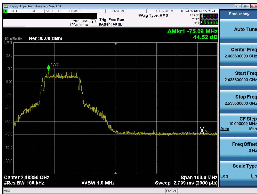
Plot 7-30. Band Edge Plot (802.11g – Ch. 10) – 6Mbps
