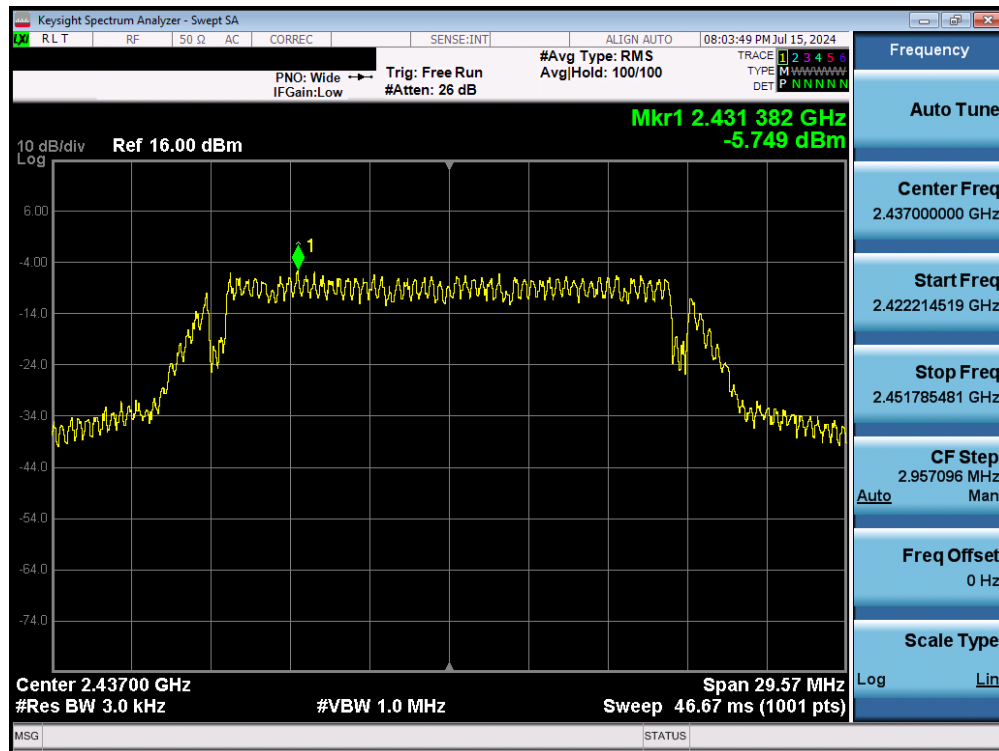
Plot 7-17. Power Spectral Density Plot (802.11g – Ch. 6) – 6Mbps
