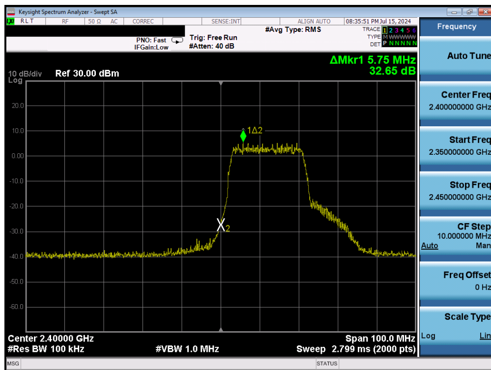
Plot 7-40. Band Edge Plot (802.11n – Ch. 1) – MCS7
