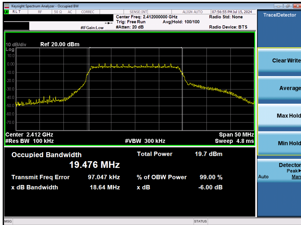
Plot 7-7. 6 dB BW and 99% OBW Plot (802.11n – Ch. 1) – MCS0
