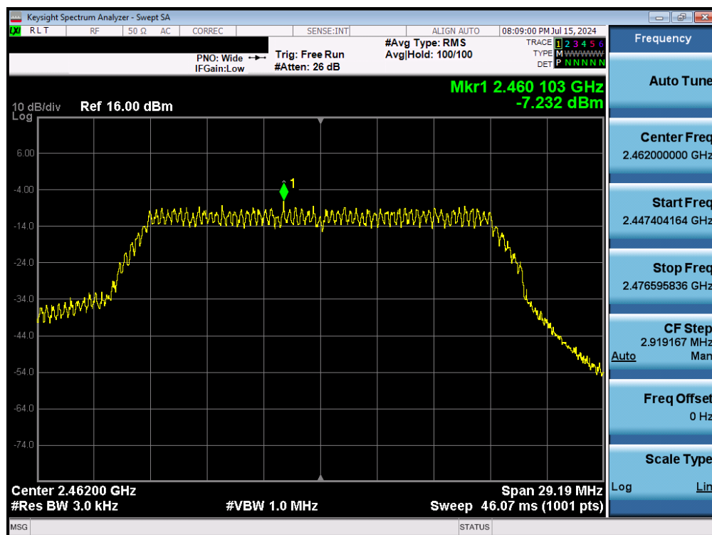
Plot 7-24. Power Spectral Density Plot (802.11n – Ch. 11) – MCS7
