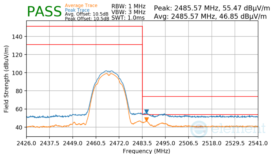
Plot 7-57. Radiated Restricted Upper Band Edge Measurement
