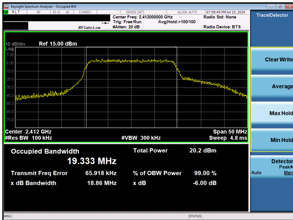
Plot 7-10. 6 dB BW and 99% OBW Plot (802.11n – Ch. 1) – MCS7
