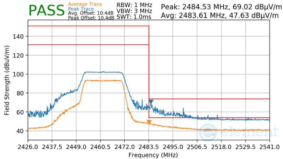
Plot 7-62. Radiated Restricted Upper Band Edge Measurement
