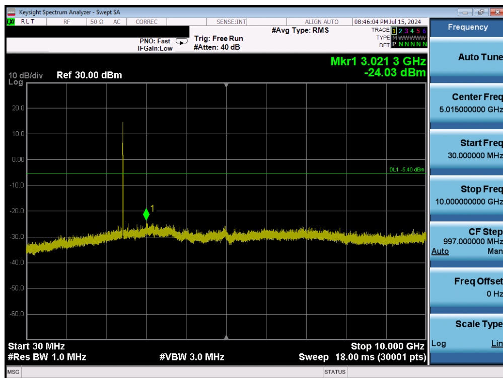
Plot 7-48. Conducted Spurious Plot (802.11b – Ch. 6) – 1Mbps
