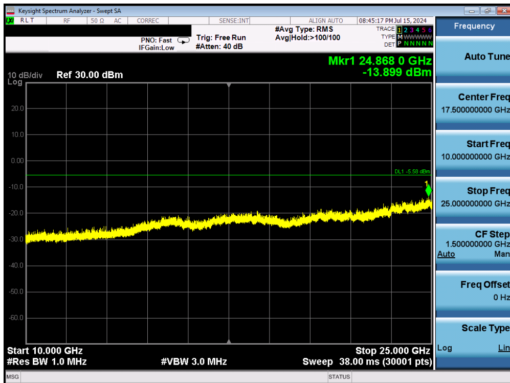
Plot 7-47. Conducted Spurious Plot (802.11b – Ch. 1) – 1Mbps
