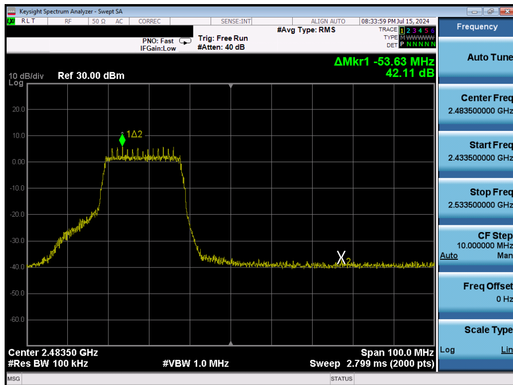
Plot 7-37. Band Edge Plot (802.11n - Ch. 11) - MCS0
