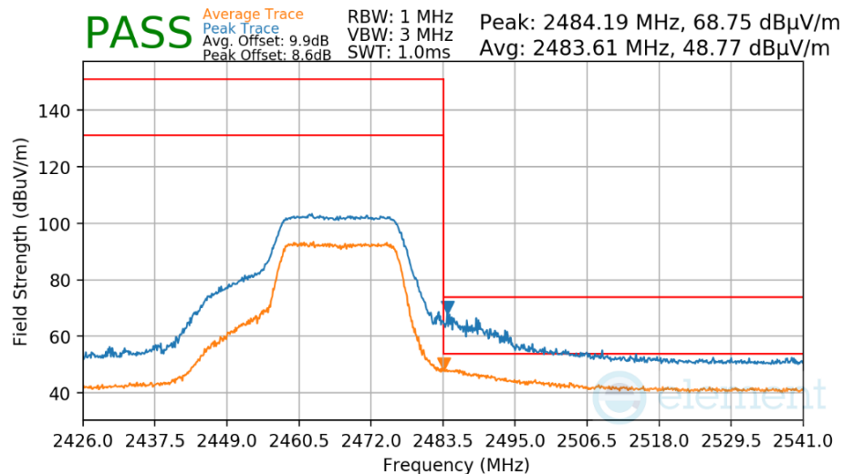
Plot 7-69. Radiated Restricted Upper Band Edge Measurement
