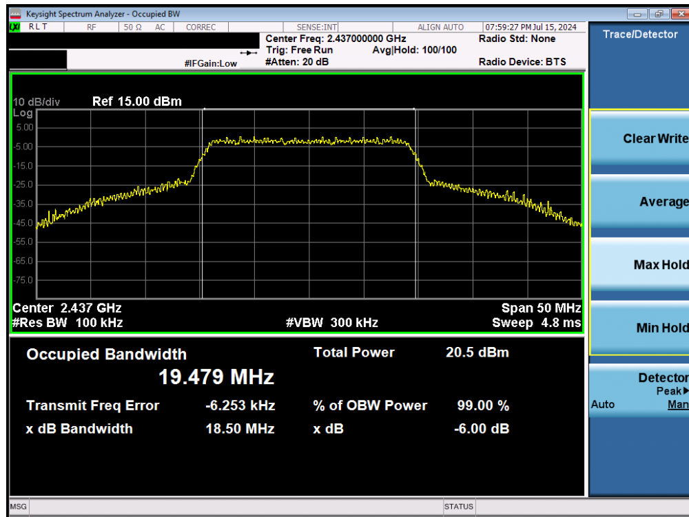
Plot 7-11. 6 dB BW and 99% OBW Plot (802.11n – Ch. 6) – MCS7
