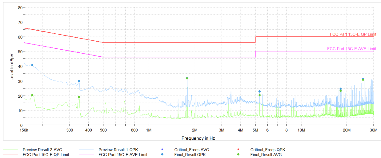
Plot 7-72. AC Line Conducted Plot 802.11b Ch.6 (L1, with host PC and Magnetic charger)
