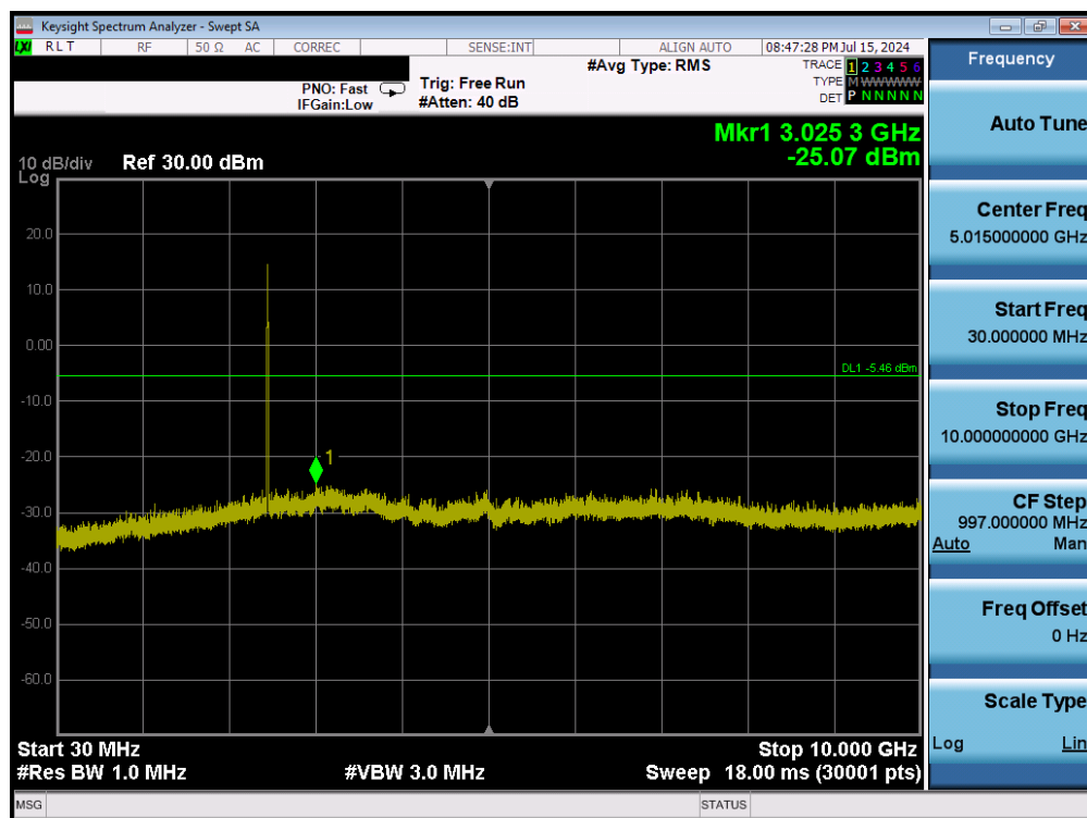
Plot 7-50. Conducted Spurious Plot (802.11b – Ch. 11) – 1Mbps
