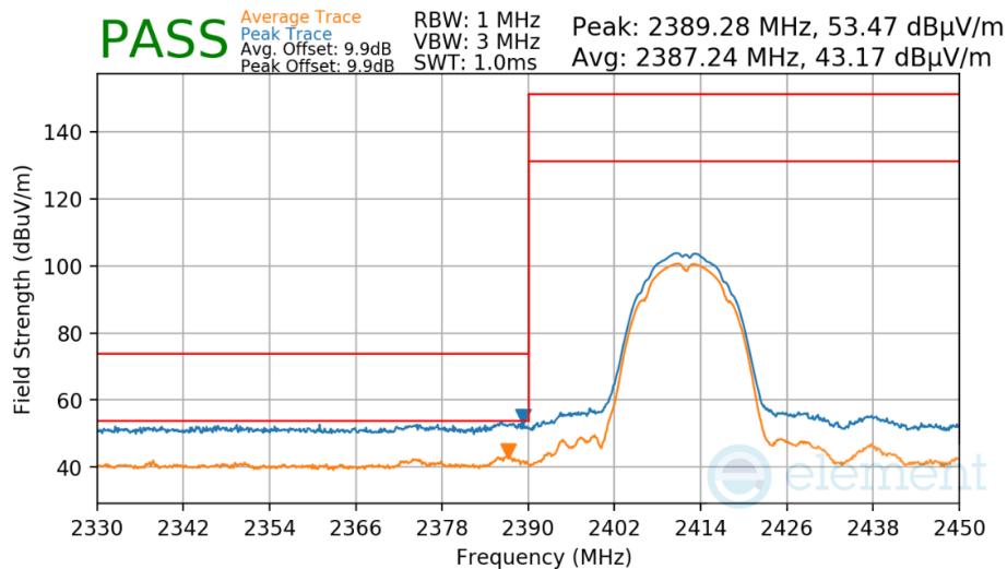
Plot 7-56. Radiated Restricted Lower Band Edge Measurement
