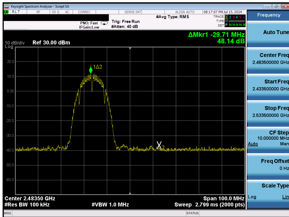
Plot 7-26. Band Edge Plot (802.11b – Ch. 12) – 1Mbps
