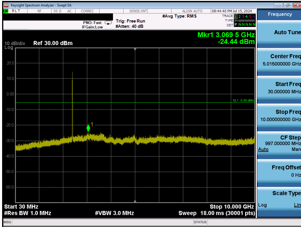
Plot 7-46. Conducted Spurious Plot (802.11b – Ch. 1) – 1Mbps
