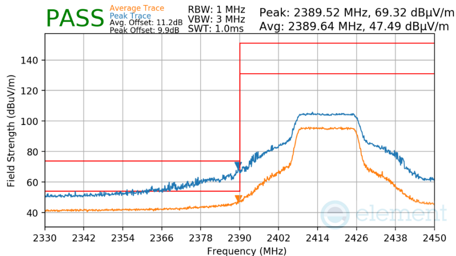
Plot 7-66. Radiated Restricted Lower Band Edge Measurement
