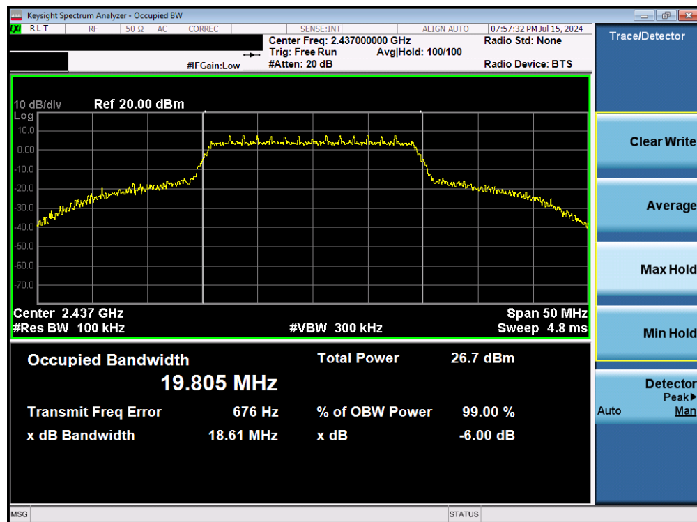
Plot 7-8. 6 dB BW and 99% OBW Plot (802.11n – Ch. 6) – MCS0
