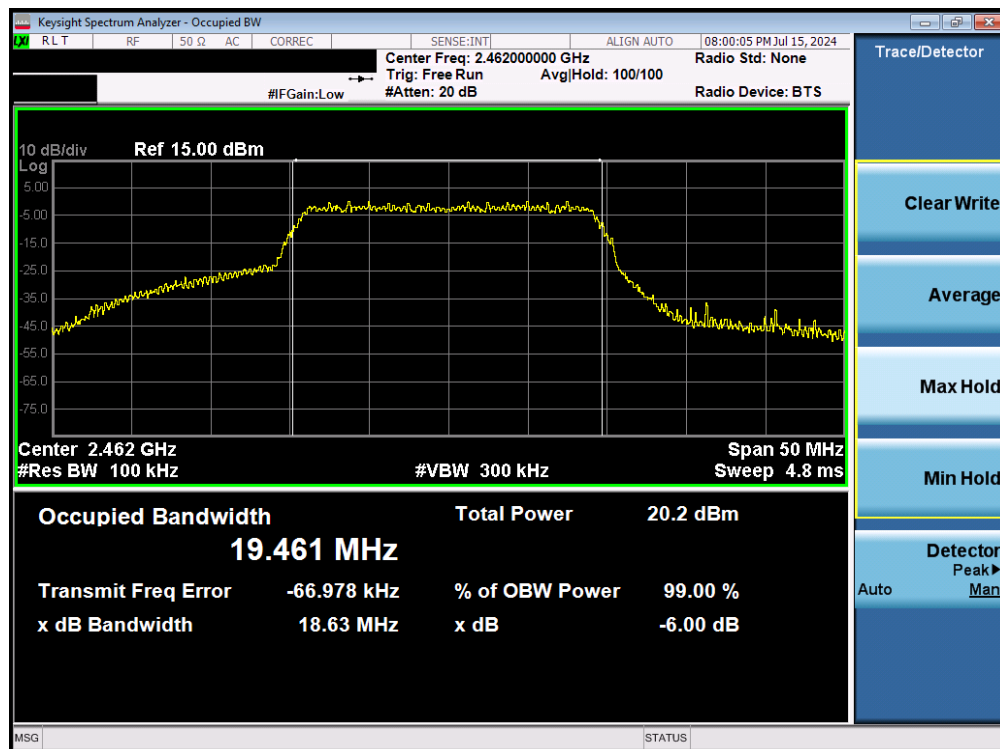
Plot 7-12. 6 dB BW and 99% OBW Plot (802.11n – Ch. 11) – MCS7
