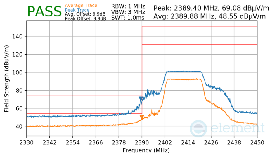
Plot 7-59. Radiated Restricted Lower Band Edge Measurement
