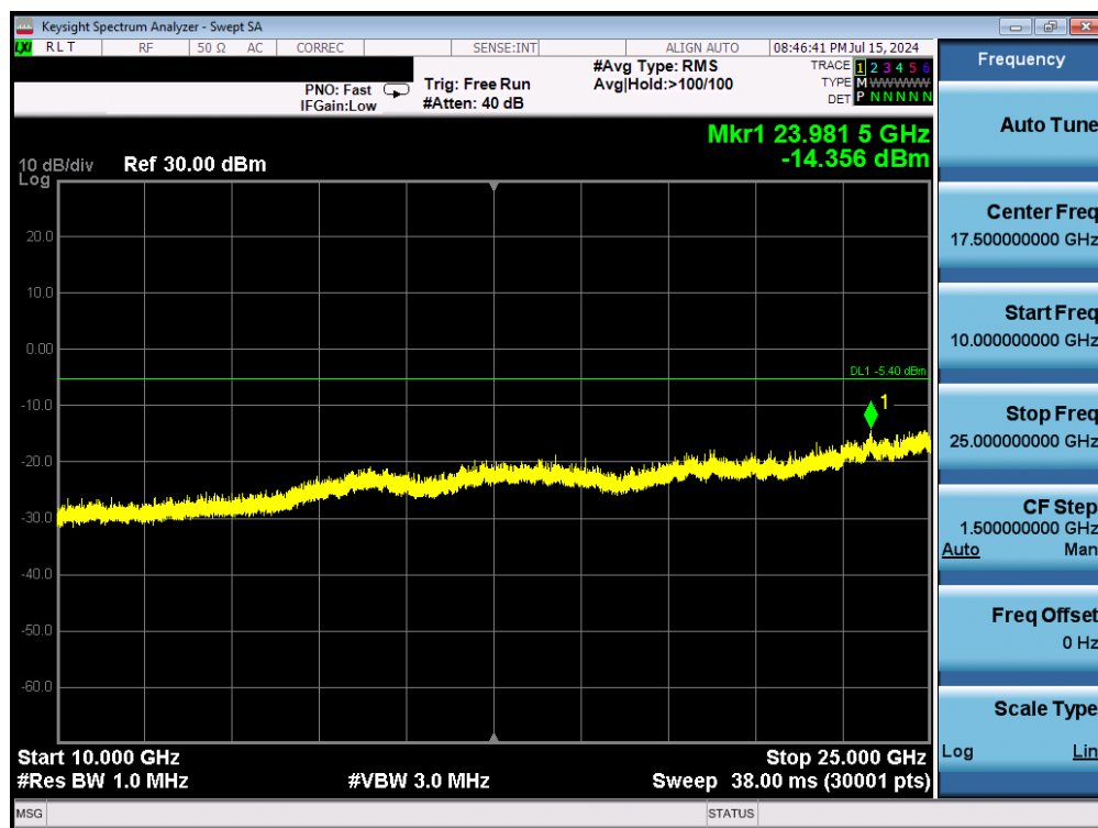
Plot 7-49. Conducted Spurious Plot (802.11b – Ch. 6) – 1Mbps
