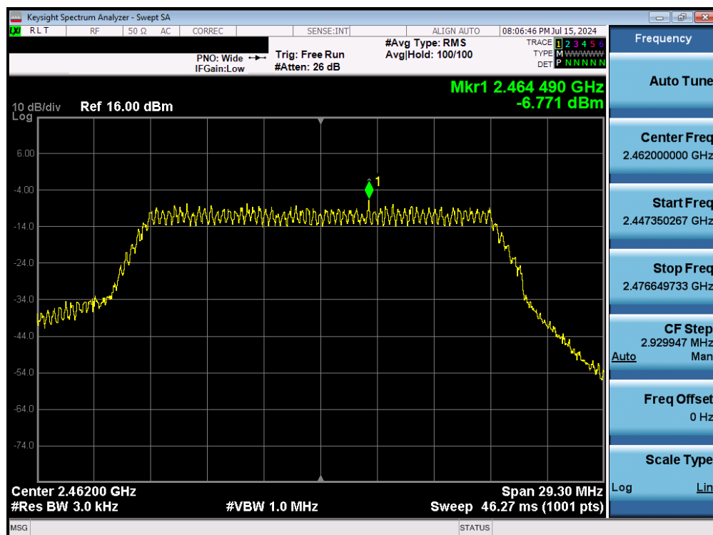
Plot 7-21. Power Spectral Density Plot (802.11n – Ch. 11) – MCS0
