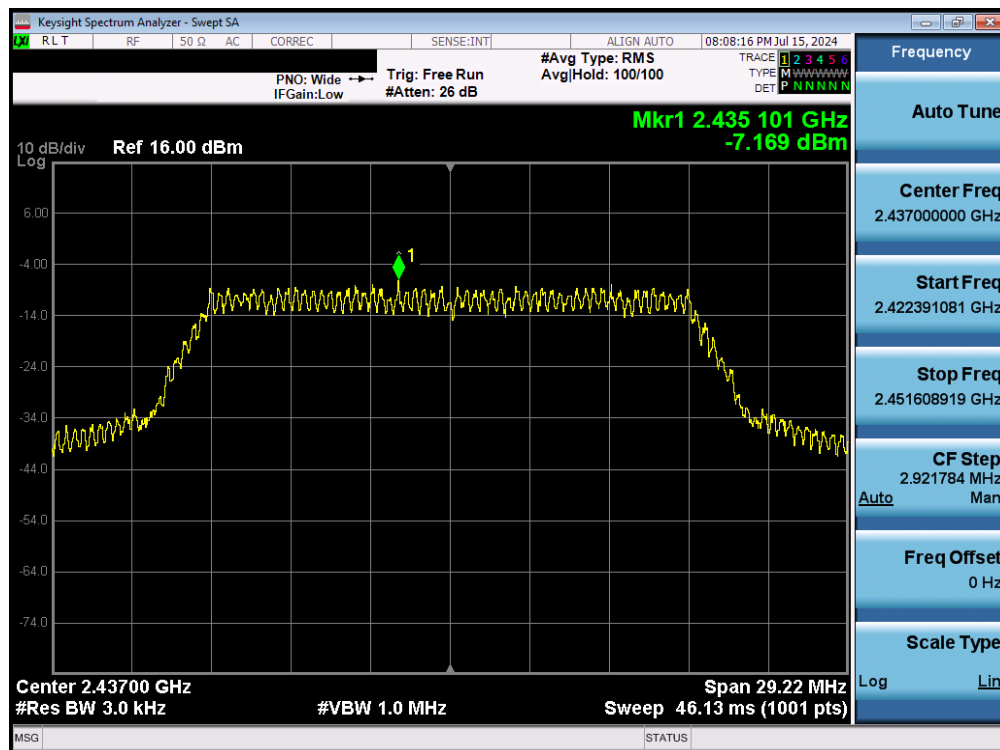
Plot 7-23. Power Spectral Density Plot (802.11n – Ch. 6) – MCS7
