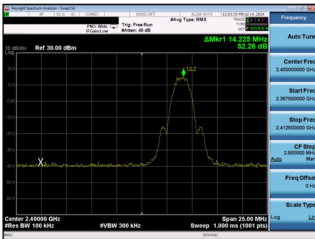
Plot 7-21. Band Edge Plot (Bluetooth (LE), 2Mbps, ePA – Ch. 1)
