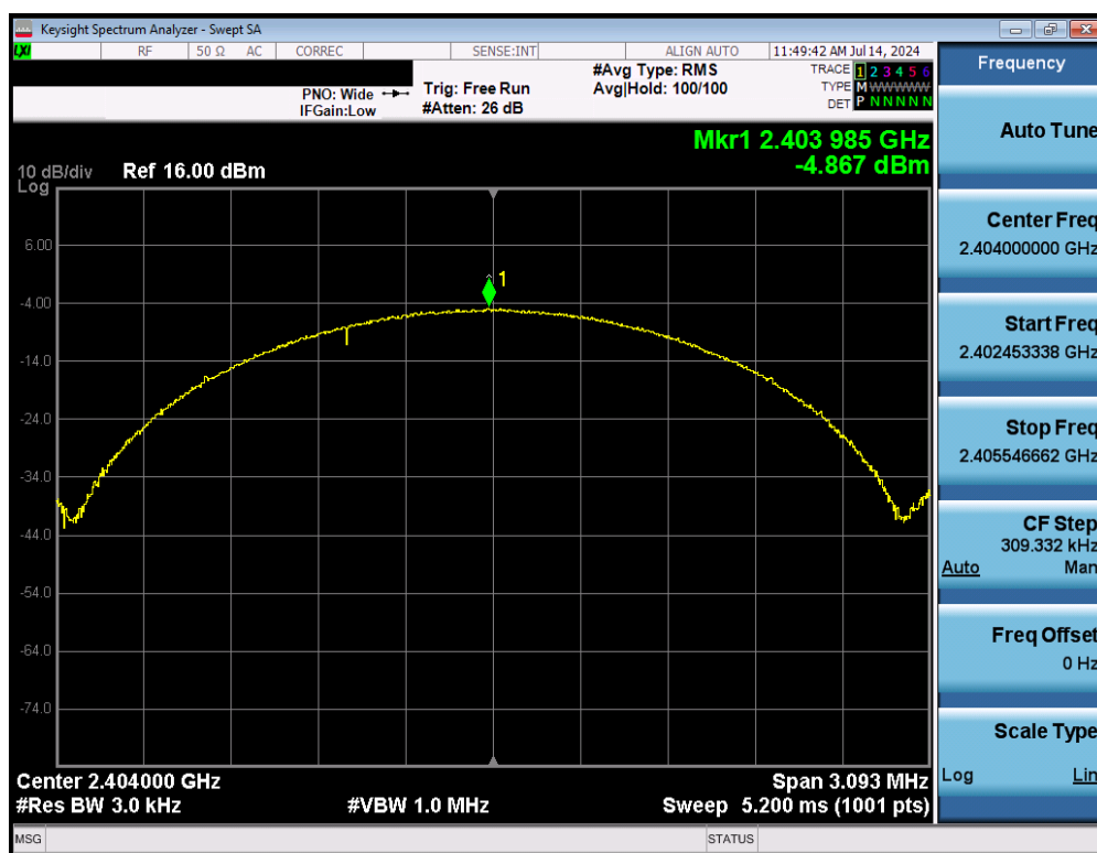
Plot 7-13. Power Spectral Density Plot (Bluetooth (LE), 2Mbps, ePA – Ch. 1)
