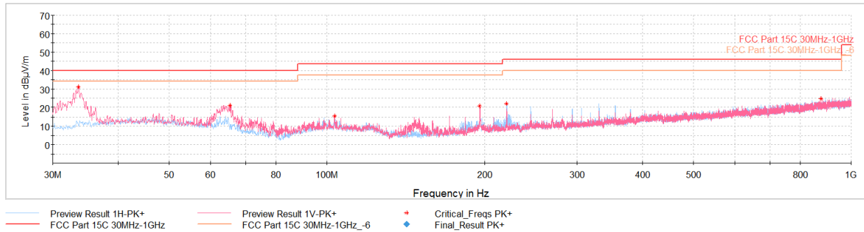
Plot 7-37. Radiated Spurious Emissions Below 1GHz (1Mbps, ePA – Ch.19, Pol. H & V, with AC/DC Adapter + Magnetic Charger)
