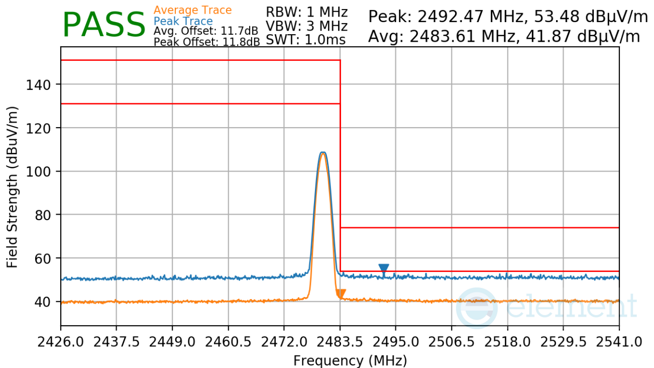
Plot 7-34. Radiated Restricted Upper Band Edge Measurement (Average & Peak)
