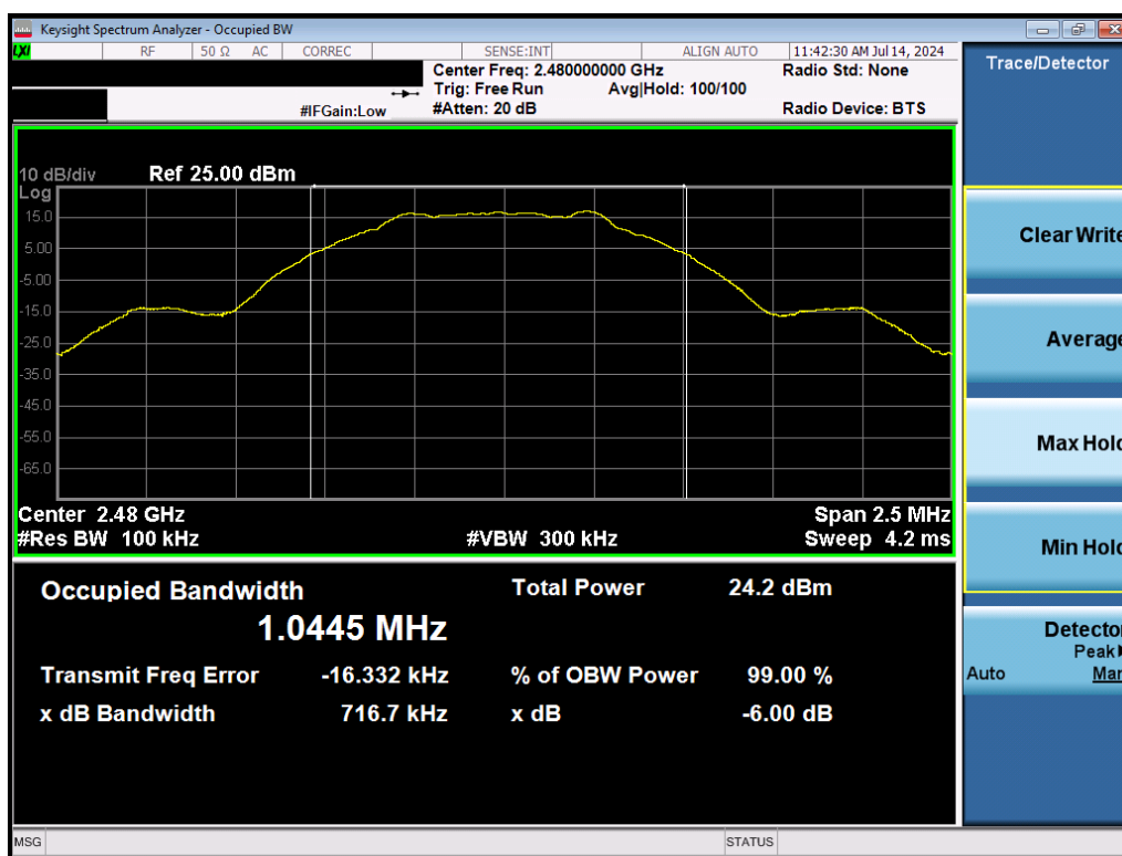
Plot 7-3. 6dB BW & 99% OBW Plot (Bluetooth (LE), 1Mbps, ePA – Ch. 39)
