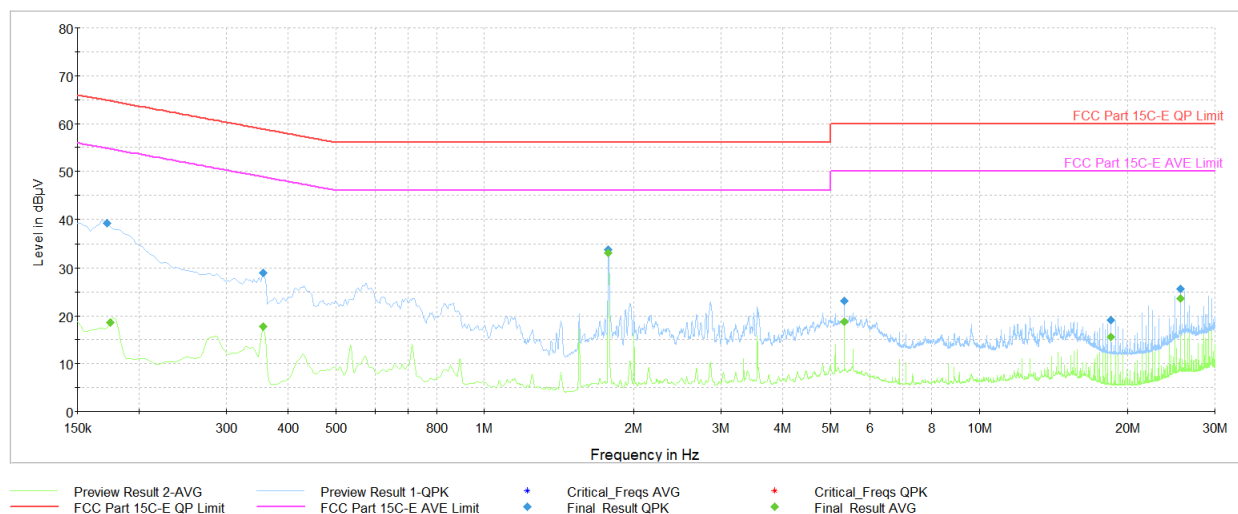
Plot 7-39. AC Line Conducted Plot with Bluetooth LE (N, 1Mbps ePA – Ch.19, with host PC and Magnetic Charger)
