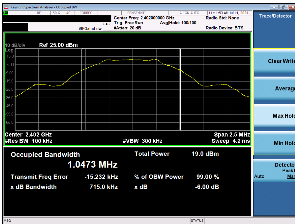
Plot 7-1. 6dB BW & 99% OBW Plot (Bluetooth (LE), 1Mbps, ePA – Ch. 0)
