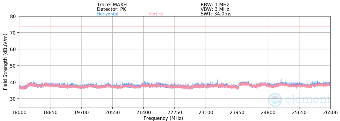
Plot 7-31. Radiated Spurious Emissions Above 18GHz (1Mbps ePA – Ch. 19)
