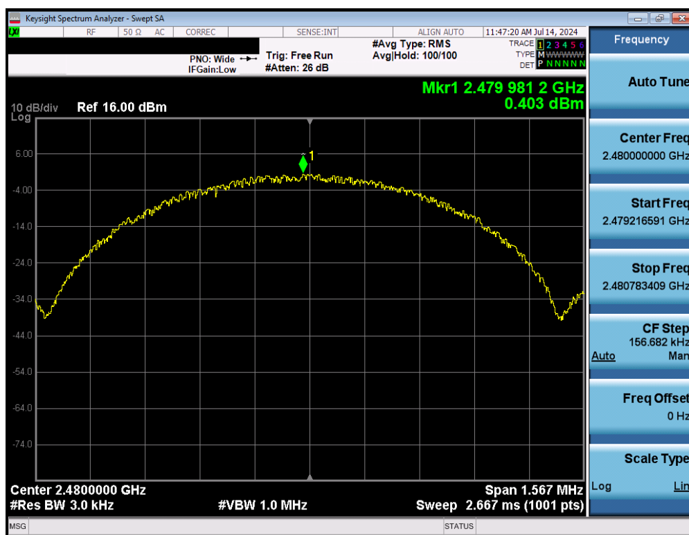
Plot 7-9. Power Spectral Density Plot (Bluetooth (LE), 1Mbps, ePA – Ch. 39)
