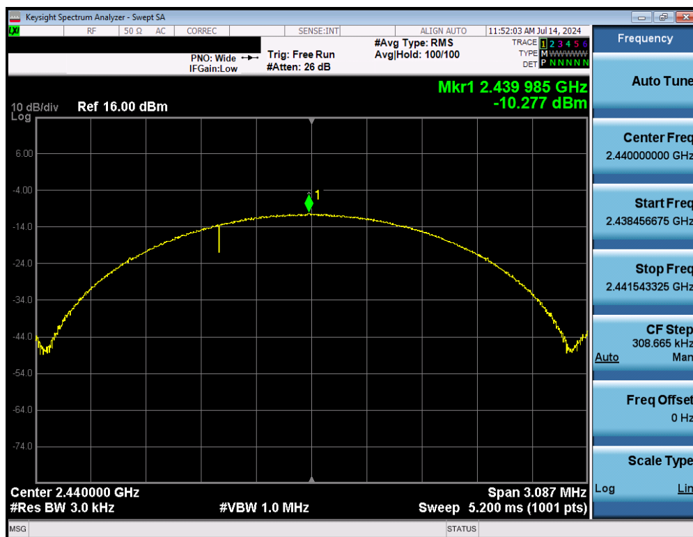
Plot 7-17. Power Spectral Density Plot (Bluetooth (LE), 2Mbps, iPA – Ch. 19)
