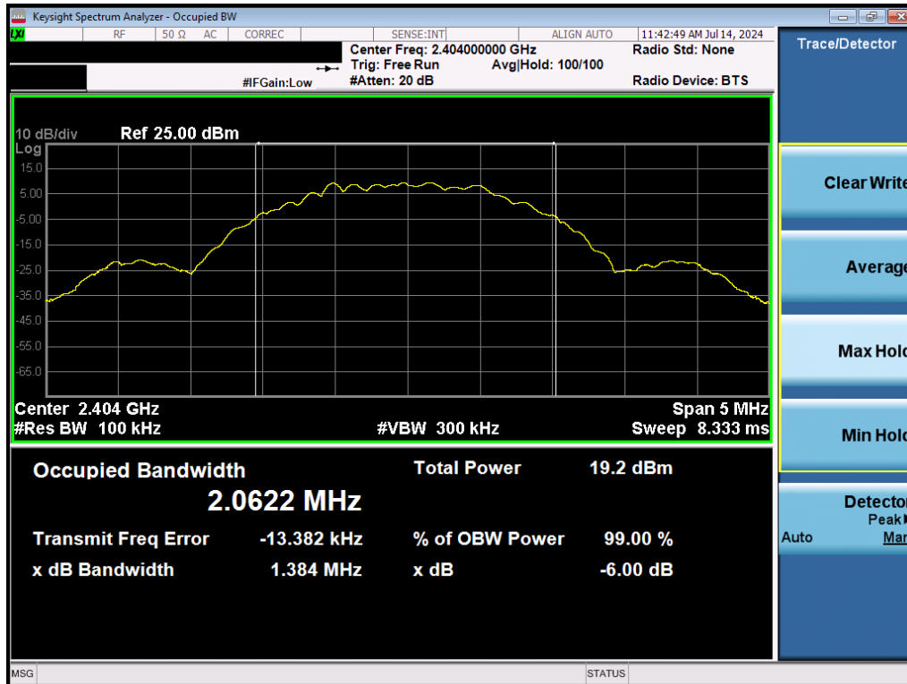
Plot 7-4. 6dB BW & 99% OBW Plot (Bluetooth (LE), 2Mbps, ePA – Ch. 1)
