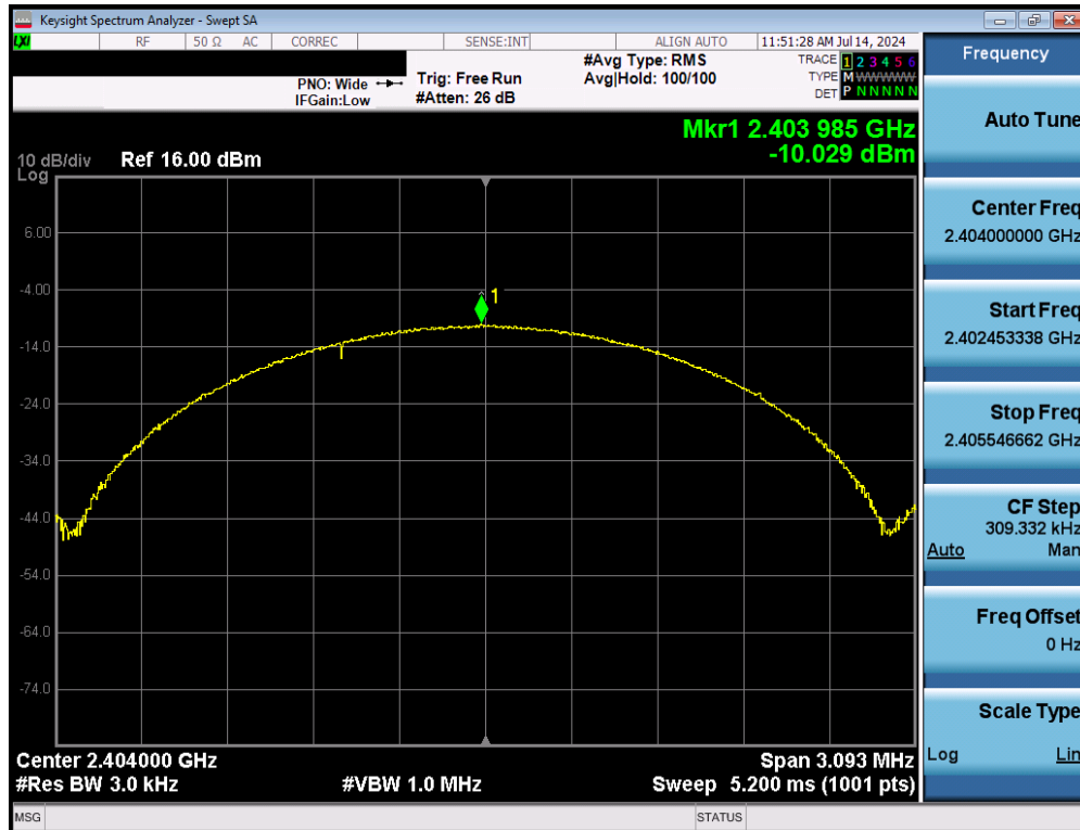
Plot 7-16. Power Spectral Density Plot (Bluetooth (LE), 2Mbps, iPA – Ch. 1)
