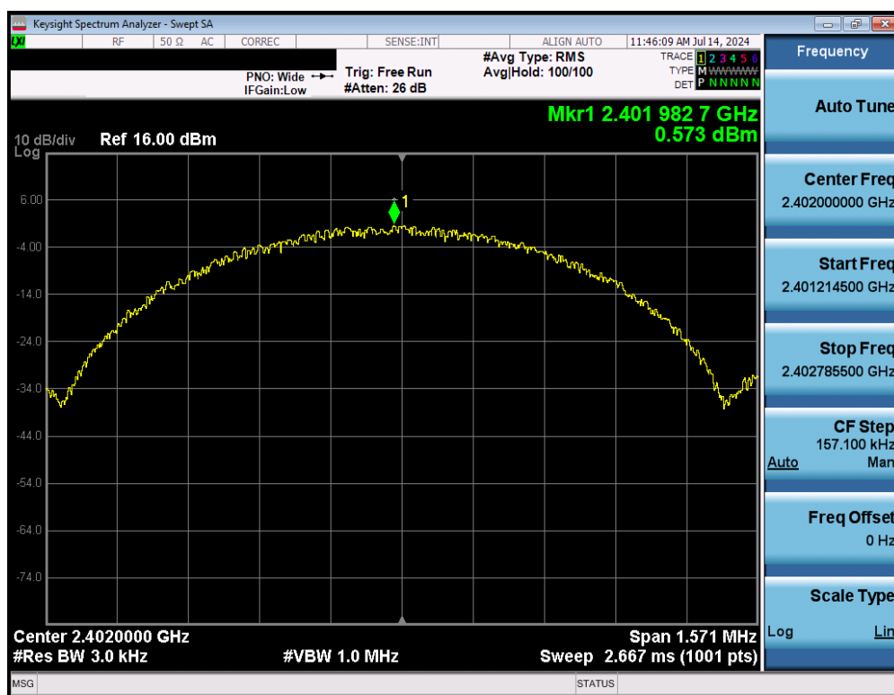
Plot 7-7. Power Spectral Density Plot (Bluetooth (LE), 1Mbps, ePA – Ch. 0)
