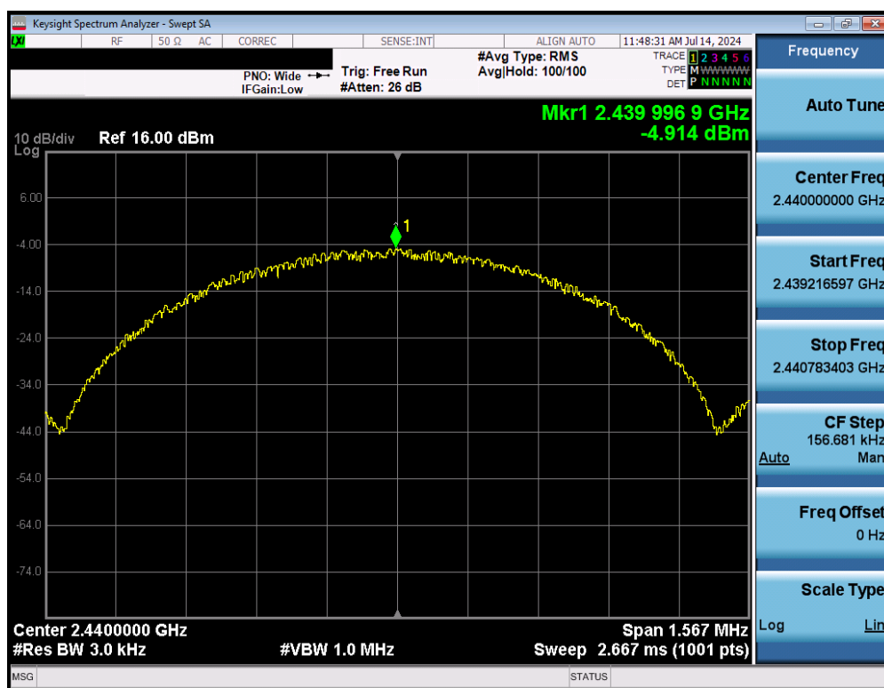
Plot 7-11. Power Spectral Density Plot (Bluetooth (LE), 1Mbps, iPA – Ch. 19)
