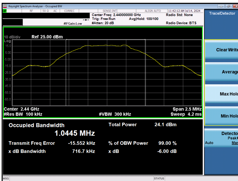
Plot 7-2. 6dB BW & 99% OBW Plot (Bluetooth (LE), 1Mbps, ePA – Ch. 19)
