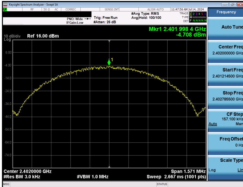
Plot 7-10. Power Spectral Density Plot (Bluetooth (LE), 1Mbps, iPA – Ch. 0)
