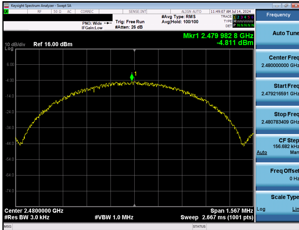
Plot 7-12. Power Spectral Density Plot (Bluetooth (LE), 1Mbps, iPA – Ch. 39)
