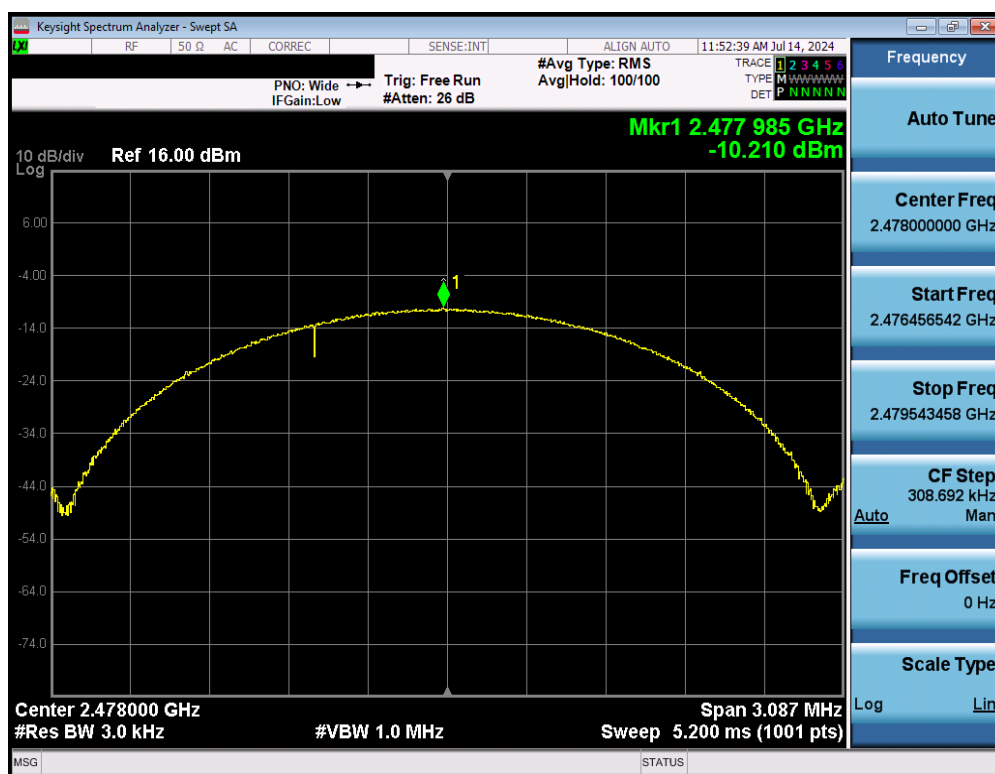
Plot 7-18. Power Spectral Density Plot (Bluetooth (LE), 2Mbps, iPA – Ch. 38)
