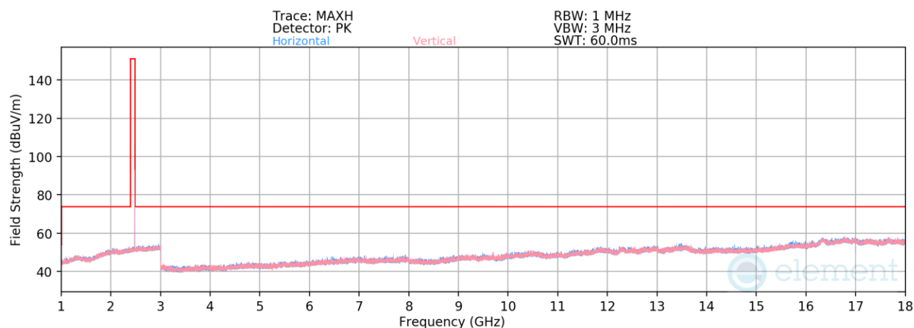
Plot 7-32. Radiated Spurious Emissions 1-18GHz (1Mbps ePA – Ch. 39)
