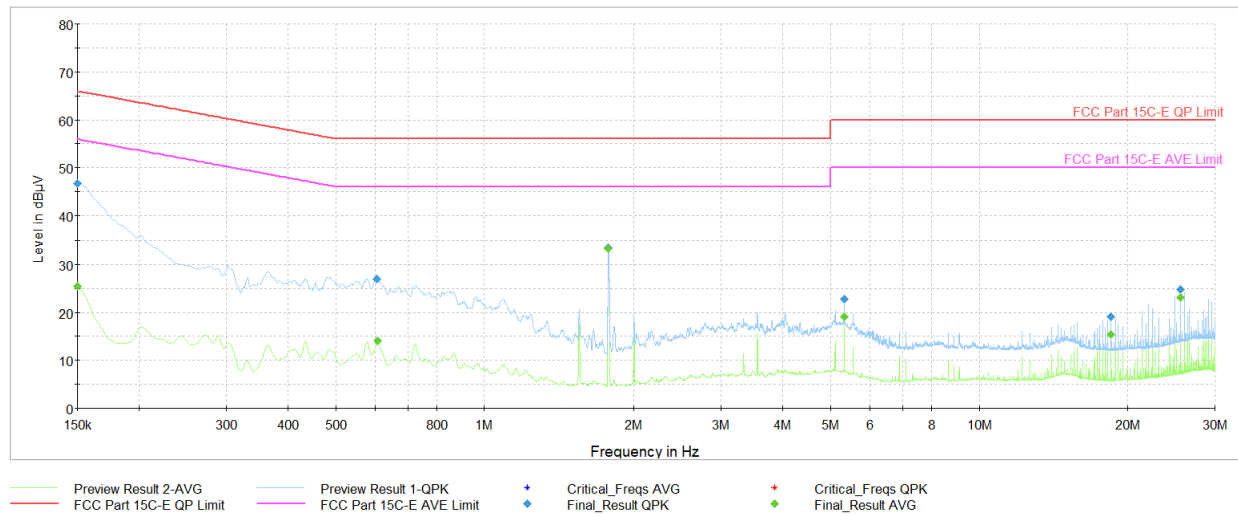
Plot 7-38. AC Line Conducted Plot with Bluetooth LE (L1, 1Mbps ePA – Ch.19 with host PC and Magnetic Charger)
