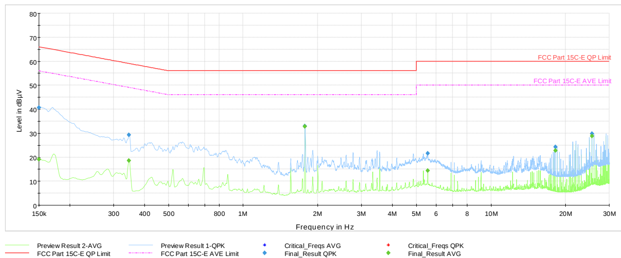
Plot 7-39. AC Line Conducted Plot with Bluetooth HDR (N, 4Mbps ePA - Ch.38 with host PC + Magnetic Charger)
