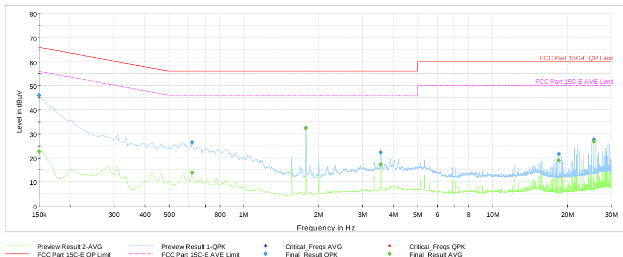
Plot 7-38. AC Line Conducted Plot with Bluetooth HDR (L1, 4Mbps ePA - Ch.38 with host PC + Magnetic Charger)
