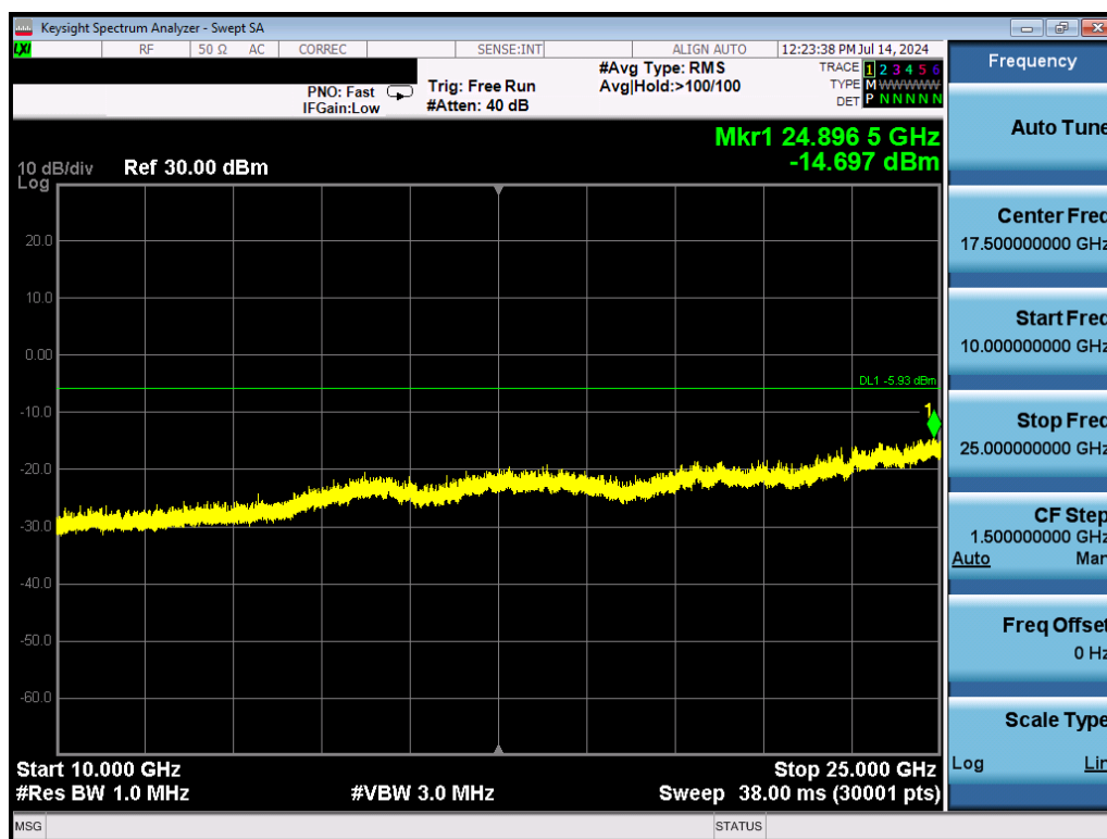
Plot 7-24. Conducted Spurious Plot (Bluetooth (HDR4), ePA – Ch. 1)
