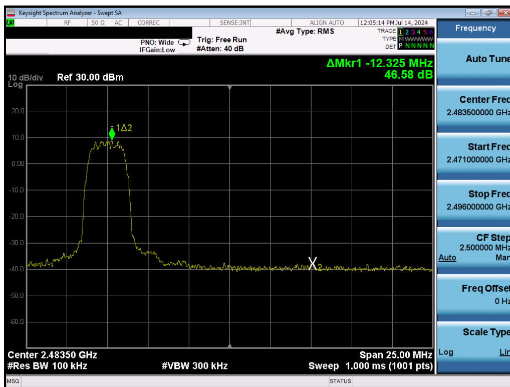
Plot 7-20. Band Edge Plot (Bluetooth (HDR4), ePA – Ch. 73)
