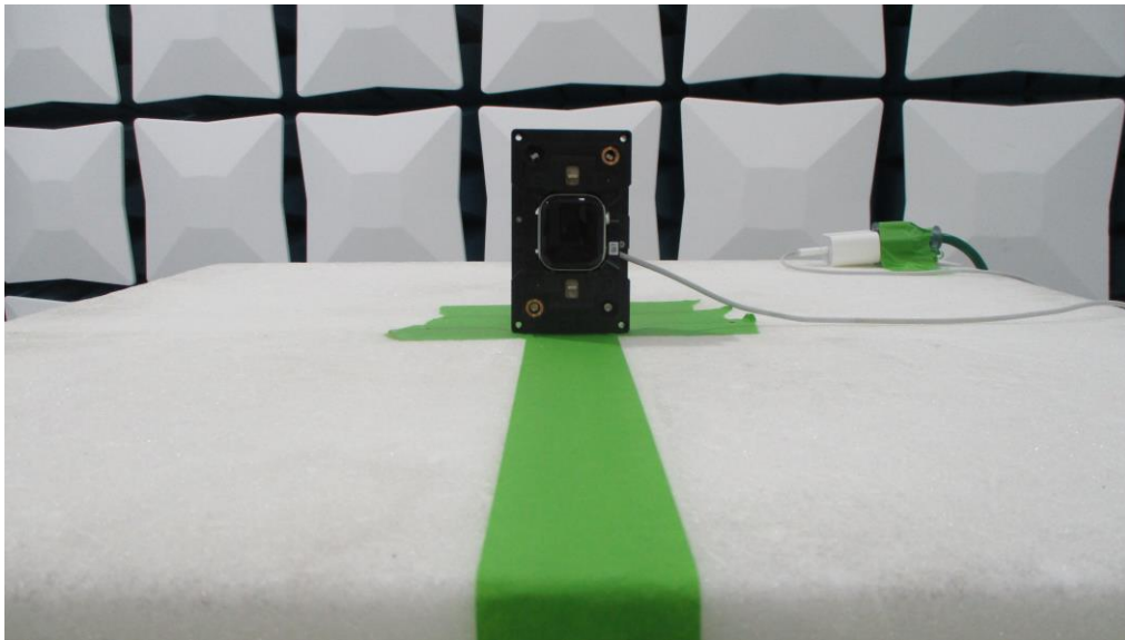
Figure 10: 1-18GHz Test Setup (Front View)
