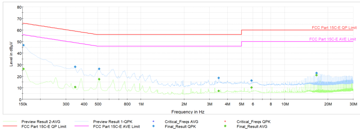
Plot 6-11. AC Line Conducted Plot (L1 - Mode 1, with Magnetic Charger & Laptop)
