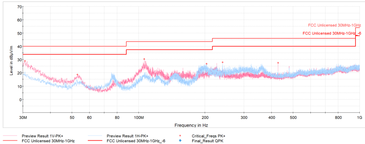
Plot 6-10. Radiated Spurious Emissions 30MHz – 1GHz (Mode 1, with Magnetic Charger & Laptop)
