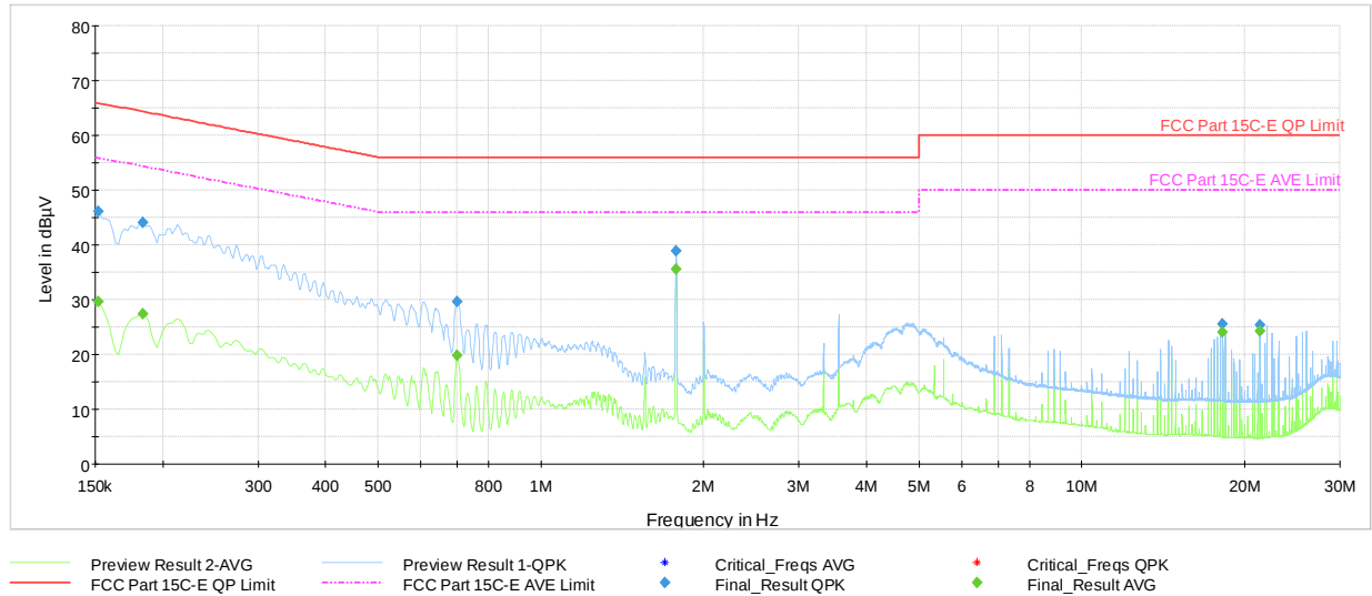
Plot 7-31. AC Line Conducted Plot (OQPSK – Ch. 24) (L1) with AC/DC Adapter & magnetic charger
