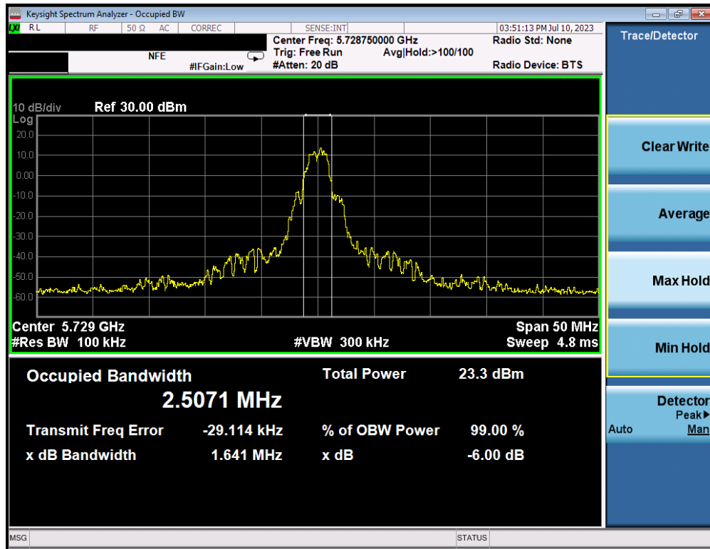
Plot 7-7. 6dB BW & 99% OBW (QPSK, 5728.75MHz, 1000kbps)
