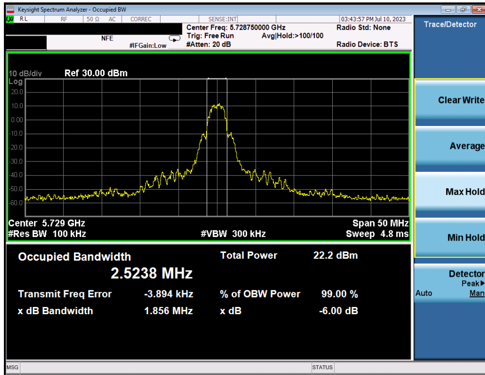
Plot 7-1. 6dB BW & 99% OBW (OQPSK, 5728.75MHz, 250kbps)
