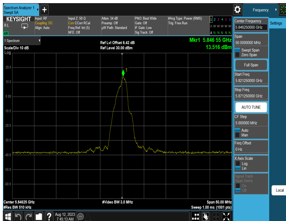
Plot 7-18. PSD (OQPSK, 5846.25MHz, 1000kbps)
