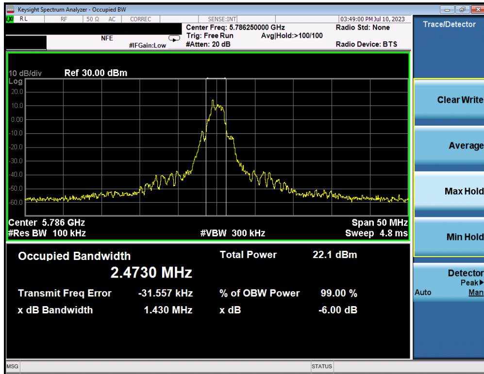
Plot 7-5. 6dB BW & 99% OBW (OQPSK, 5786.25MHz, 500kbps)
