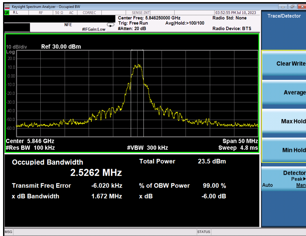
Plot 7-9. 6dB BW & 99% OBW (OQPSK, 5846.25MHz, 1000kbps)
