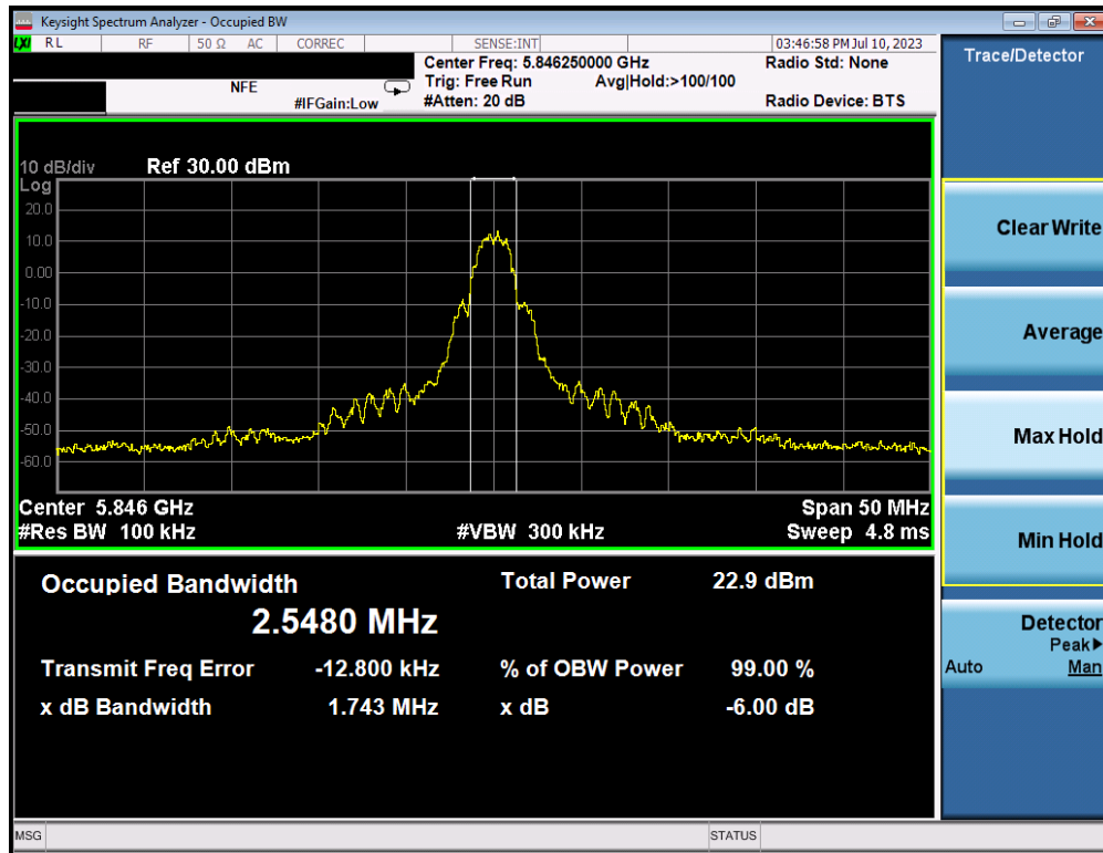
Plot 7-3. 6dB BW & 99% OBW (OQPSK, 5846.25MHz, 250kbps)
