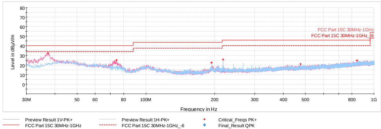
Plot 7-41. Radiated Spurious Emissions Below 1GHz (GFSK ePA – Ch.78, with AC/DC Adapter + Magnetic Charger)
