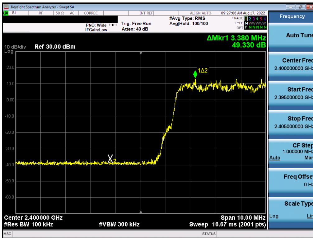
Plot 7-13. Band Edge Plot (Bluetooth with Hopping Enabled, 8DPSK, ePA)
