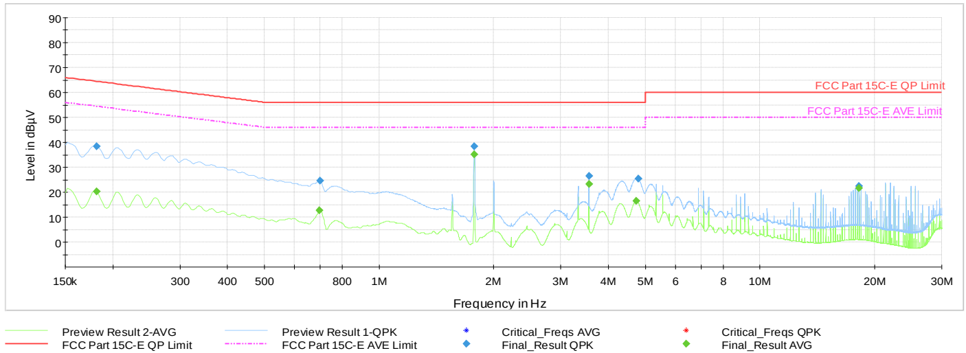
Plot 7-43. AC Line-Conducted Test Plot (N, GFSK ePA – Ch.78, with AC/DC Adapter + Magnetic Charger)
