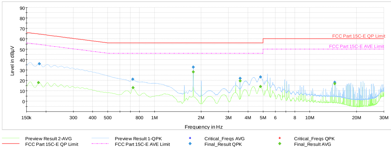
Plot 7-42. AC Line-Conducted Test Plot (L1, GFSK ePA – Ch.78, with AC/DC Adapter + Magnetic Charger)
