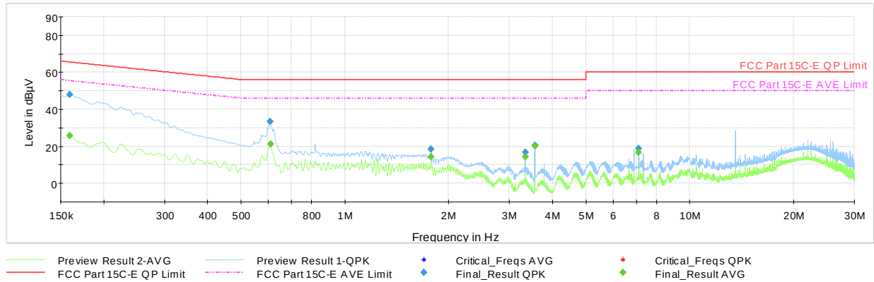
Plot 7-15. AC Line-Conducted Plot (N, Reader A 848kbps, with Laptop and Magnetic Charger)
