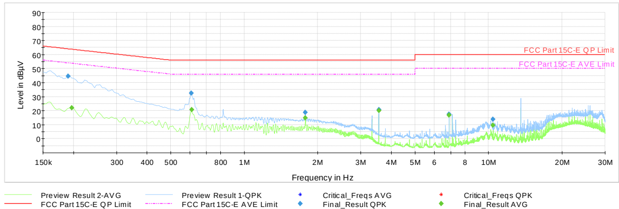
Plot 7-14. AC Line-Conducted Plot (L1, Reader A 848kbps, with Laptop and Magnetic Charger)
