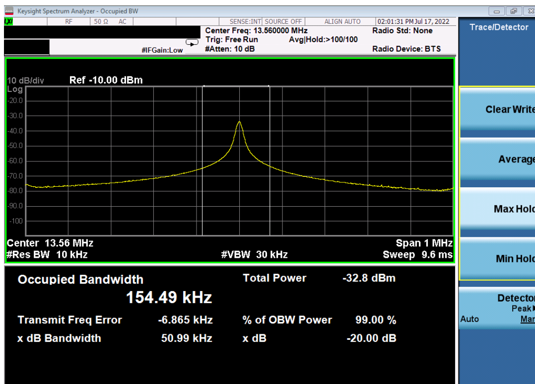
Plot 7-1. 20dB and 99% Bandwidth Plot (CE A 848kbps)
