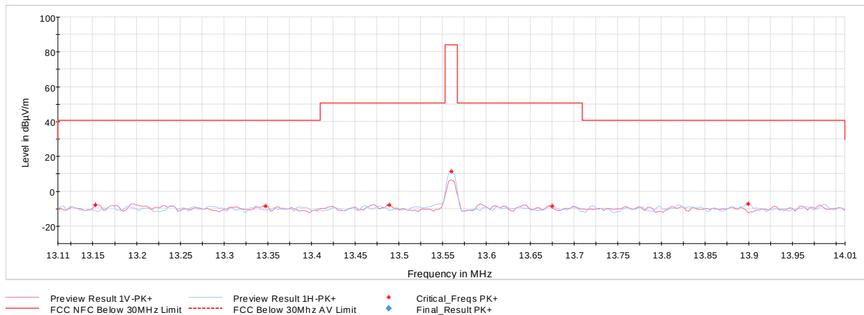
Plot 7-6. In Band Radiated Spurious Emissions (CE A 848kbps, with AC/DC Adapter and Magnetic Charger)
