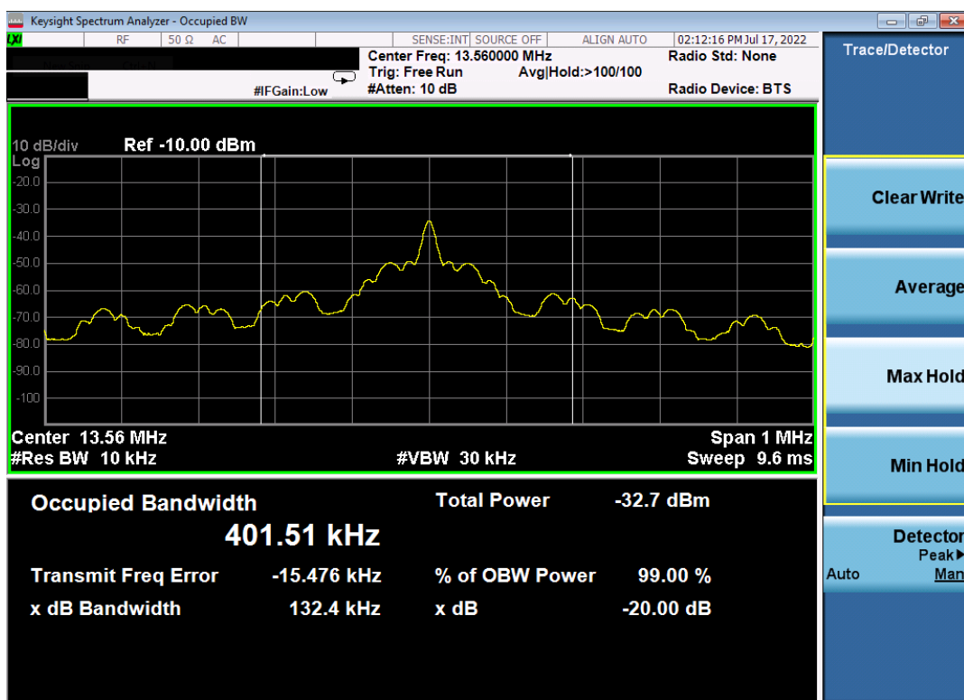
Plot 7-5. 20dB and 99% Bandwidth Plot (Reader 10% ASK 1 out of 256)
