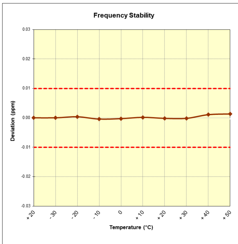
Figure 7-3. Frequency Stability Plot (CE A 848kbps)
