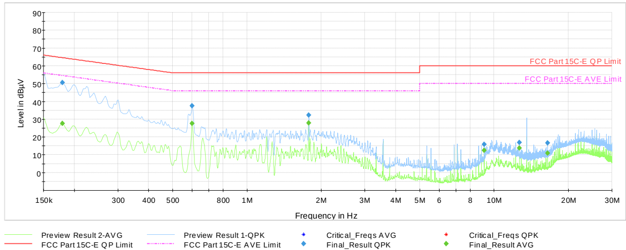
Plot 7-12. AC Line-Conducted Plot (L1, CE A 848kbps, with Laptop and Magnetic Charger)
