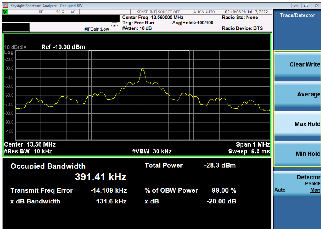
Plot 7-4. 20dB and 99% Bandwidth Plot (Reader 10% ASK 1 out of 4)
