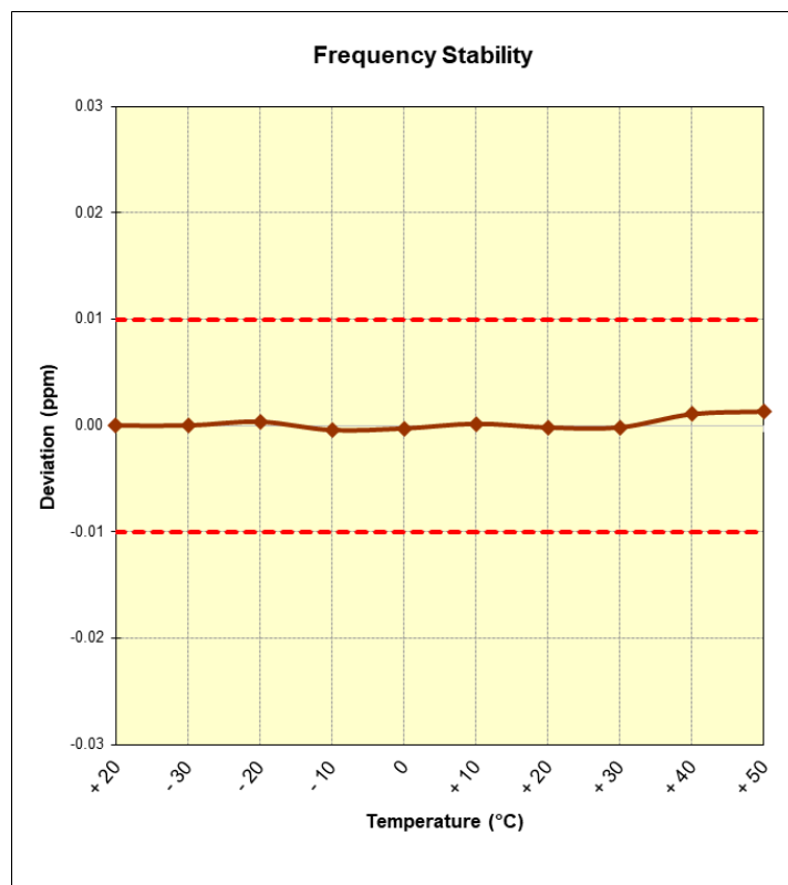
Figure 7-4. Frequency Stability Plot (Reader 10% ASK 1 out of 256)
