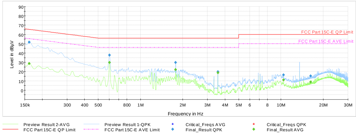
Plot 7-13. AC Line-Conducted Plot (N, CE A 848kbps, with Laptop and Magnetic Charger)
