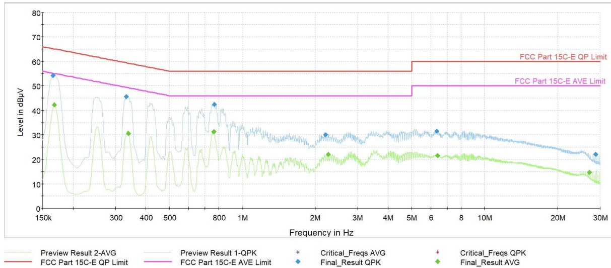
Plot 7-39. AC Line Conducted Plot with Bluetooth HDR (L1, 4Mbps ePA - Ch.38 with AC/DC Adapter + Magnetic Charger)
