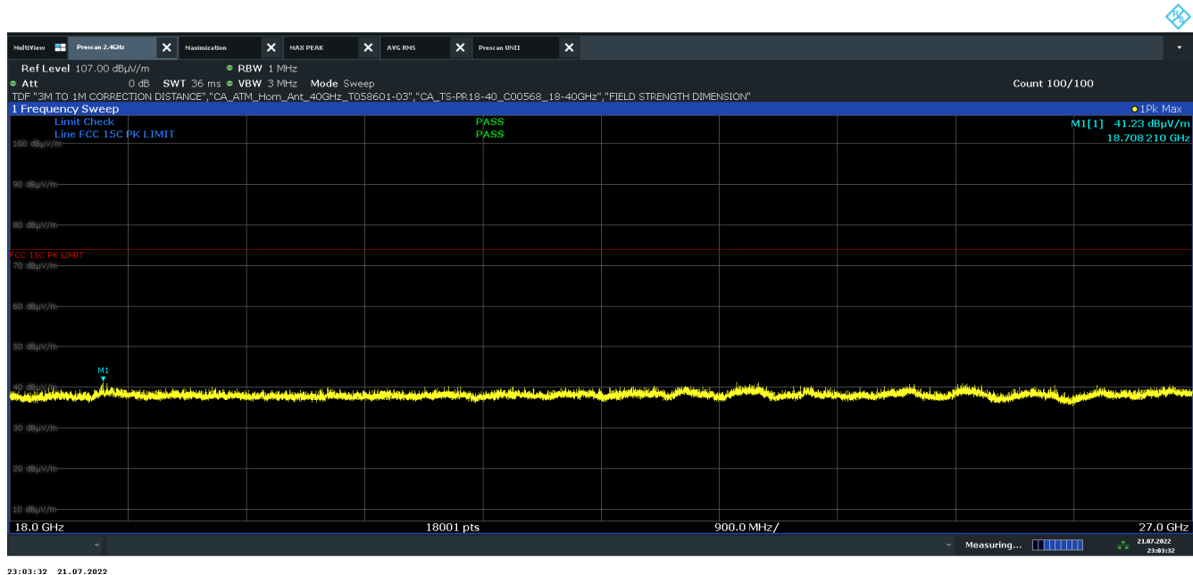
Plot 7-33. Radiated Spurious Plot Above 18GHz (4Mbps, HDR4, ePA – Ch.38 , Ant. Pol. V)
