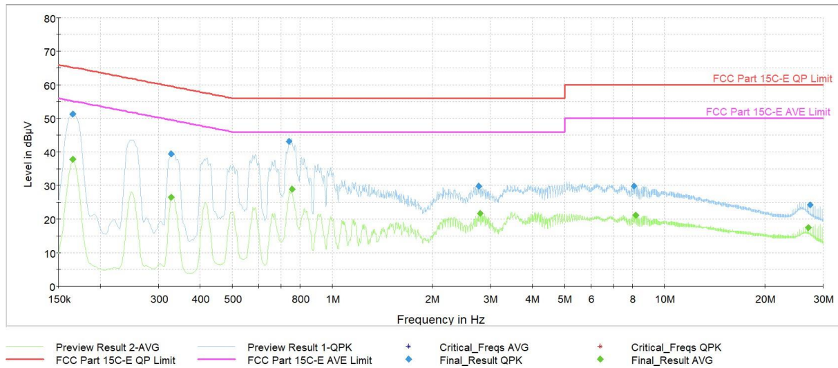
Plot 7-40. AC Line Conducted Plot with Bluetooth HDR (N, 4Mbps ePA - Ch.38 with AC/DC Adapter + Magnetic Charger)
