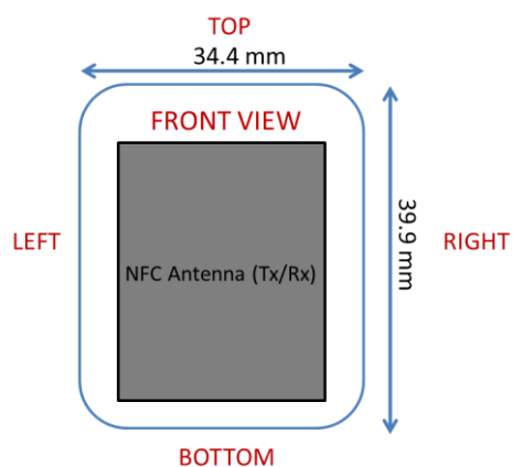
Figure B-2 NFC Antenna Location
