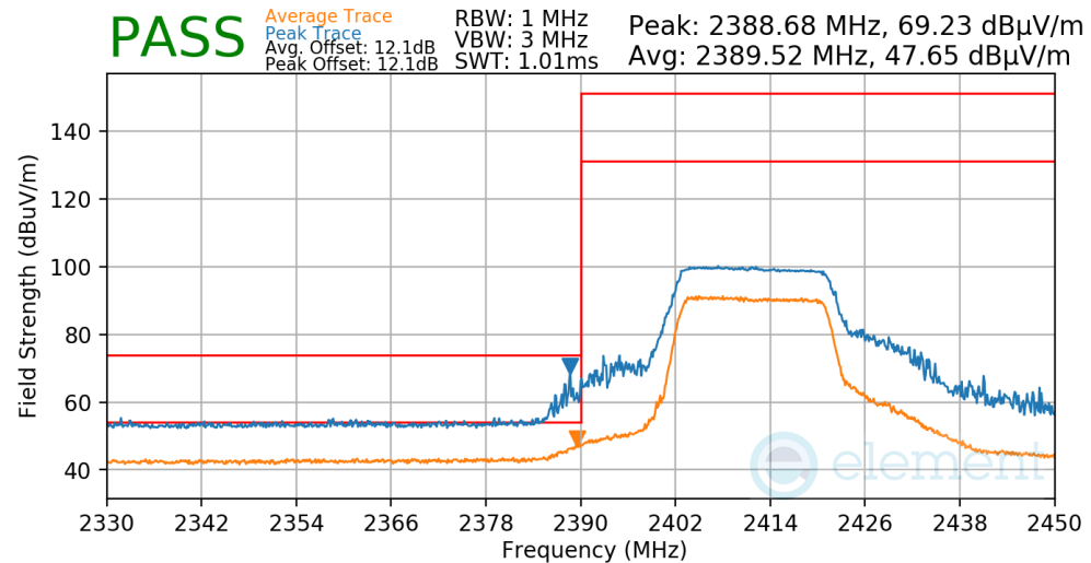
Plot 7-62. Radiated Restricted Lower Band Edge Measurement
