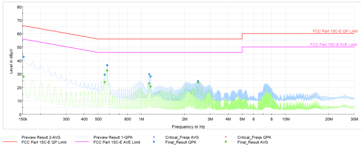
Plot 7-75. AC Line Conducted Plot 11b Ch.6 (N, with Laptop Charger + Magnetic Charger)
