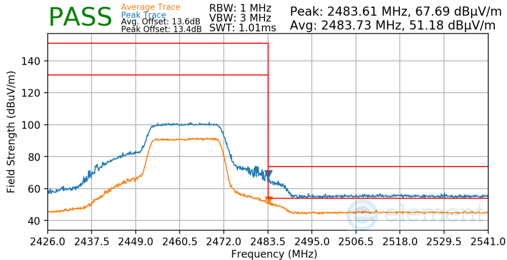
Plot 7-69. Radiated Restricted Upper Band Edge Measurement
