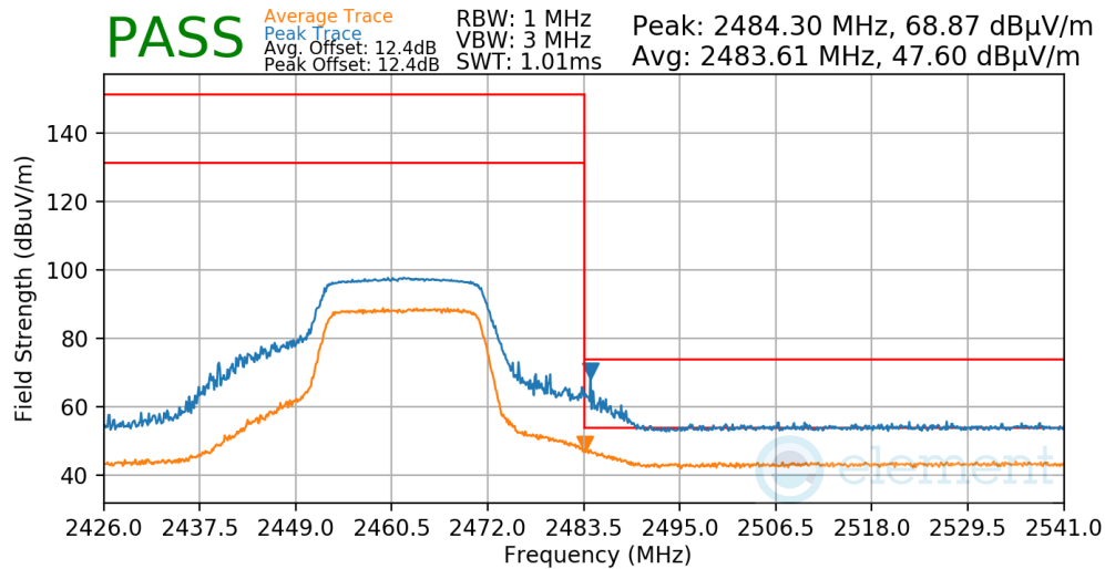
Plot 7-65. Radiated Restricted Upper Band Edge Measurement
