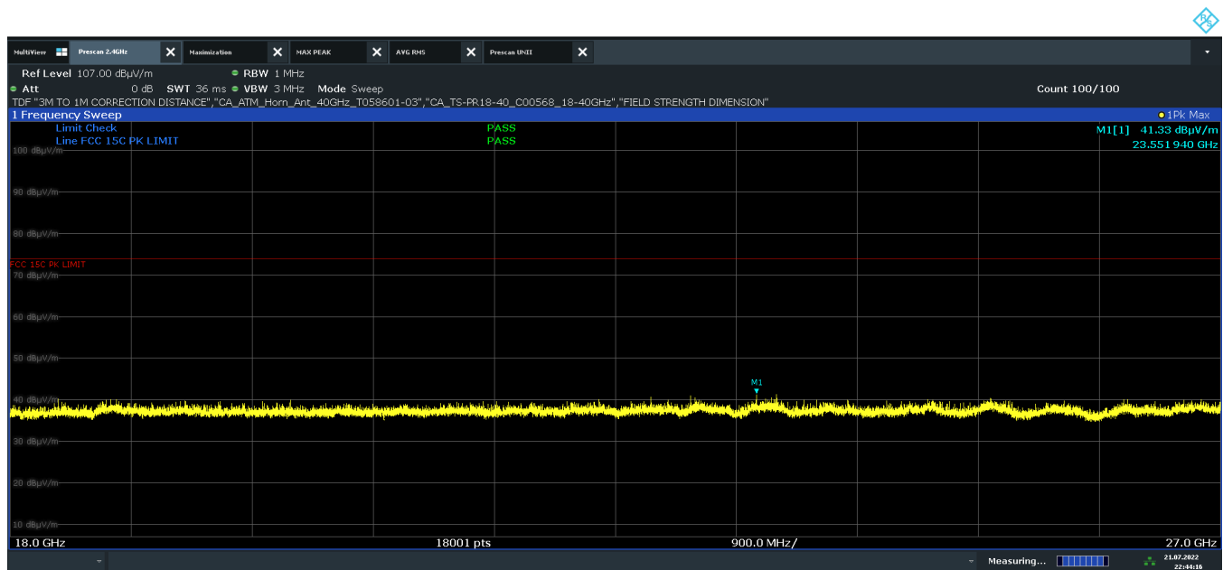
Plot 7-55. Radiated Spurious Emissions above 18GHz (802.11b – Ch.6, Pol V)
