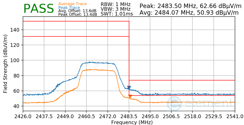
Plot 7-70. Radiated Restricted Upper Band Edge Measurement
