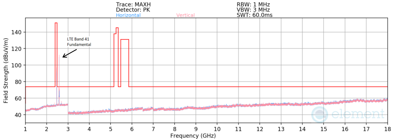
Plot 7-56. Radiated Spurious Emissions 1 - 18GHz – Simultaneous Transmission
