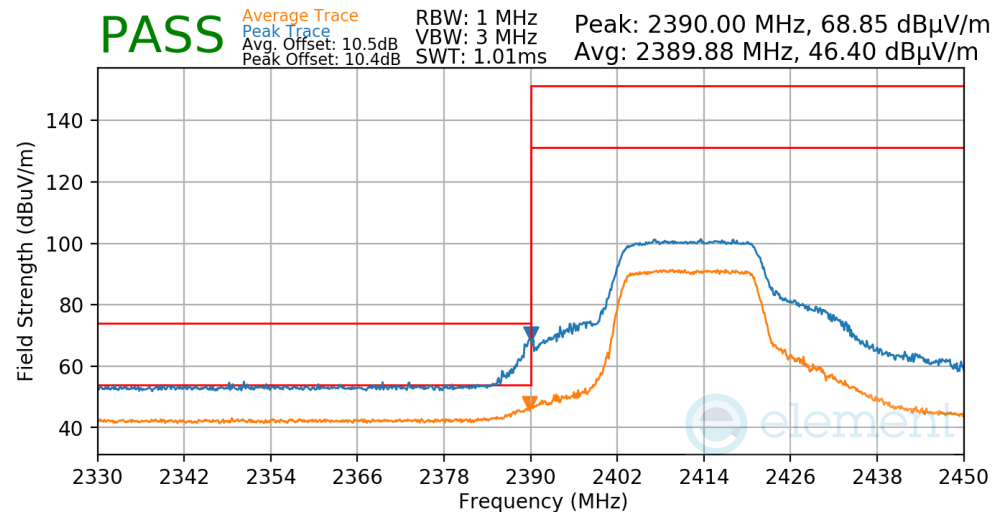
Plot 7-68. Radiated Restricted Lower Band Edge Measurement
