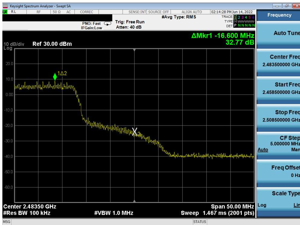
Plot 7-42. Band Edge Plot (802.11n (2.4GHz) – Ch. 11) – MCS7
