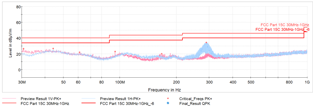
Plot 7-72. Radiated Spurious Emissions below 1GHz 11b Ch.6, with AC/DC Adapter and Magnetic Charger
