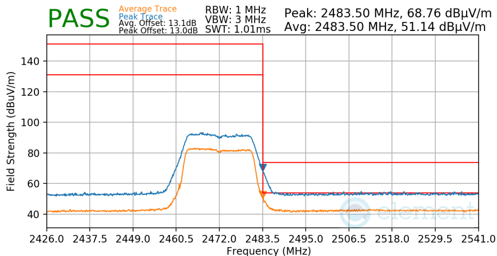
Plot 7-71. Radiated Restricted Upper Band Edge Measurement
