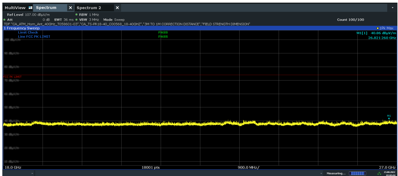
Plot 7-58. Radiated Spurious Emissions above 18GHz – Simultaneous Transmission (Pol. V)
