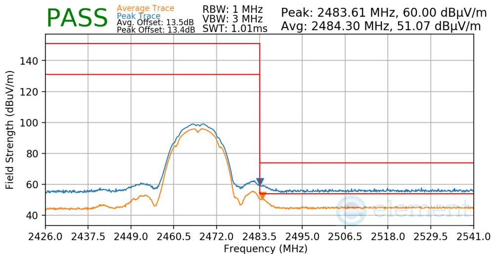
Plot 7-60. Radiated Restricted Upper Band Edge Measurement
