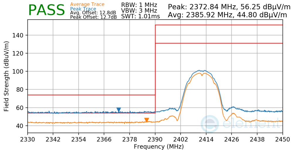
Plot 7-59. Radiated Restricted Lower Band Edge Measurement
