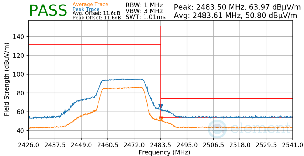
Plot 7-66. Radiated Restricted Upper Band Edge Measurement
