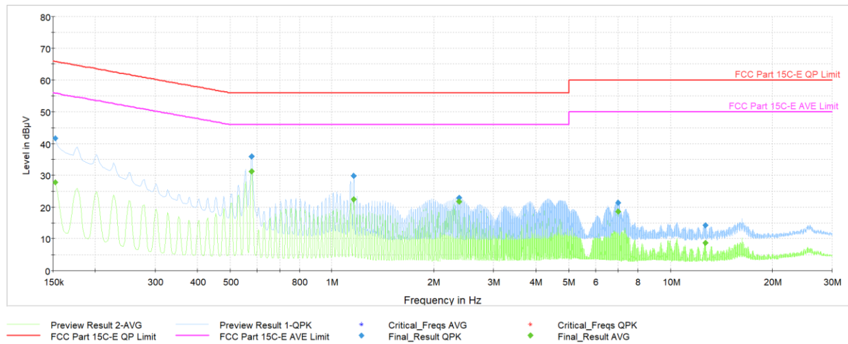
Plot 7-74. AC Line Conducted Plot 11b Ch.6 (L1, with Laptop Charger + Magnetic Charger)
