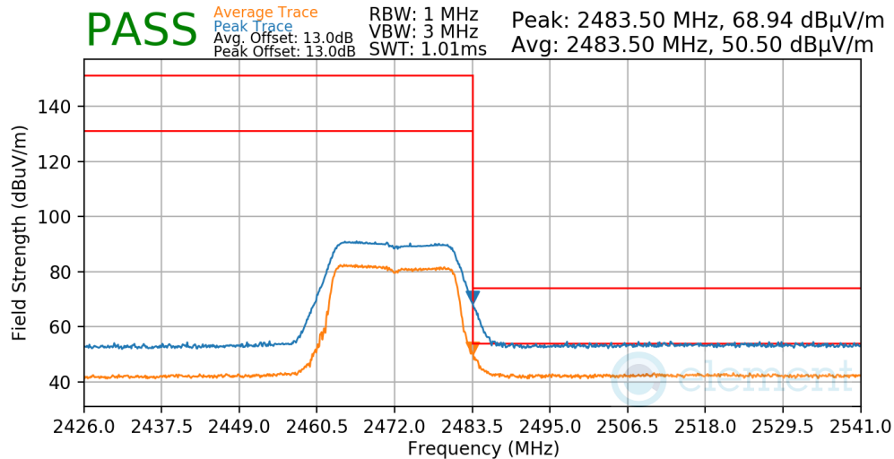
Plot 7-67. Radiated Restricted Upper Band Edge Measurement
