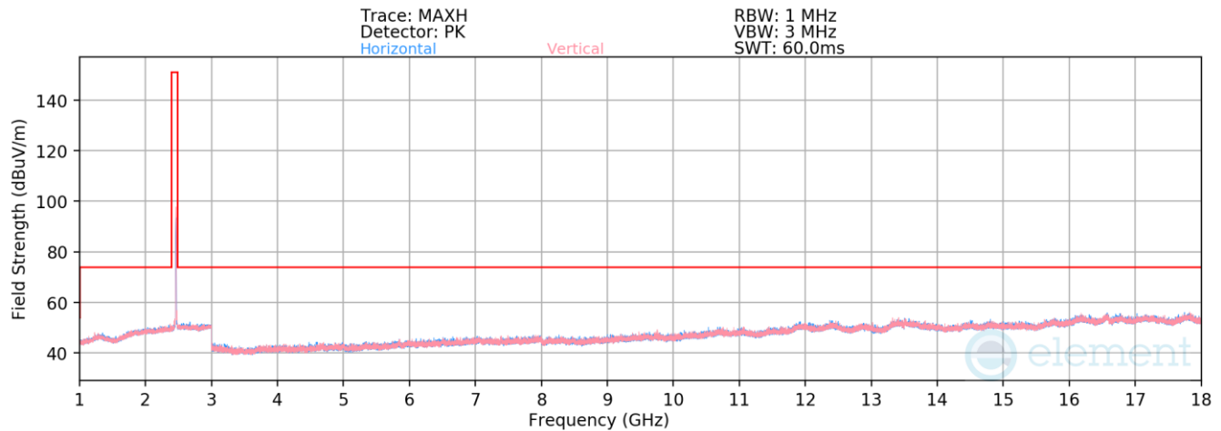
Plot 7-53. Radiated Spurious Emissions above 1GHz (802.11b – Ch. 11)
