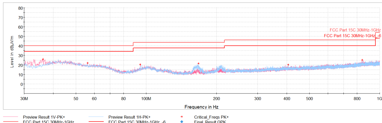
Plot 7-36. Co-Tx Radiated Spurious Emissions Below 1GHz with AC/DC Adapter
