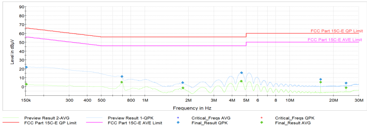
Plot 7-38. AC Line Conducted Plot with Bluetooth LE (N, 1Mbps – Ch.19, with AC/DC Adapter)
