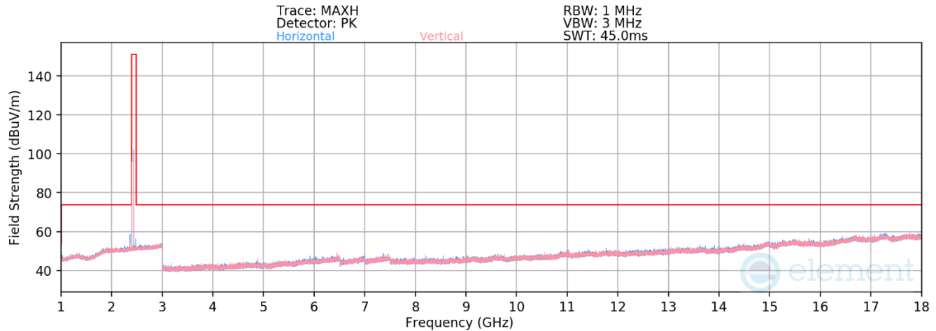
Plot 7-28. Radiated Spurious Emissions – Co-Tx 1-18GHz (1Mbps – Ch.19)
