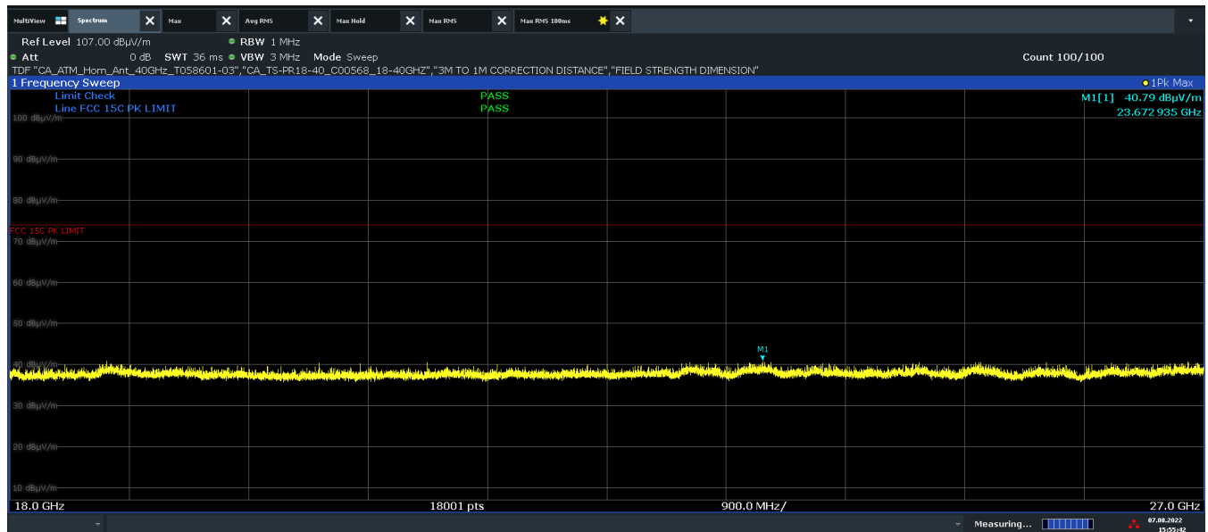
Plot 7-29. Radiated Spurious Emissions Above 18GHz – Co-Tx (1Mbps – Ch. 19 Pol. H)
