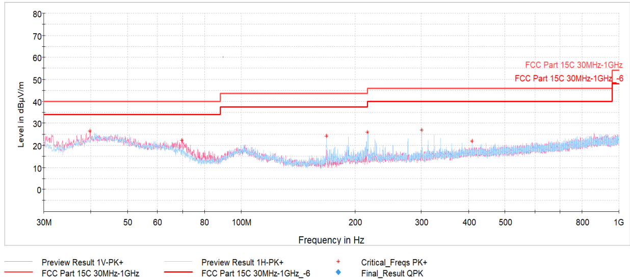
Plot 7-35. Radiated Spurious Emissions Below 1GHz (1Mbps – Ch.19, Pol. H & V, with AC/DC Adapter)
