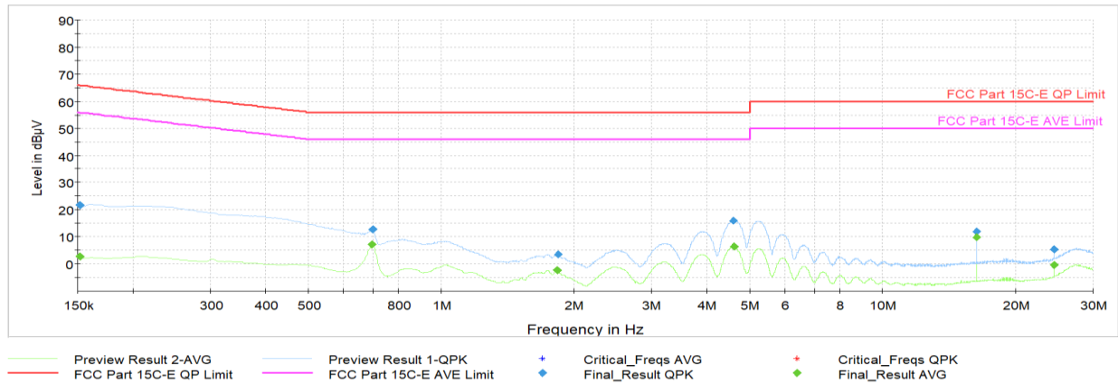
Plot 7-37. AC Line Conducted Plot with Bluetooth LE (L1, 1Mbps – Ch.19 with AC/DC Adapter)
