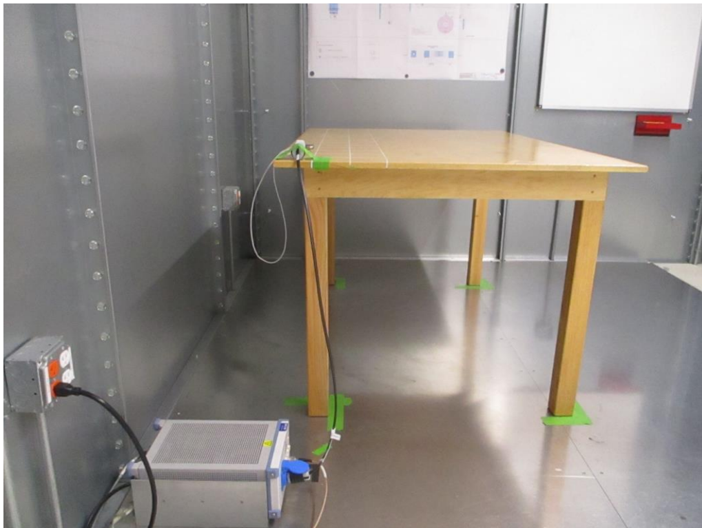
Figure 2: AC Line Conducted Emissions (Side View)
