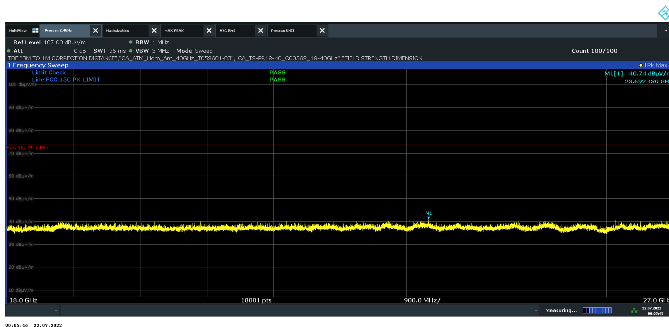
Plot 7-62. Radiated Spurious Plot Above 18GHz (802.11b – Ch. 6 Pol V)
