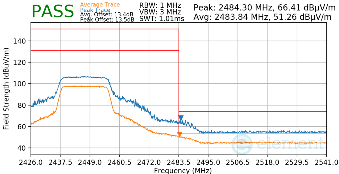
Plot 7-70. Radiated Restricted Upper Band Edge Measurement
