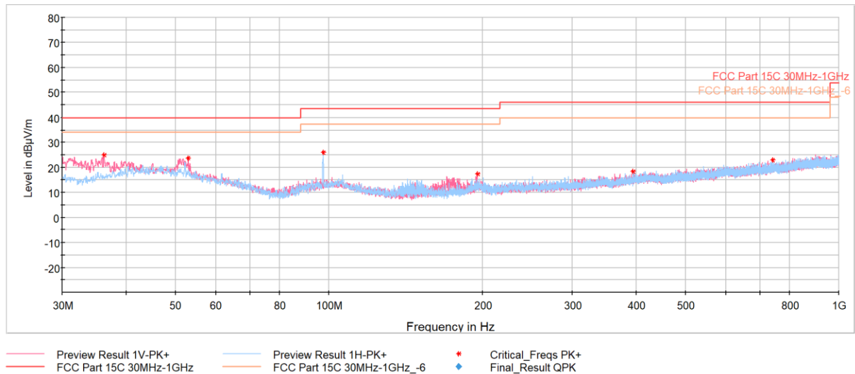
Plot 7-81. Radiated Spurious Emissions 30MHz - 1GHz 802.11b - Ch.6, with AC/DC Adapter and Magnetic Charger
