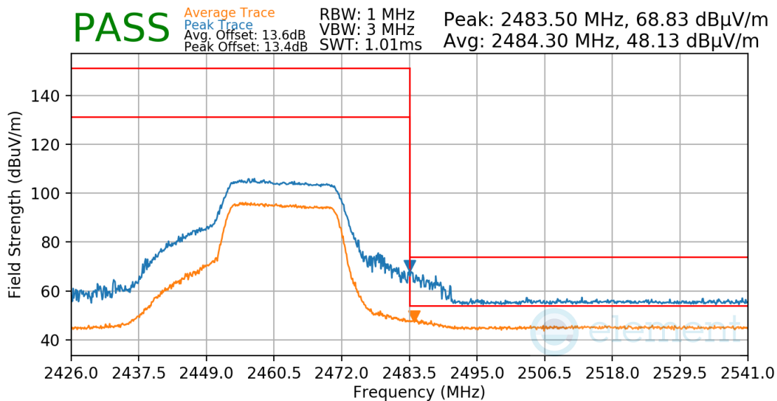
Plot 7-78. Radiated Restricted Upper Band Edge Measurement
