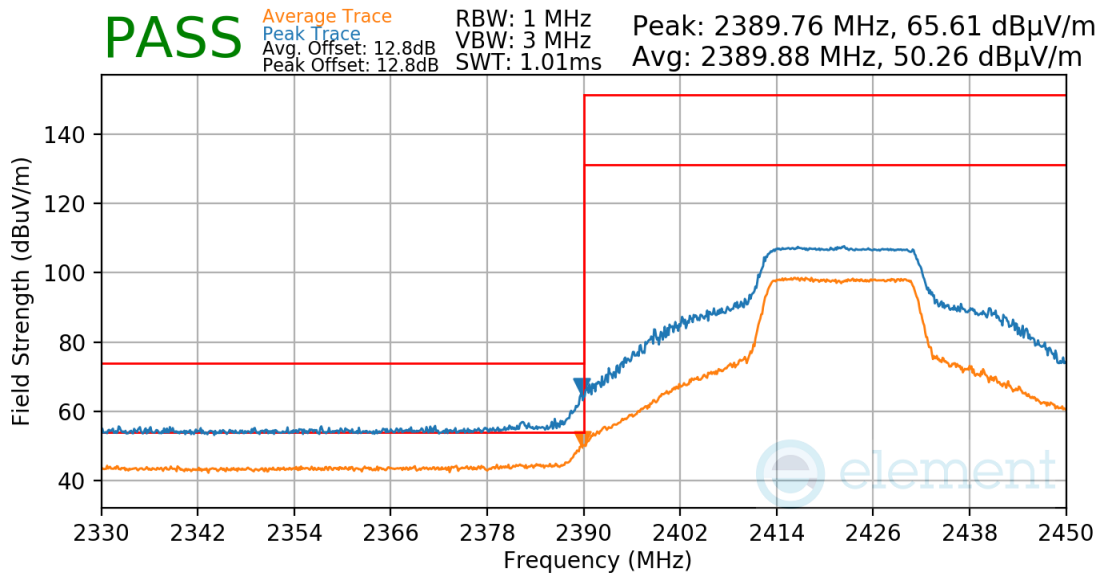
Plot 7-69. Radiated Restricted Lower Band Edge Measurement
