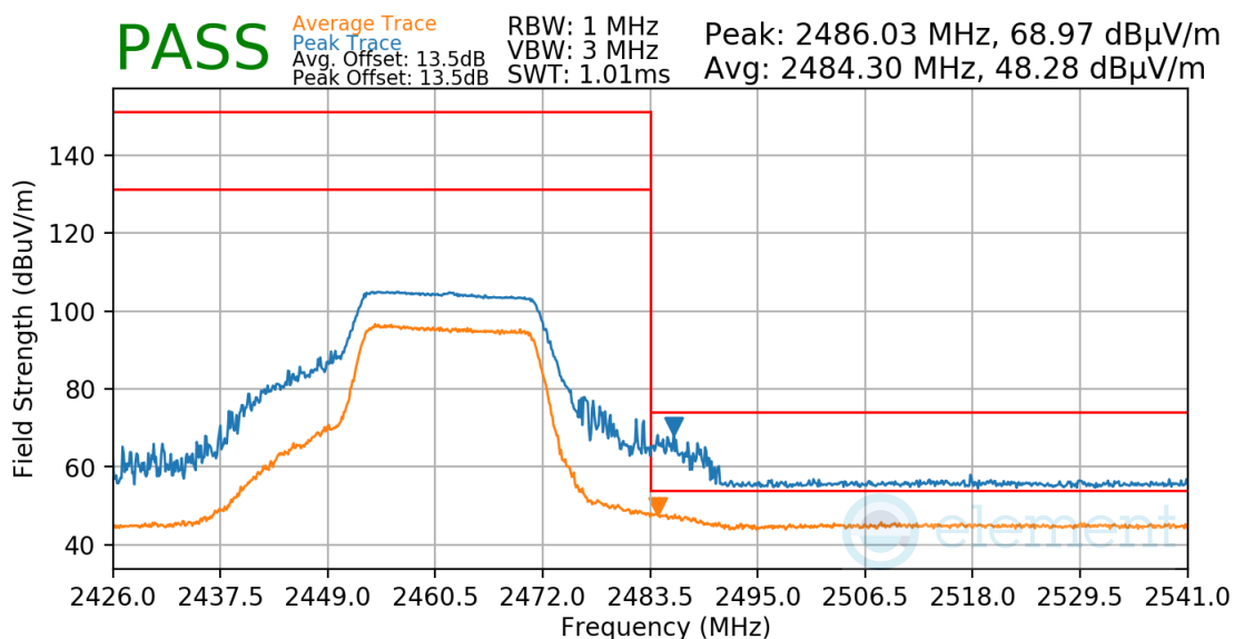
Plot 7-73. Radiated Restricted Upper Band Edge Measurement
