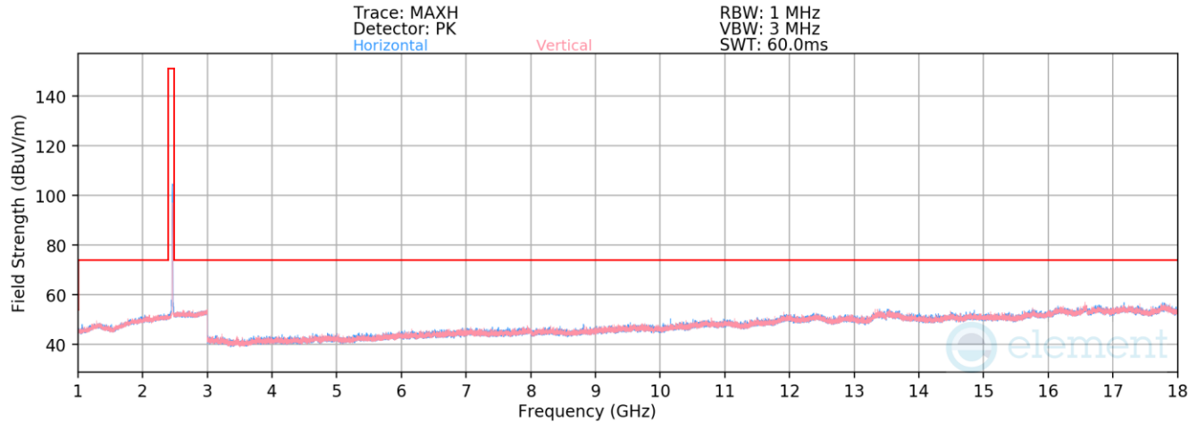
Plot 7-60. Radiated Spurious Emissions above 1GHz (802.11b – Ch. 11)
