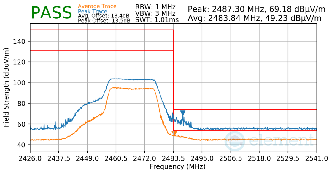
Plot 7-74. Radiated Restricted Upper Band Edge Measurement
