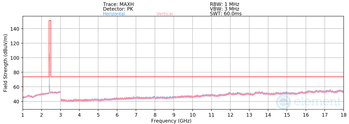
Plot 7-58. Radiated Spurious Emissions above 1GHz (802.11b – Ch. 1)
