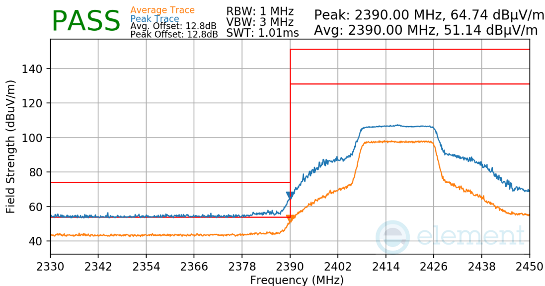
Plot 7-68. Radiated Restricted Lower Band Edge Measurement
