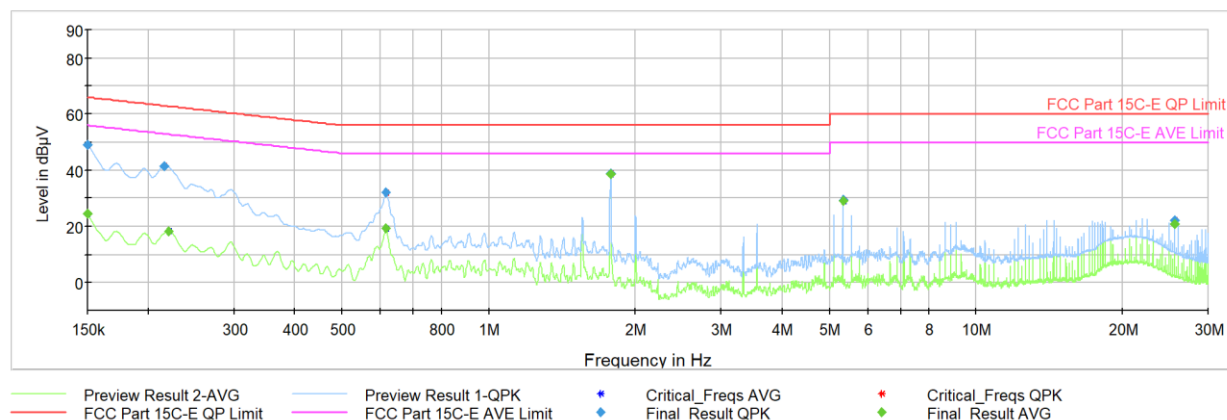
Plot 7-83. AC Line Conducted Plot 802.11b - Ch.6 (L1, with host PC and Magnetic charger)
