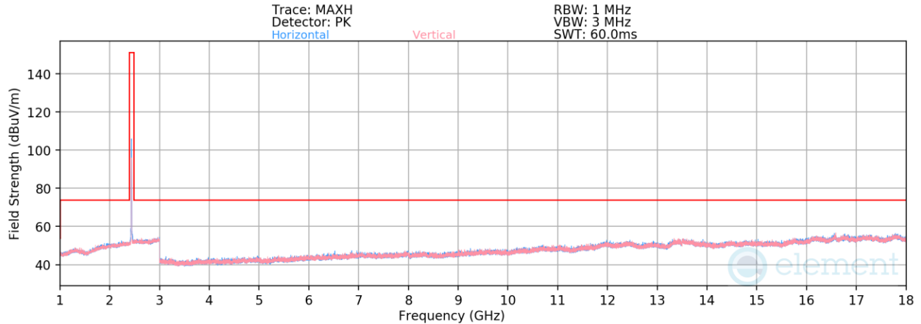
Plot 7-59. Radiated Spurious Emissions above 1GHz (802.11b – Ch. 6)
