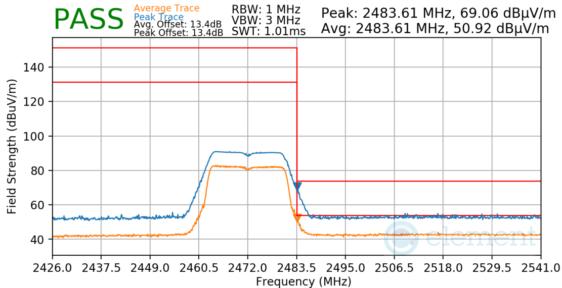
Plot 7-75. Radiated Restricted Upper Band Edge Measurement
