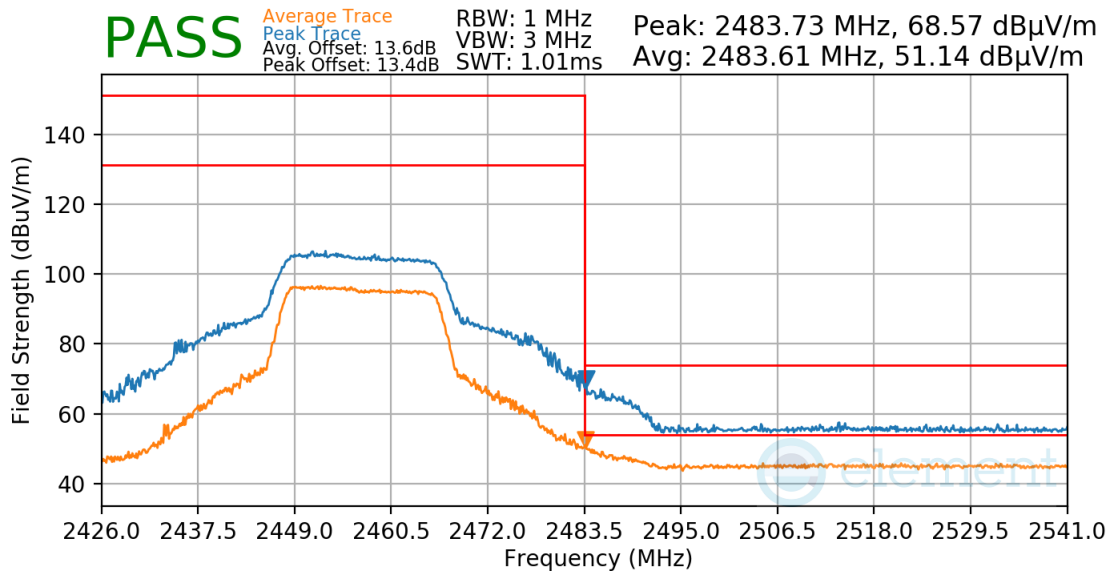
Plot 7-77. Radiated Restricted Upper Band Edge Measurement
