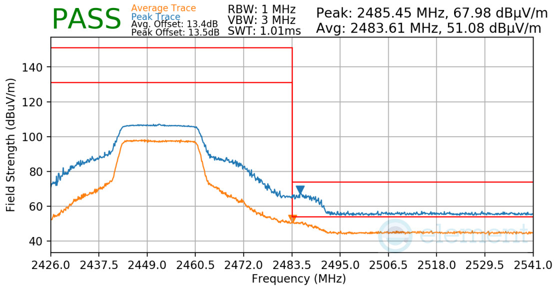
Plot 7-71. Radiated Restricted Upper Band Edge Measurement
