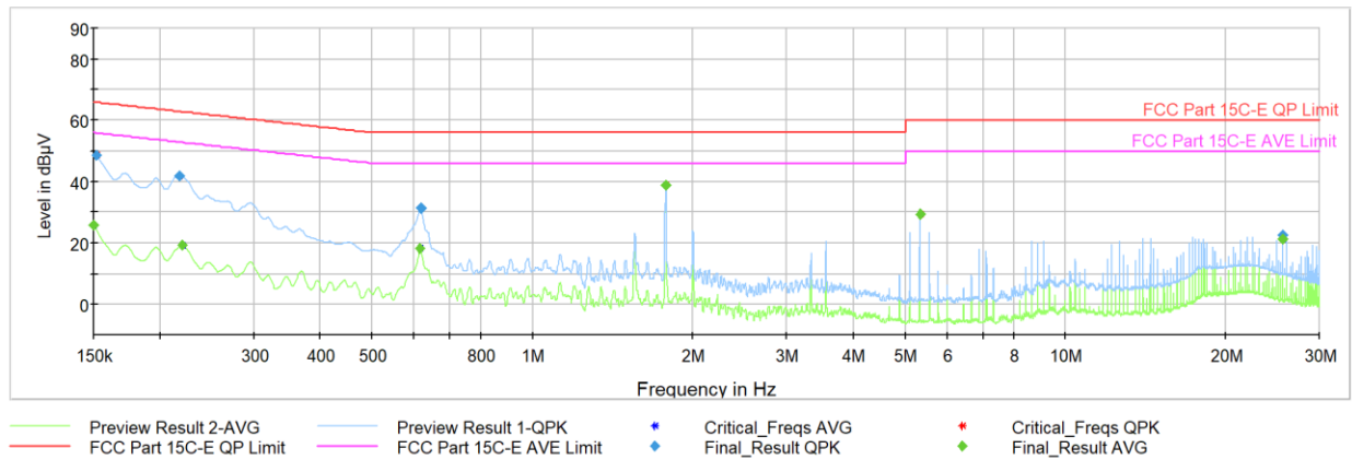
Plot 7-82. AC Line Conducted Plot 802.11b - Ch.6 (L1, with host PC and Magnetic charger)
