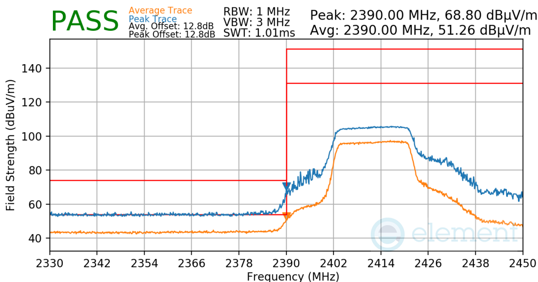
Plot 7-67. Radiated Restricted Lower Band Edge Measurement
