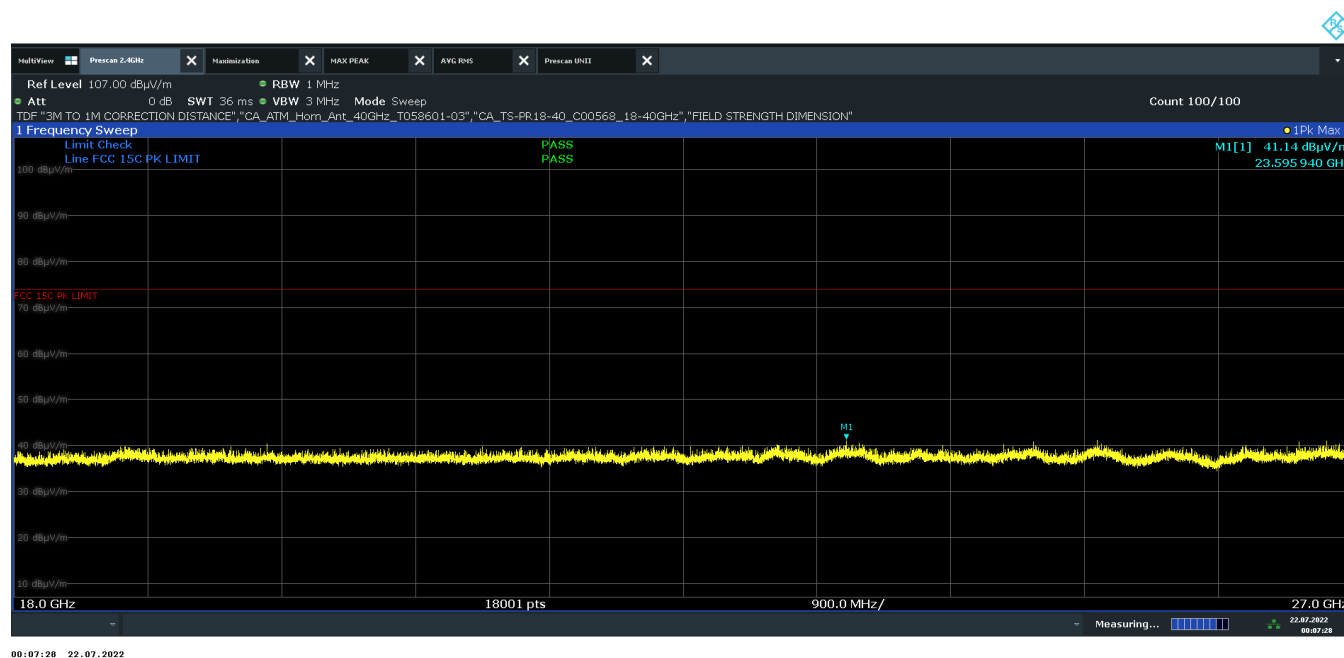
Plot 7-61. Radiated Spurious Plot Above 18GHz (802.11b – Ch. 6 Pol H)
