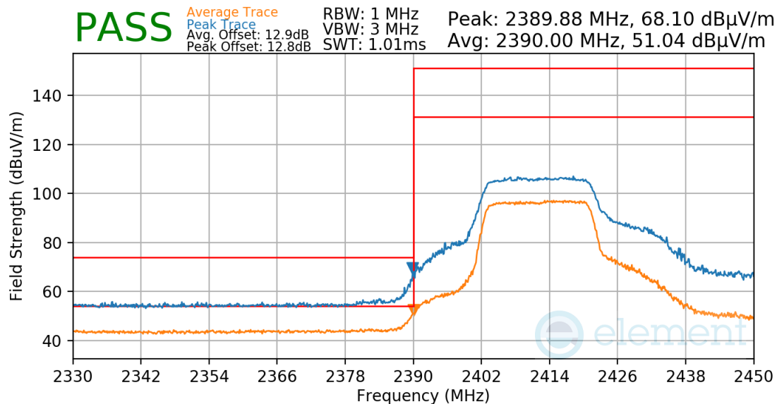
Plot 7-76. Radiated Restricted Lower Band Edge Measurement
