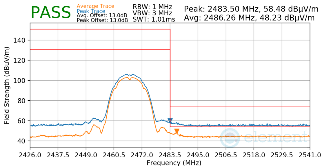
Plot 7-65. Radiated Restricted Upper Band Edge Measurement
