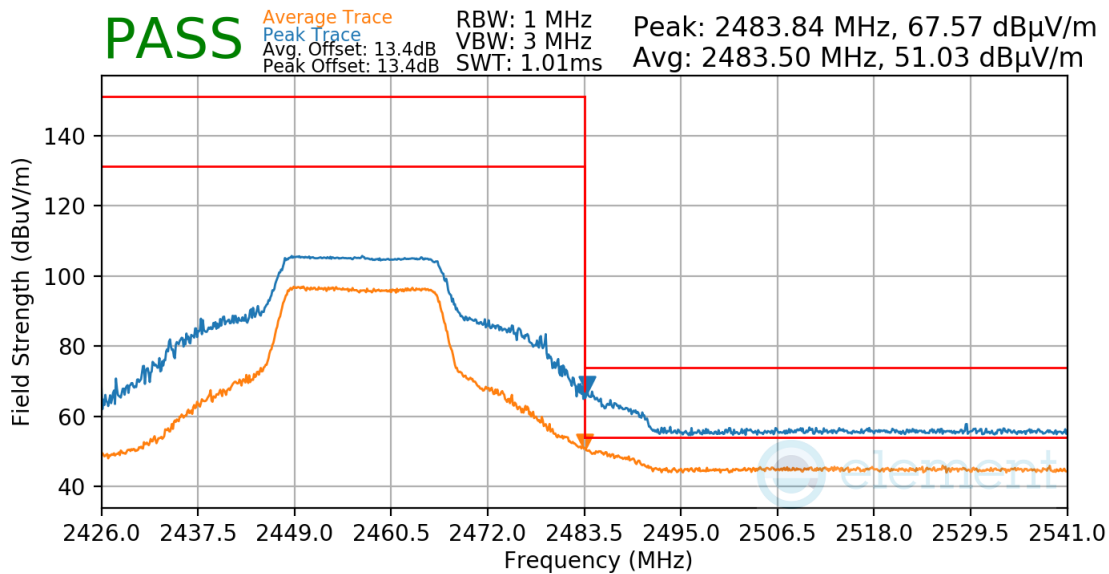
Plot 7-72. Radiated Restricted Upper Band Edge Measurement
