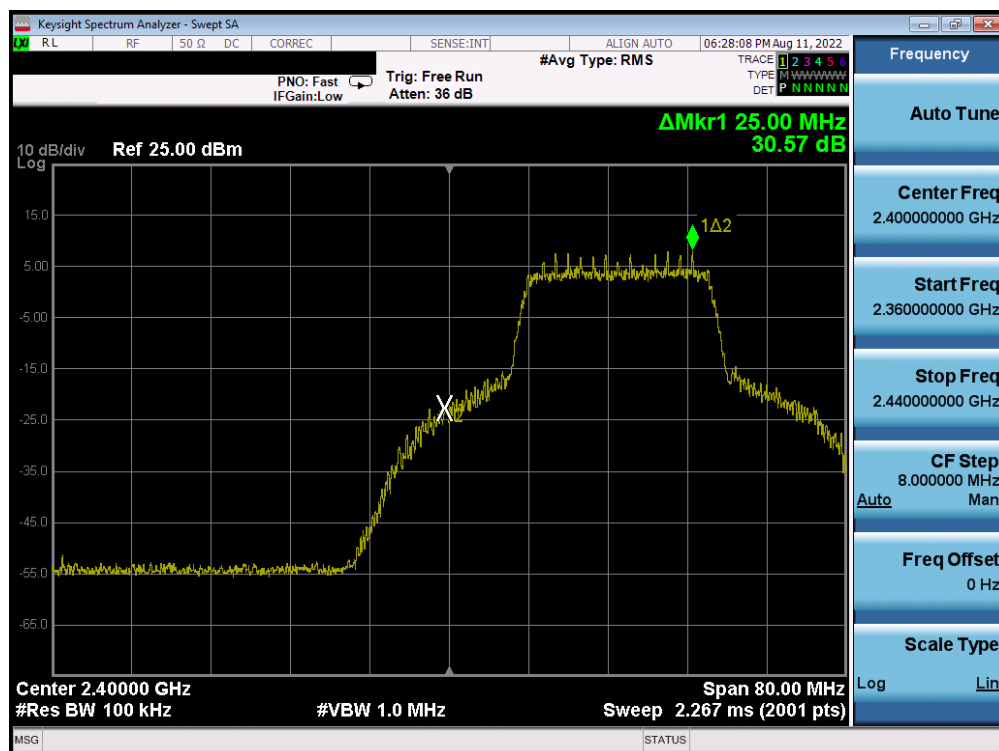
Plot 7-40. Band Edge Plot (802.11n MCS0 – Ch. 3)
