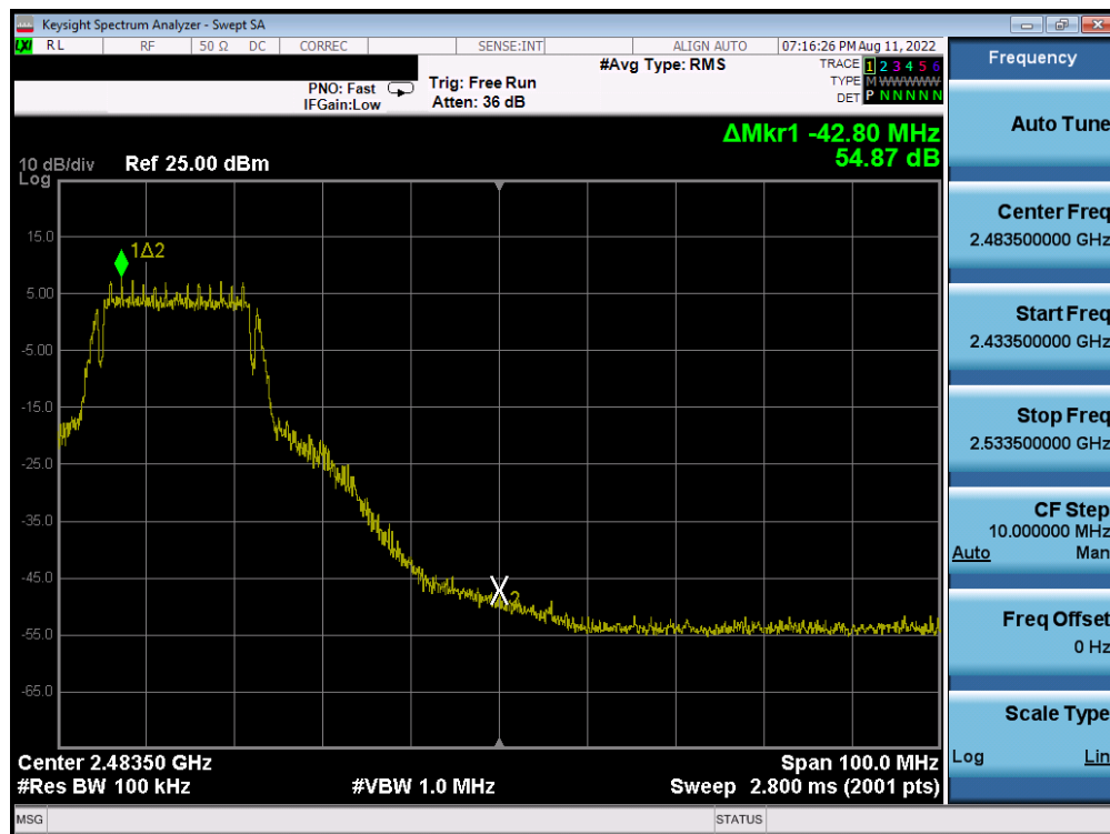
Plot 7-32. Band Edge Plot (802.11g– Ch. 8)
