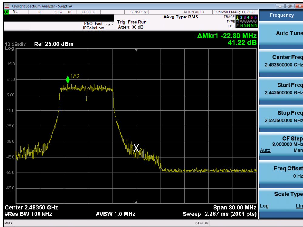
Plot 7-50. Band Edge Plot (802.11n MCS7 – Ch. 12)
