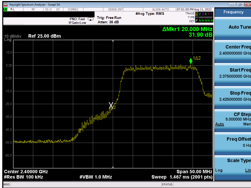
Plot 7-47. Band Edge Plot (802.11n MCS7 – Ch. 1)
