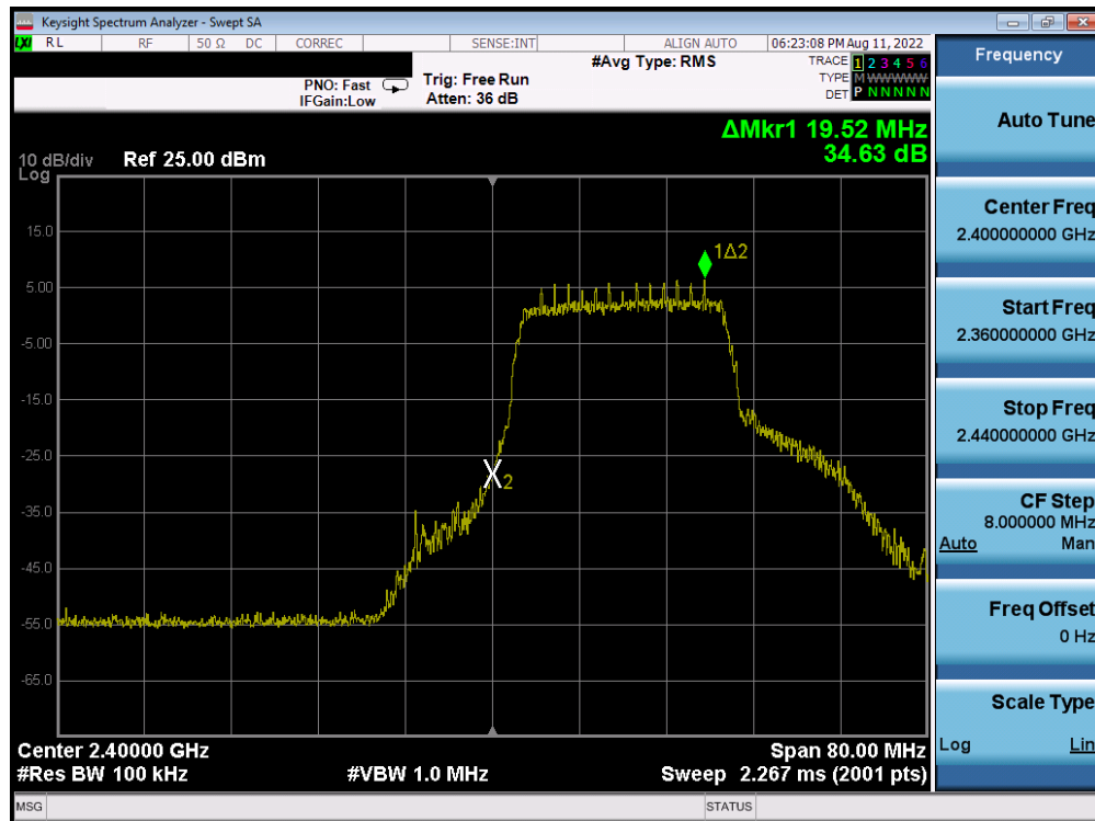
Plot 7-38. Band Edge Plot (802.11n MCS0 – Ch. 1)
