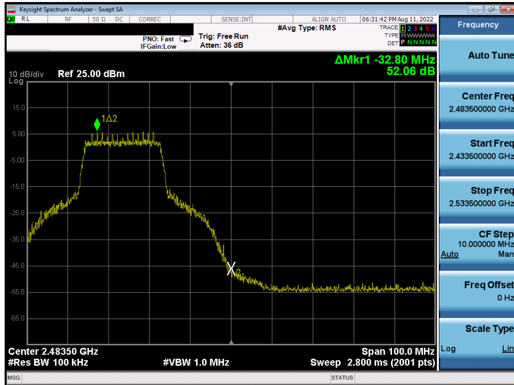
Plot 7-43. Band Edge Plot (802.11n MCS0 – Ch. 10)
