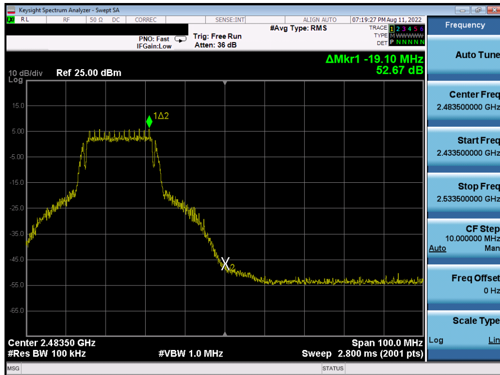
Plot 7-34. Band Edge Plot Antenna 1 (802.11g – Ch. 10)
