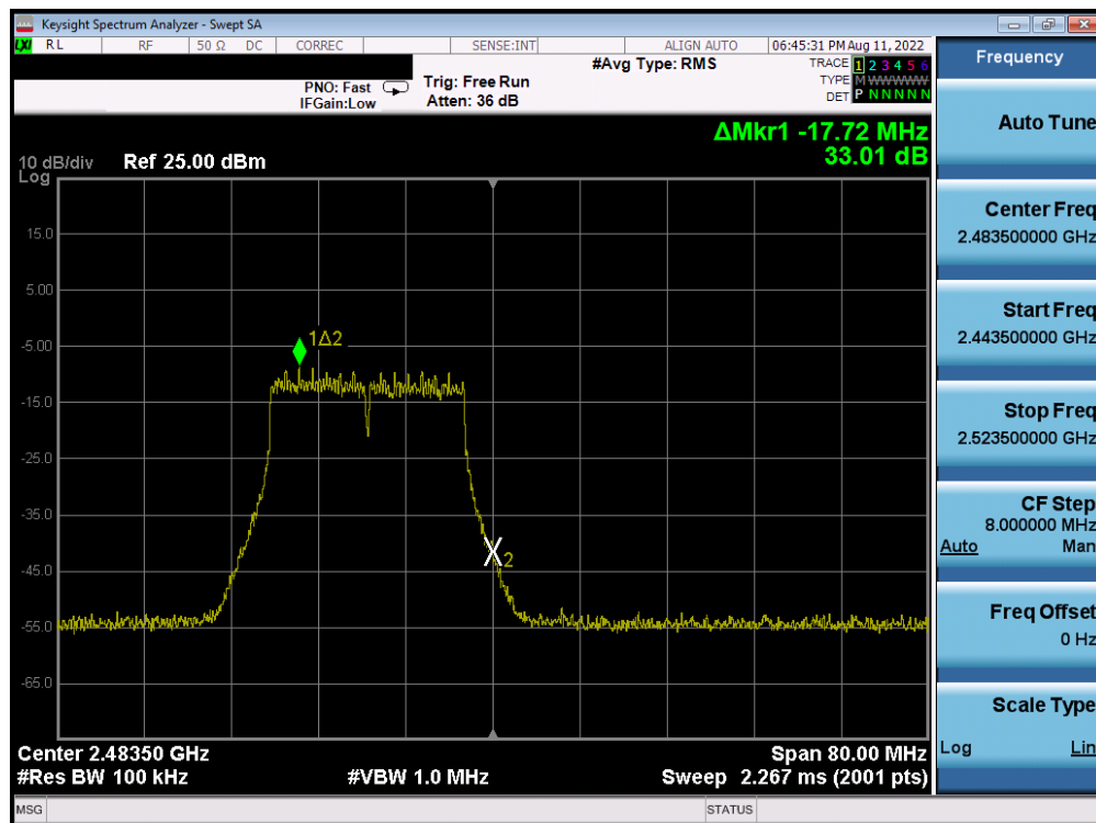
Plot 7-51. Band Edge Plot (802.11n MCS7 – Ch. 13)
