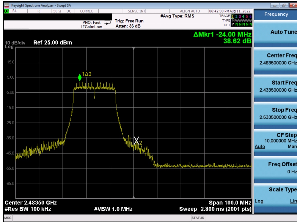
Plot 7-45. Band Edge Plot (802.11n MCS0 – Ch. 12)
