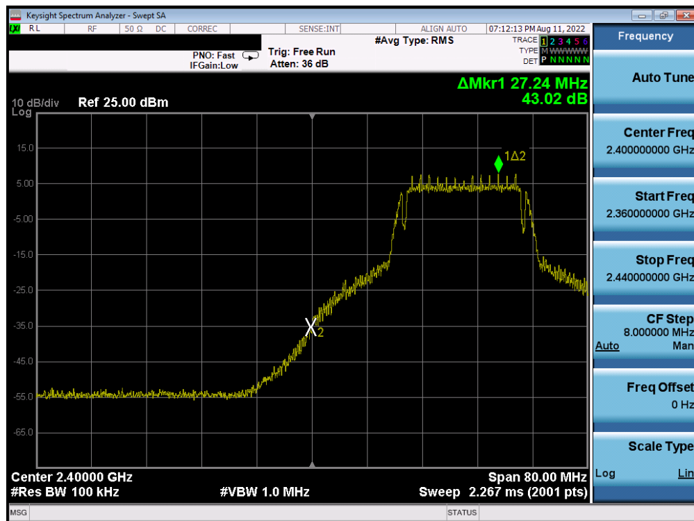
Plot 7-31. Band Edge Plot (802.11g– Ch. 3)
