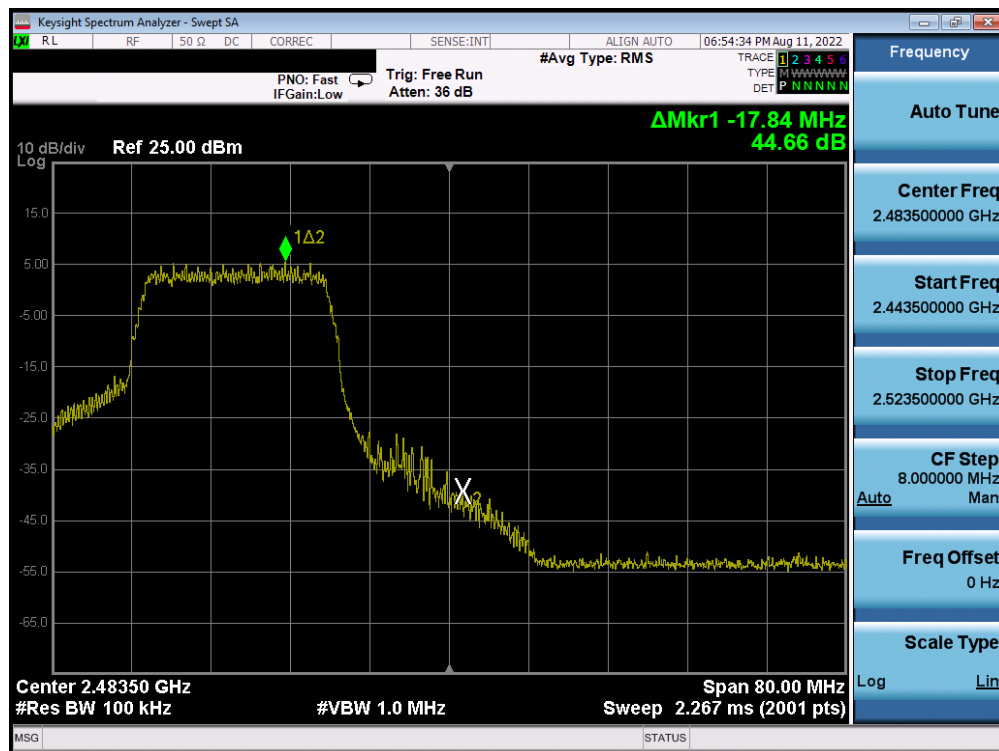
Plot 7-48. Band Edge Plot (802.11n MCS7 – Ch. 10)
