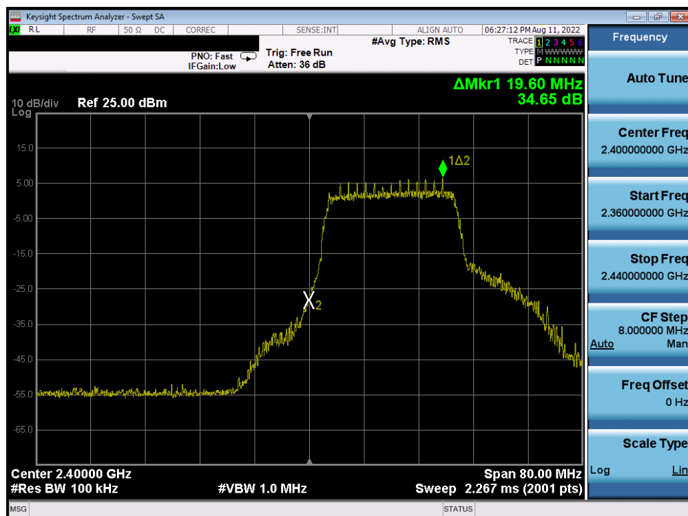
Plot 7-39. Band Edge Plot (802.11n MCS0 – Ch. 2)
