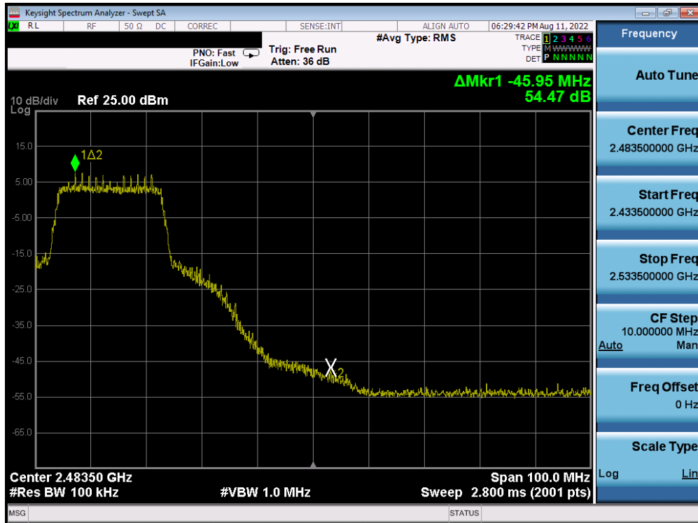
Plot 7-41. Band Edge Plot (802.11n MCS0 – Ch. 8)
