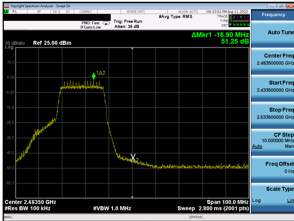
Plot 7-44. Band Edge Plot (802.11n MCS0 – Ch. 11)
