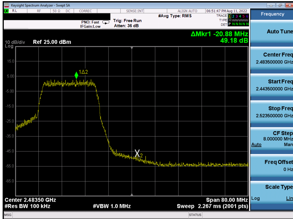
Plot 7-49. Band Edge Plot (802.11n MCS7 – Ch. 11)
