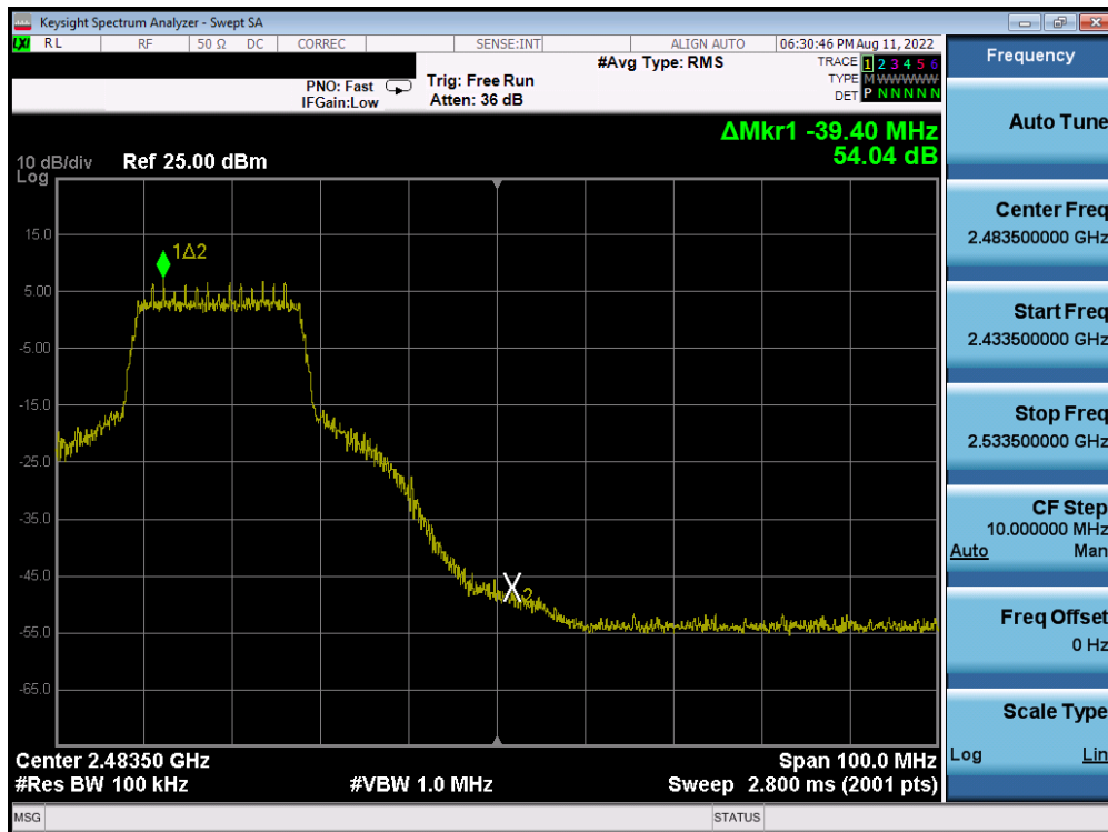
Plot 7-42. Band Edge Plot (802.11n MCS0 – Ch. 9)
