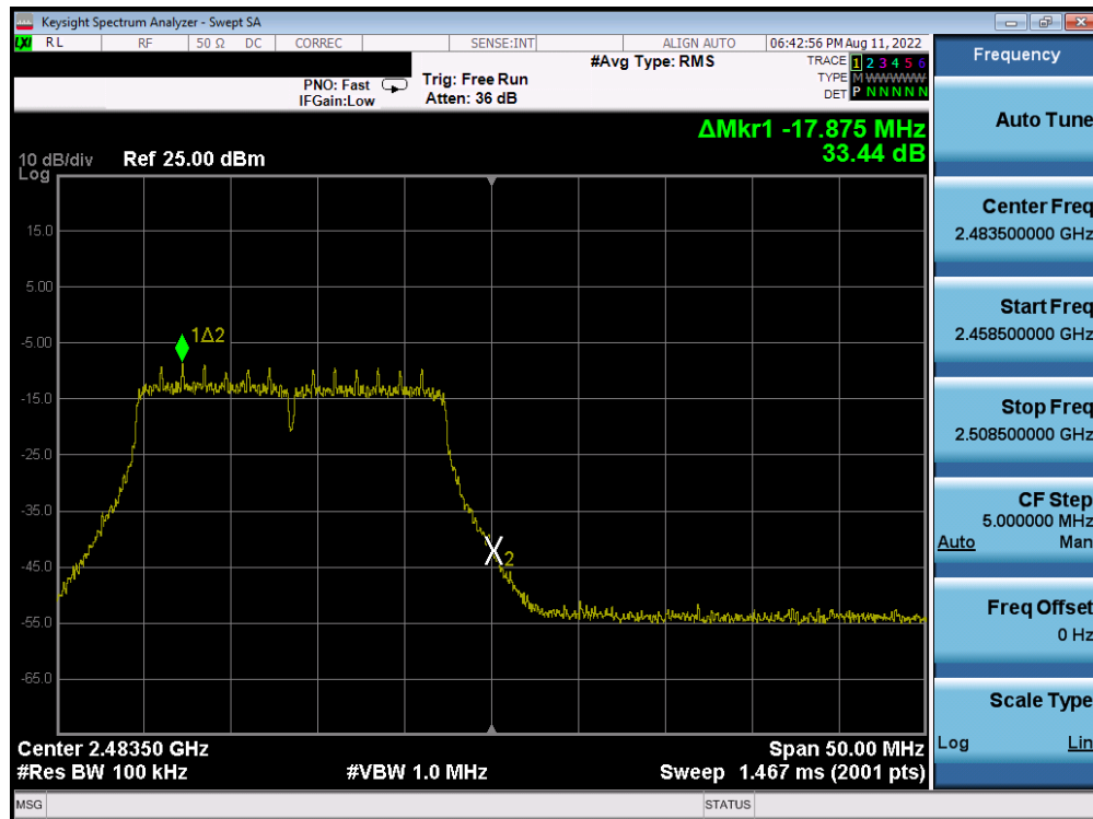
Plot 7-46. Band Edge Plot (802.11n MCS0 – Ch. 13)
