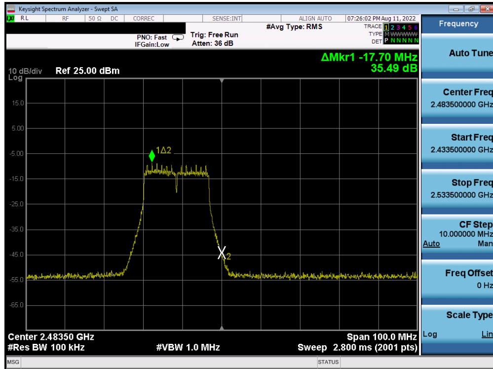
Plot 7-37. Band Edge Plot Antenna 1 (802.11g – Ch. 13)
