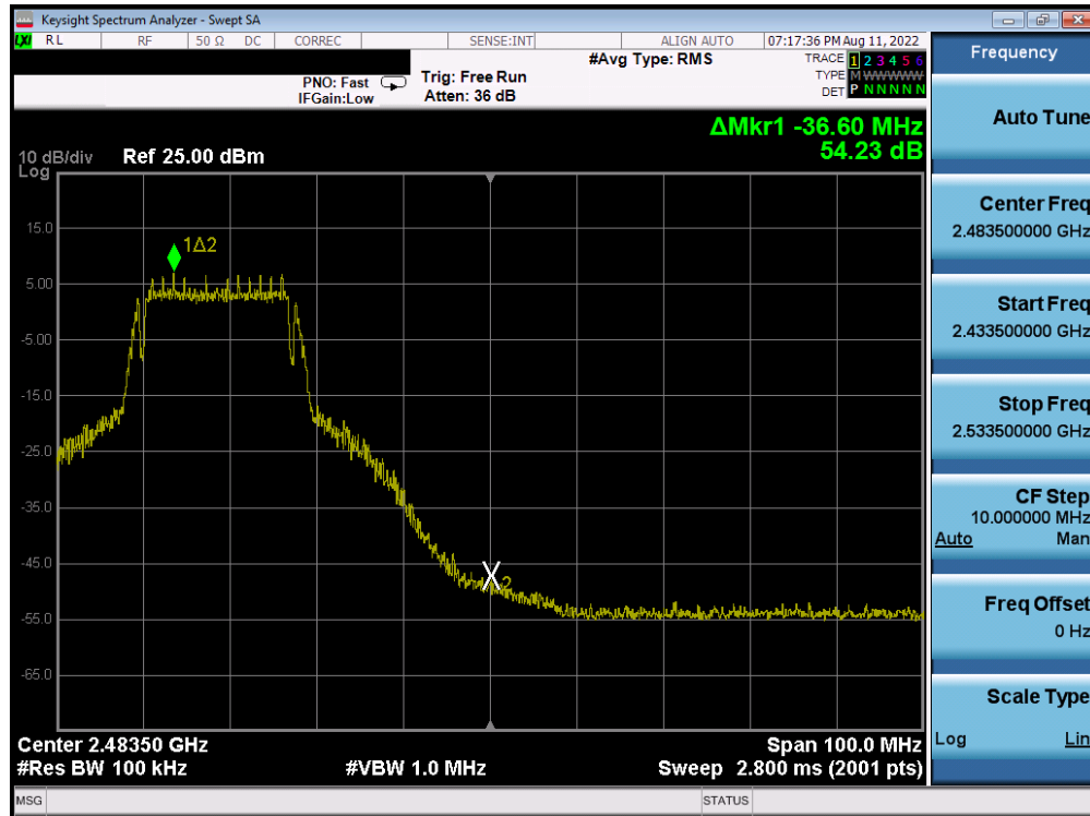
Plot 7-33. Band Edge Plot Antenna 1 (802.11g – Ch. 9)
