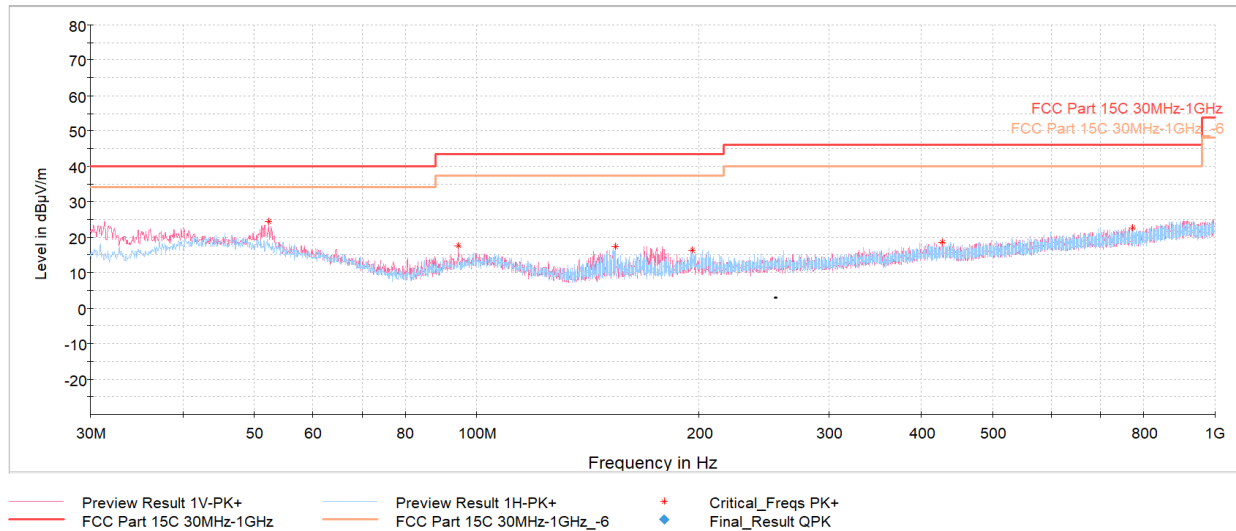
Plot 7-38. Radiated Spurious Emissions Below 1GHz (HDR4 ePA – Ch.38 with AC/DC Adapter + Magnetic Charger)
