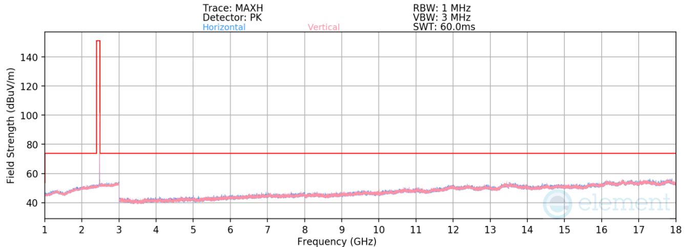
Plot 7-31. Radiated Spurious Emissions 1-18GHz (4Mbps, HDR4, ePA – Ch. 75)
