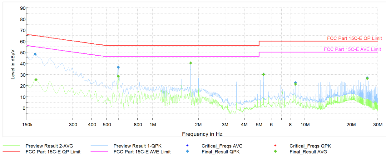
Plot 7-40. AC Line Conducted Plot with Bluetooth HDR (N, 4Mbps ePA - Ch.1 with AC/DC Adapter + Magnetic Charger)
