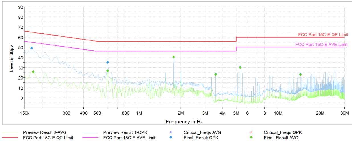
Plot 7-39. AC Line Conducted Plot with Bluetooth HDR (L1, 4Mbps ePA - Ch.1 with AC/DC Adapter + Laptop Charger)
