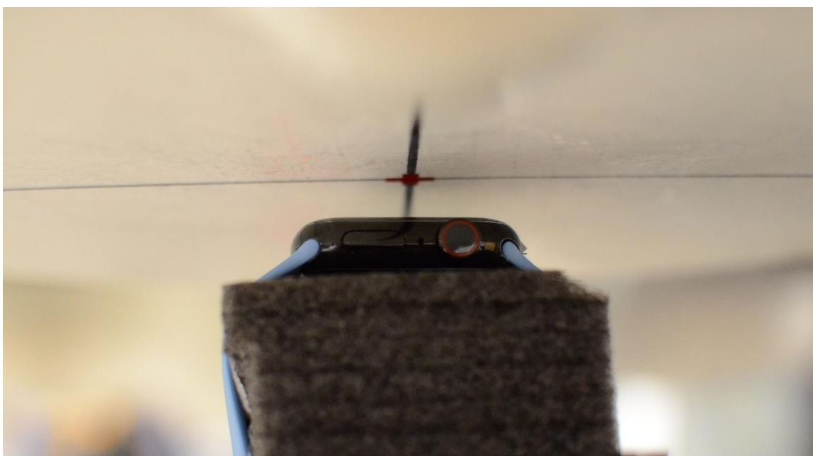
SAR Test Setup Photo 4: Head, Stainless Steel with Sport Wristband, Front side at 1.0 cm
