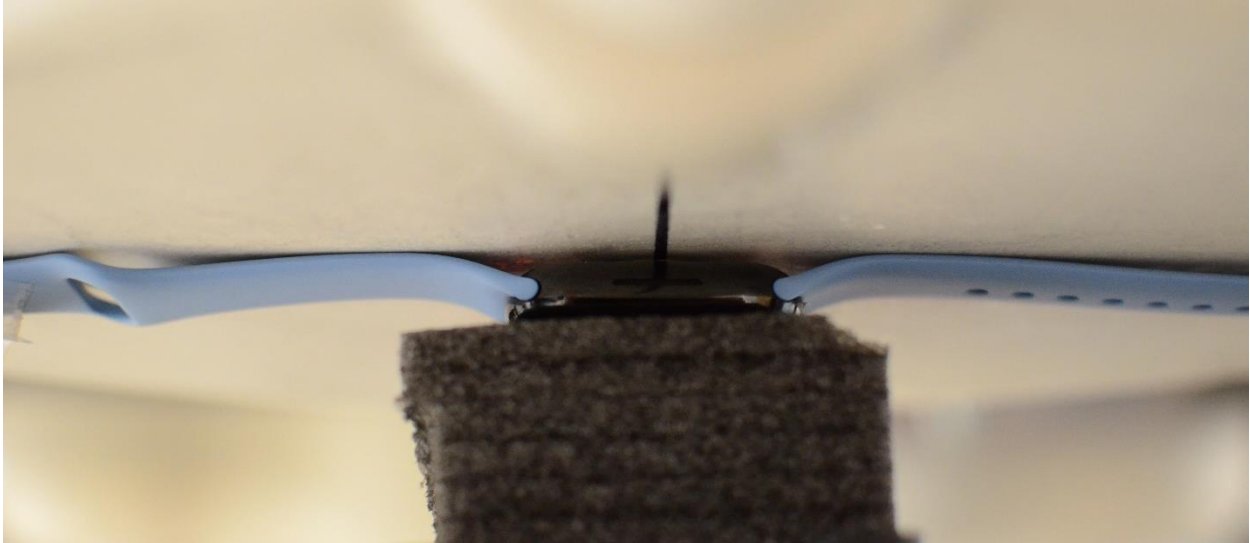
SAR Test Setup Photo 13: Extremity, Stainless Steel with Sport Wristband, Back side at 0.0 cm
