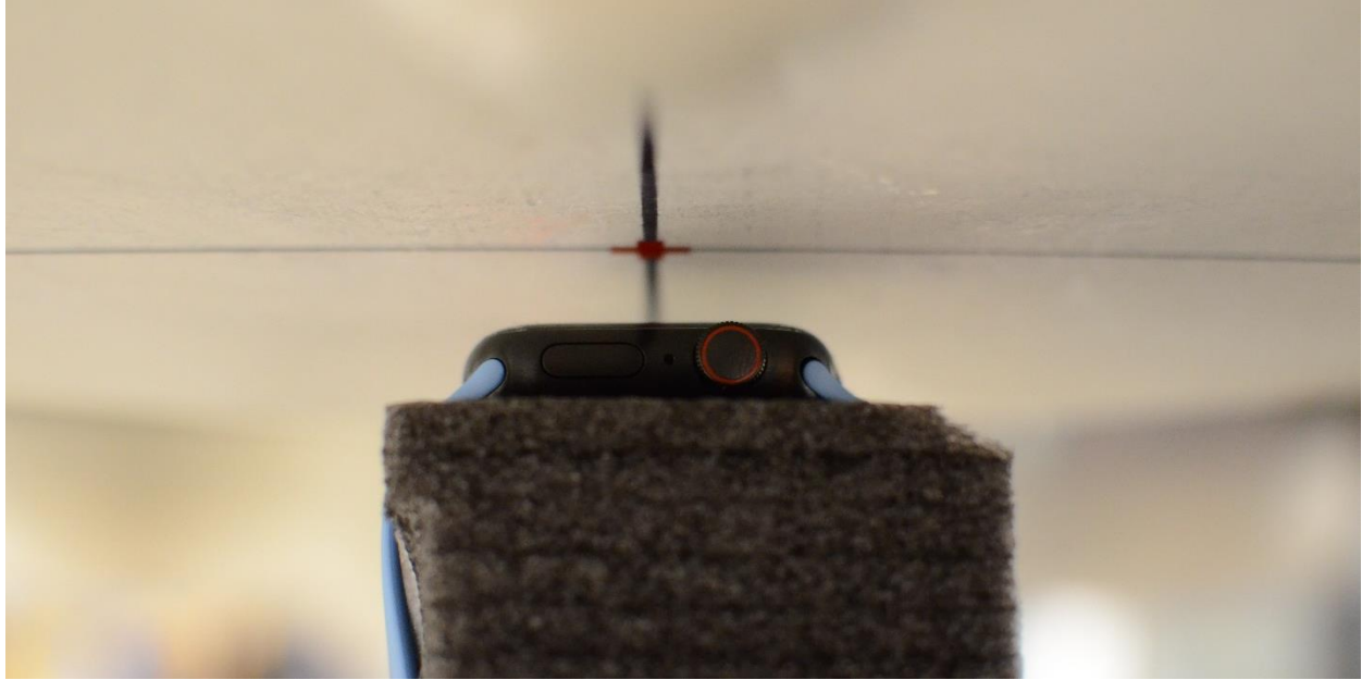
SAR Test Setup Photo 7: Head, Titanium with Sport Wristband, Front side at 1.0 cm
