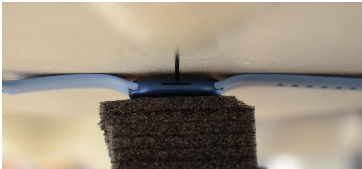
SAR Test Setup Photo 10: Extremity, Aluminum with Sport Wristband, Back side at 0.0 cm
