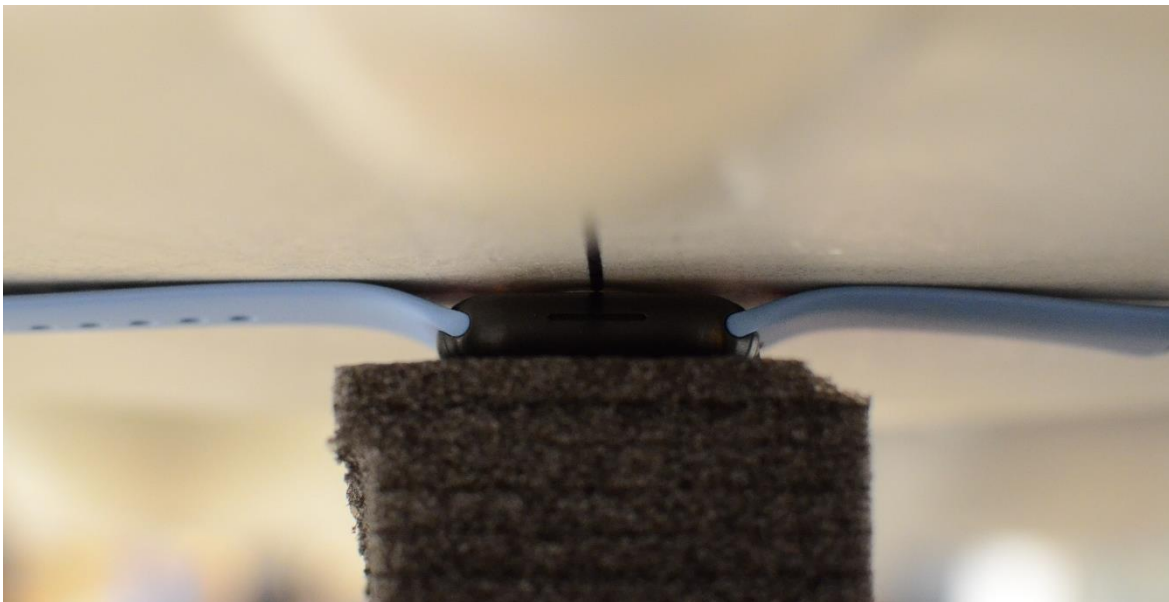
SAR Test Setup Photo 16: Extremity, Titanium with Sport Wristband, Back side at 0.0 cm
