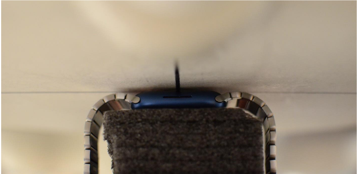
SAR Test Setup Photo 11: Extremity, Aluminum with Metal Links Wristband, Back side at 0.0 cm
