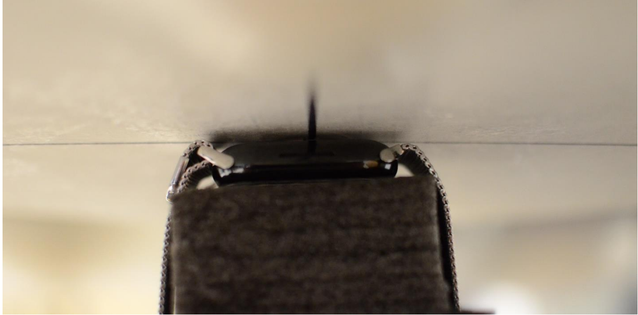
SAR Test Setup Photo 15: Extremity, Stainless Steel with Metal Loop Wristband, Back side at 0.0 cm
