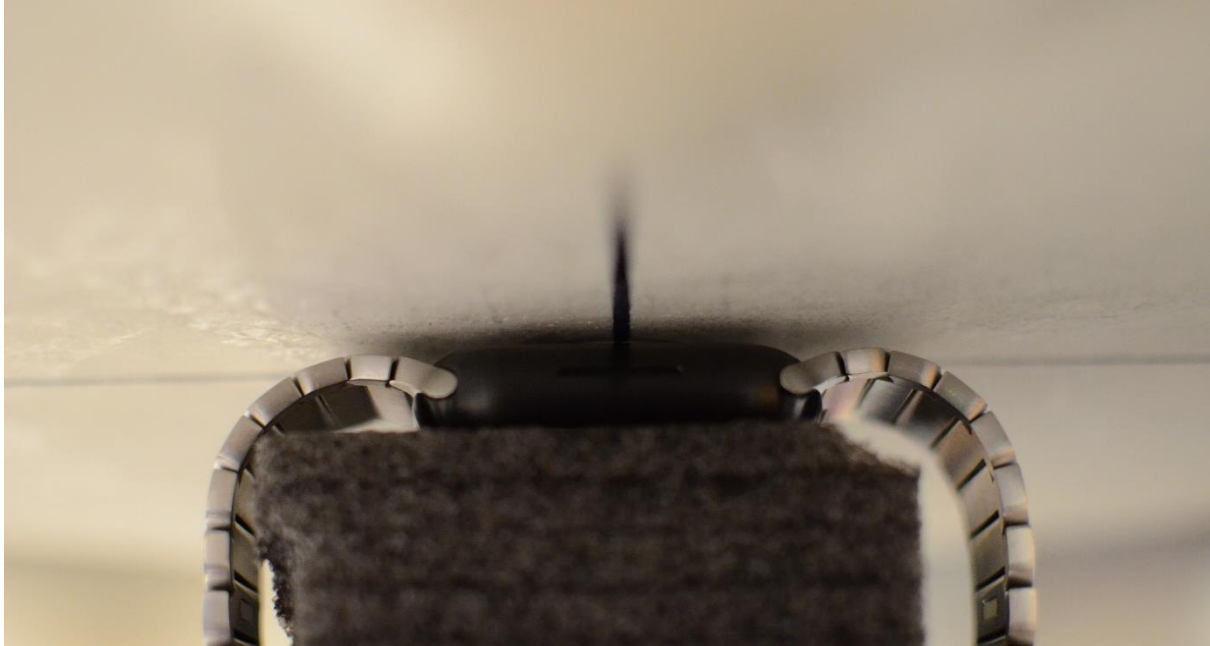
SAR Test Setup Photo 17: Extremity, Titanium with Metal Links Wristband, Back side at 0.0 cm
