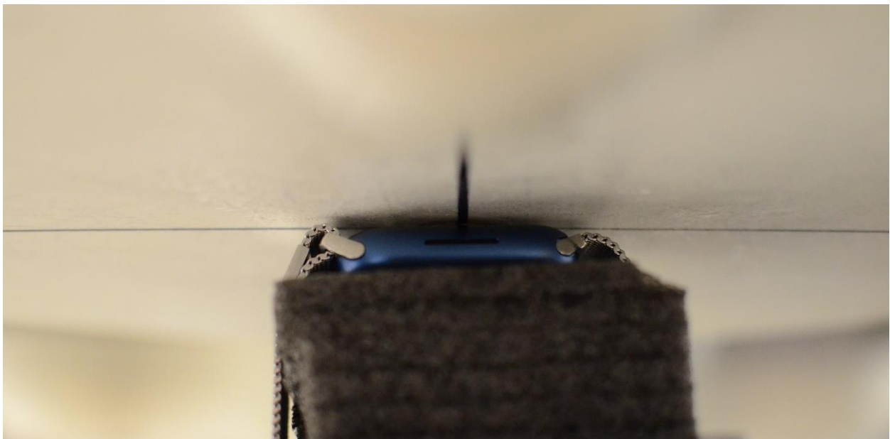
SAR Test Setup Photo 12: Extremity, Aluminum with Metal Loop Wristband, Back side at 0.0 cm
