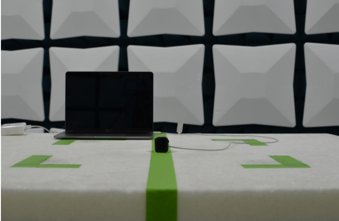
Figure 21: 30MHz-1GHz Test Setup (Front View)
