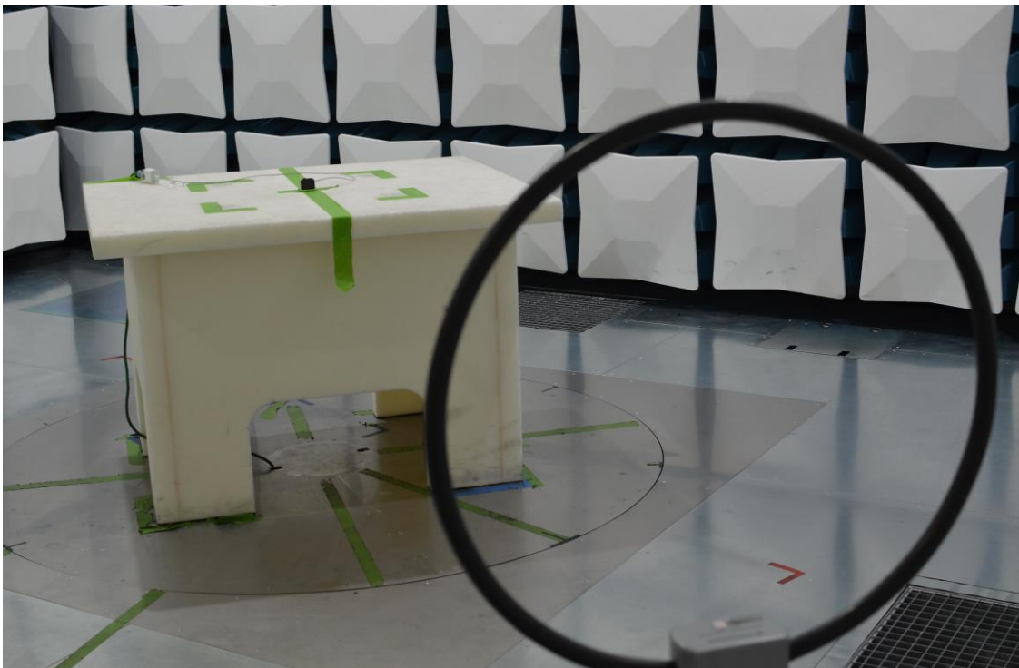
Figure 24: 9kHz-30MHz Test Setup (Front View)
