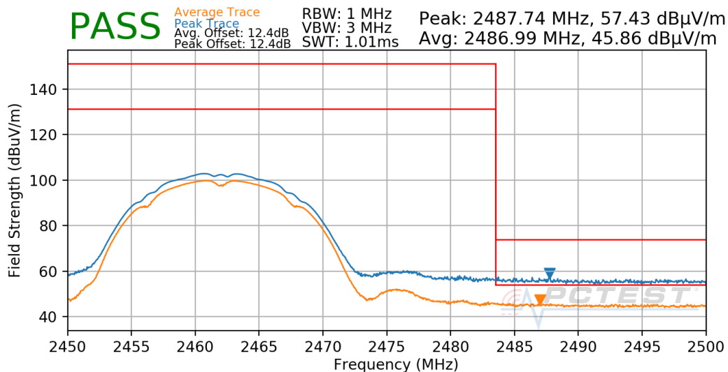
Plot 7-59. Radiated Restricted Upper Band Edge Measurement
