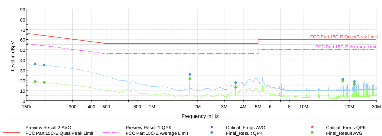
Plot 7-75.AC Line Conducted Plot 802.11b – Ch.6 (N), with AC/DC Adapter and Magnetic Charger
