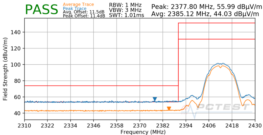
Plot 7-58. Radiated Restricted Lower Band Edge Measurement
