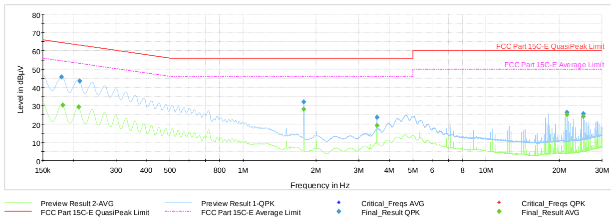
Plot 7-74.AC Line Conducted Plot 802.11b – Ch.6 (L1), with AC/DC Adapter and Magnetic Charger
