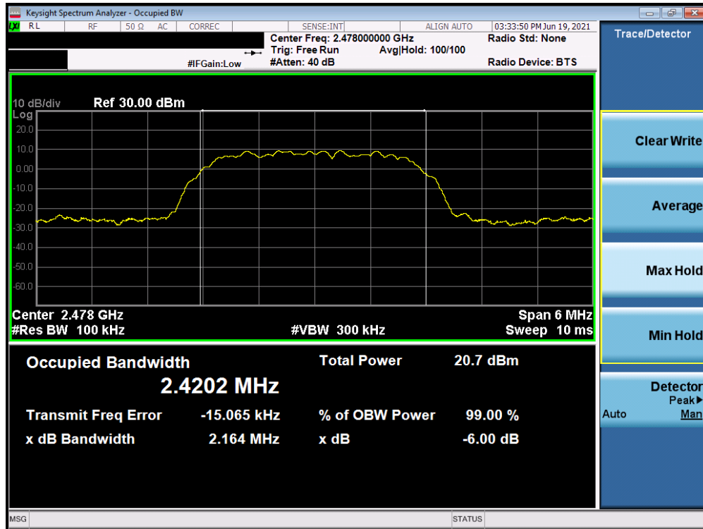
Plot 7-3. 6dB and 99% OBW Plot (Bluetooth (HDR4), 4Mbps, ePA – Ch. 75)
