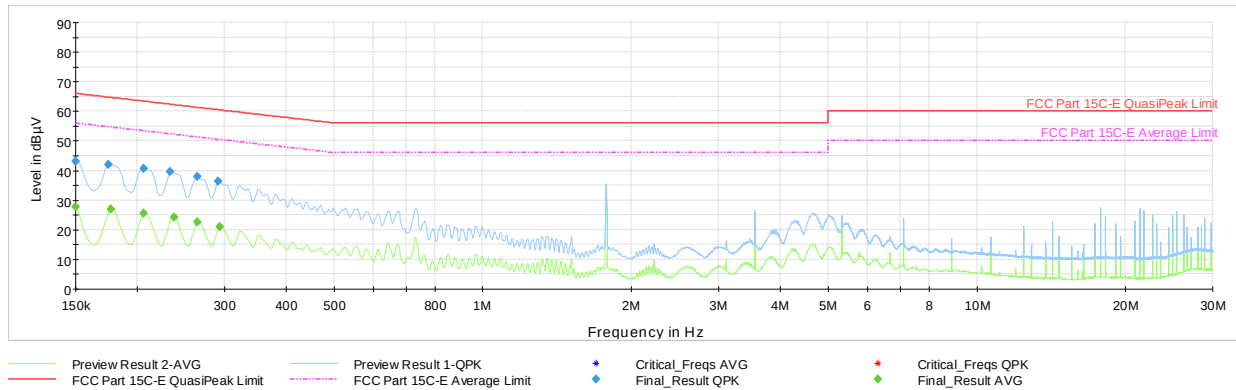
Plot 7-40. AC Line Conducted Emissions with Bluetooth HDR (N, 4Mbps ePA – Ch.38 with AC/DC Adapter + Magnetic Charger)
