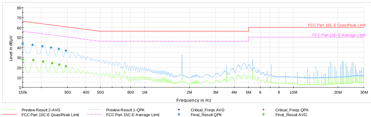
Plot 7-39. AC Line Conducted Emissions with Bluetooth HDR (L1, 4Mbps ePA – Ch.38 with AC/DC Adapter + Magnetic Charger)
