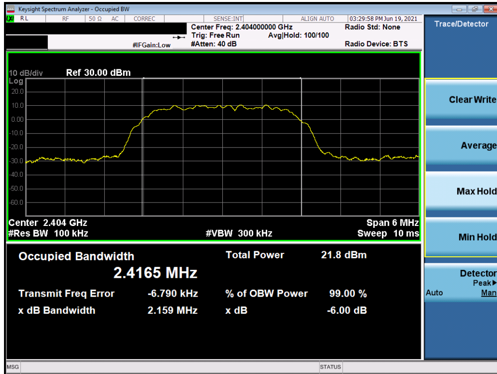
Plot 7-1. 6dB and 99% OBW Plot (Bluetooth (HDR4), 4Mbps, ePA – Ch. 1)
