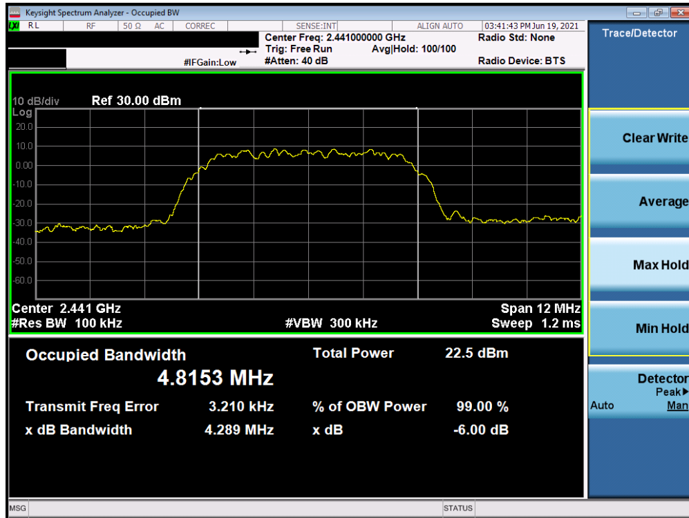
Plot 7-5. 6dB and 99% OBW Plot (Bluetooth (HDR8), 8Mbps, ePA – Ch. 38)
