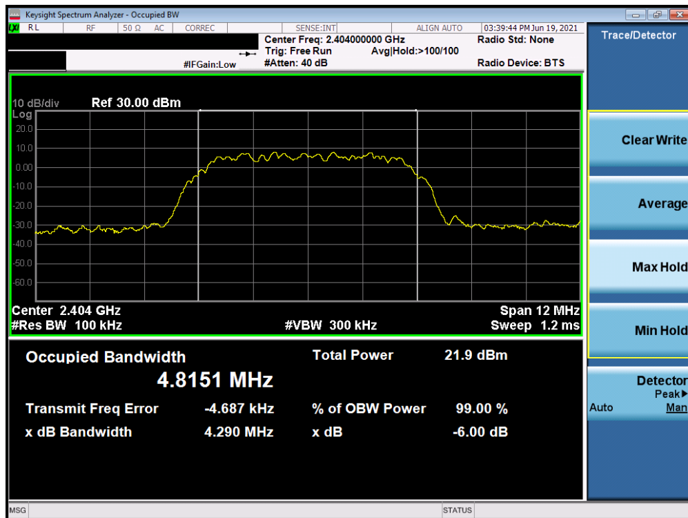
Plot 7-4. 6dB and 99% OBW Plot (Bluetooth (HDR8), 8Mbps, ePA – Ch. 1)
