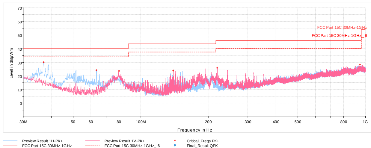
Plot 7-38. Radiated Spurious Emissions below 1GHz (HDR4 ePA – Ch.38, Pol. H & V, with AC/DC Adapter + Magnetic Charger)
