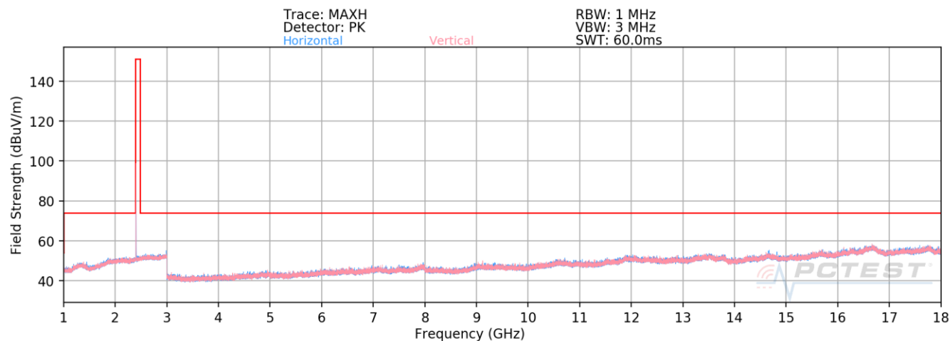
Plot 7-29. Radiated Spurious Emissions Above 1GHz (4Mbps, HDR4, ePA – Ch. 1, Ant. Pol. H & V)
