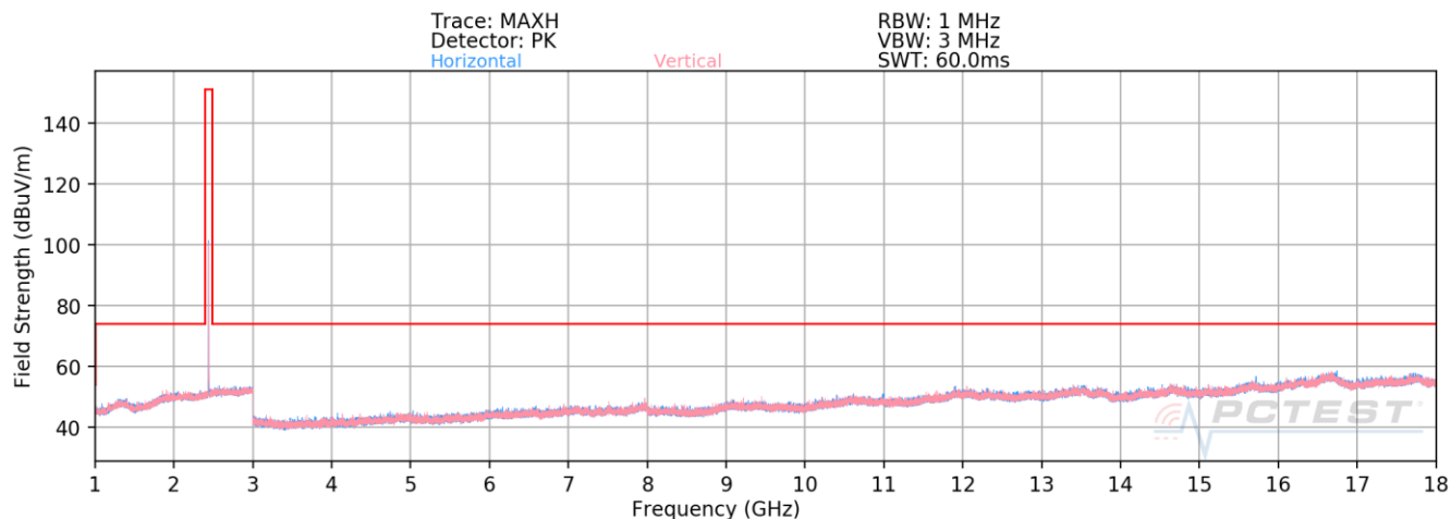
Plot 7-30. Radiated Spurious Emissions Above 1GHz (4Mbps, HDR4, ePA – Ch. 38, Ant. Pol. H & V)
