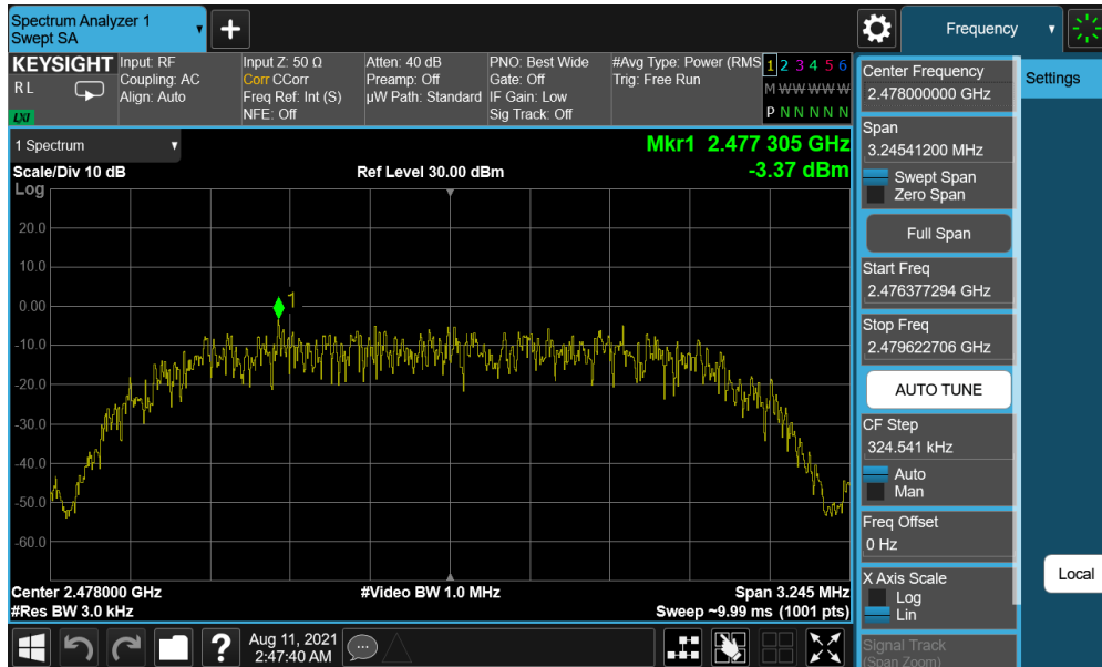
Plot 7-9. Power Spectral Density Plot (Bluetooth (HDR4), 4Mbps, ePA – Ch. 75)
