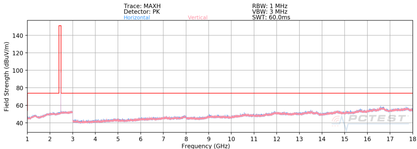
Plot 7-31. Radiated Spurious Emissions Above 1GHz (4Mbps, HDR4, ePA – Ch. 75, Ant. Pol. H & V)
