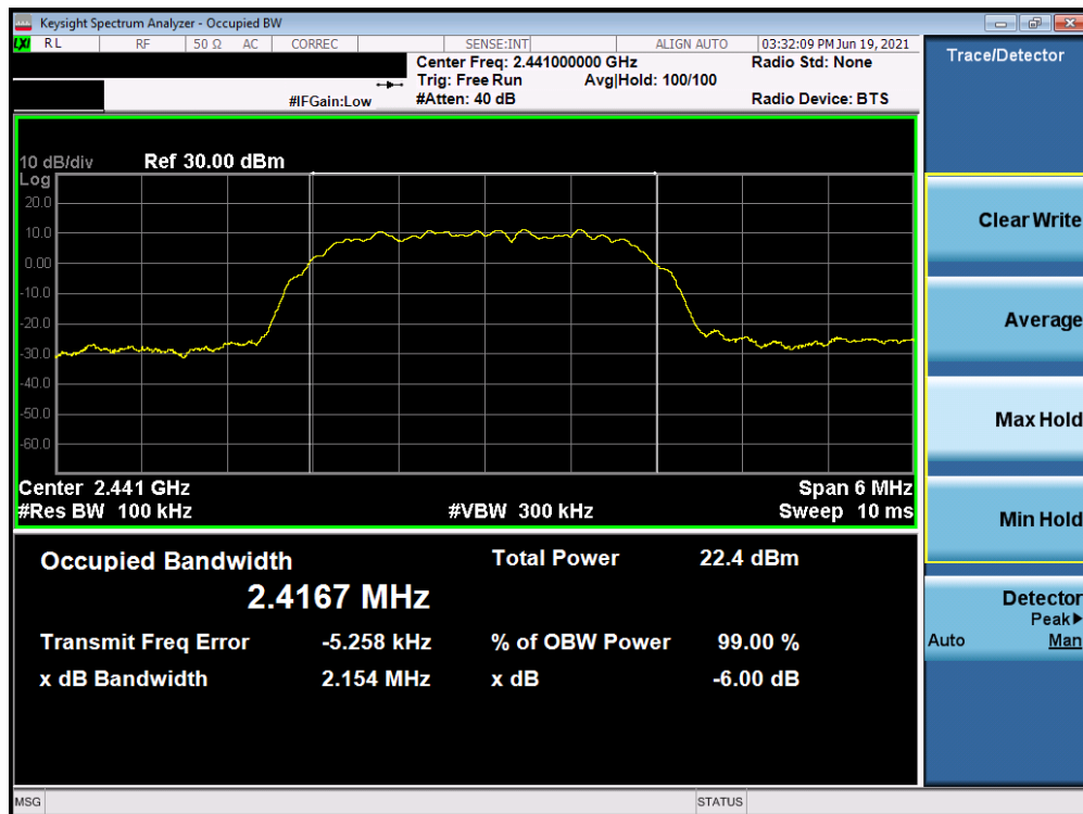
Plot 7-2. 6dB and 99% OBW Plot (Bluetooth (HDR4), 4Mbps, ePA – Ch. 38)
