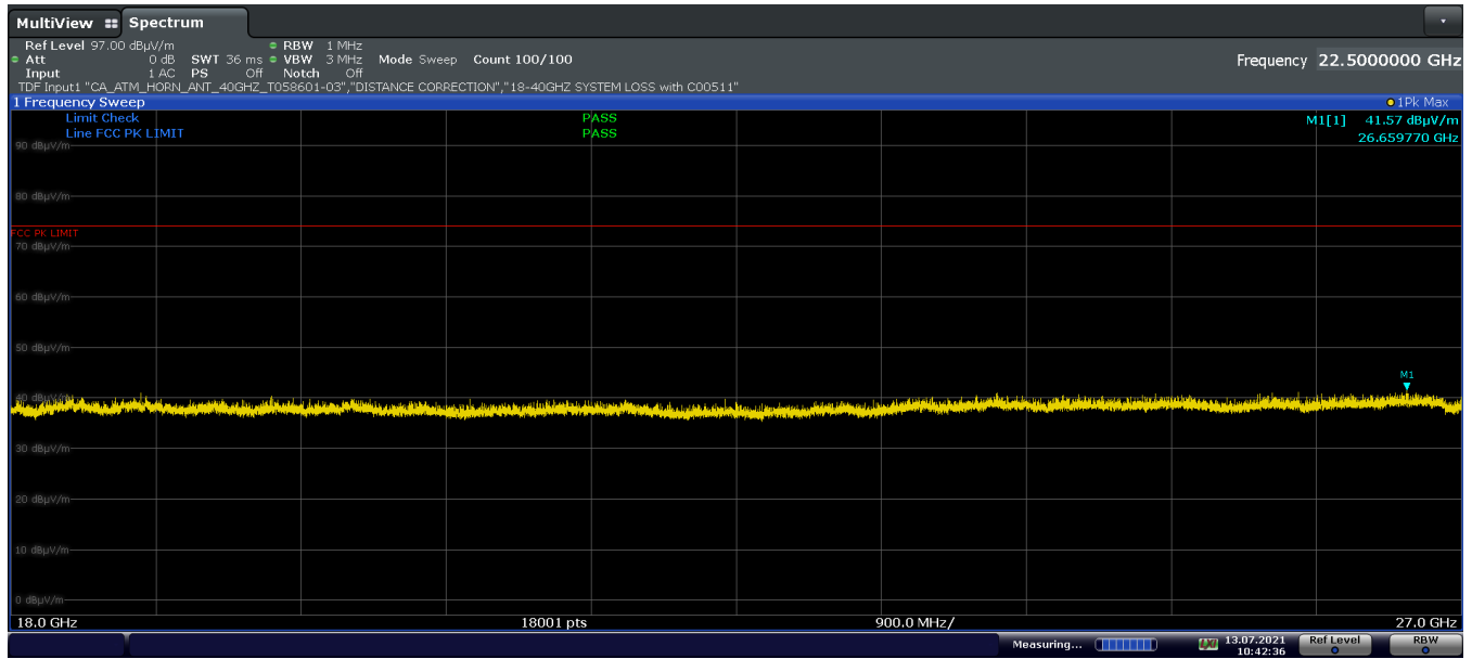
Plot 7-32. Radiated Spurious Plot Above 18GHz (4Mbps, HDR4, ePA – Ch.38, Ant. Pol. H)
