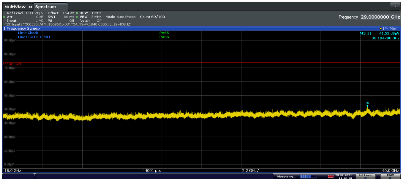
Plot 7-36. Radiated Spurious Emissions above 18GHz – Simultaneous Transmission (Pol. V)
