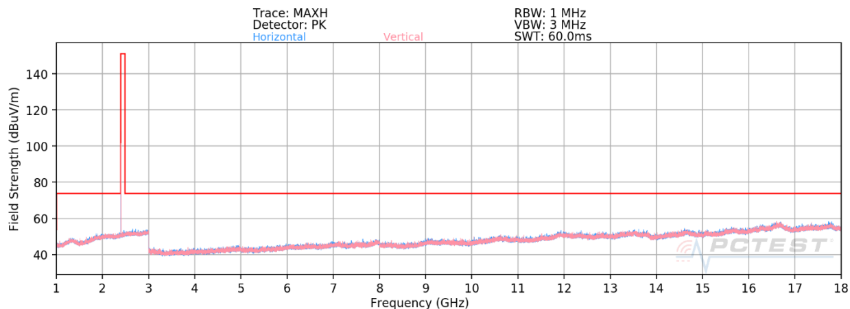
Plot 7-29. Radiated Spurious Emissions above 1GHz (BT GFSK ePA – Ch. 0)
