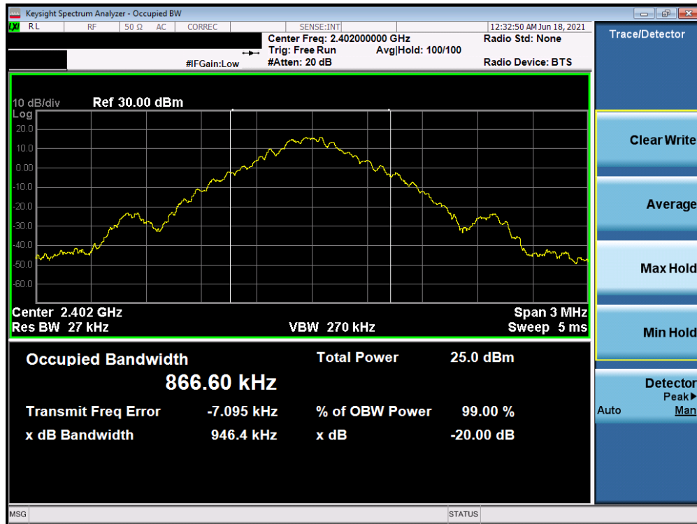
Plot 7-1. Conducted 20dB and 99% OBW Plot (Bluetooth, GFSK, ePA – Ch. 0)
