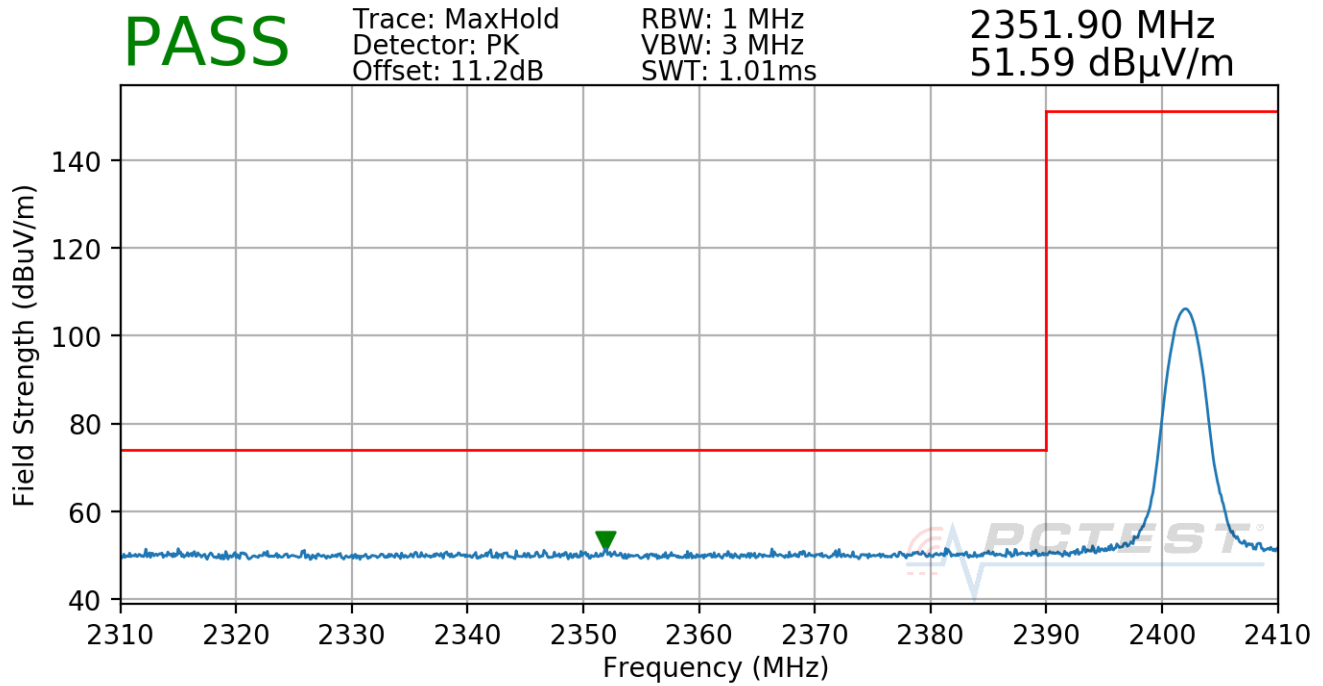
7-39. Radiated Restricted Lower Band Edge Measurement (Peak)
