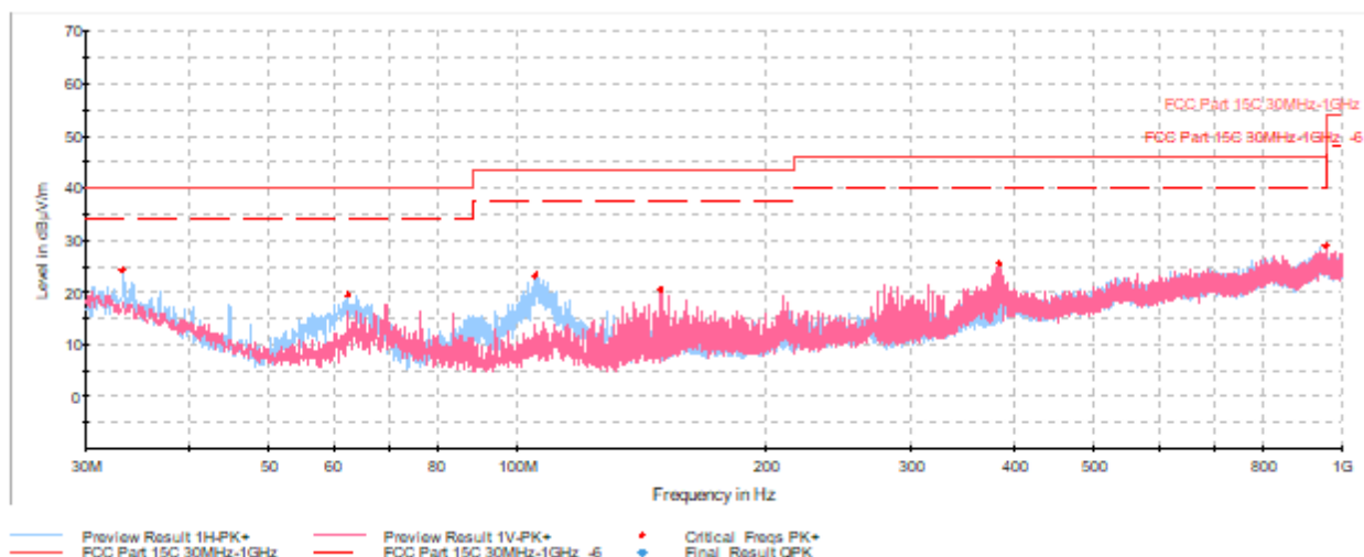
Plot 7-41. Radiated Spurious Plot below 1GHz (GFSK ePA – Ch.39, Pol. H & V, with 39 with AC/DC Adapter and Magnetic Charger)
