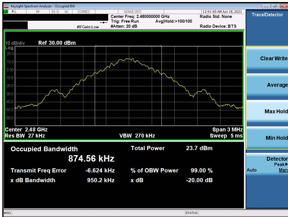
Plot 7-3. Conducted 20dB and 99% OBW Plot (Bluetooth, GFSK, ePA – Ch. 78)
