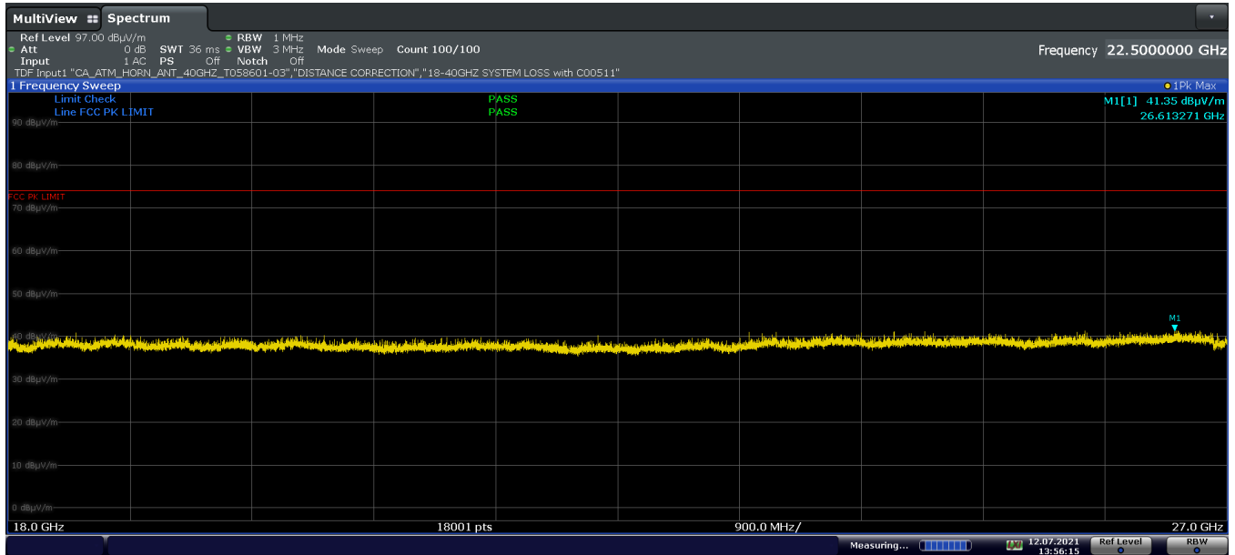
Plot 7-32. Radiated Spurious Emissions above 18GHz (GFSK ePA – Ch.39, Pol. H)
