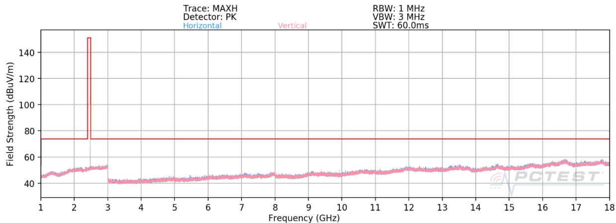
Plot 7-31. Radiated Spurious Emissions above 1GHz (BT GFSK ePA – Ch. 78)
