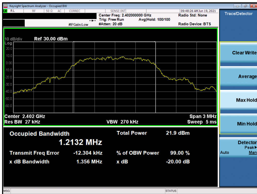
Plot 7-4. Conducted 20dB and 99% OBW Plot (Bluetooth, 8DPSK, ePA – Ch. 0)
