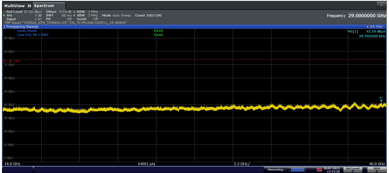
Plot 7-35. Radiated Spurious Emissions above 18GHz – Simultaneous Transmission (Pol. H)
