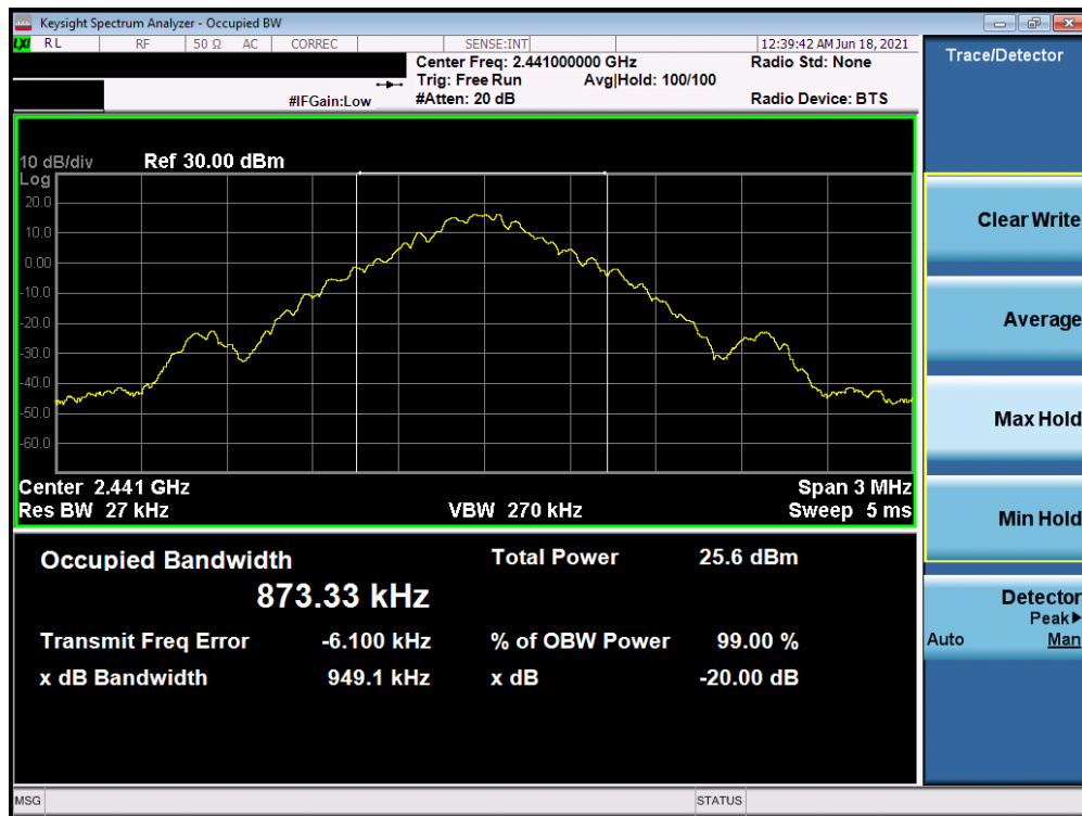
Plot 7-2. Conducted 20dB and 99% OBW Plot (Bluetooth, GFSK, ePA – Ch. 39)
