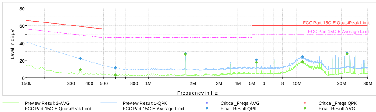
Plot 7-43. AC Line-Conducted Test Plot (L1, GFSK – Ch.39, with AC/DC Adapter + Magnetic Charger)
