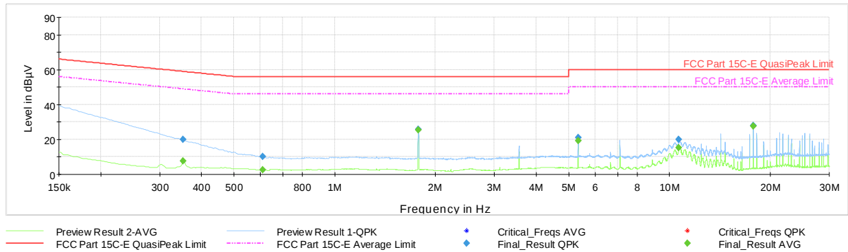
Plot 7-44. AC Line-Conducted Test Plot (N, GFSK – Ch.39, with AC/DC Adapter + Magnetic Charger)
