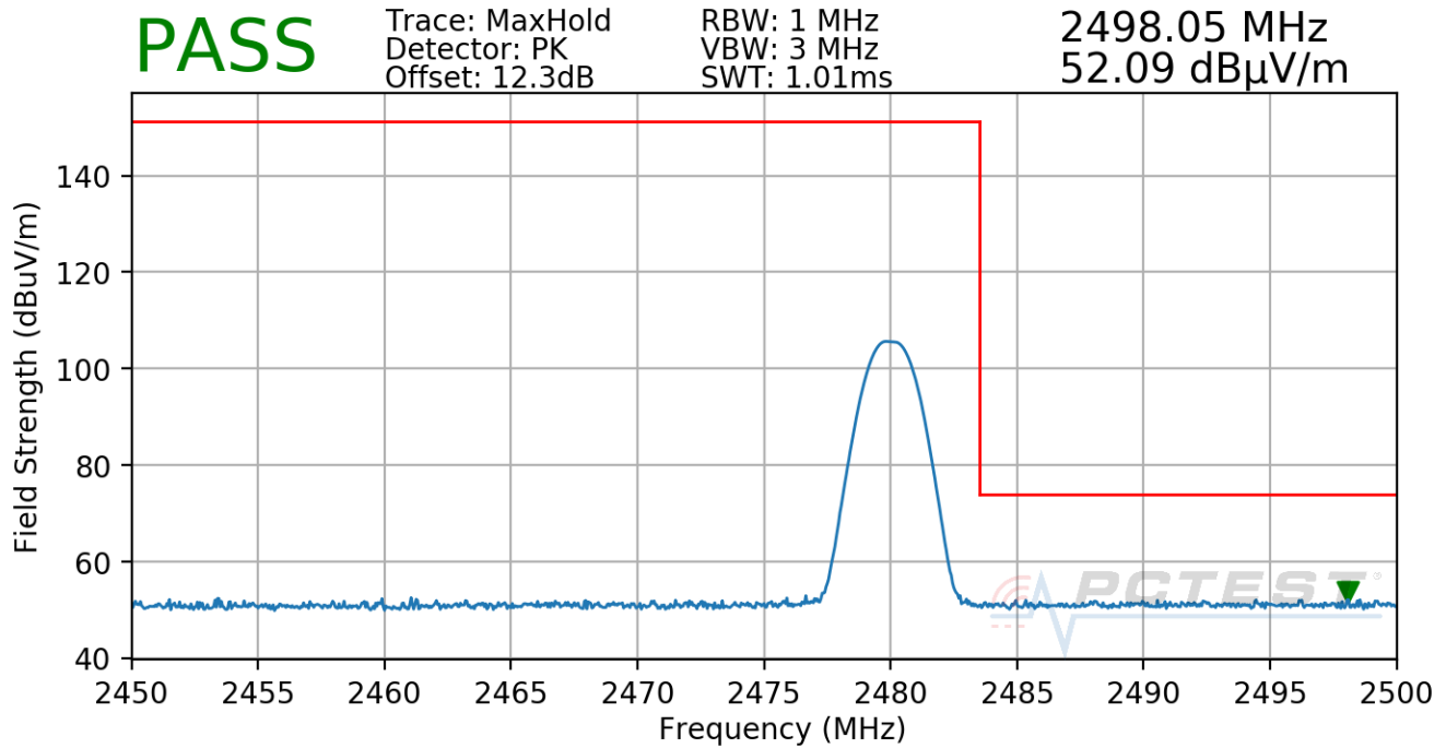
Plot 7-38. Radiated Restricted Lower Upper Band Edge Measurement (Peak)
