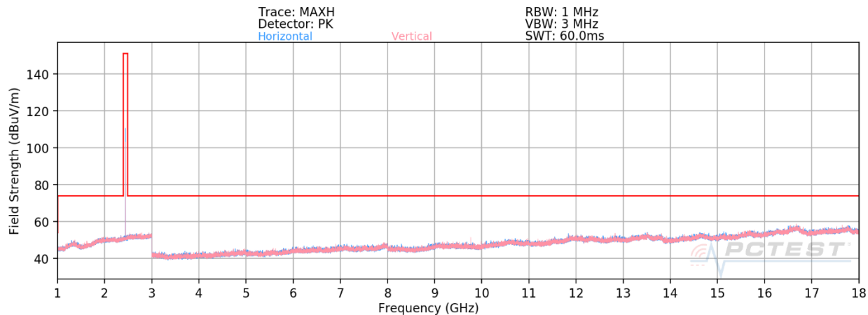
Plot 7-30. Radiated Spurious Emissions above 1GHz (BT GFSK ePA – Ch. 39)
