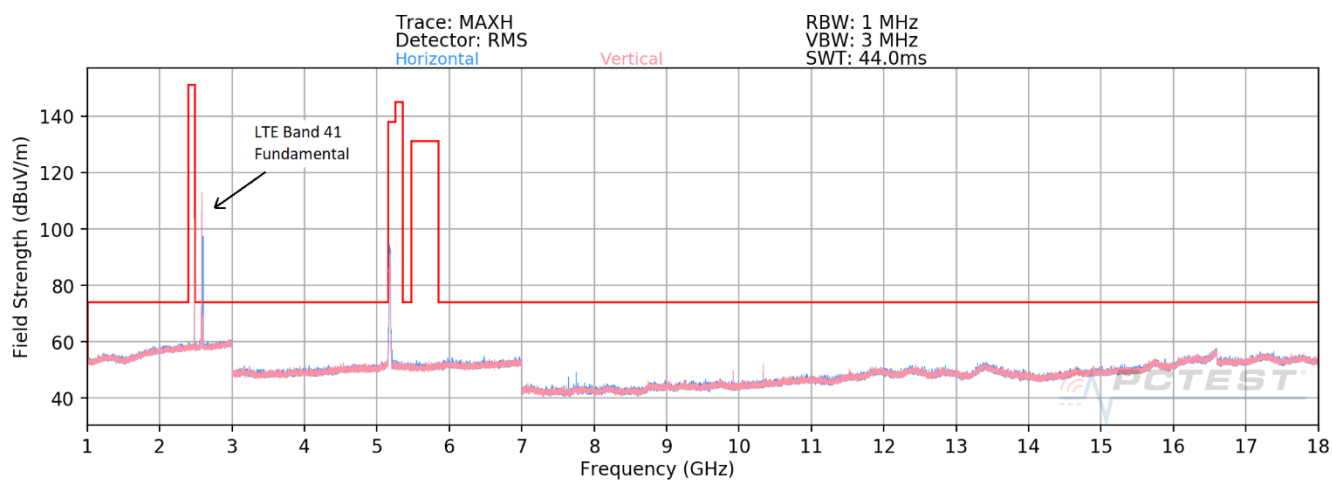
Plot 7-34. Radiated Spurious Emissions – Simultaneous Transmission 1GHz - 18GHz
