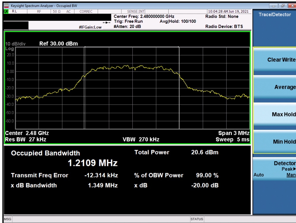
Plot 7-6. Conducted 20dB and 99% OBW Plot (Bluetooth, 8DPSK, ePA – Ch. 78)
