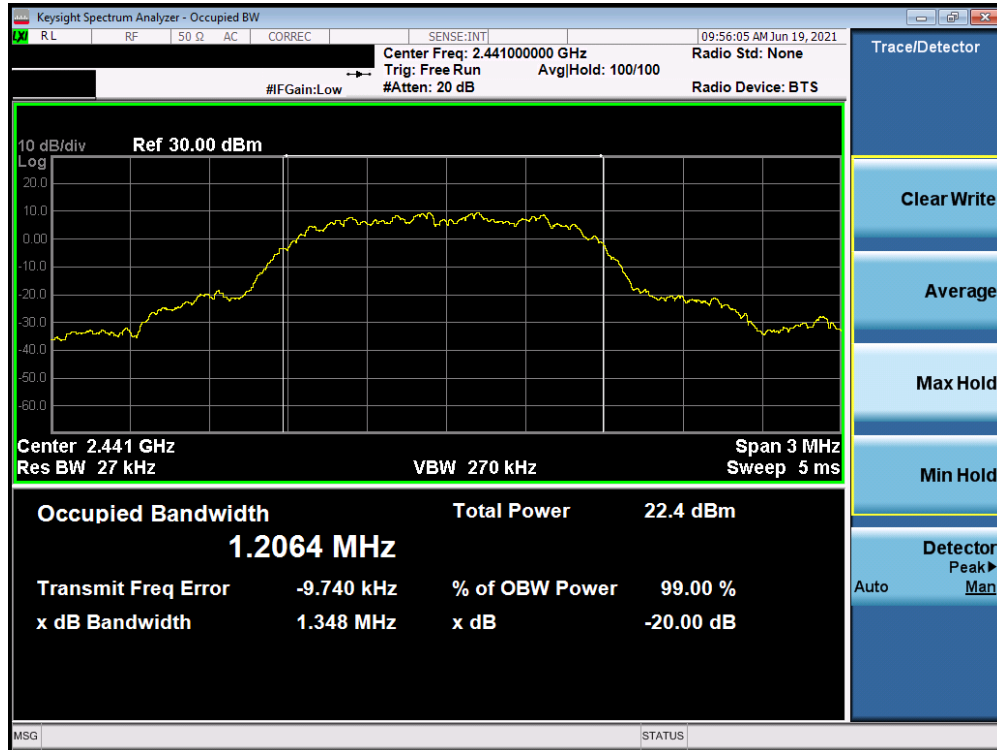
Plot 7-5. Conducted 20dB and 99% OBW Plot (Bluetooth, 8DPSK, ePA – Ch. 39)
