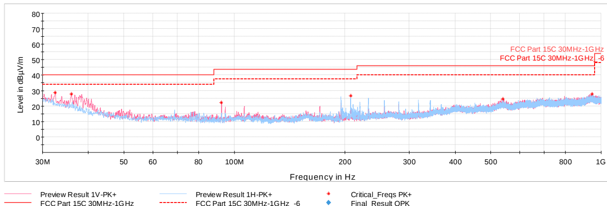
Plot 7-42. Radiated Spurious Plot below 1GHz – Simultaneous Transmission, with AC/DC Adapter and Magnetic Charger.
