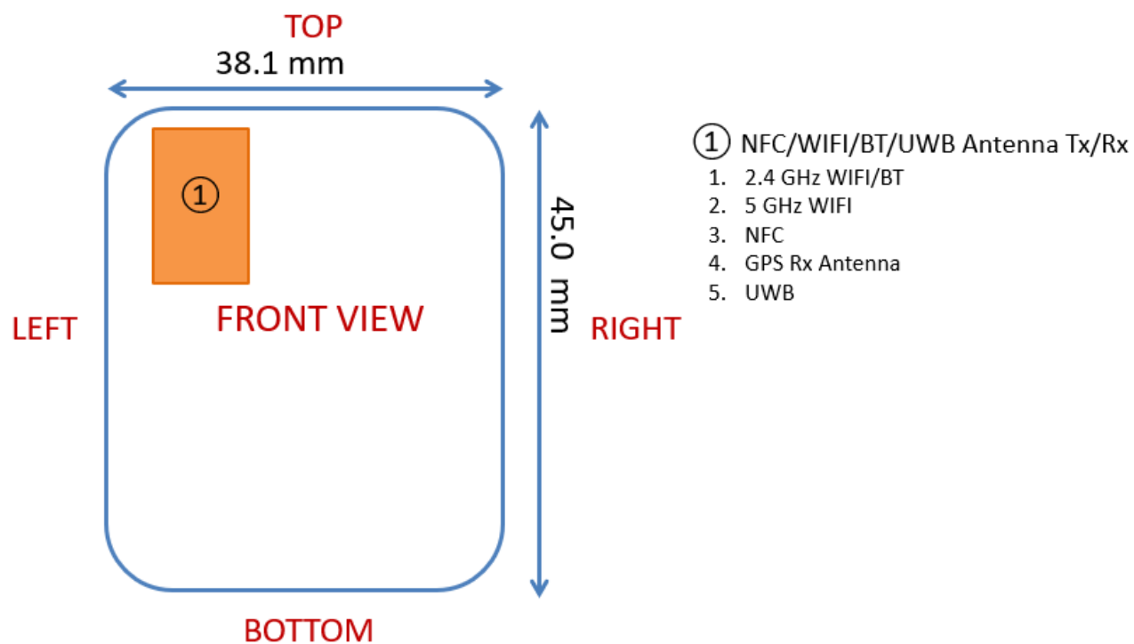
Figure E-1 DUT Antenna Locations
