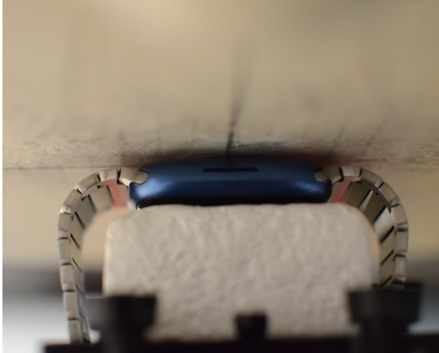
SAR Test Setup Photo 5: Aluminum with Metal Links Wrist Band, Extremity, Back Side at 0.0 cm
