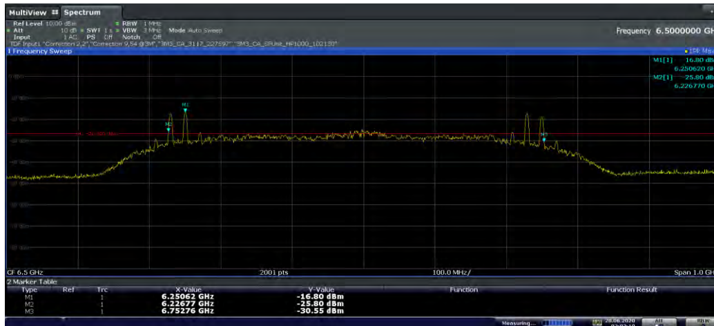
Plot 7-6. 10dBc Bandwidth (Ch. 5, Config 1/Payload 125)
