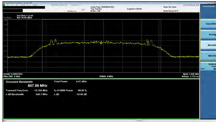
Plot 7-21. ISSED Occupied Bandwidth (Ch. 5, Config 0/Payload 25)
