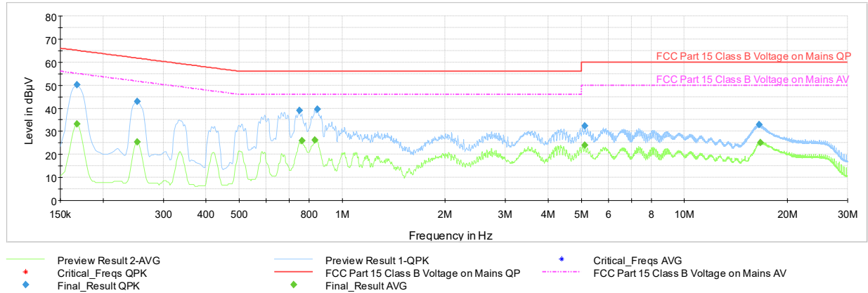
Plot 7-114. AC Line Conducted (Ch. 5, Config 3, Payload 125 N, with WCP + AC/DC Adapter)
