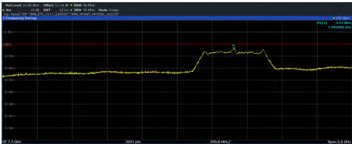
Plot 7-53. Peak Radiated Power (Ch. 9, Config 0/Payload 125)
