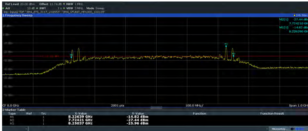
Plot 7-14. 10dBc Bandwidth (Ch. 9, Config 1/Payload 45)
