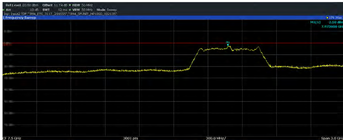
Plot 7-51. Peak Radiated Power (Ch. 9, Config 0/Payload 25)
