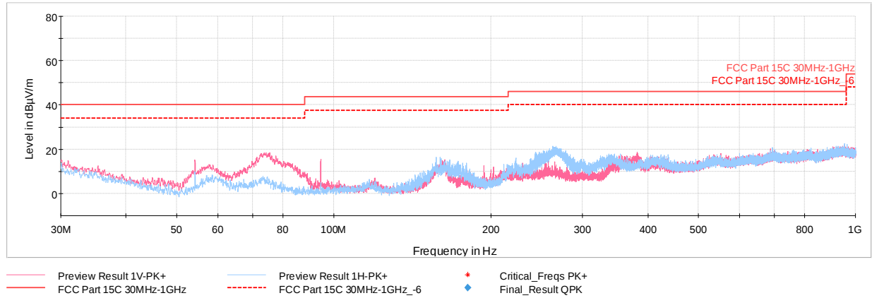
Plot 7-10. Radiated Spurious Emissions 30MHz – 1GHz (CE A 848kbps, with WCP + AC/DC Adapter)
