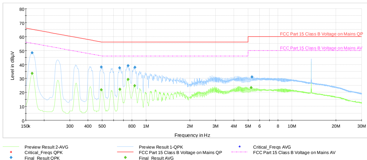
Plot 7-13. AC Line-Conducted Test Plot (N, with WCP + AC/DC Adapter)
