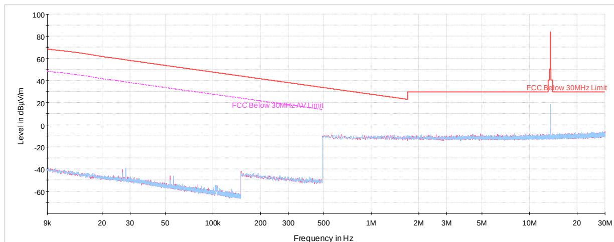
Plot 7-8. Radiated Spurious Emissions 9kHz – 30MHz (CE A 848kbps, with WCP + AC/DC Adapter)
