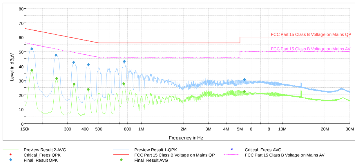
Plot 7-12. AC Line-Conducted Test Plot (L1, with WCP + AC/DC Adapter)
