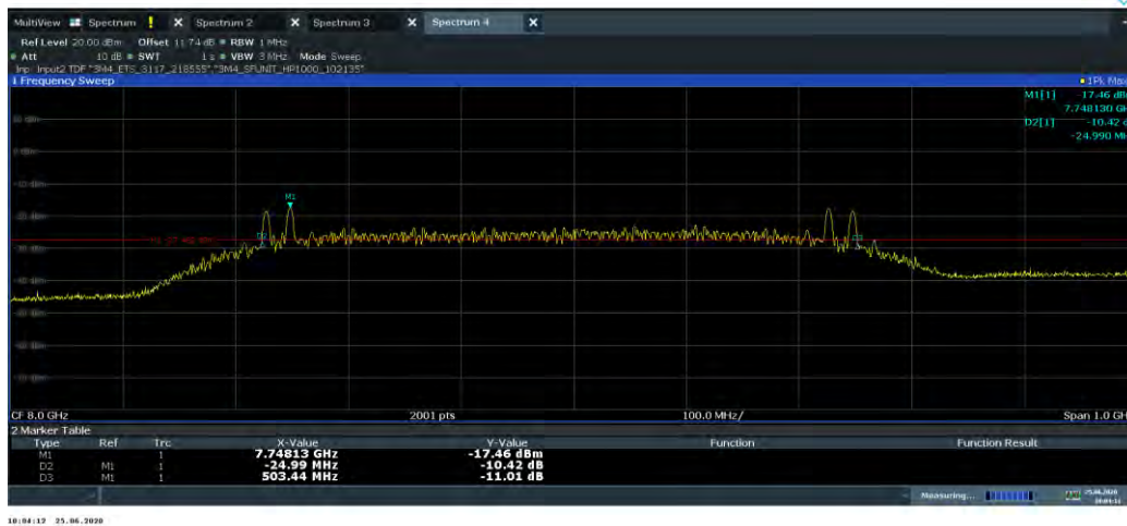
Plot 7-20. 10dBc Bandwidth (Ch. 9, Config 5/Payload 0)
