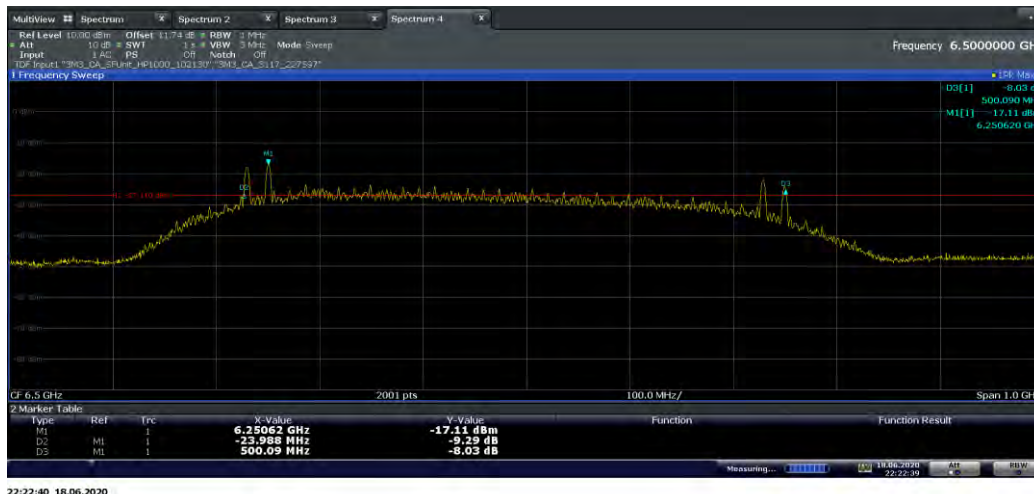
Plot 7-9. 10dBc Bandwidth (Ch. 5, Config 4/Payload 0)
