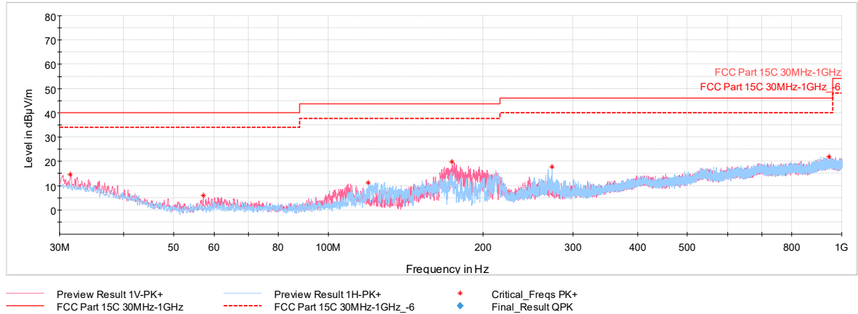
Plot 7-116. Radiated Spurious Emission – Simultaneous Transmission below 960 MHz with WCP + AC/DC Adapter
