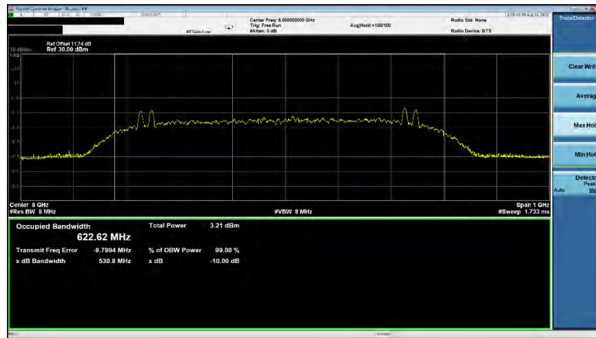
Plot 7-31. ISSED Occupied Bandwidth (Ch. 9, Config 0/Payload 25)
