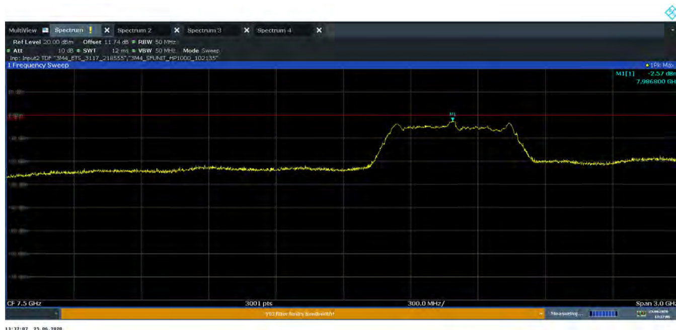
Plot 7-52. Peak Radiated Power (Ch. 9, Config 0/Payload 65)
