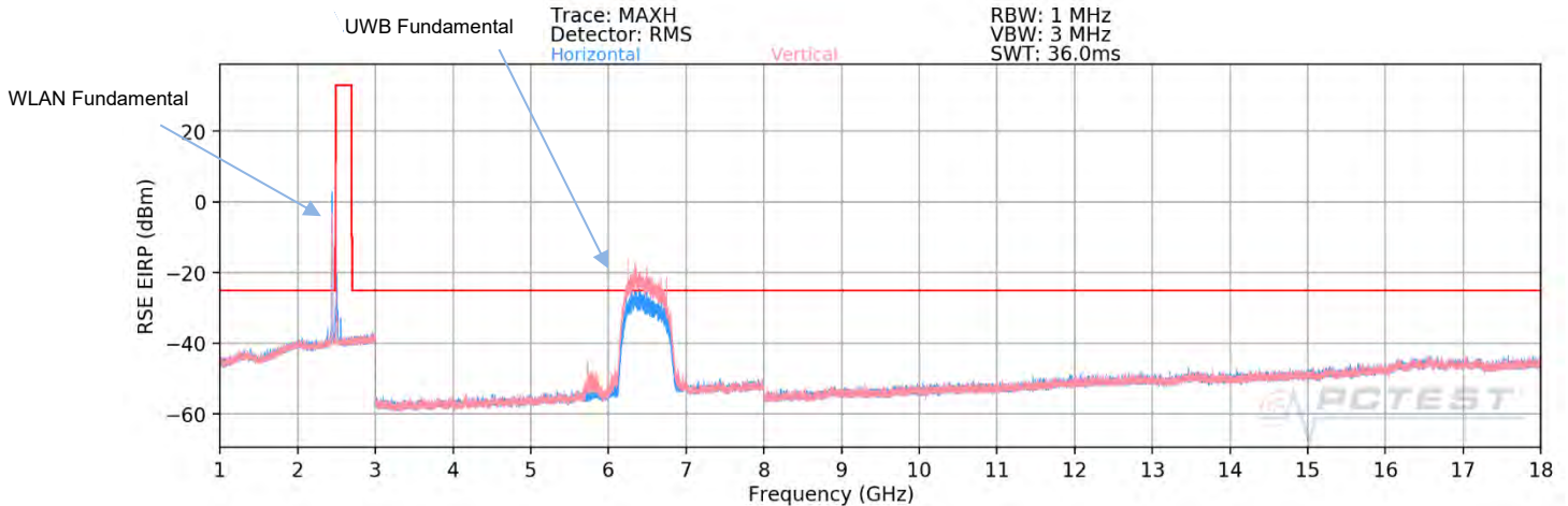
Plot 7-111. Radiated Spurious Simultaneous TX 1-18GHz (Ch. 5, Config 3, Payload 125)
