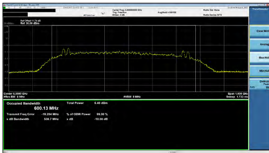
Plot 7-21. ISCED Occupied Bandwidth (Ch. 5, Config 0/Payload 25)
