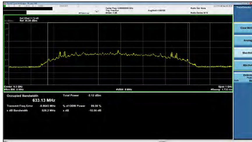
Plot 7-27. ISSED Occupied Bandwidth (Ch. 5, Config 2/Payload 125)
