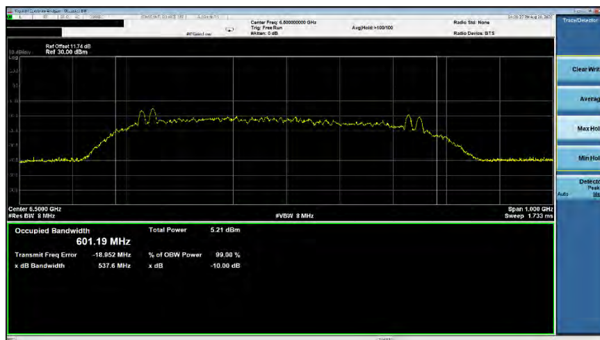
Plot 7-23. ISCED Occupied Bandwidth (Ch. 5, Config 0/Payload 125)
