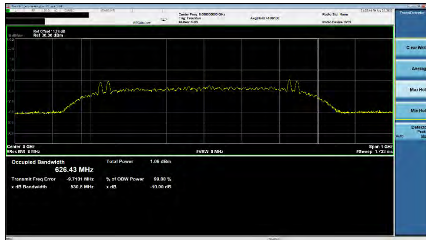
Plot 7-33. ISSED Occupied Bandwidth (Ch. 9, Config 0/Payload 125)
