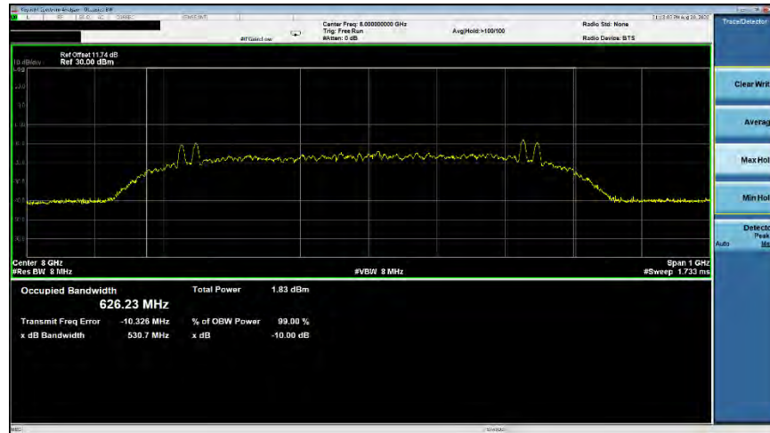
Plot 7-32. ISSED Occupied Bandwidth (Ch. 9, Config 0/Payload 65)
