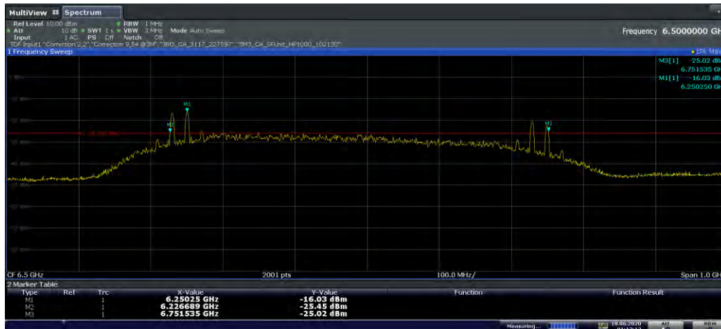
Plot 7-2. 10dBc Bandwidth (Ch. 5, Config 0/Payload 65)
