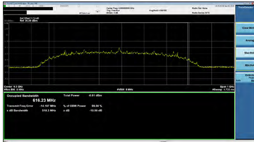
Plot 7-28. ISSED Occupied Bandwidth (Ch. 5, Config 3/Payload 125)
