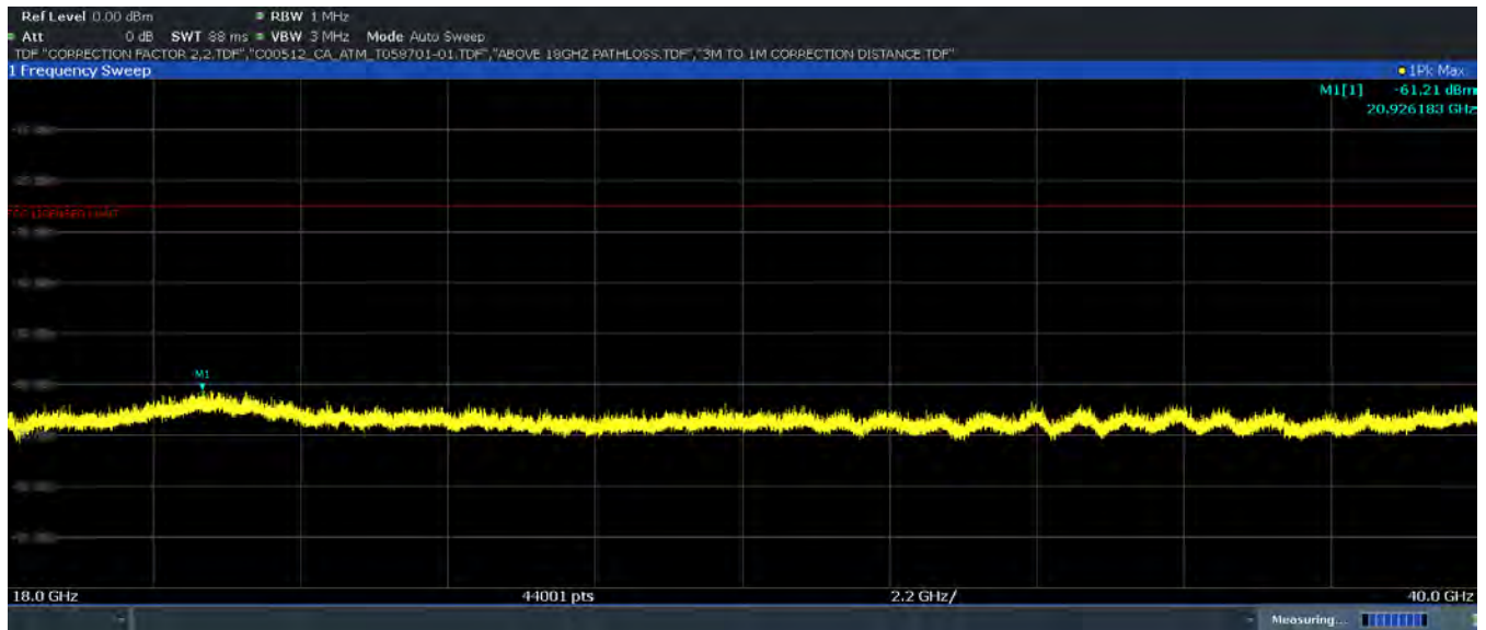
Plot 7-113. Radiated Spurious Emission- Simultaneous Transmission 18GHz-40GHz Pol. V
