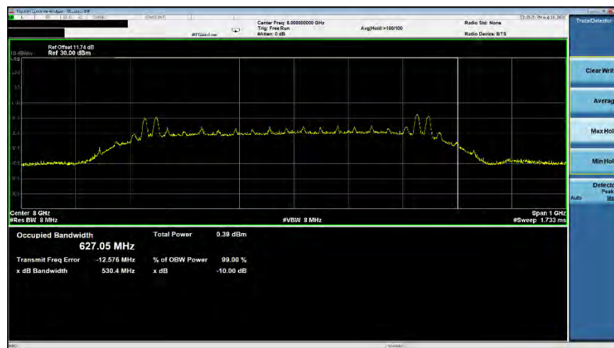
Plot 7-39. ISSED Occupied Bandwidth (Ch. 9, Config 4/Payload 0)
