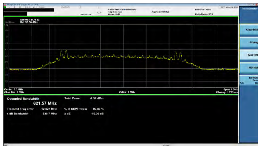
Plot 7-29. ISSED Occupied Bandwidth (Ch. 5, Config 4/Payload 0)
