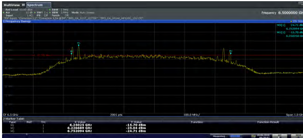
Plot 7-1. 10dBc Bandwidth (Ch. 5, Config 0/Payload 25)
