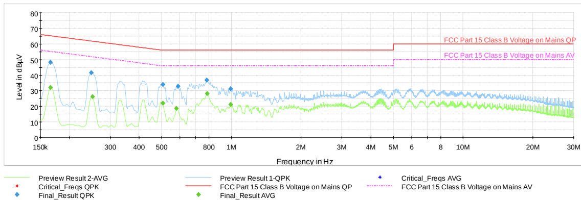
Plot 7-40. AC Line-Conducted Plot – GFSK ePA Ch.39 (N, with WCP + AC/DC Adapter)
