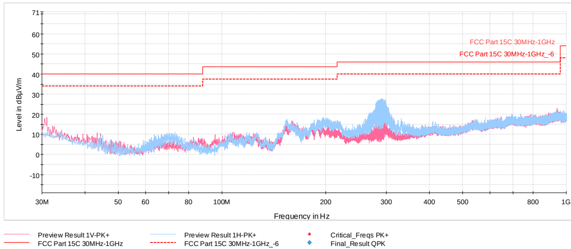
Plot 7-38. Radiated Spurious Emissions 30MHz-1GHz (GFSK ePA – Ch.39, with WCP + Laptop)
