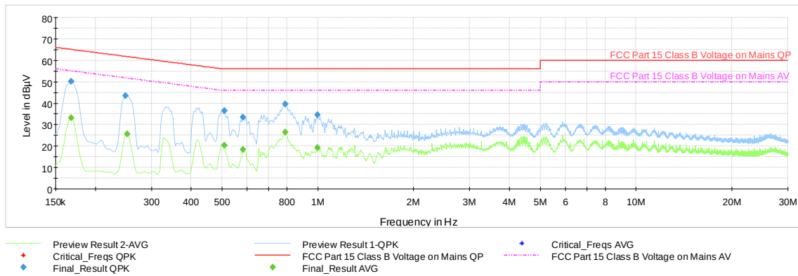
Plot 7-39. AC Line-Conducted Plot – GFSK ePA Ch.39 (L1, with WCP + AC/DC Adapter)
