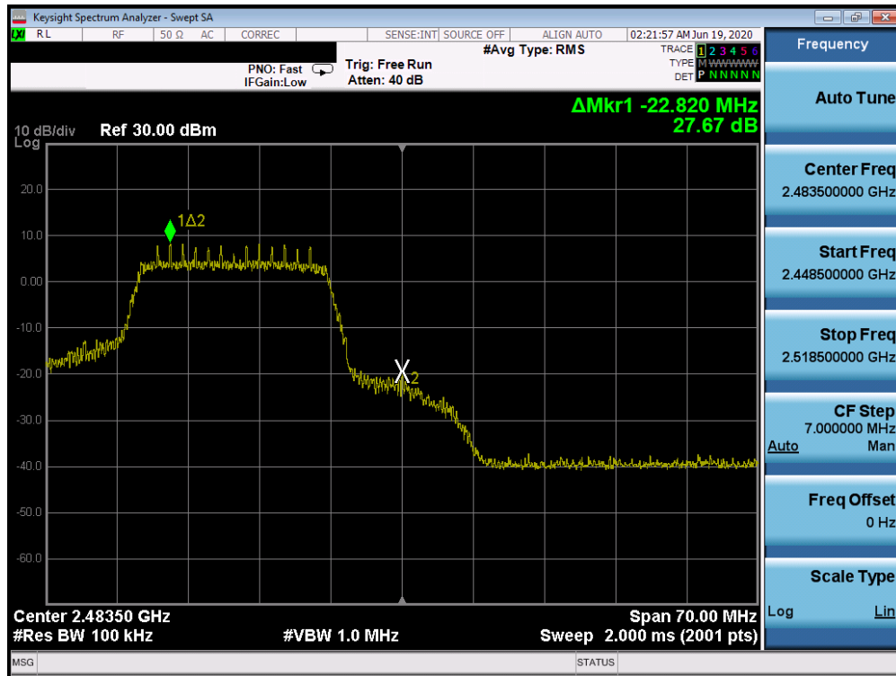
Plot 7-35. Band Edge Plot (802.11n (2.4GHz) – Ch. 12)
