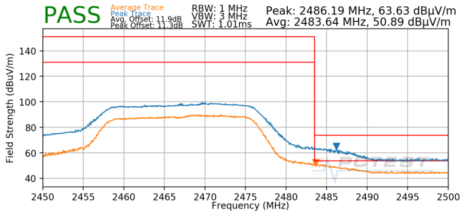
Plot 7-60. Radiated Restricted Upper Band Edge Measurement
