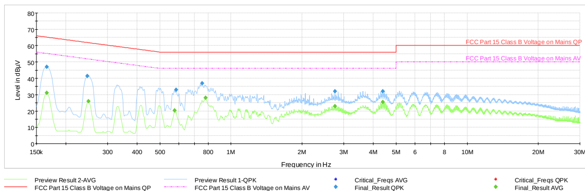
Plot 7-65. AC Line Conducted Plot with 802.11b Ch.6 (N, with WCP + AC/DC Adapter)
