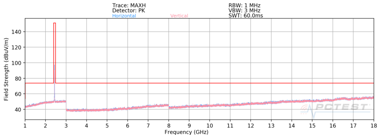
Plot 7-44. Radiated Spurious Emissions 1-18GHz (802.11b – Ch. 6)
