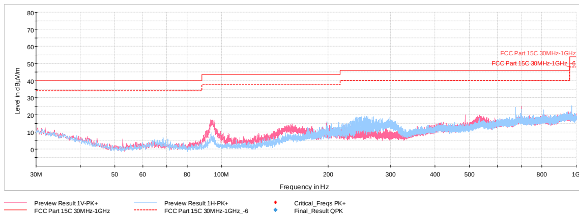
Plot 7-62. Radiated Spurious Emissions 30MHz-1GHz (802.11b – Ch.6, with WCP + Laptop)
