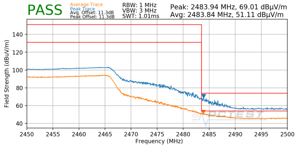
Plot 7-58. Radiated Restricted Upper Band Edge Measurement
