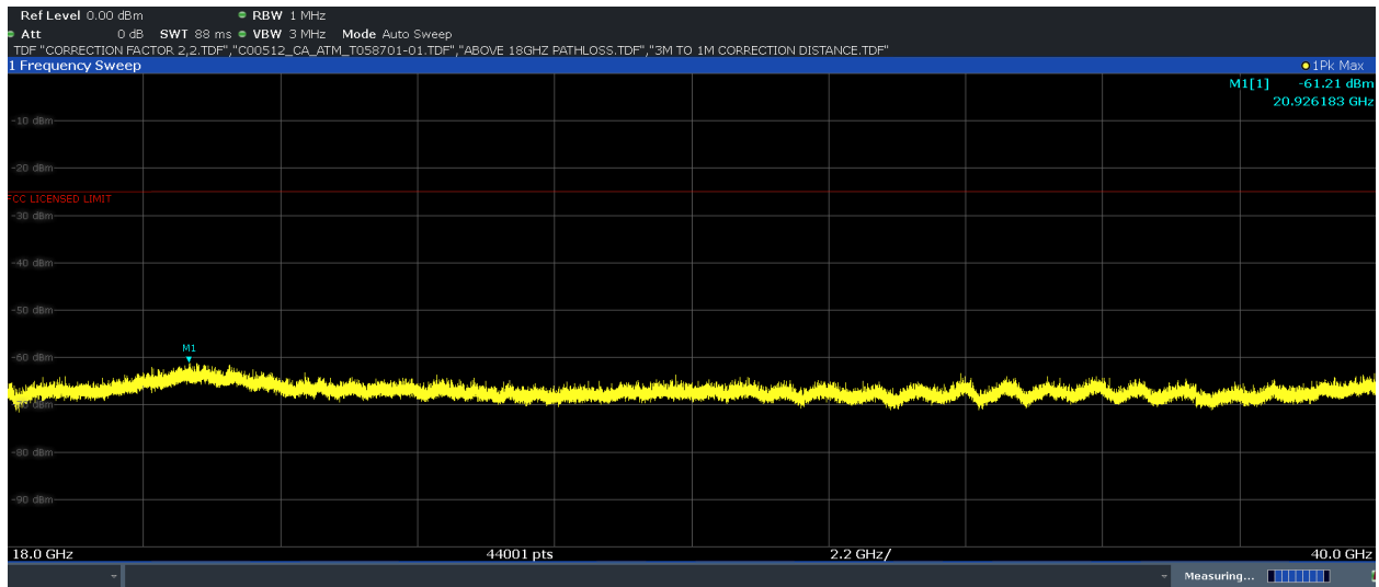
Plot 7-50. Radiated Spurious Emissions 18-40GHz (Simultaneous Transmission, Ant. Pol. V)
