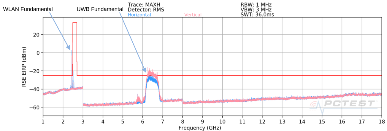
Plot 7-48. Radiated Spurious Emissions 1-18GHz (Simultaneous Transmission)
