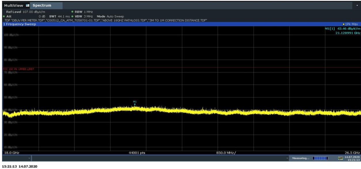
Plot 7-46. Radiated Spurious Emissions 18-26.5GHz (802.11b – Ch. 6, Ant. Pol. H)
