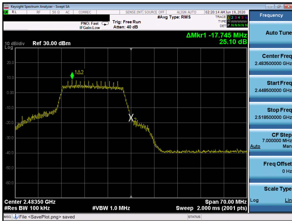
Plot 7-36. Band Edge Plot (802.11n (2.4GHz) – Ch. 13)
