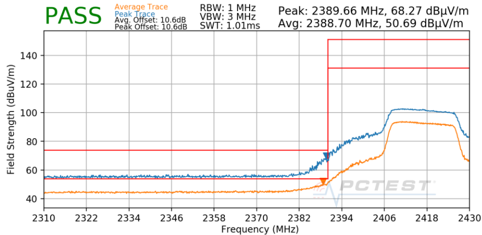
Plot 7-56. Radiated Restricted Lower Band Edge Measurement
