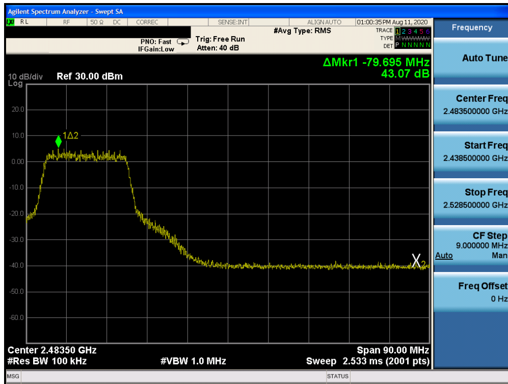
Plot 7-32. Band Edge Plot (802.11n (2.4GHz) – Ch. 9)
