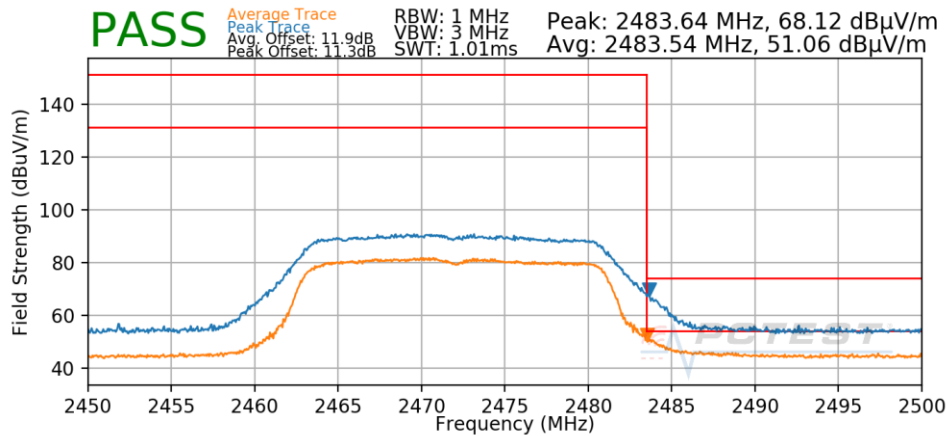
Plot 7-61. Radiated Restricted Upper Band Edge Measurement
