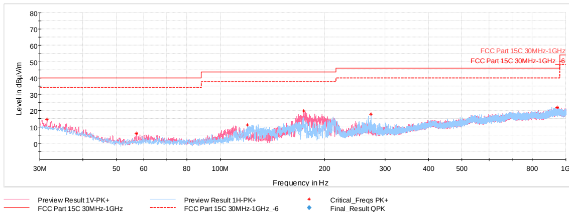
Plot 7-63. Radiated Spurious Emissions 30MHz-1GHz (Simultaneous Transmission, with WCP + AC/DC adapter)
