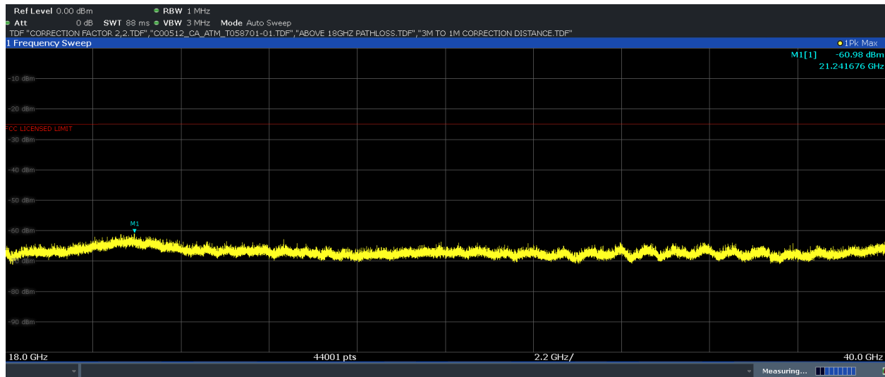
Plot 7-49. Radiated Spurious Emissions 18-40GHz (Simultaneous Transmission, Ant. Pol. H)
