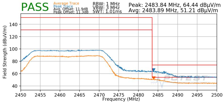
Plot 7-59. Radiated Restricted Upper Band Edge Measurement
