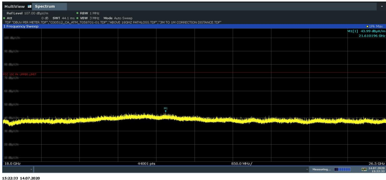
Plot 7-47. Radiated Spurious Emissions 18-26.5GHz (802.11b – Ch. 6, Ant. Pol. V)
