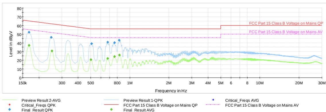
Plot 7-64. AC Line Conducted Plot with 802.11b Ch.6 (L1, with WCP + AC/DC Adapter)
