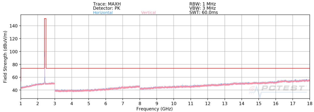
Plot 7-43. Radiated Spurious Emissions 1-18GHz (802.11b – Ch. 1)
