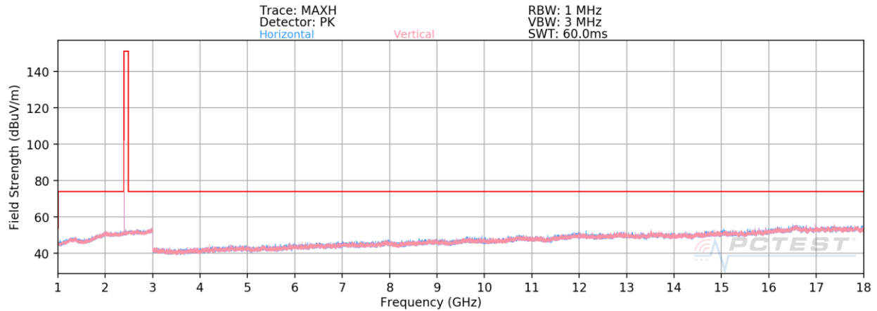
Plot 7-29. Radiated Spurious Emissions 1-18 (1Mbps, ePA – Ch. 0)
