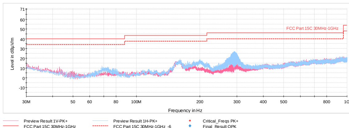
Plot 7-38. Radiated Spurious Emissions 30M Hz-1GHz (1Mbps, ePA – Ch.0, with WCP + Laptop)
