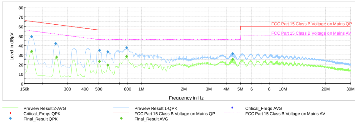
Plot 7-40. AC Line Conducted Plot with Bluetooth LE (1Mbps, ePA – Ch.19, N, with WCP + AC/DC Adapter)
