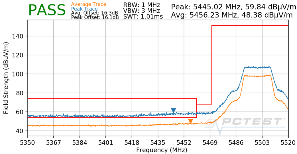
Plot 7-41. Radiated Lower Band Edge Plot (UNII Band 2C)
