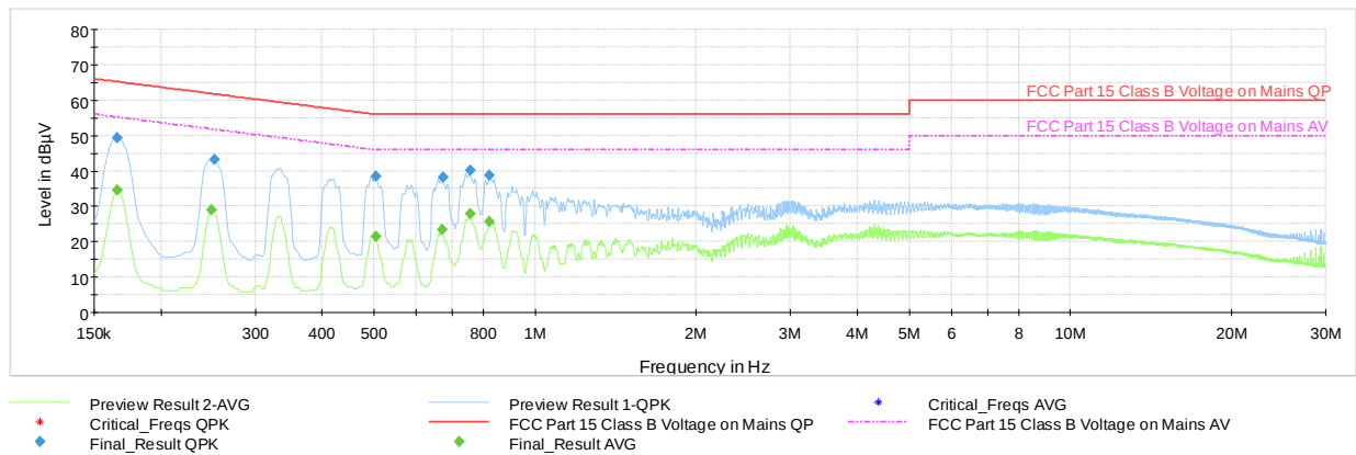
Plot 7-48. AC Line Conducted Plot with 802.11n UNII Band 1 – Ch.36 (N) with WCP + AC/DC Adapter
