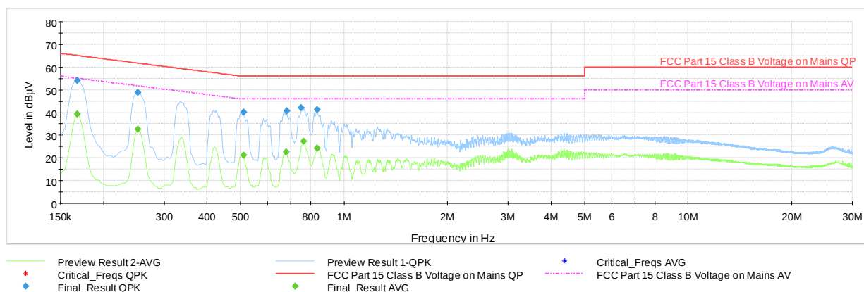
Plot 7-47. AC Line Conducted Plot with 802.11n UNII Band 1 – Ch.36 (L1) with WCP + AC/DC Adapter
