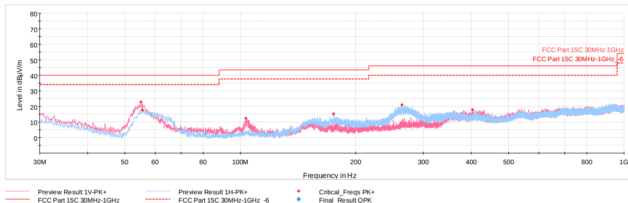
Plot 7-46. Radiated Spurious Emissions below 1GHz (802.11n – U1 Ch. 36) with WCP + Laptop
