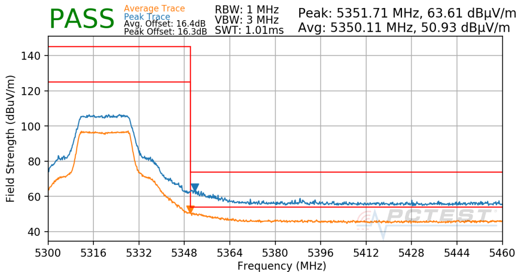
Plot 7-40. Radiated Upper Band Edge Plot (UNII Band 2A)
