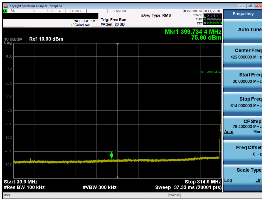
Plot 7-12. Conducted Spurious Plot (LTE Band 26 - 5MHz QPSK - RB Size 1, RB Offset 0 - High Channel)
