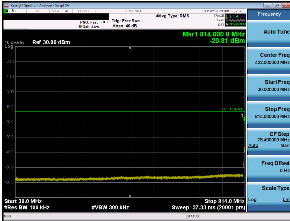
Plot 7-9. Conducted Spurious Plot (LTE Band 26 - 5MHz QPSK - RB Size 1, RB Offset 0 - Low Channel)
