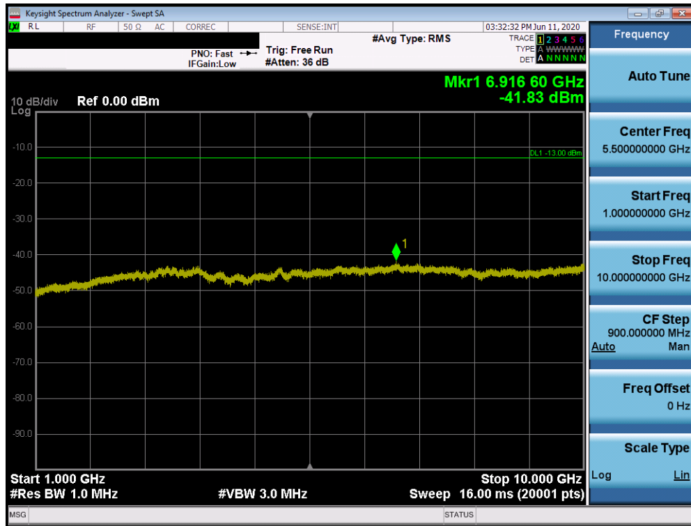
Plot 7-11. Conducted Spurious Plot (LTE Band 26 - 5MHz QPSK - RB Size 1, RB Offset 0 - Low Channel)
