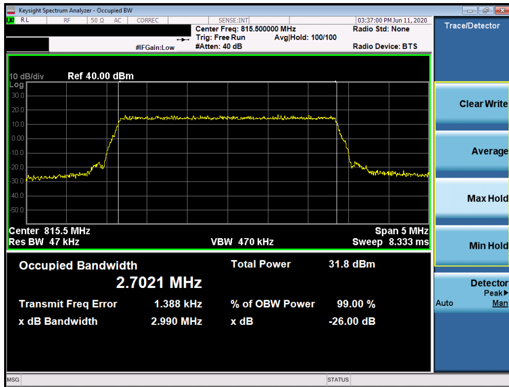
Plot 7-6. Occupied Bandwidth Plot (LTE Band 26 - 3MHz 16-QAM - Full RB Configuration)
