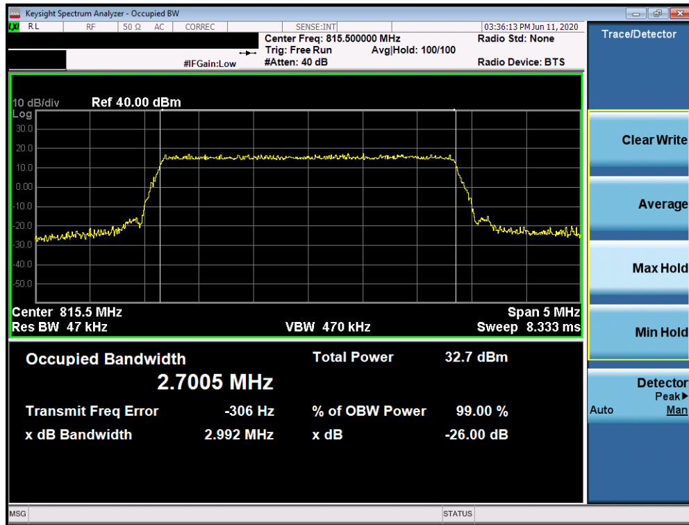
Plot 7-5. Occupied Bandwidth Plot (LTE Band 26 - 3MHz QPSK - Full RB Configuration)
