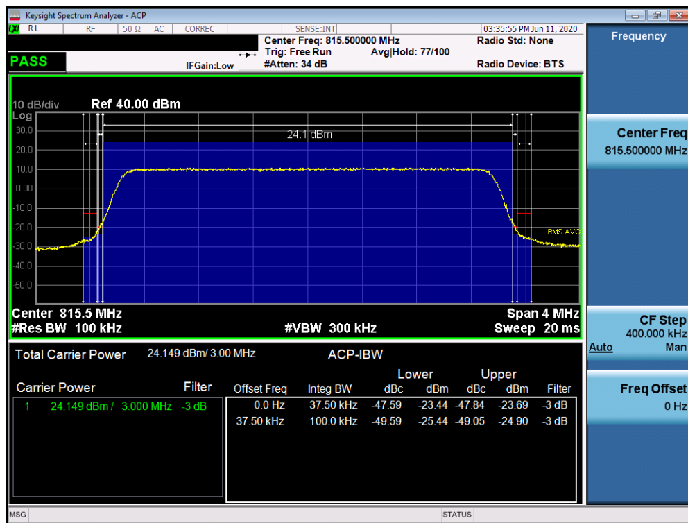
Plot 7-18. Channel Edge Plot (LTE Band 26 - 3MHz QPSK - Low Channel)
