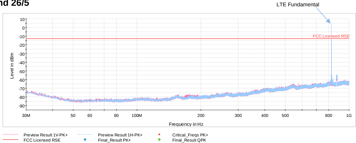
Plot 7-262. Radiated Spurious Emissions below 1GHz (Band 26/5)
