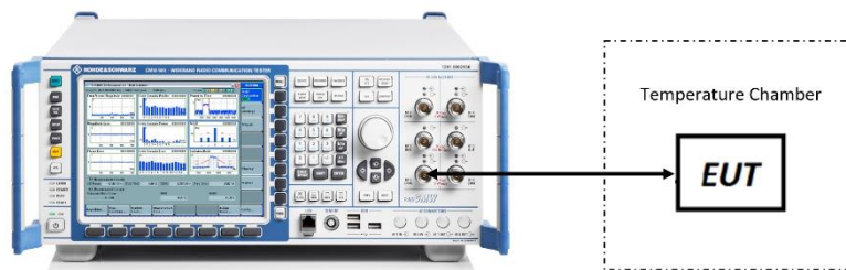
Figure 7-8. Test Instrument & Measurement Setup
