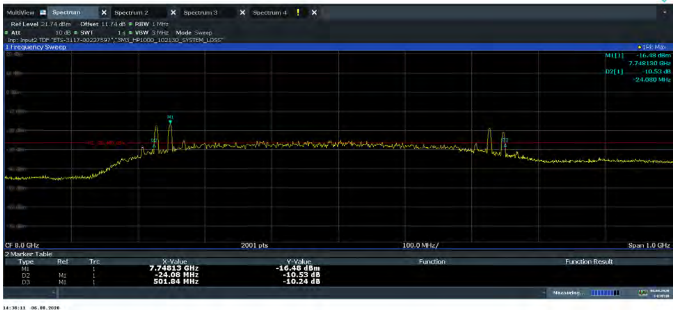
Plot 7-13. 10dBc Bandwidth (Ch. 9, Config 0/Payload 65)
