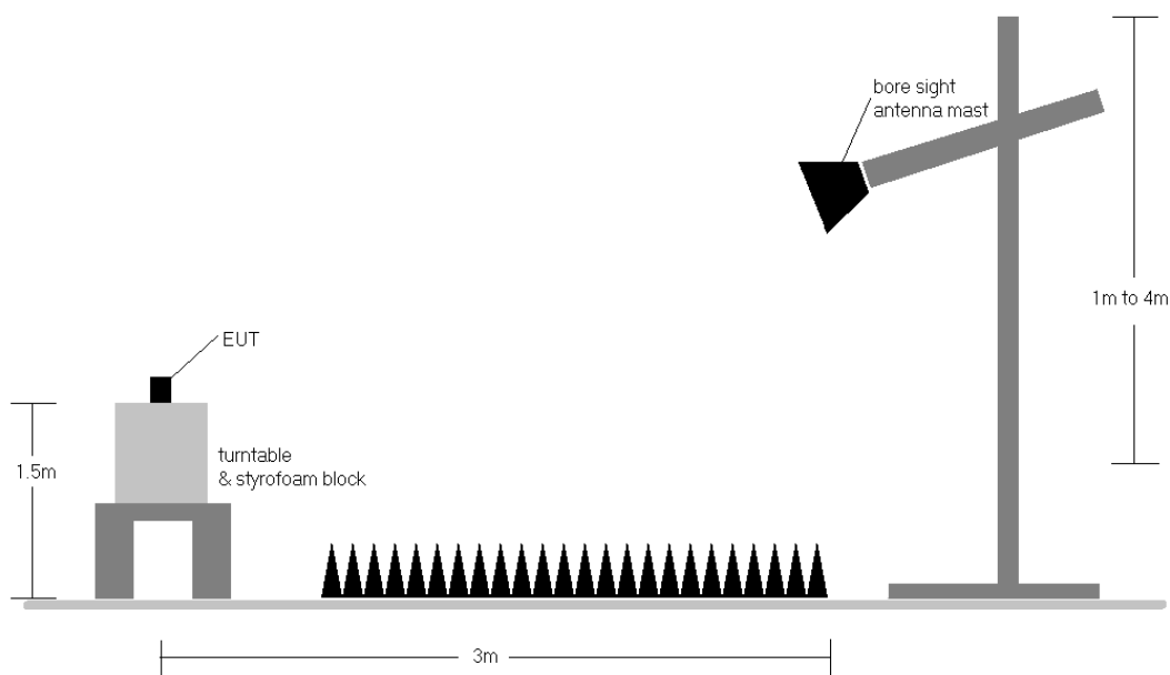
Figure 7-1. Test Setup
