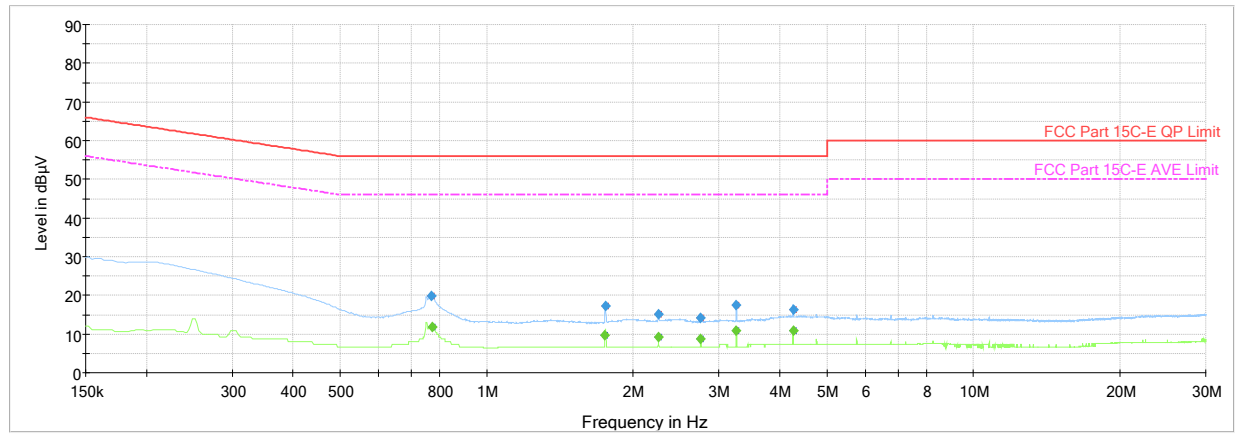
Plot 7-109. AC Line Conducted (Ch. 9, Config 0, Payload 125 L1, with AC/DC Adapter)
