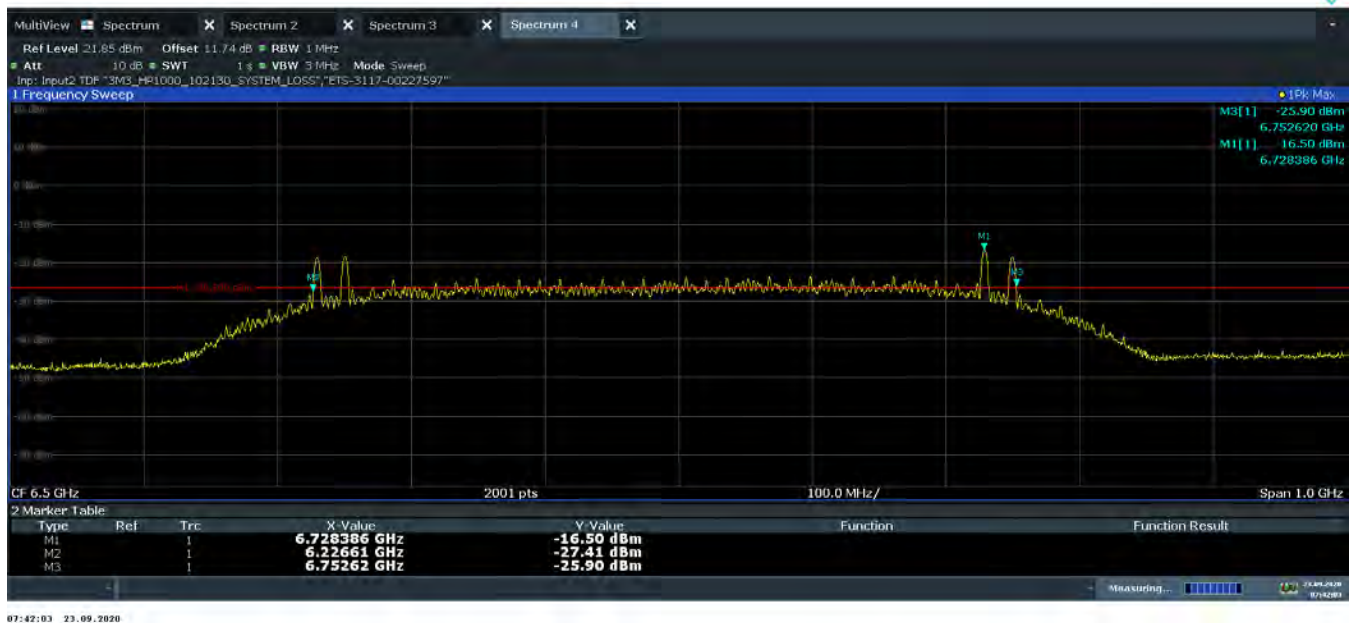
Plot 7-9. 10dBc Bandwidth (Ch. 5, Config 4/Payload 0)
