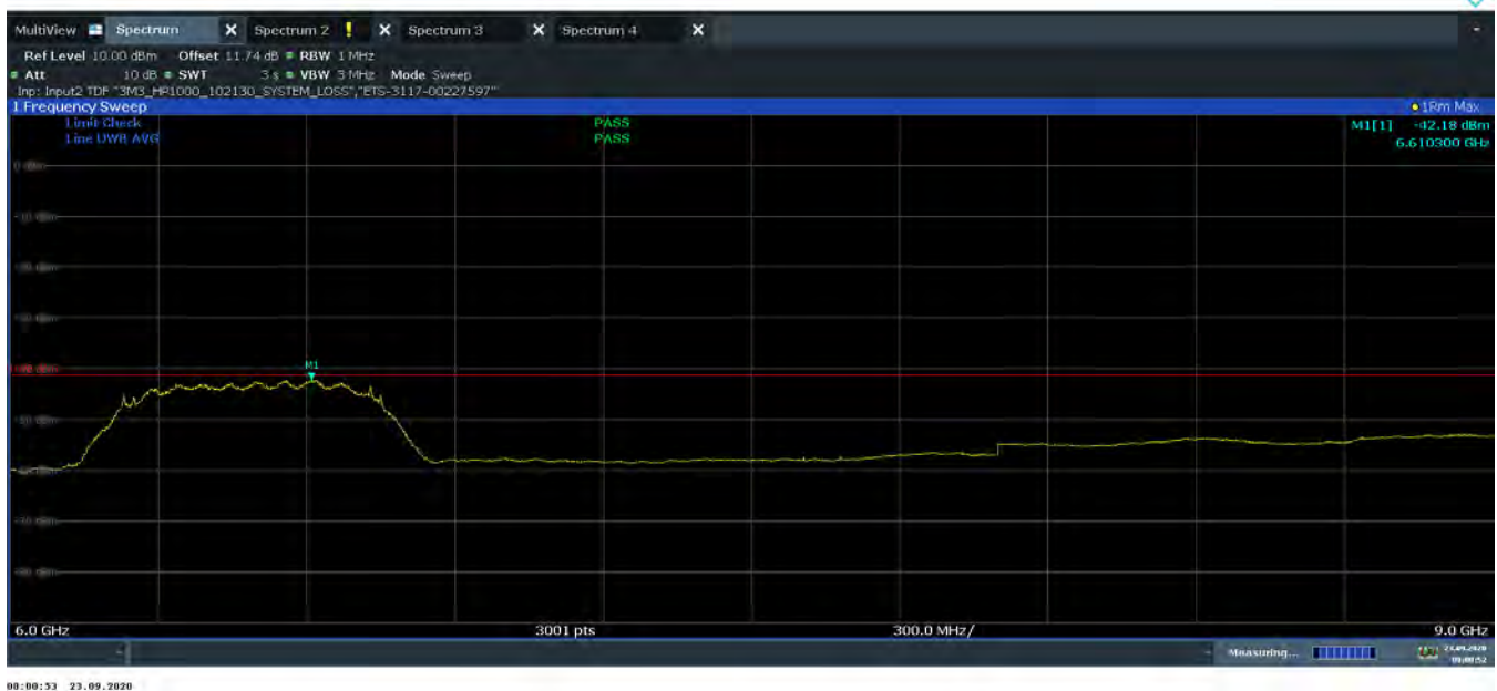
Plot 7-70. Average Radiated Power (Ch. 5, Config 5/Payload 0)
