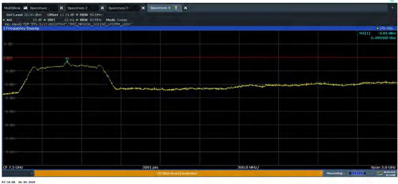
Plot 7-44. Peak Radiated Power (Ch. 5, Config 0/Payload 125)
