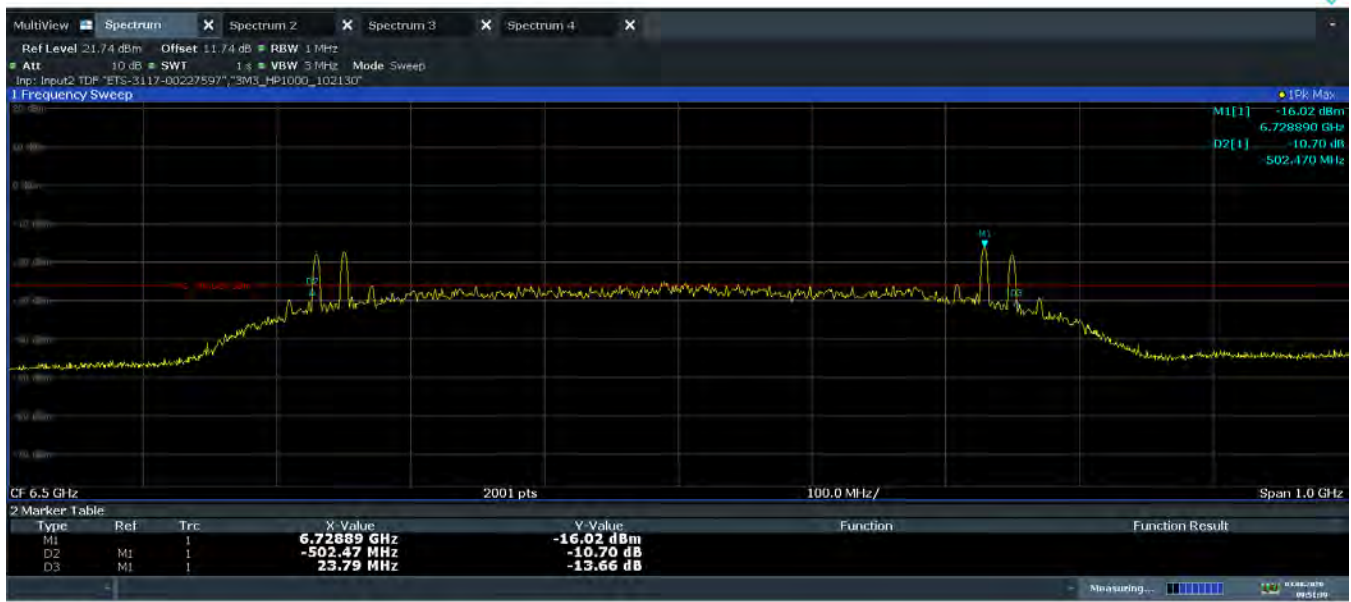
Plot 7-3. 10dBc Bandwidth (Ch. 5, Config 0/Payload 65)
