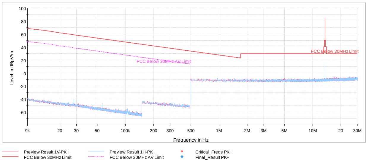
Plot 7-8. Radiated Spurious Emissions 9kHz – 30MHz (CE B 848kbps, with WCP + AC/DC Adapter)
