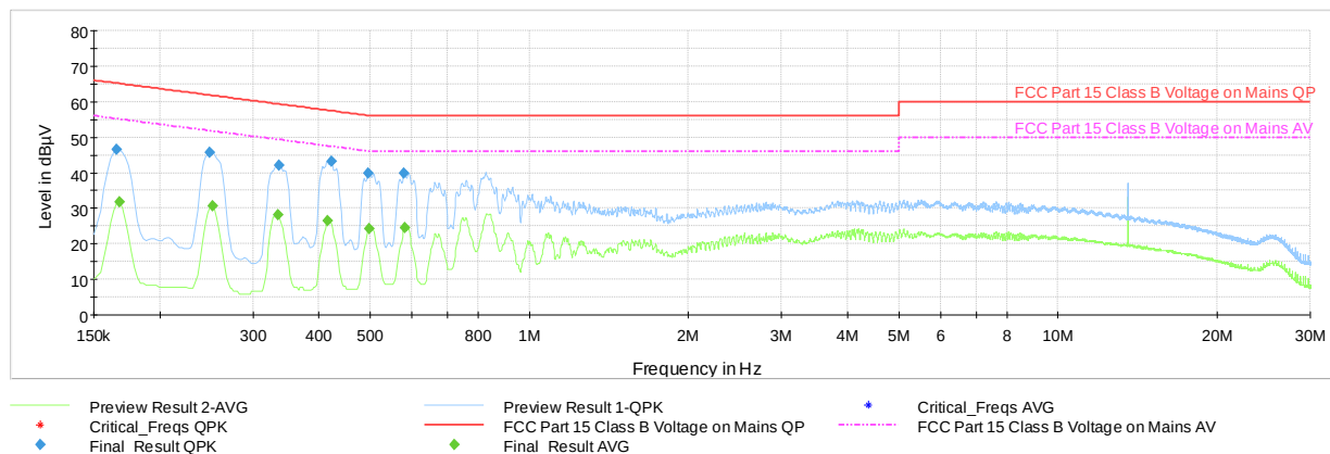
Plot 7-12. AC Line-Conducted Test Plot (L1, CE B 848kbps, with WCP + AC/DC Adapter)
