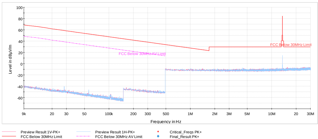
Plot 7-9. Radiated Spurious Emissions 9kHz – 30MHz (Reader 10% Ask 1 out of 4, with WCP + AC/DC Adapter)
