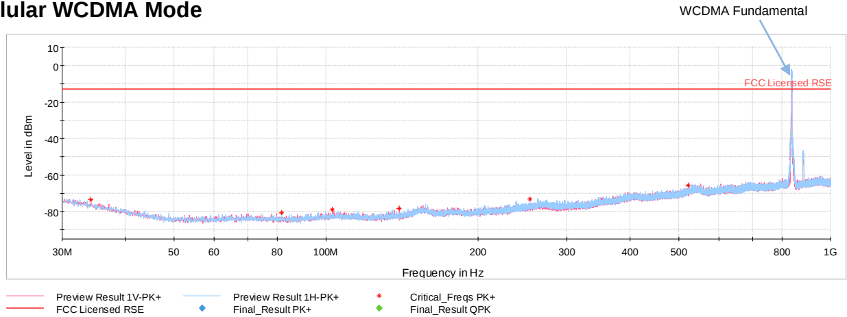
Plot 7-44. Radiated Spurious Emissions below 1GHz (Cellular WCDMA Mode – Ch. 4233)
