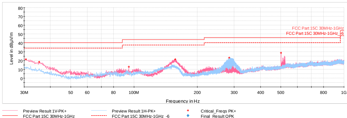
Plot 7-38. Radiated Spurious Emissions 30MHz-1GHz (4Mbps, ePA – Ch.38, with WCP + AC/DC adapter)
