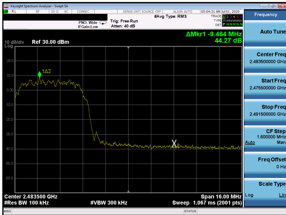
Plot 7-22. Band Edge Plot (Bluetooth (HDR8), ePA – Ch. 75)
