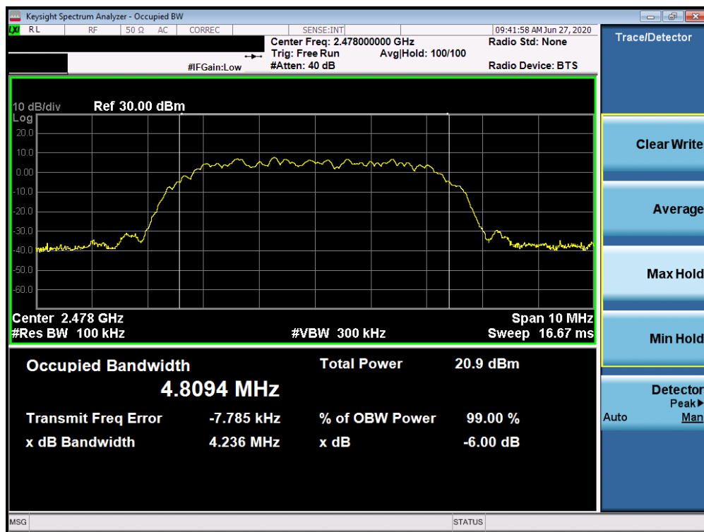
Plot 7-6. 6dB Bandwidth Plot (Bluetooth (HDR8), 8Mbps, ePA – Ch. 75)
