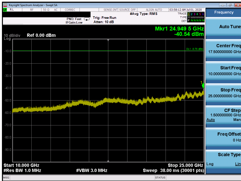
Plot 7-28. Conducted Spurious Plot (Bluetooth (HDR4), 4 Mbps, ePA – Ch. 75)
