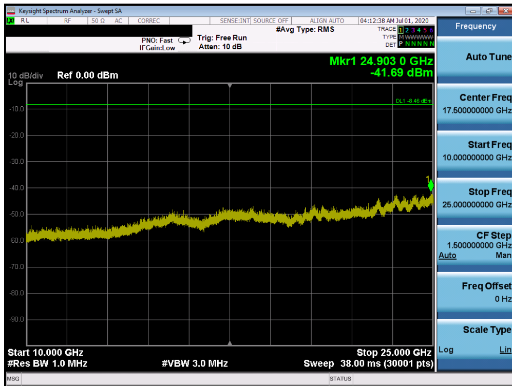
Plot 7-26. Conducted Spurious Plot (Bluetooth (HDR4), 4 Mbps, ePA – Ch. 38)
