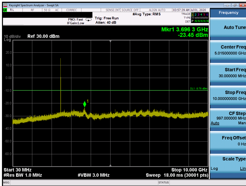
Plot 7-27. Conducted Spurious Plot (Bluetooth (HDR4), 4 Mbps, ePA – Ch. 75)
