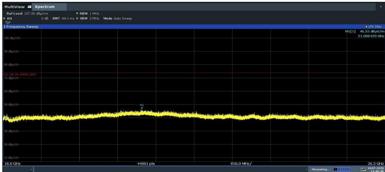
Plot 7-33. Radiated Spurious Emissions 18-26.5GHz (4Mbps, ePA – Ch.38, Ant. Pol. V)
