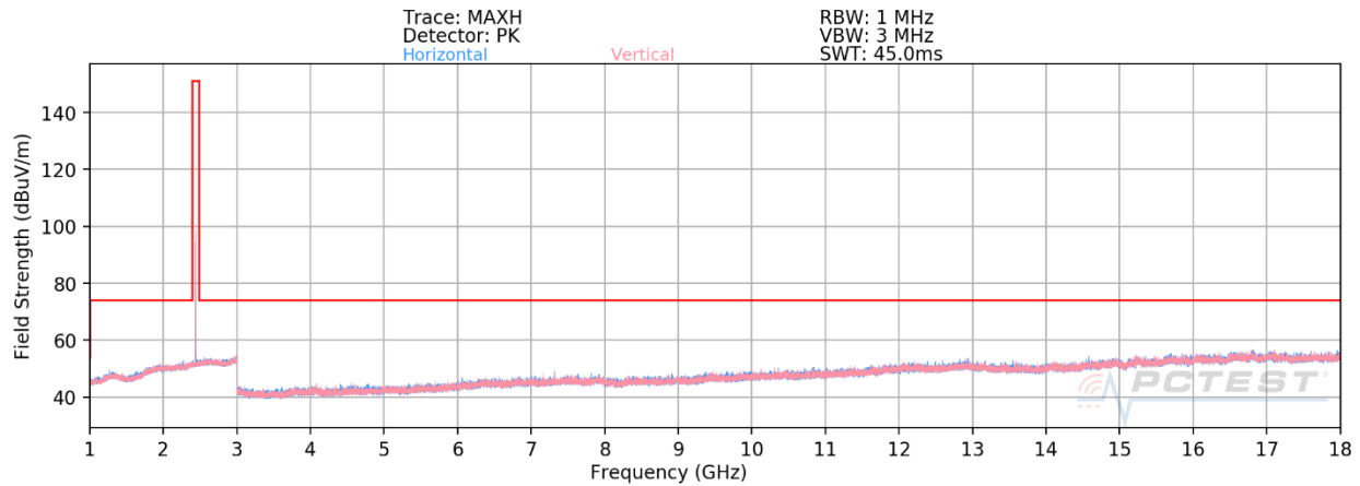
Plot 7-30. Radiated Spurious Emissions 1-18GHz (4Mbps, ePA – Ch. 38)
