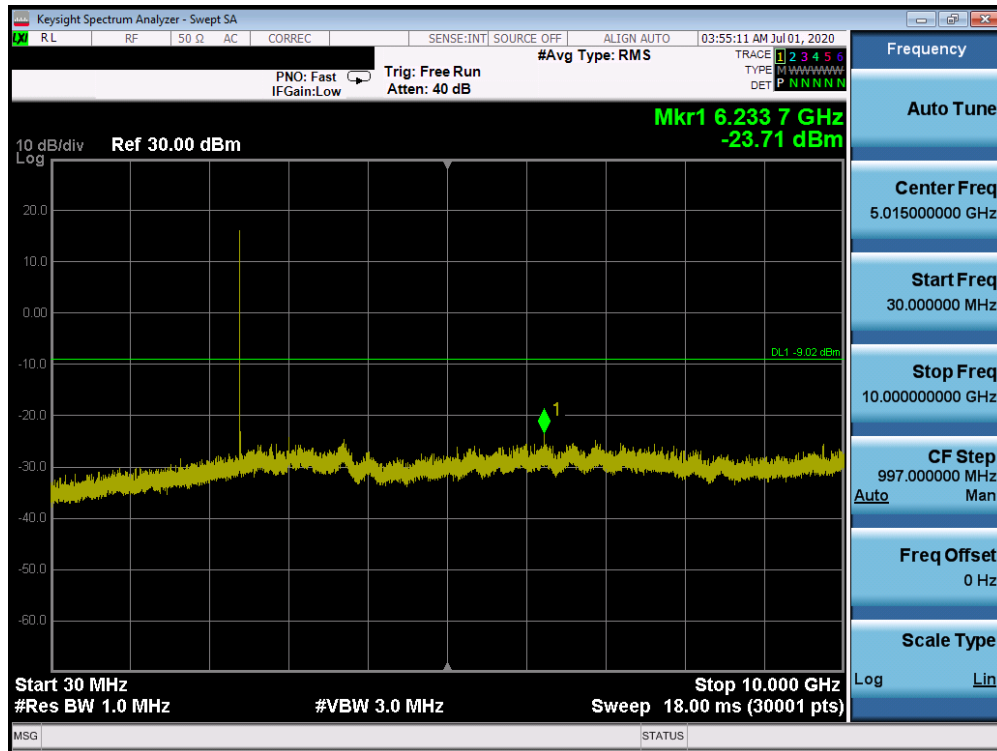
Plot 7-23. Conducted Spurious Plot (Bluetooth (HDR4), 4 Mbps, ePA – Ch. 1)
