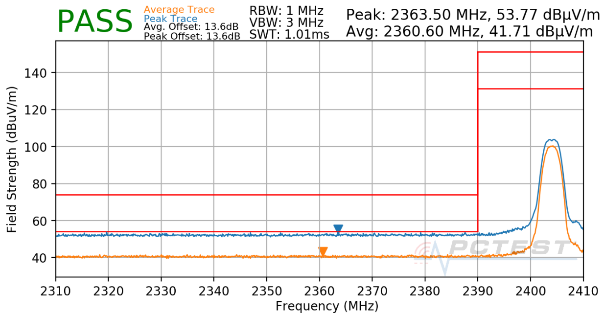
Plot 7-34. Radiated Restricted Lower Band Edge Measurement
