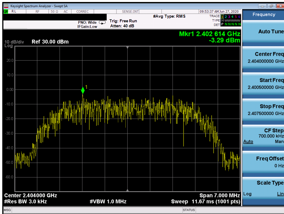
Plot 7-13. Power Spectral Density Plot (Bluetooth (HDR8), 8Mbps, ePA – Ch. 1)
