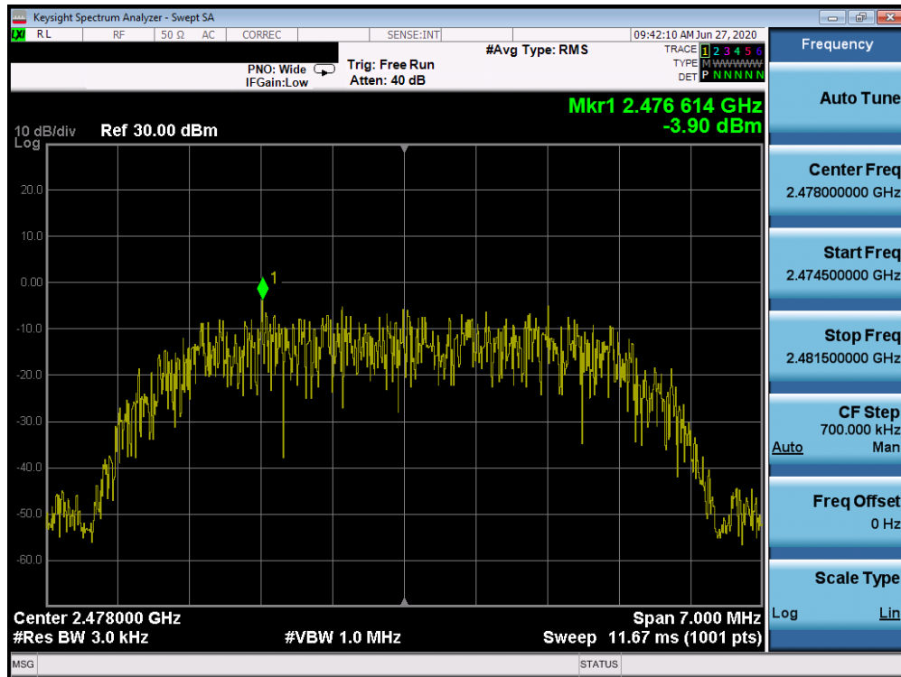
Plot 7-15. Power Spectral Density Plot (Bluetooth (HDR8), 8Mbps, ePA – Ch. 75)
