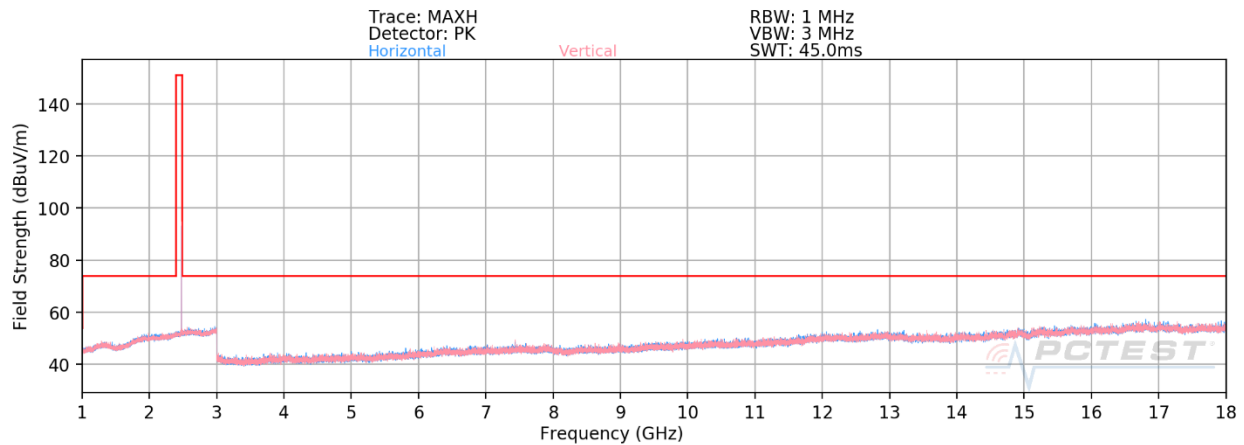
Plot 7-31. Radiated Spurious Emissions 1-18GHz (4Mbps, ePA – Ch. 75)
