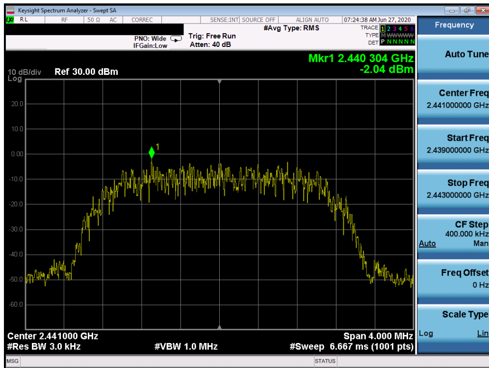
Plot 7-8. Power Spectral Density Plot (Bluetooth (HDR4), 4Mbps, ePA – Ch. 38)
