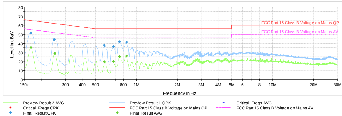
Plot 7-39. AC Line Conducted Emission with Bluetooth HDR (L1 – 4Mbps, ePA, Ch.38, with WCP + AC/DC Adapter)
