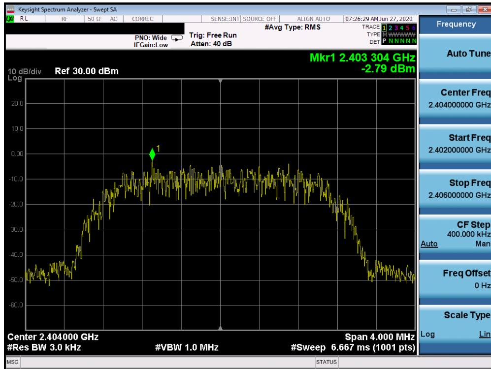
Plot 7-7. Power Spectral Density Plot (Bluetooth (HDR4), 4Mbps, ePA – Ch. 1)
