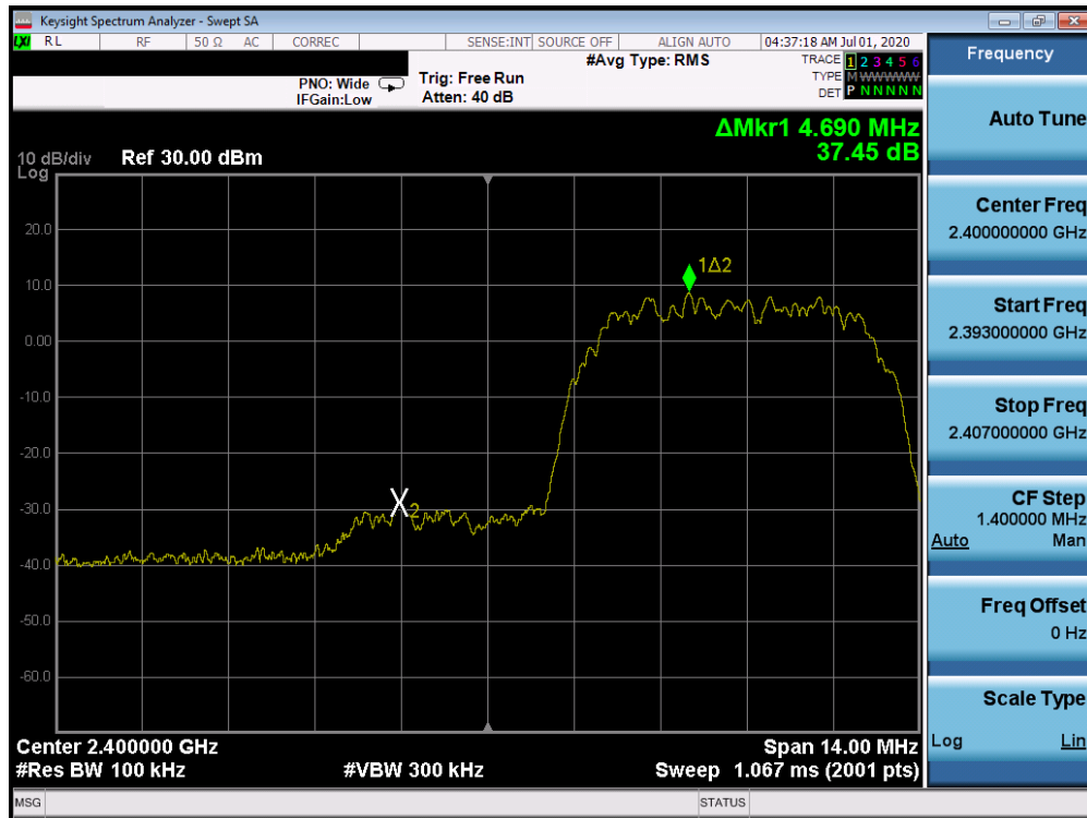
Plot 7-21. Band Edge Plot (Bluetooth (HDR8), ePA – Ch. 1)
