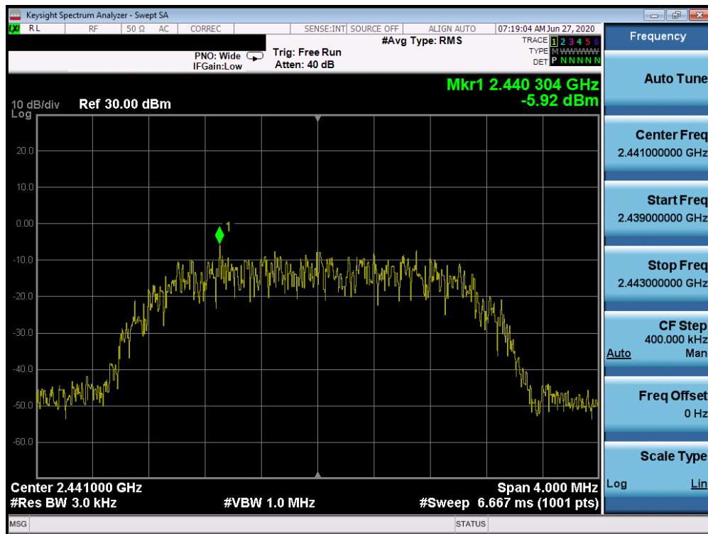
Plot 7-11. Power Spectral Density Plot (Bluetooth (HDR4), 4Mbps, iPA – Ch. 38)
