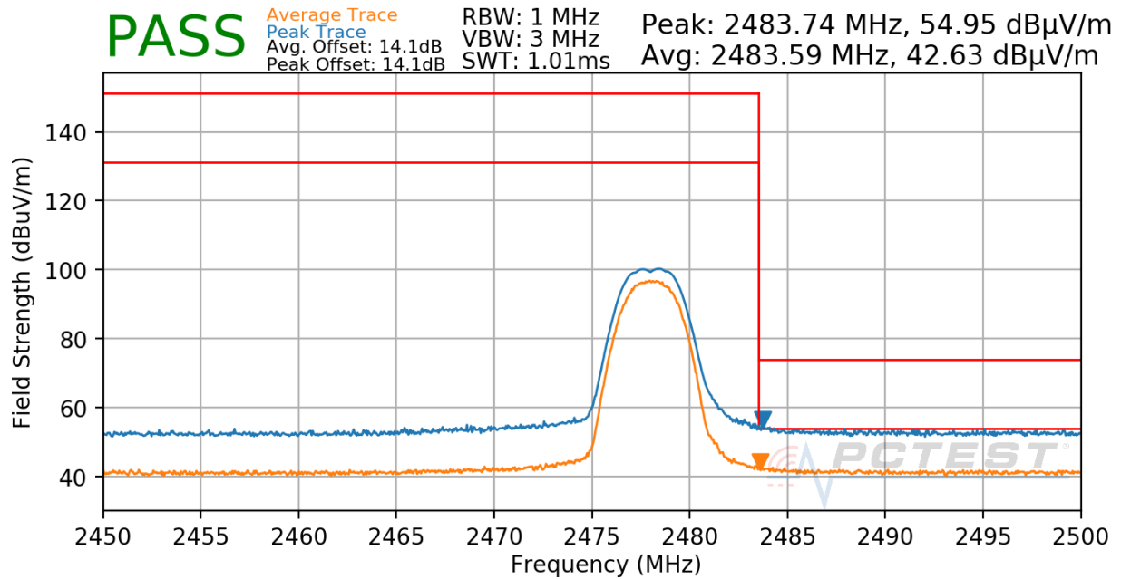
Plot 7-36. Radiated Restricted Upper Band Edge Measurement
