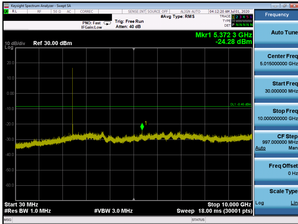
Plot 7-25. Conducted Spurious Plot (Bluetooth (HDR4), 4 Mbps, ePA – Ch. 38)
