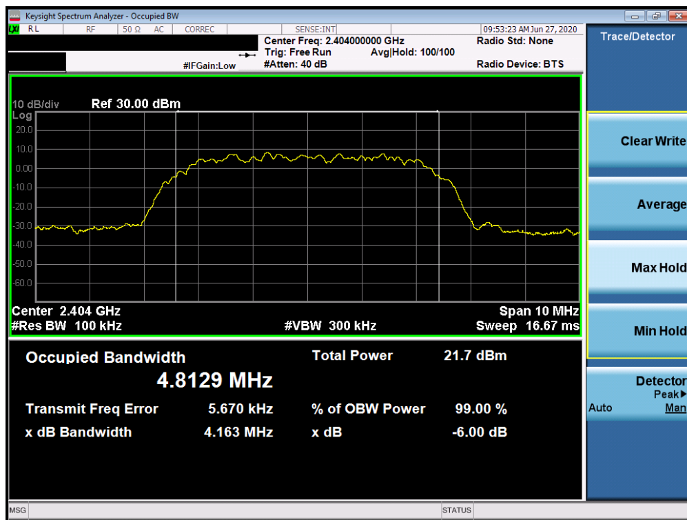
Plot 7-4. 6dB Bandwidth Plot (Bluetooth (HDR8), 8Mbps, ePA – Ch. 1)
