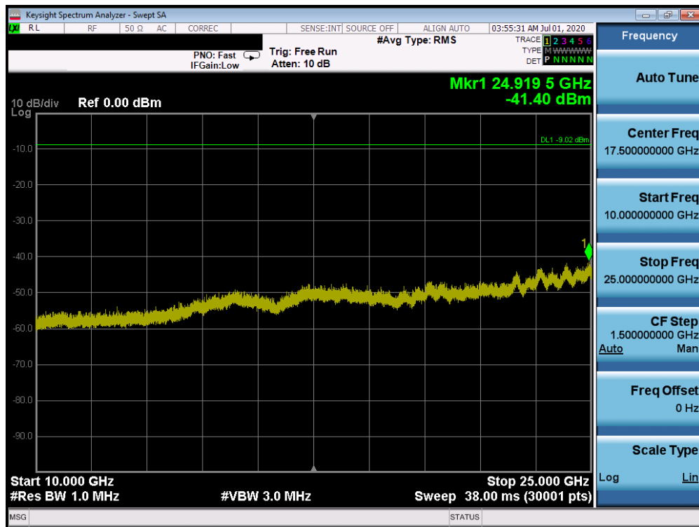
Plot 7-24. Conducted Spurious Plot (Bluetooth (HDR4), 4 Mbps, ePA – Ch. 1)
