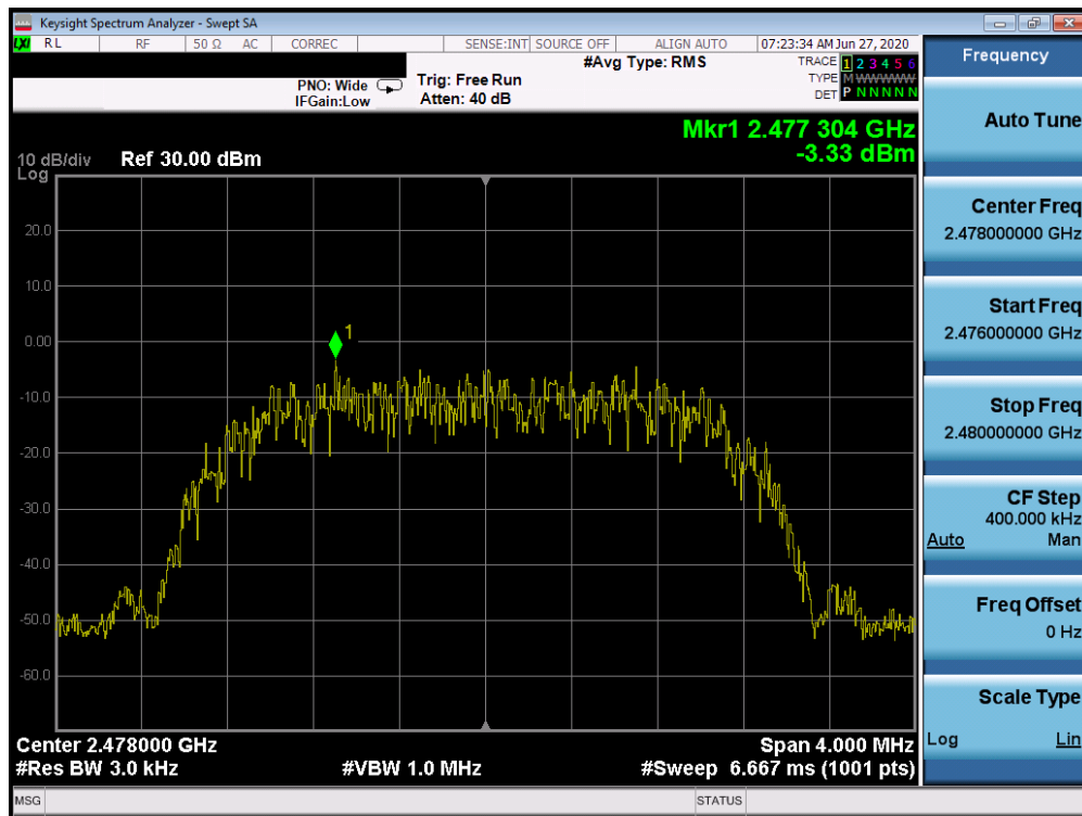
Plot 7-9. Power Spectral Density Plot (Bluetooth (HDR4), 4Mbps, ePA – Ch. 75)
