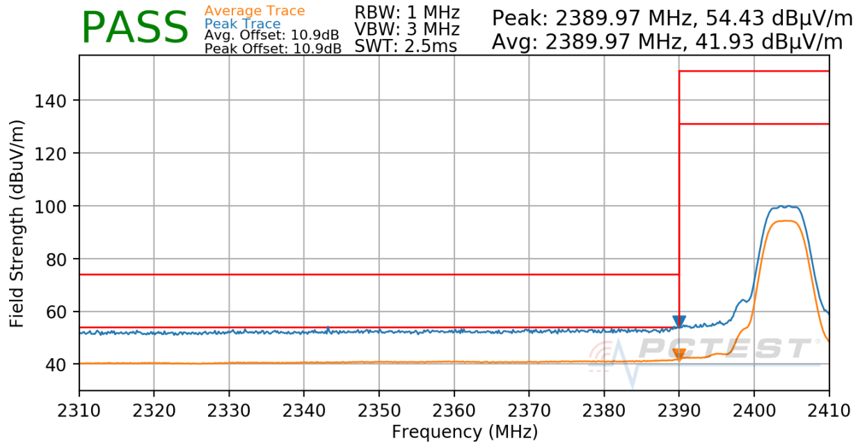
Plot 7-35. Radiated Restricted Lower Band Edge Measurement
