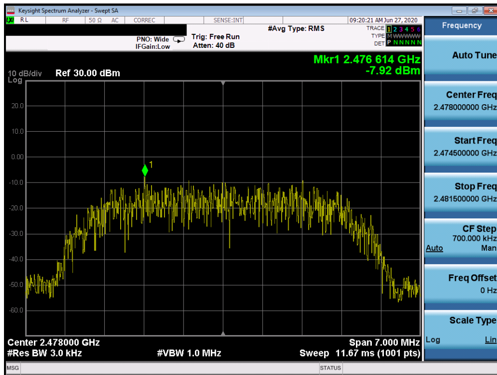
Plot 7-18. Power Spectral Density Plot (Bluetooth (HDR8), 8Mbps, iPA – Ch. 75)
