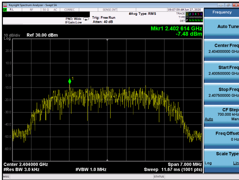
Plot 7-16. Power Spectral Density Plot (Bluetooth (HDR8), 8Mbps, iPA – Ch. 1)
