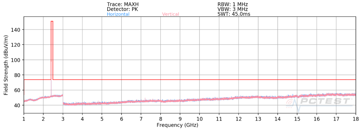
Plot 7-29. Radiated Spurious Emissions 1-18GHz (4Mbps, ePA – Ch. 1)
