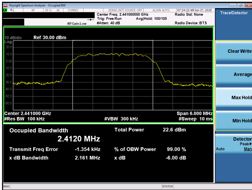
Plot 7-2. 6dB Bandwidth Plot (Bluetooth (HDR4), 4Mbps, ePA – Ch. 38)
