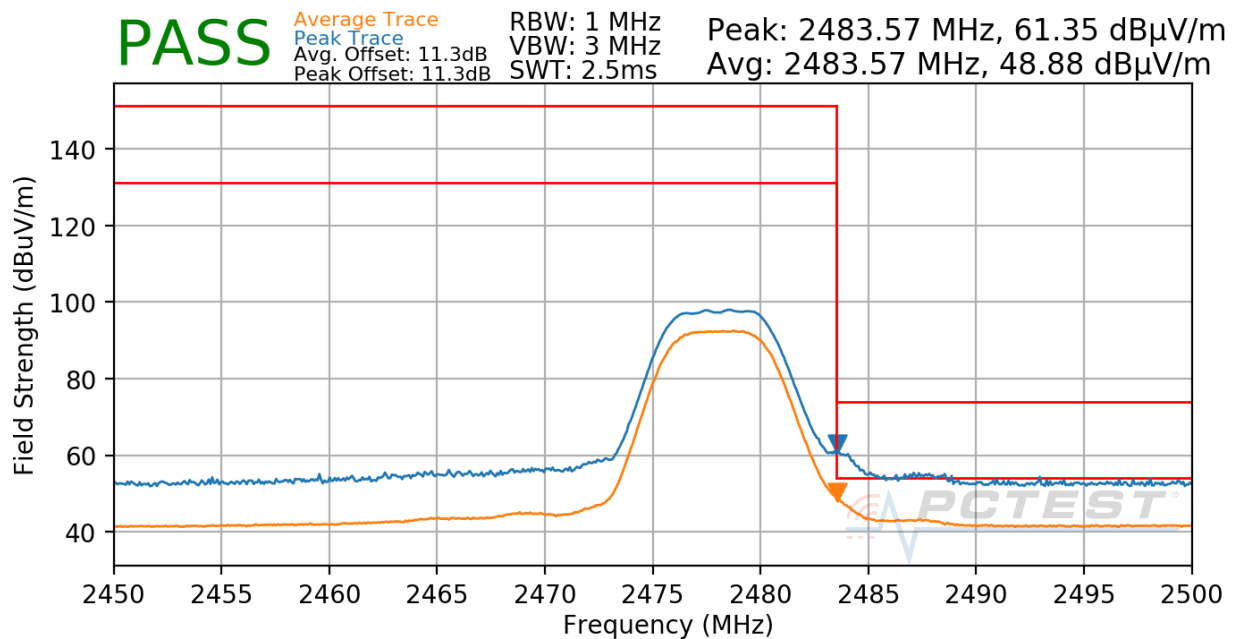
Plot 7-37. Radiated Restricted Upper Band Edge Measurement
