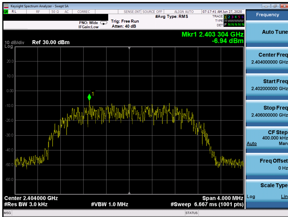
Plot 7-10. Power Spectral Density Plot (Bluetooth (HDR4), 4Mbps, iPA – Ch. 1)
