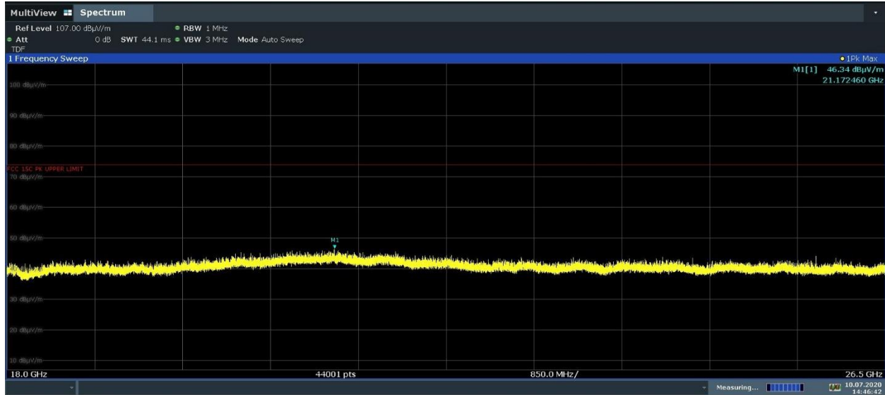
Plot 7-32. Radiated Spurious Emissions 18-26.5GHz (4Mbps, ePA – Ch.38, Ant. Pol. H)
