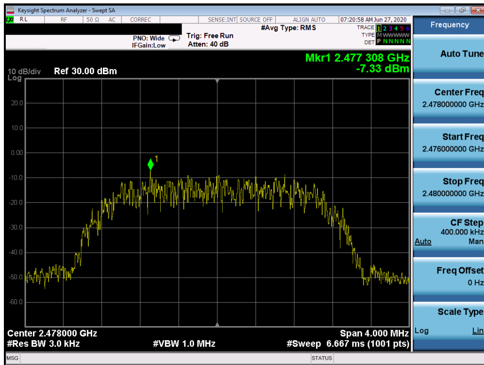
Plot 7-12. Power Spectral Density Plot (Bluetooth (HDR4), 4Mbps, iPA – Ch. 75)
