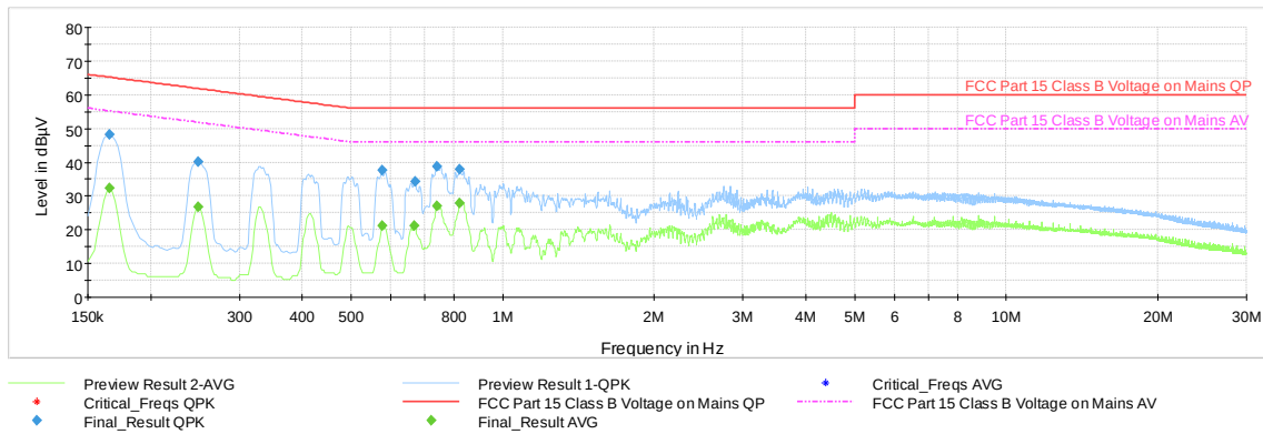
Plot 7-40. AC Line Conducted Emission with Bluetooth HDR (N – 4Mbps, ePA, Ch.38, with WCP + AC/DC Adapter)
