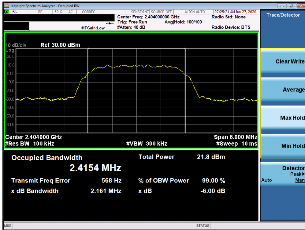
Plot 7-1. 6dB Bandwidth Plot (Bluetooth (HDR4), 4Mbps, ePA – Ch. 1)
