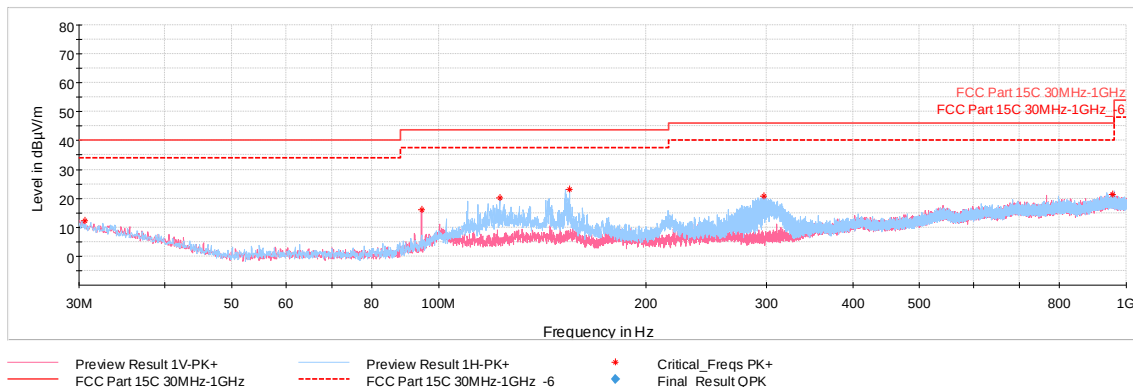
Plot 7-41. Radiated Spurious Emissions 30MHz-1GHz (GFSK ePA – Ch.39, with WCP + Laptop)
