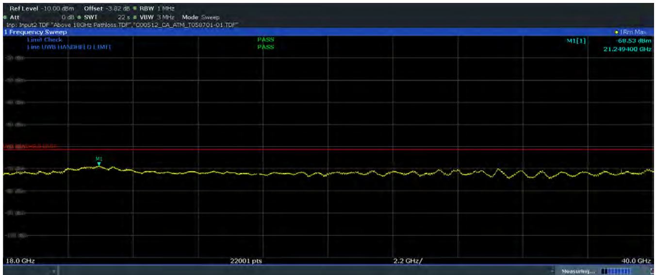
Plot 7-108. Radiated Spurious Emission 18-40GHz (Ch. 5, Config 3, Payload 125 Ant. Pol. V)
