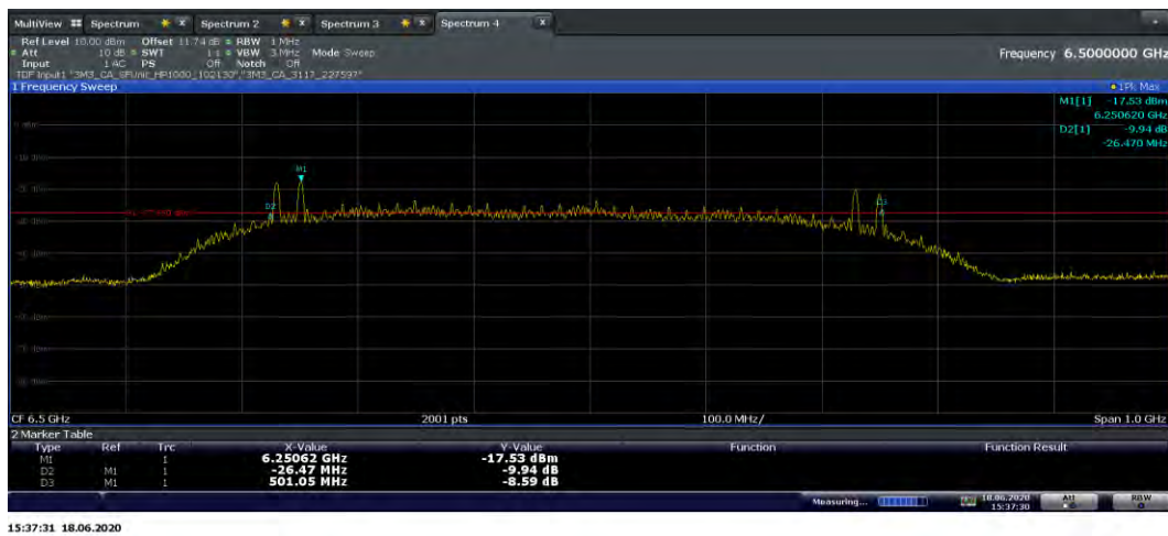
Plot 7-9. 10dBc Bandwidth (Ch. 5, Config 4/Payload 0)
