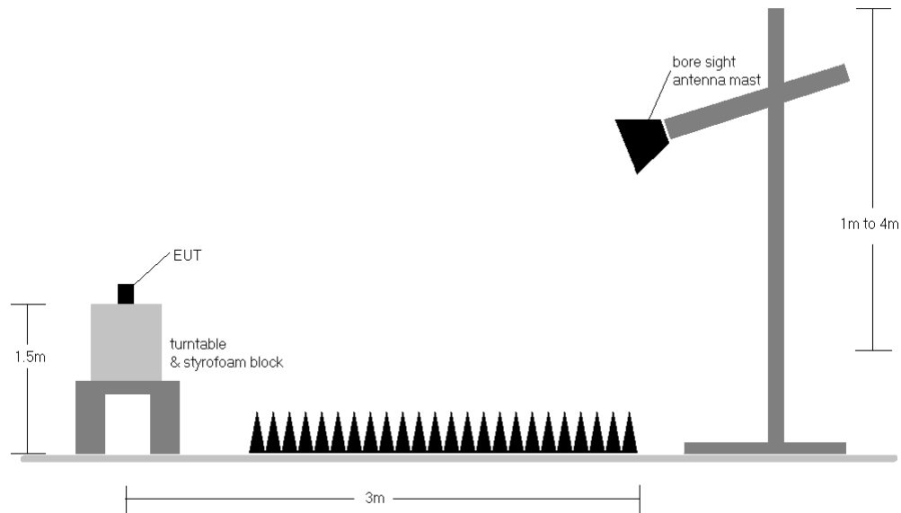
Figure 7-3. Test Setup
