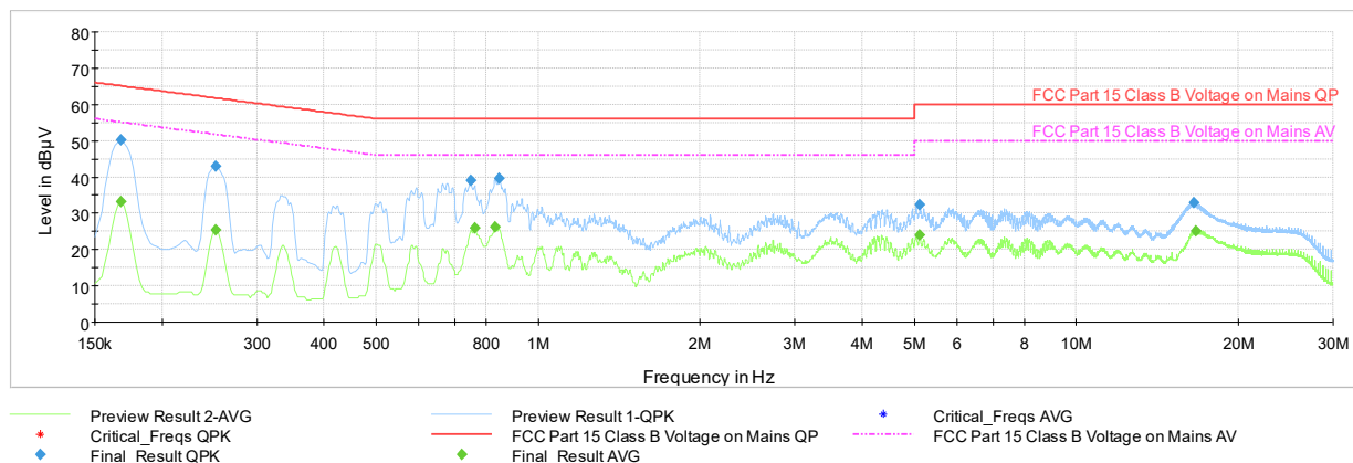
Plot 7-114. AC Line Conducted (Ch. 5, Config 3, Payload 125 N, with AC/DC Adapter)
