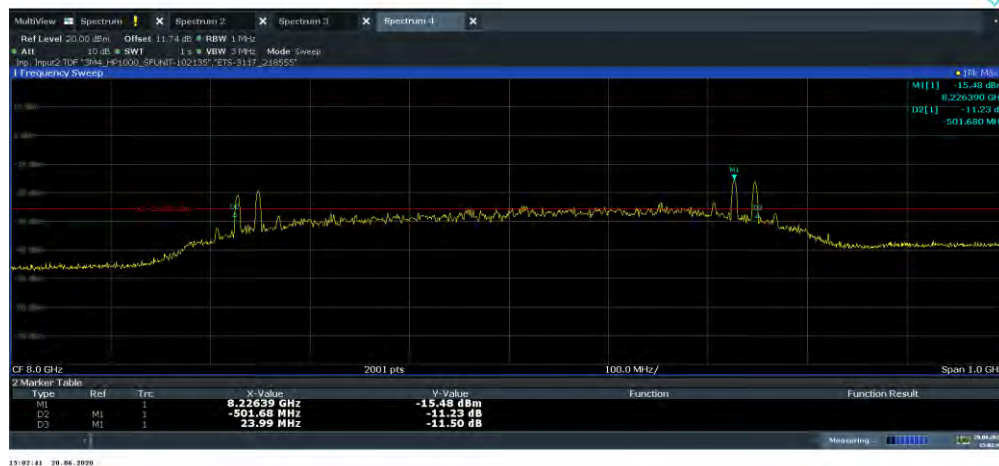
Plot 7-11. 10dBc Bandwidth (Ch. 9, Config 0/Payload 25)
