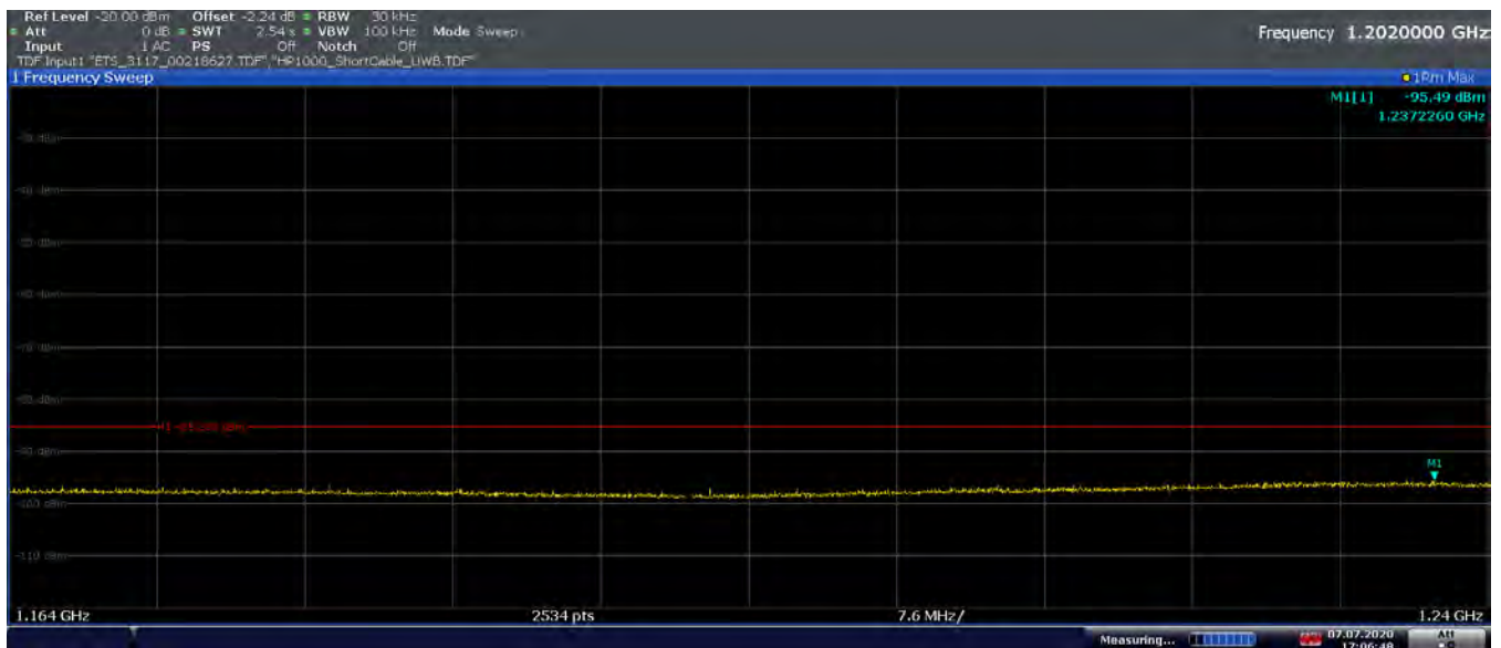
Plot 7-101. Radiated Spurious Emission 1164-1240MHz (Ch. 9, Config 3, Payload 125 Ant. Pol. H)
