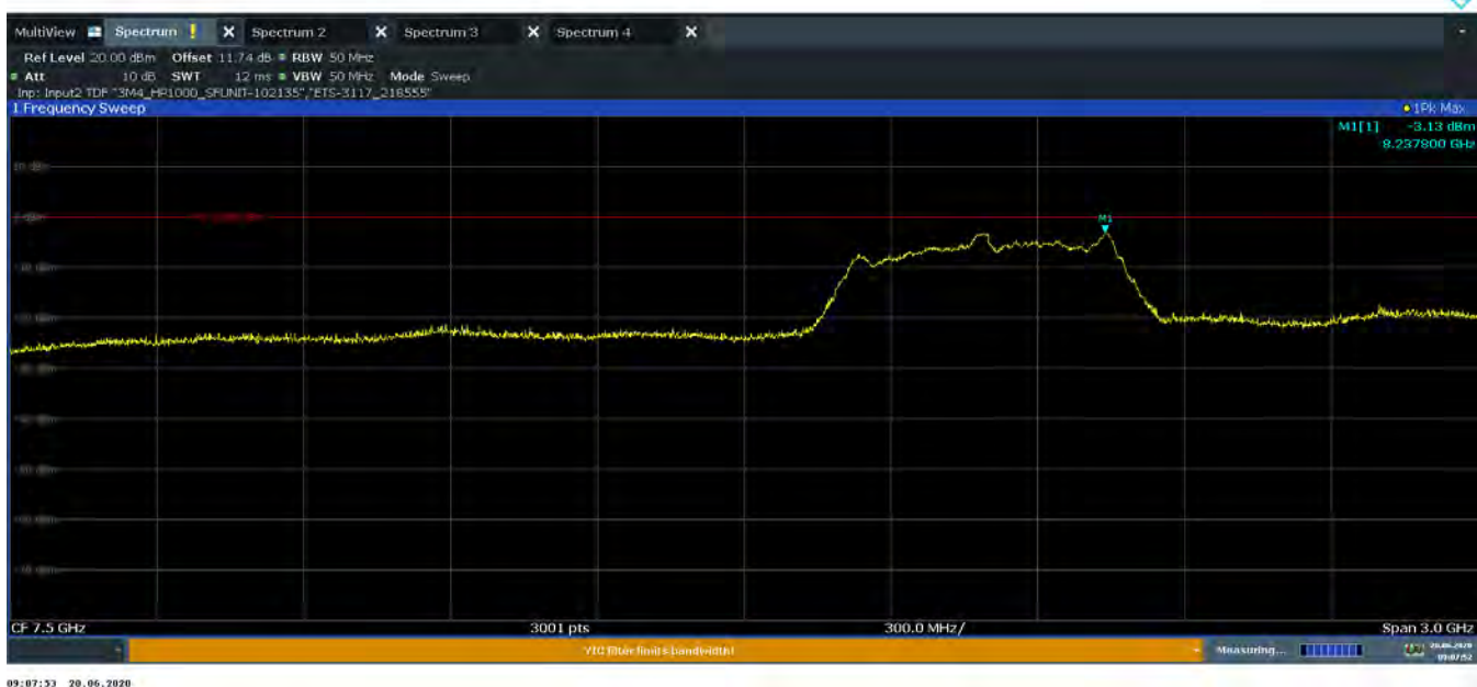
Plot 7-56. Peak Radiated Power (Ch. 9, Config 1/Payload 125)
