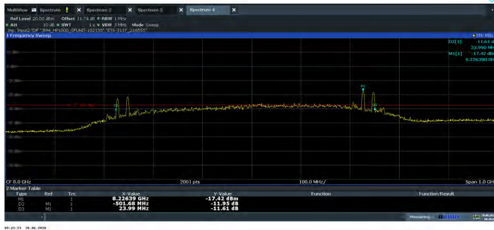
Plot 7-13. 10dBc Bandwidth (Ch. 9, Config 0/Payload 125)
