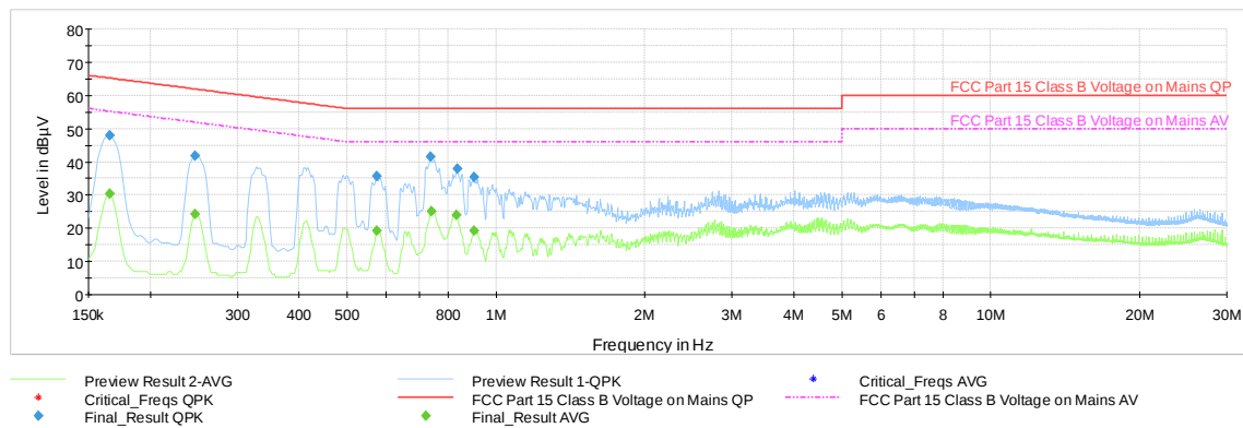
Plot 7-43. AC Line-Conducted Plot with GFSK ePA Ch.39 (L1, with WCP + AC/DC Adapter)
