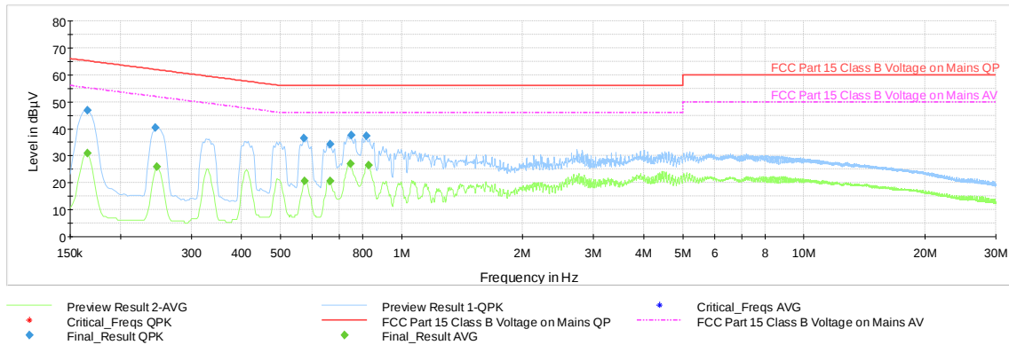
Plot 7-44. AC Line-Conducted Plot with GFSK ePA Ch.39 (N, with WCP + AC/DC Adapter)
