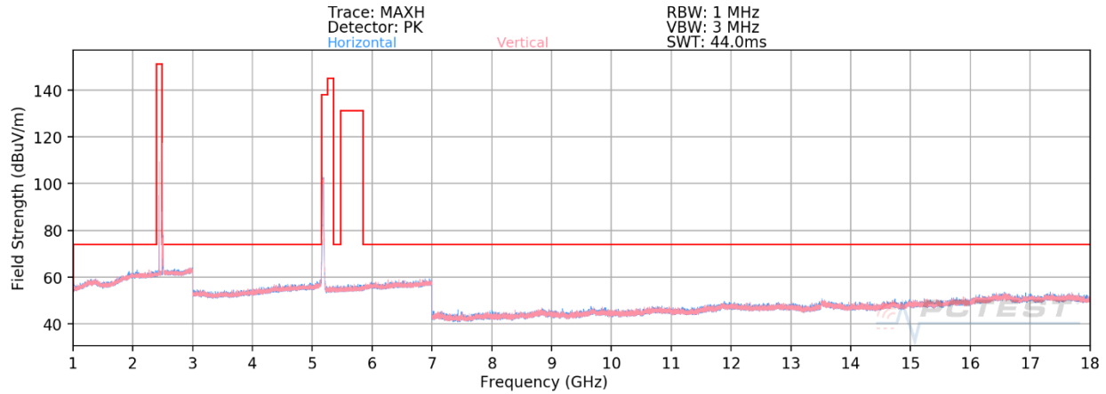
Plot 7-34. Radiated Spurious Emissions 1-18GHz (Simultaneous Transmission)
