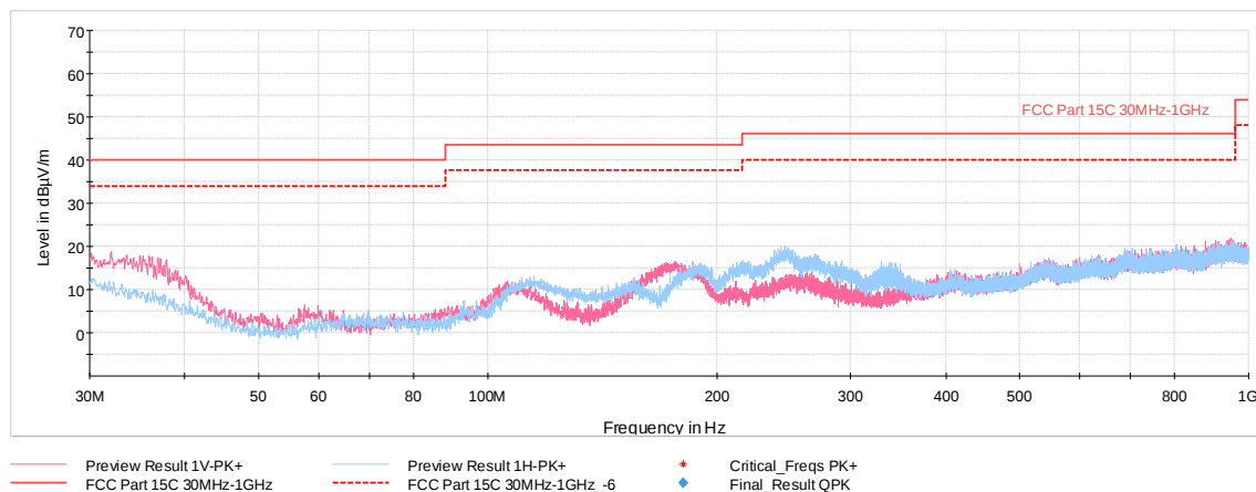
Plot 7-41. Radiated Spurious Emissions 30MHz-1GHz (GFSK ePA – Ch.39, with WCP + AC/DC Adapter)
