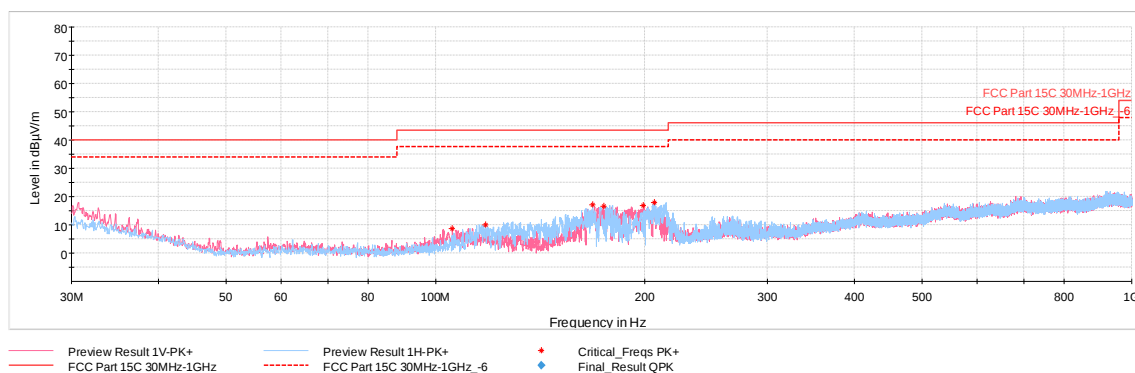
Plot 7-42. Radiated Spurious Emissions 30MHz-1GHz (Simultaneous Transmission, with WCP + AC/DC Adapter)
