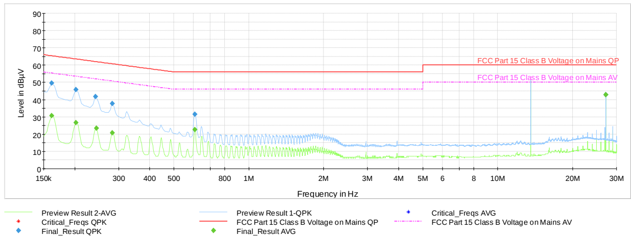
Plot 7-6. Line-Conducted Test Plot (N)
