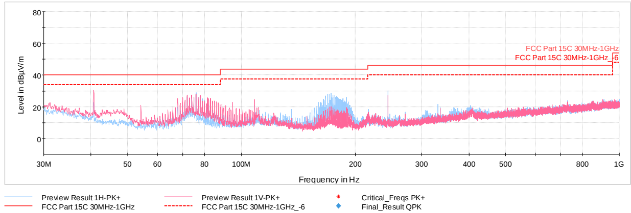
Plot 7-4. Radiated Spurious Plot 30MHz – 1GHz
