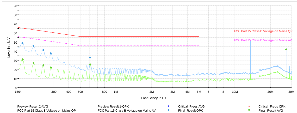
Plot 7-5. Line-Conducted Test Plot (L1)
