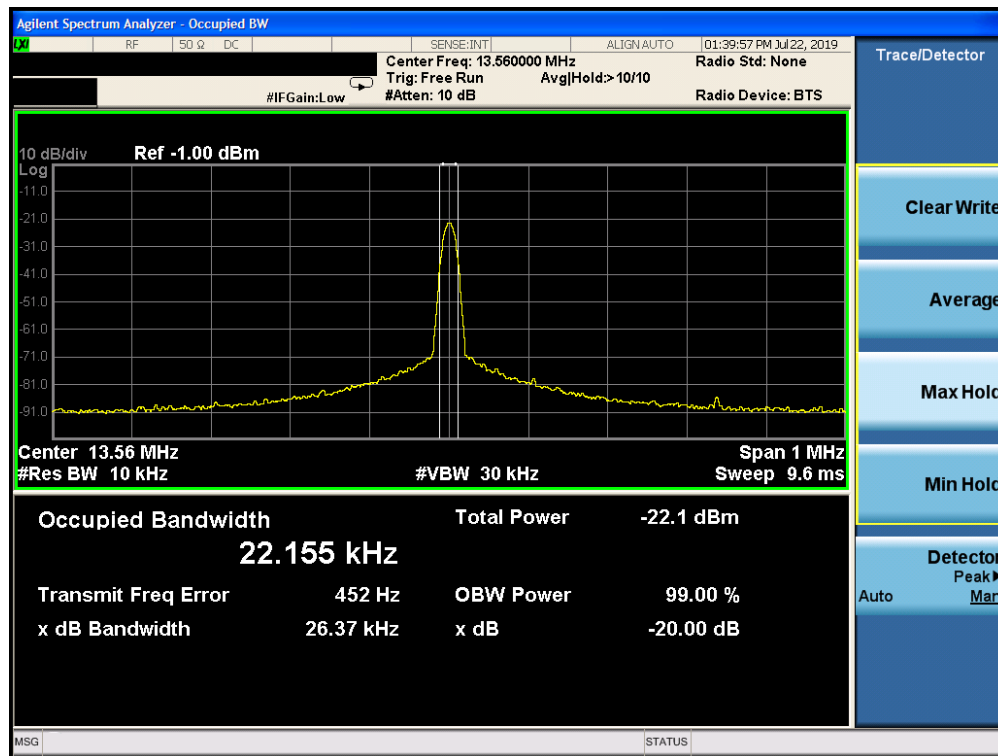
Plot 7-1. 20dB Bandwidth Plot
