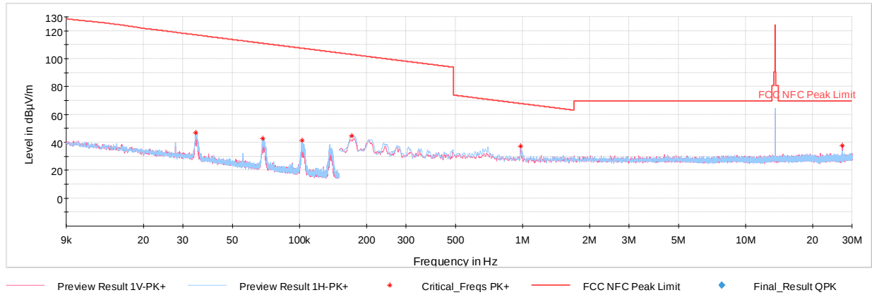
Plot 7-3. Radiated Spurious Plot 9kHz – 30MHz
