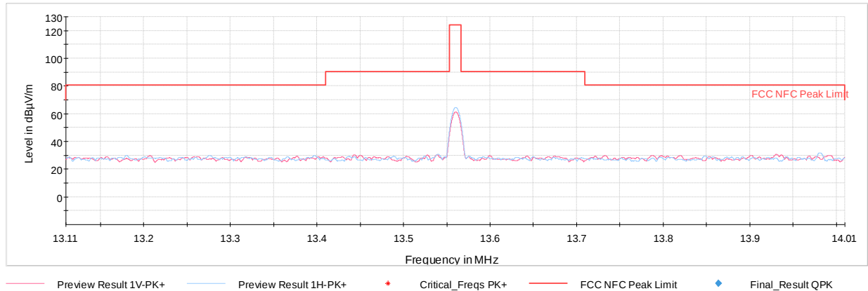
Plot 7-2. In Band Radiated Spurious Plot
