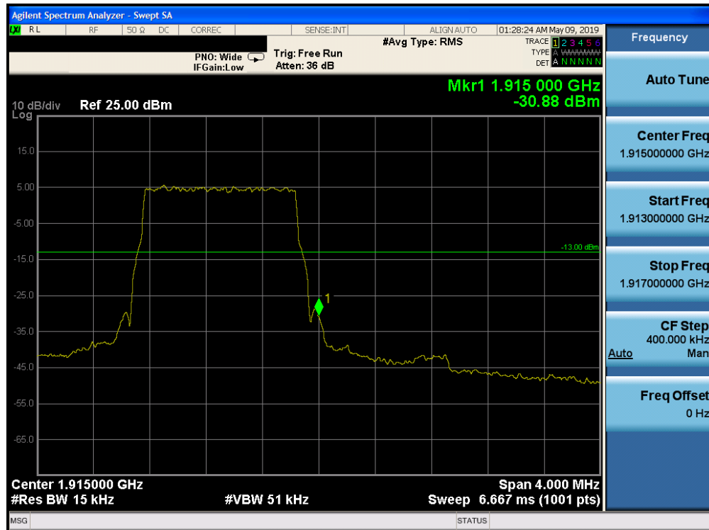
Plot 7-160. Upper Band Edge Plot (Band 25 - 1.4MHz QPSK - Full RB Configuration)
