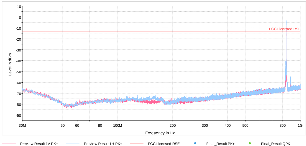
Plot 7-44. Radiated Spurious Plot Below 1GHz (Cellular WCDMA Mode – Ch. 4183)
